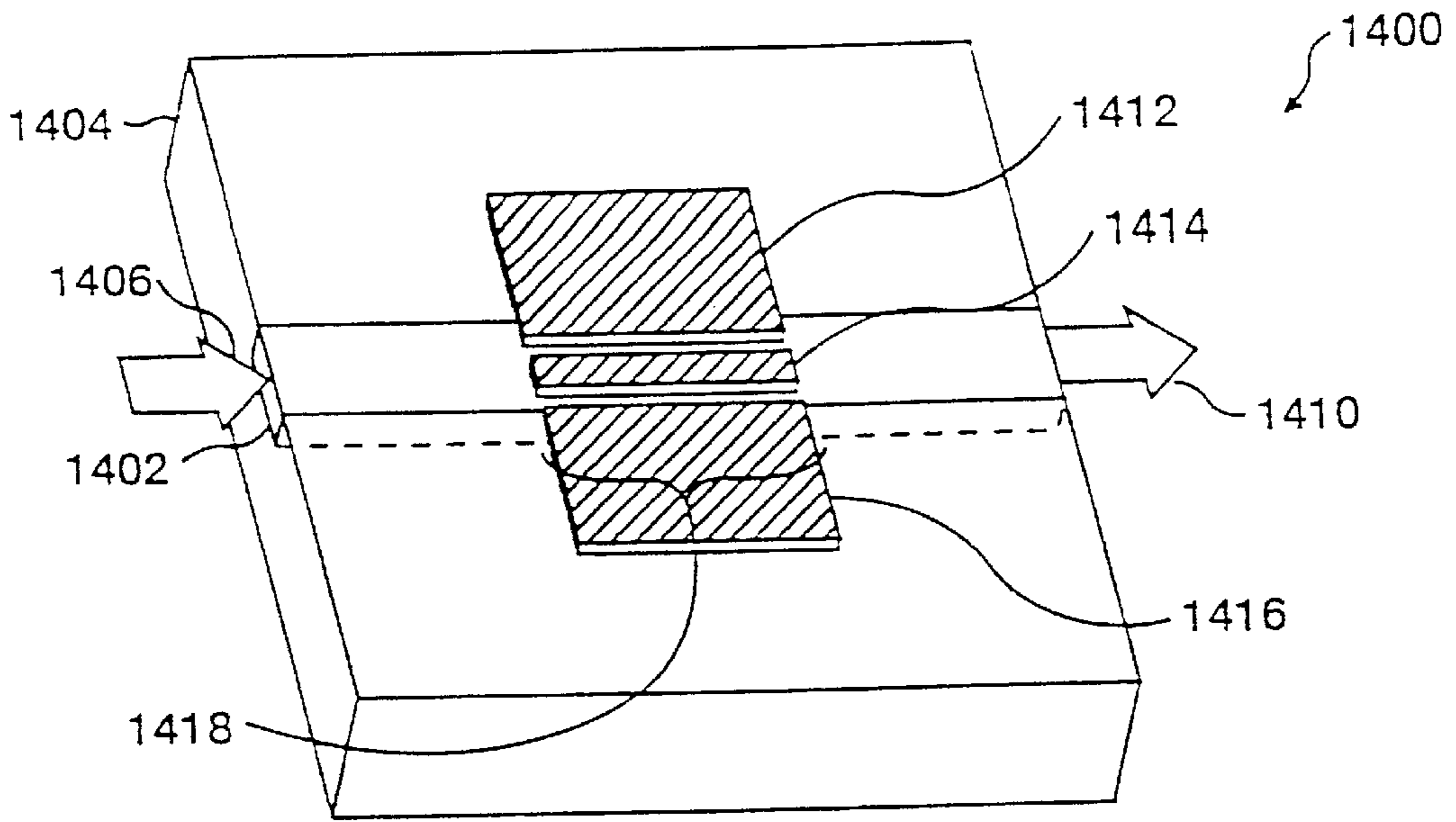
Figure 50 (Prior Art)
