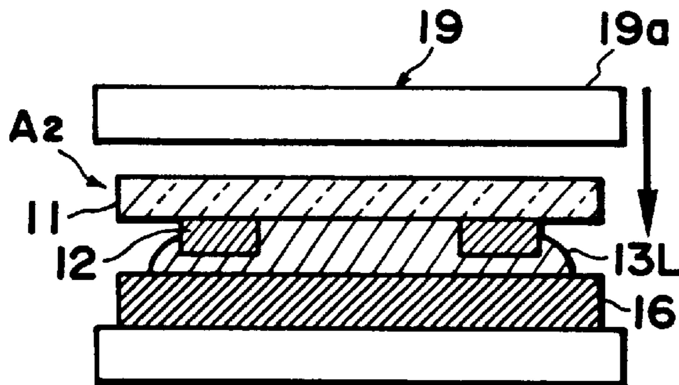
FIG. 3C PRIOR ART
