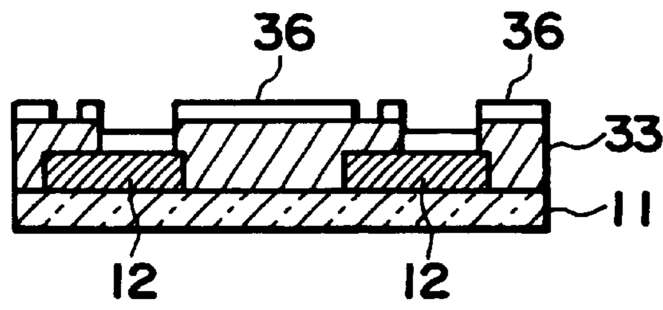
FIG. 7 PRIOR ART
