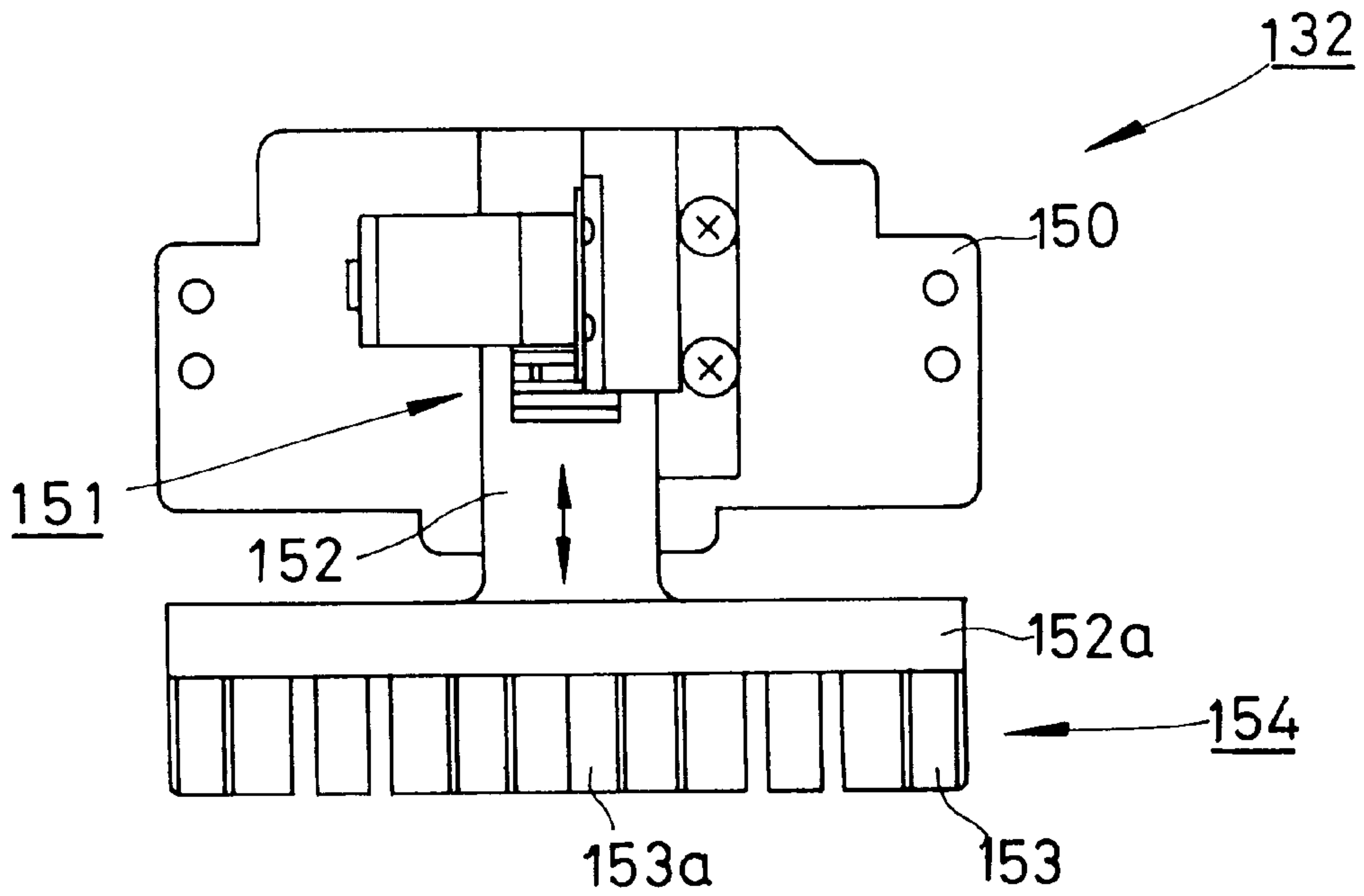
FIG. 35 (PRIOR ART)
