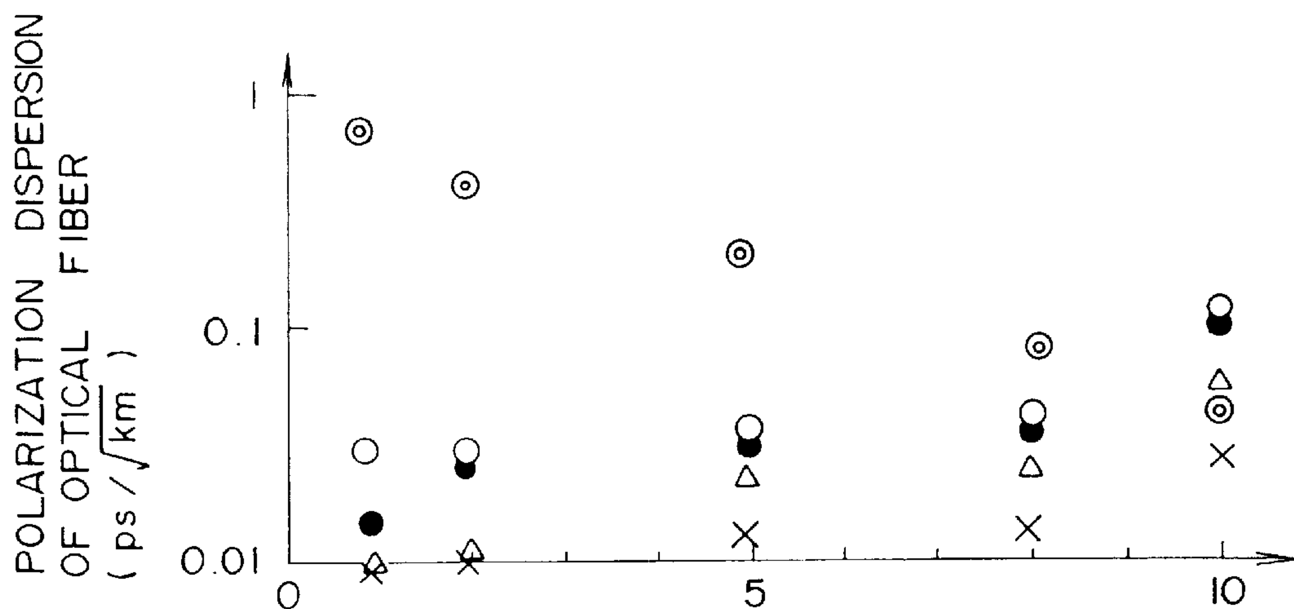
GAP d (mm) BETWEEN PAIR OF GUIDE ROLLERS FOR OPTICAL FIBER SWING SUPPRESSION
