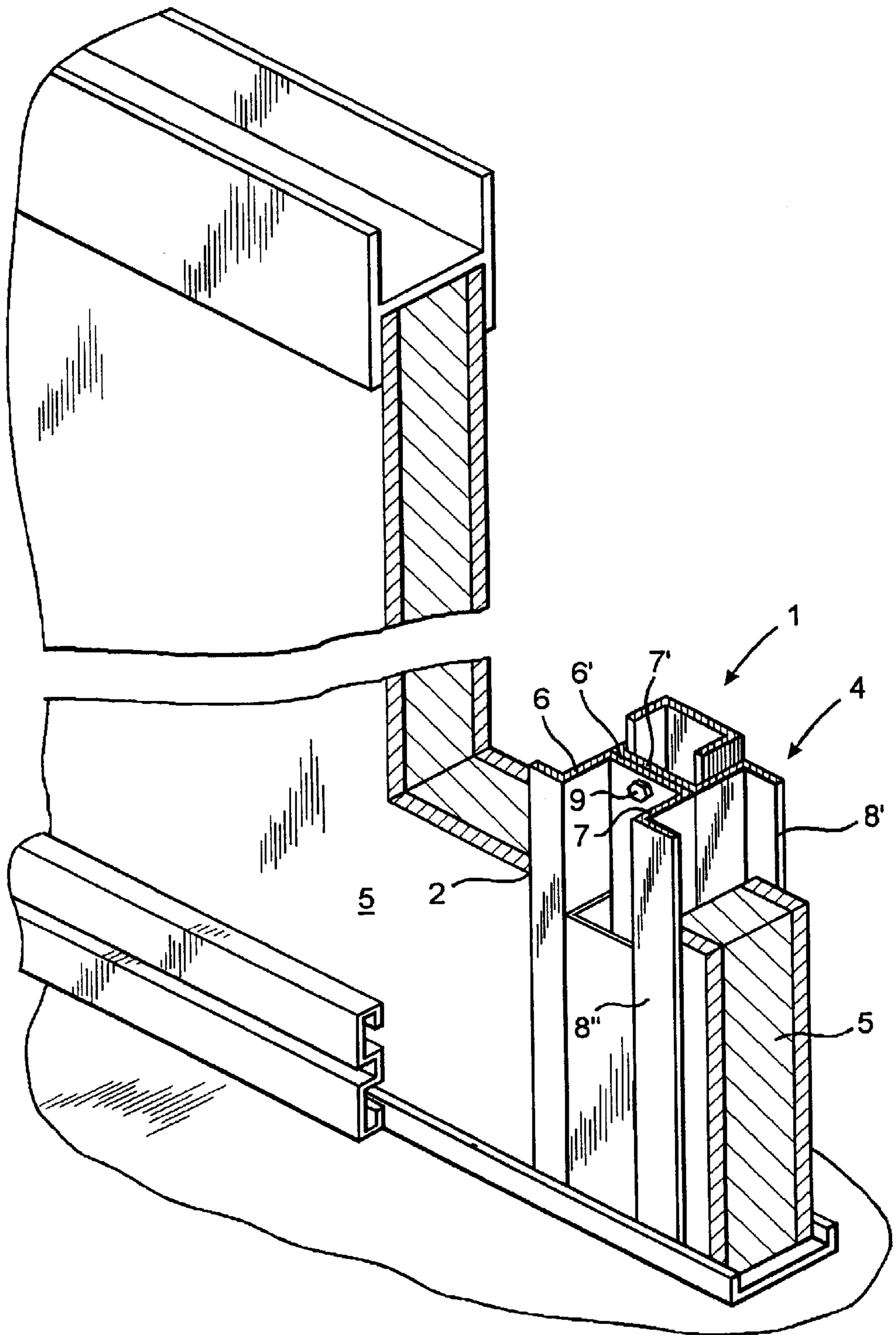
FIG. 1 PRIOR ART
