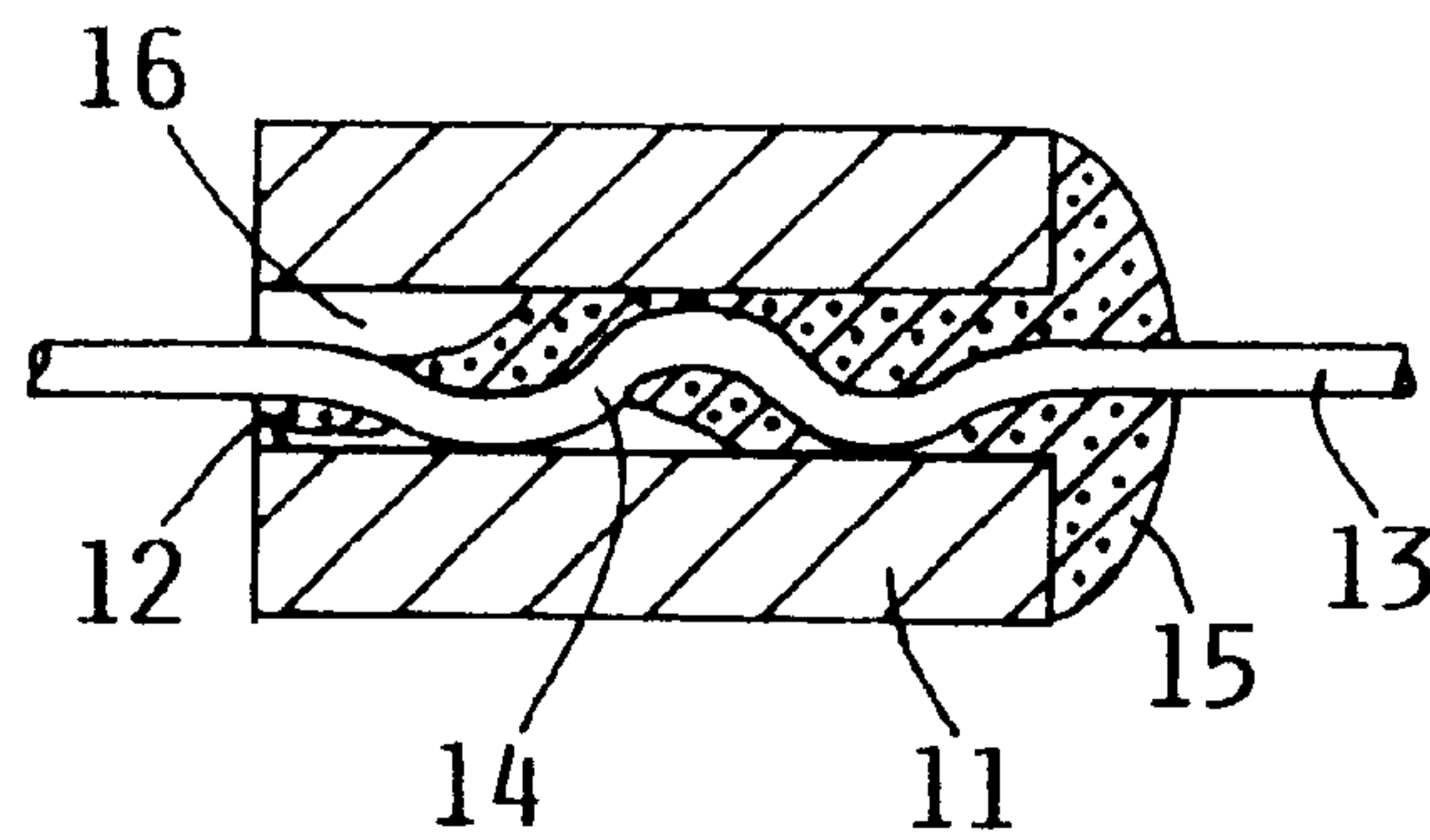
FIG. 6 (PRIOR ART)
