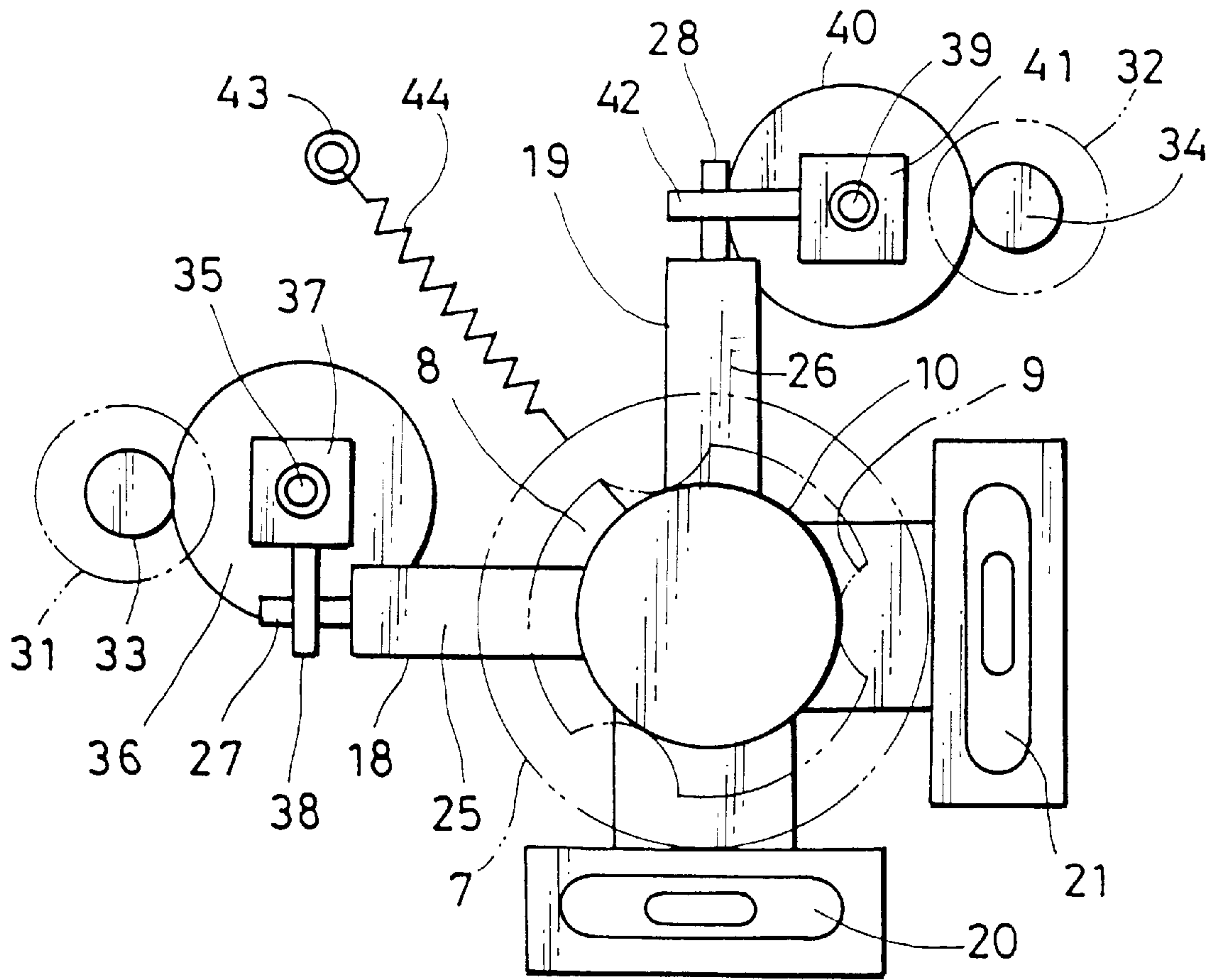
FIG. 30 PRIOR ART
