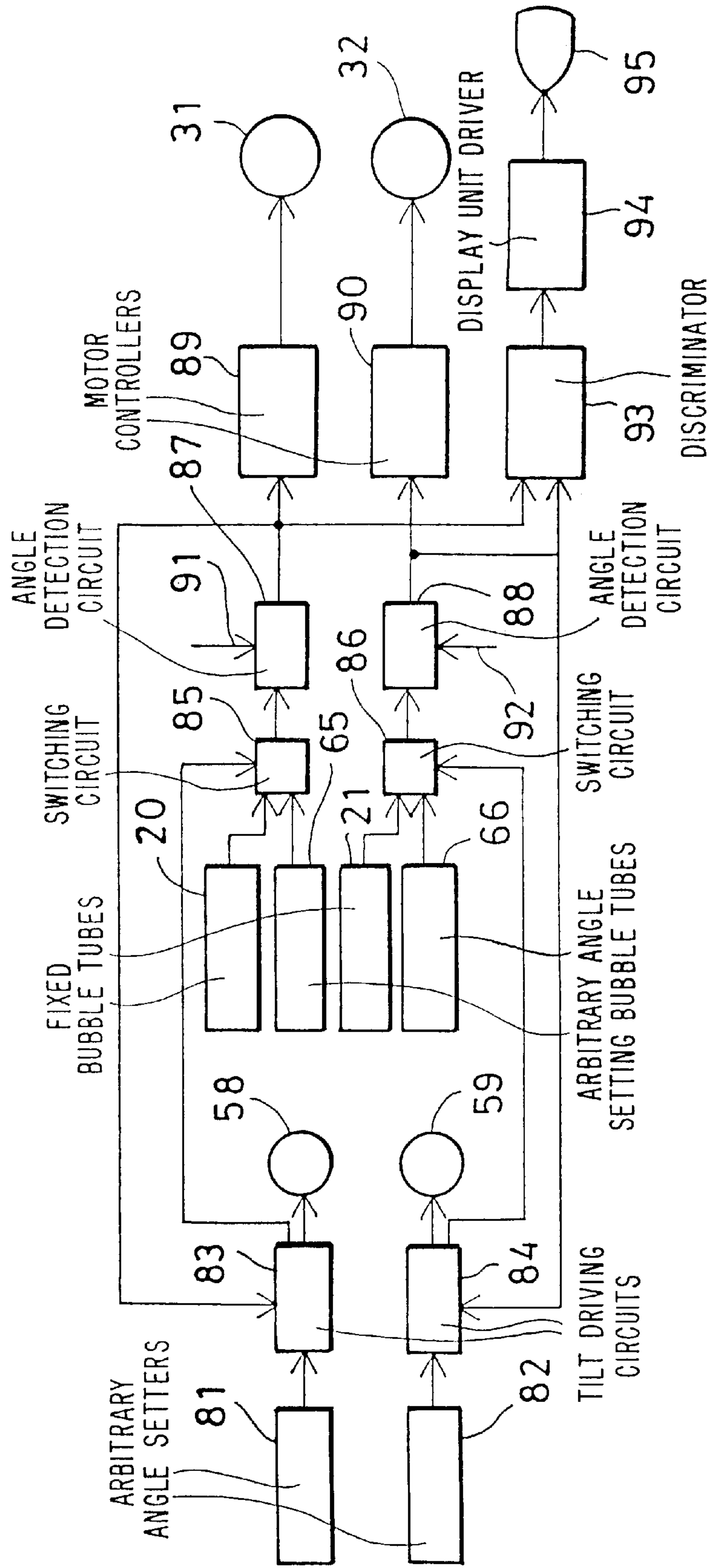
FIG. 33 PRIOR ART
