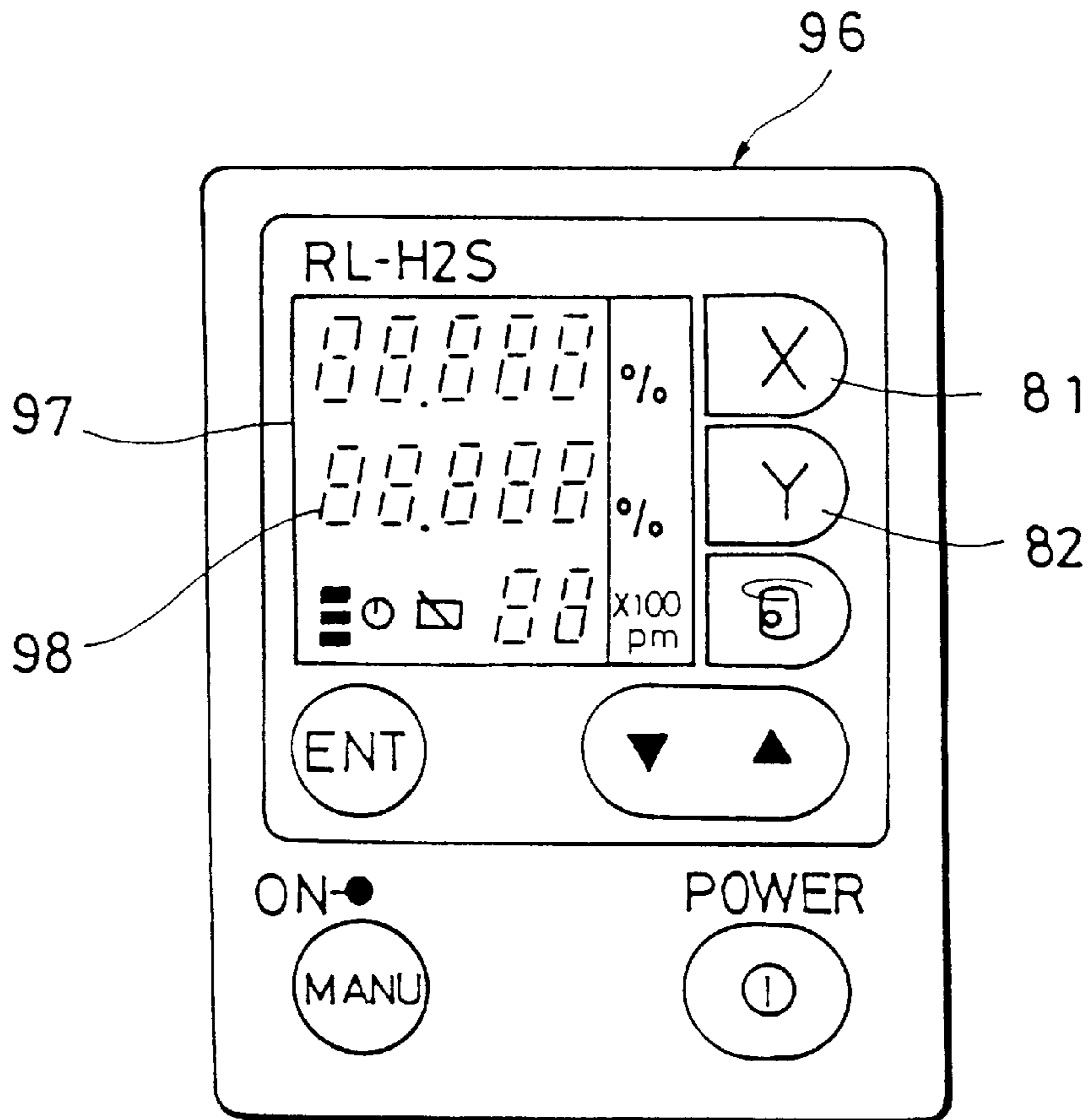
FIG. 35 PRIOR ART
