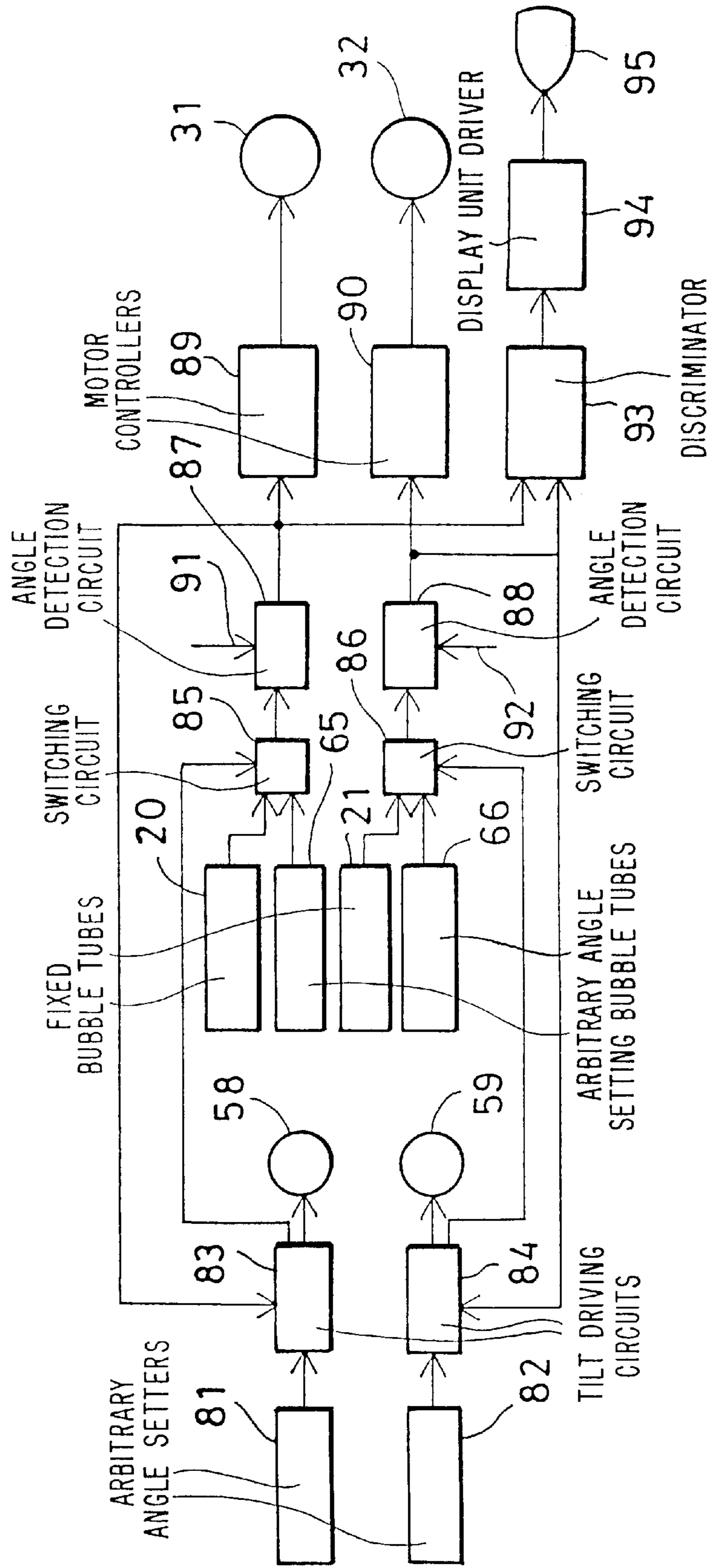
FIG. 33 PRIOR ART
