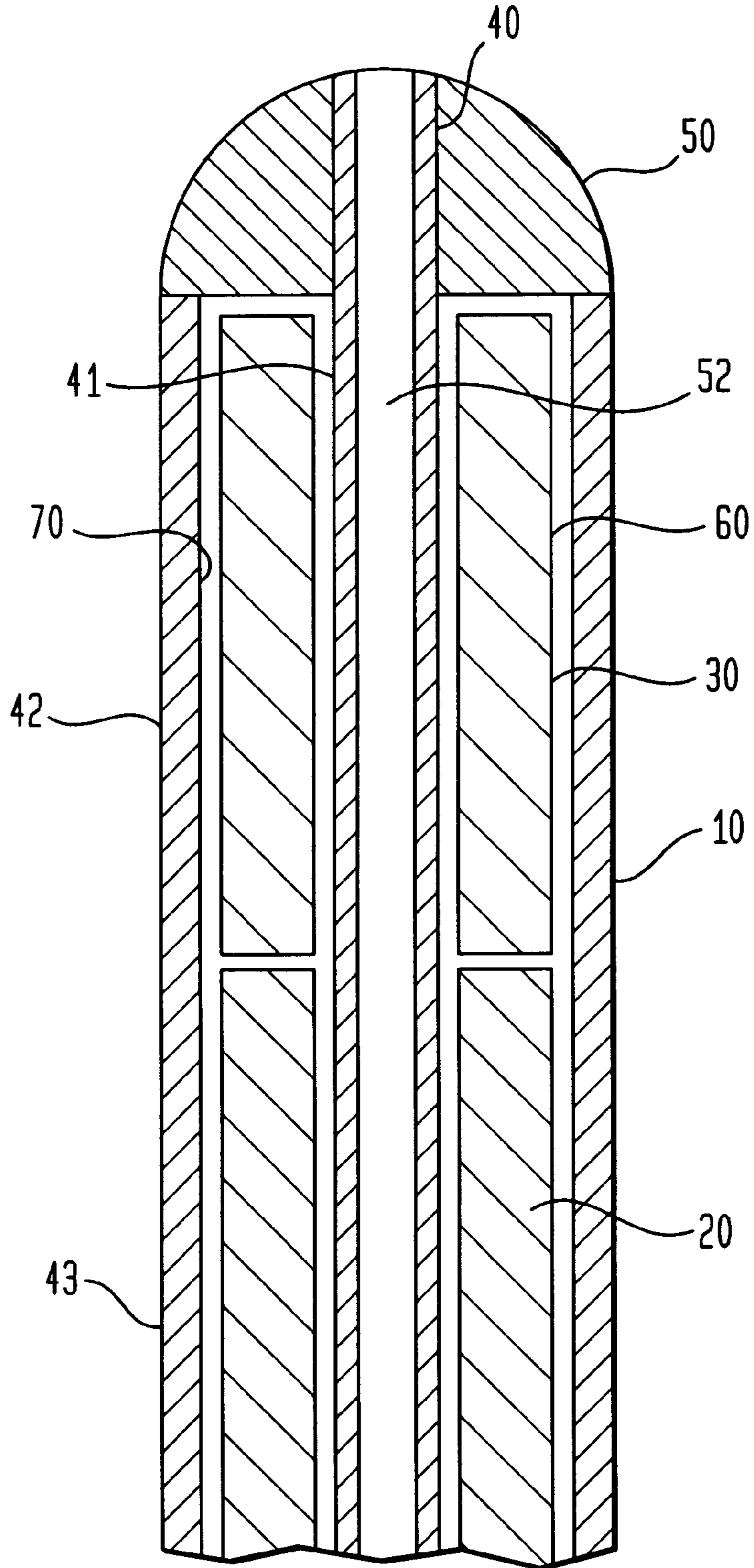
FIG. 1 (PRIOR ART)
