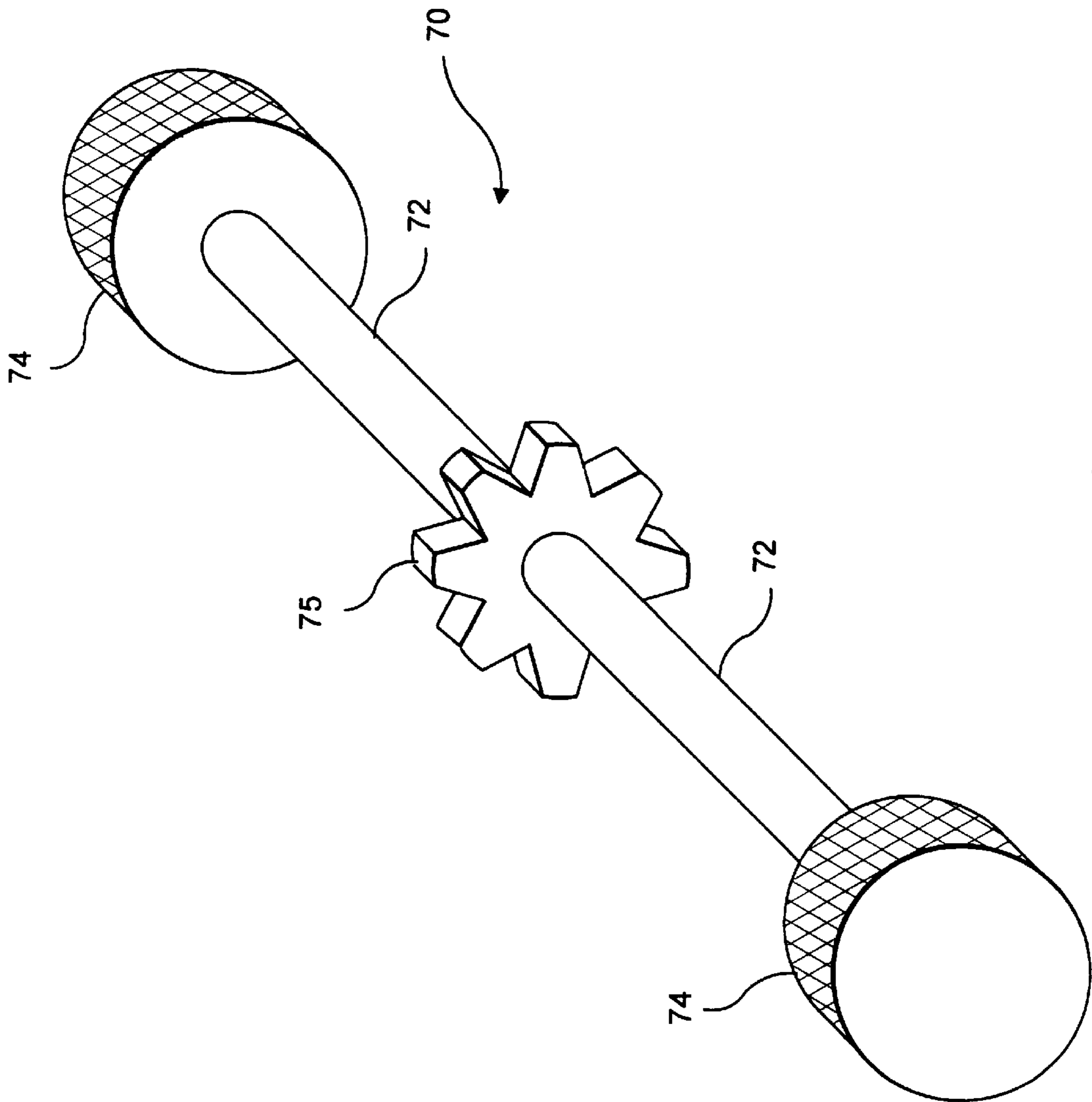
FIG. 10 PRIOR ART
