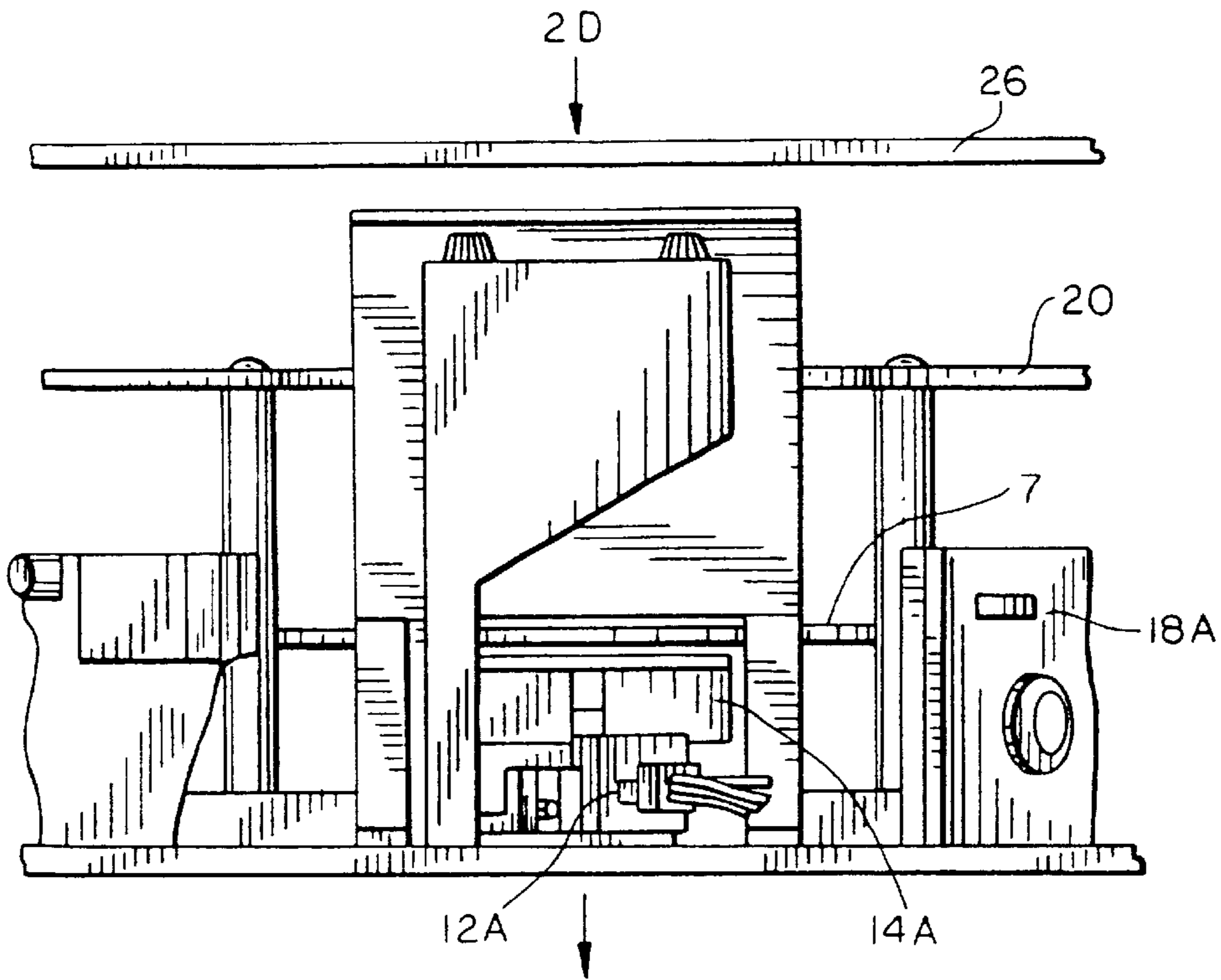
2D FIG. 2C
