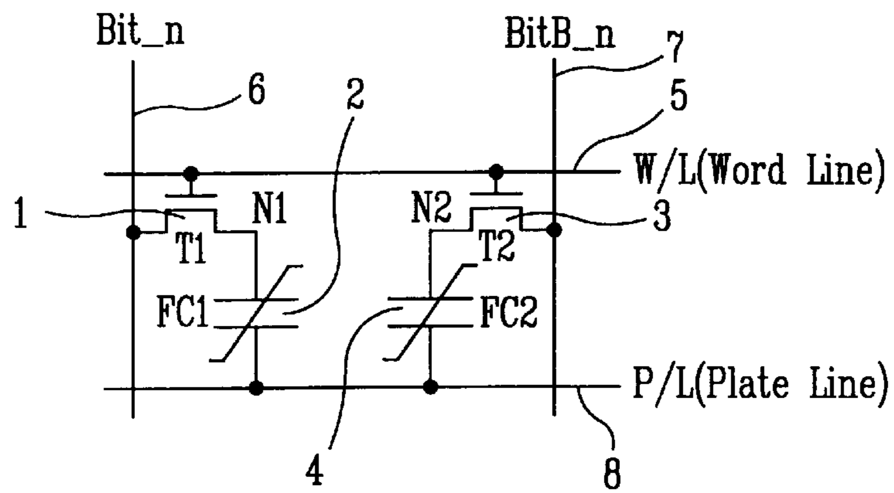
FIG.3 Related Art
