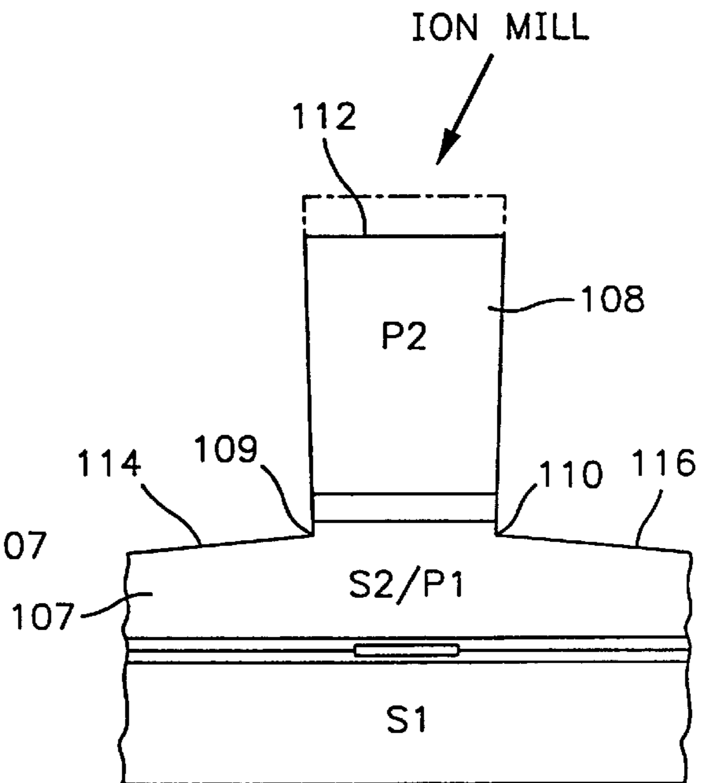
FIG. 9 (PRIOR ART)
