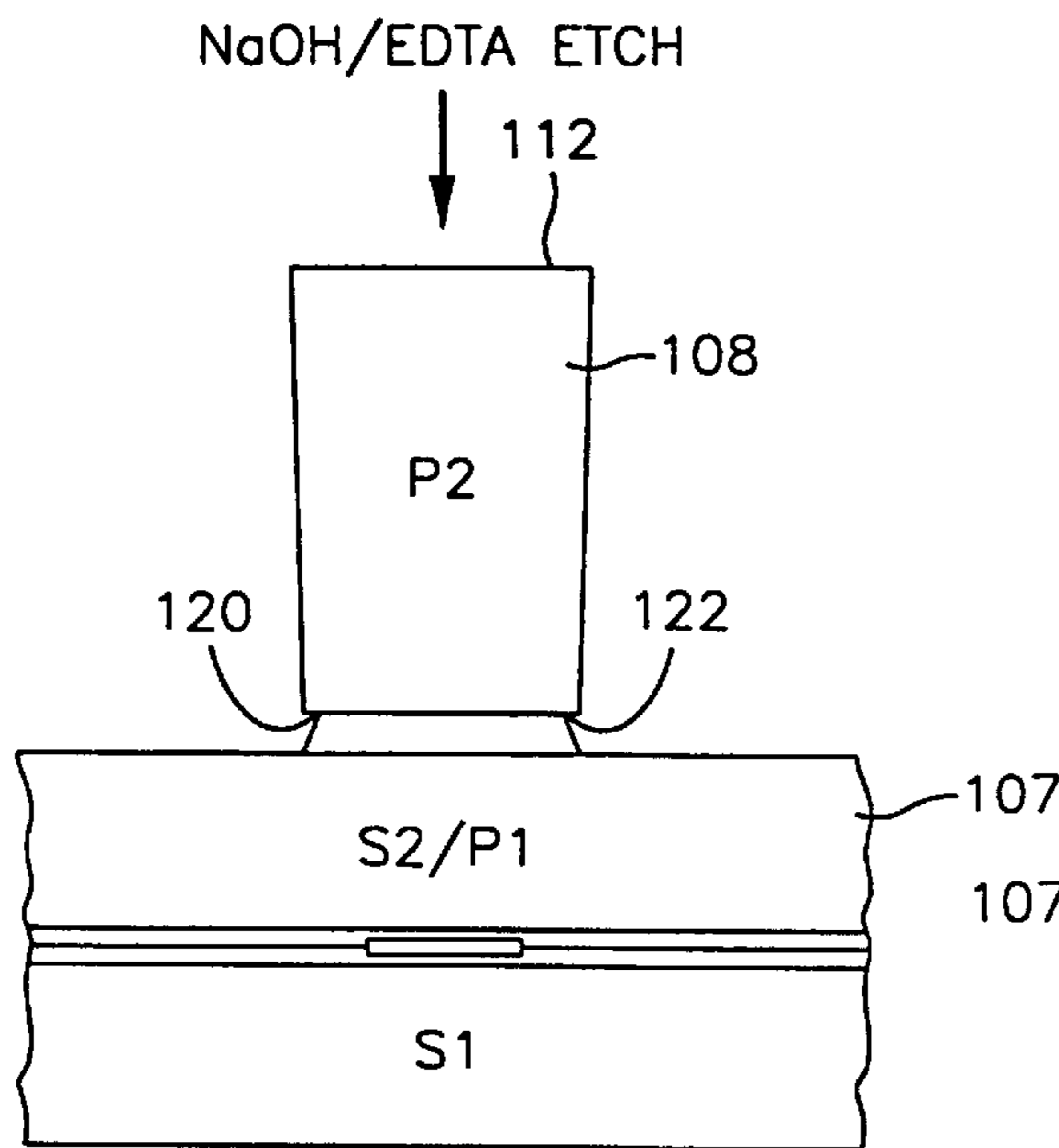
FIG. 10 (PRIOR ART)
