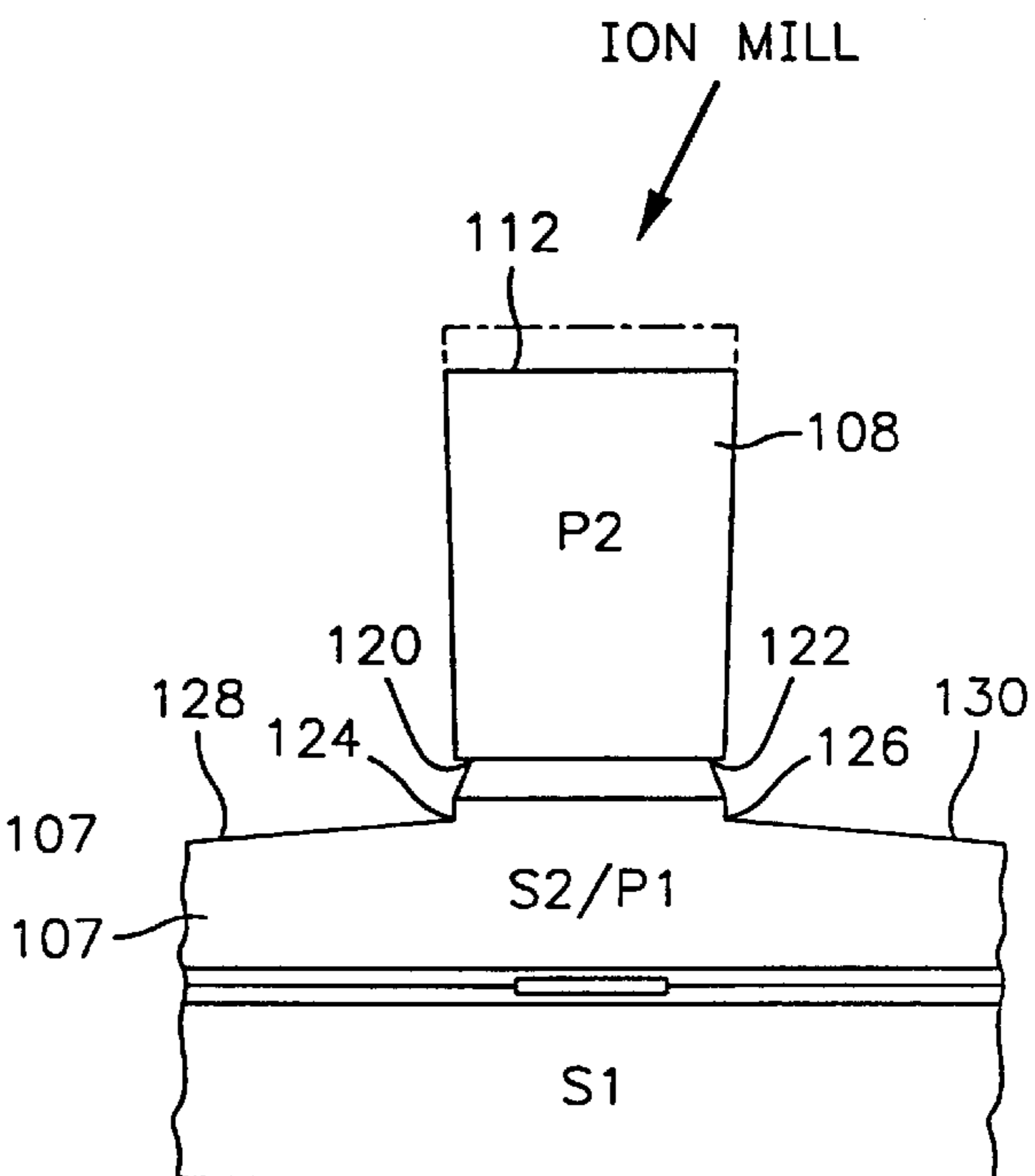
FIG. 11 (PRIOR ART)
