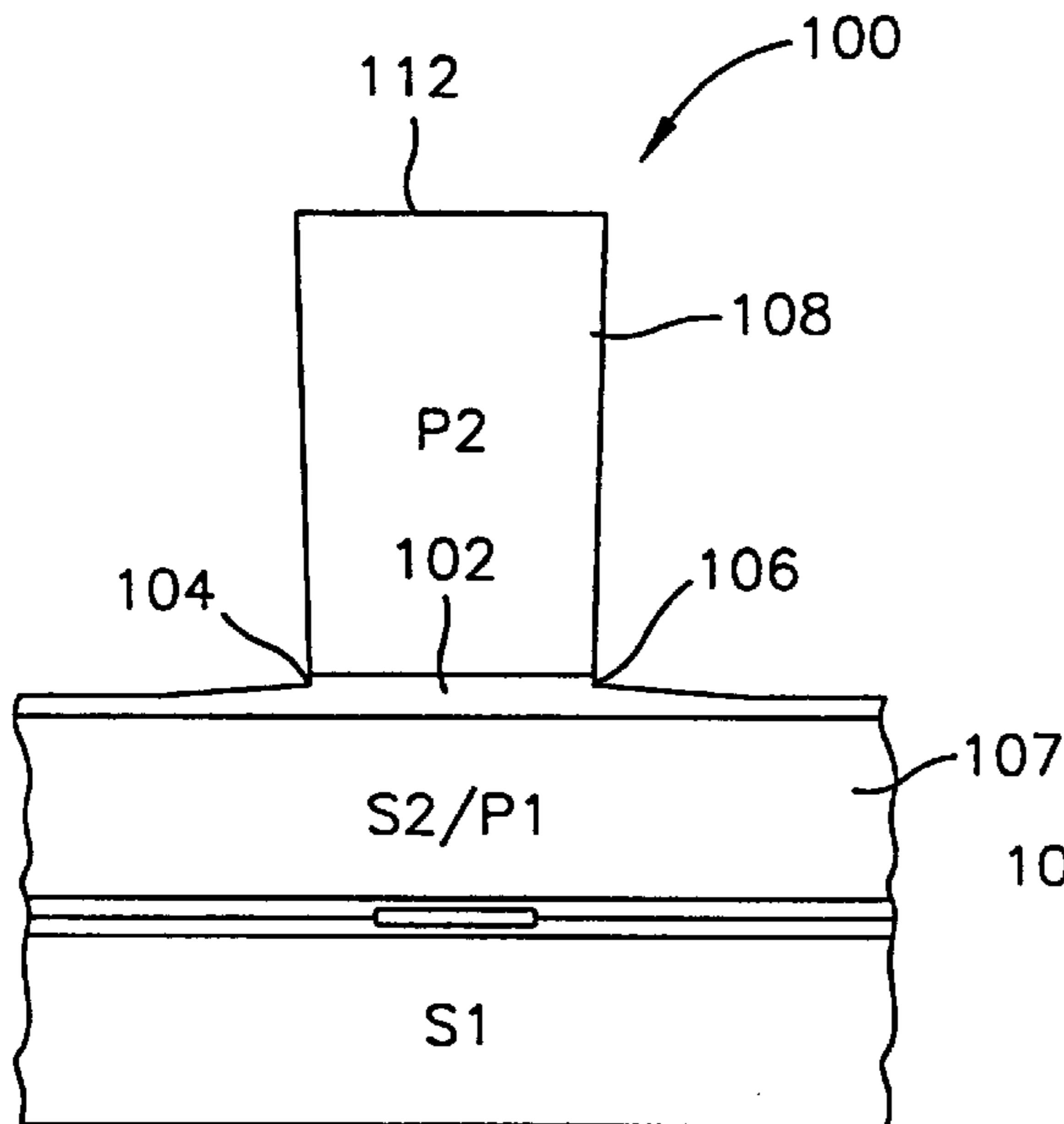
FIG. 8 (PRIOR ART)
