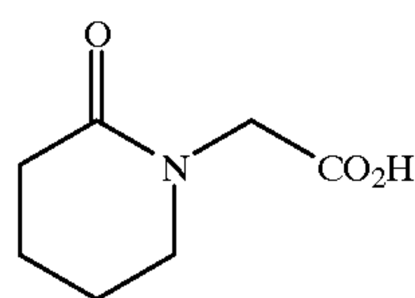
1-Carboxymethyl-2-piperdone
