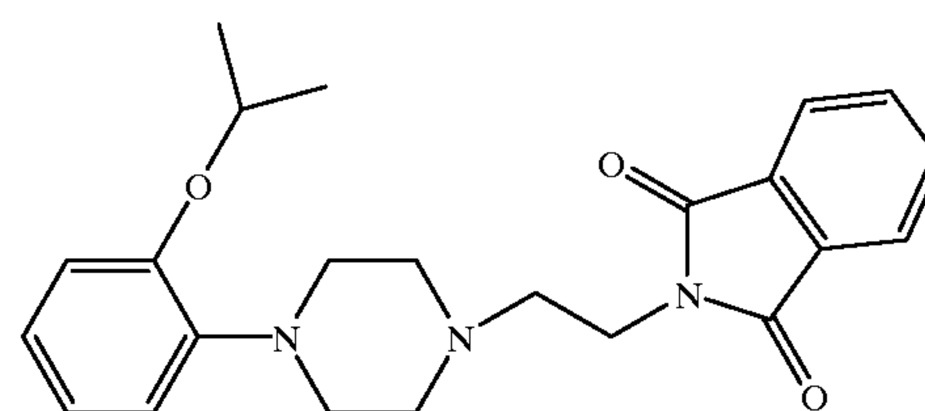
1-(2-phthalimidoethyl)-4-(2-isopropoxyphenyl) piperazine
