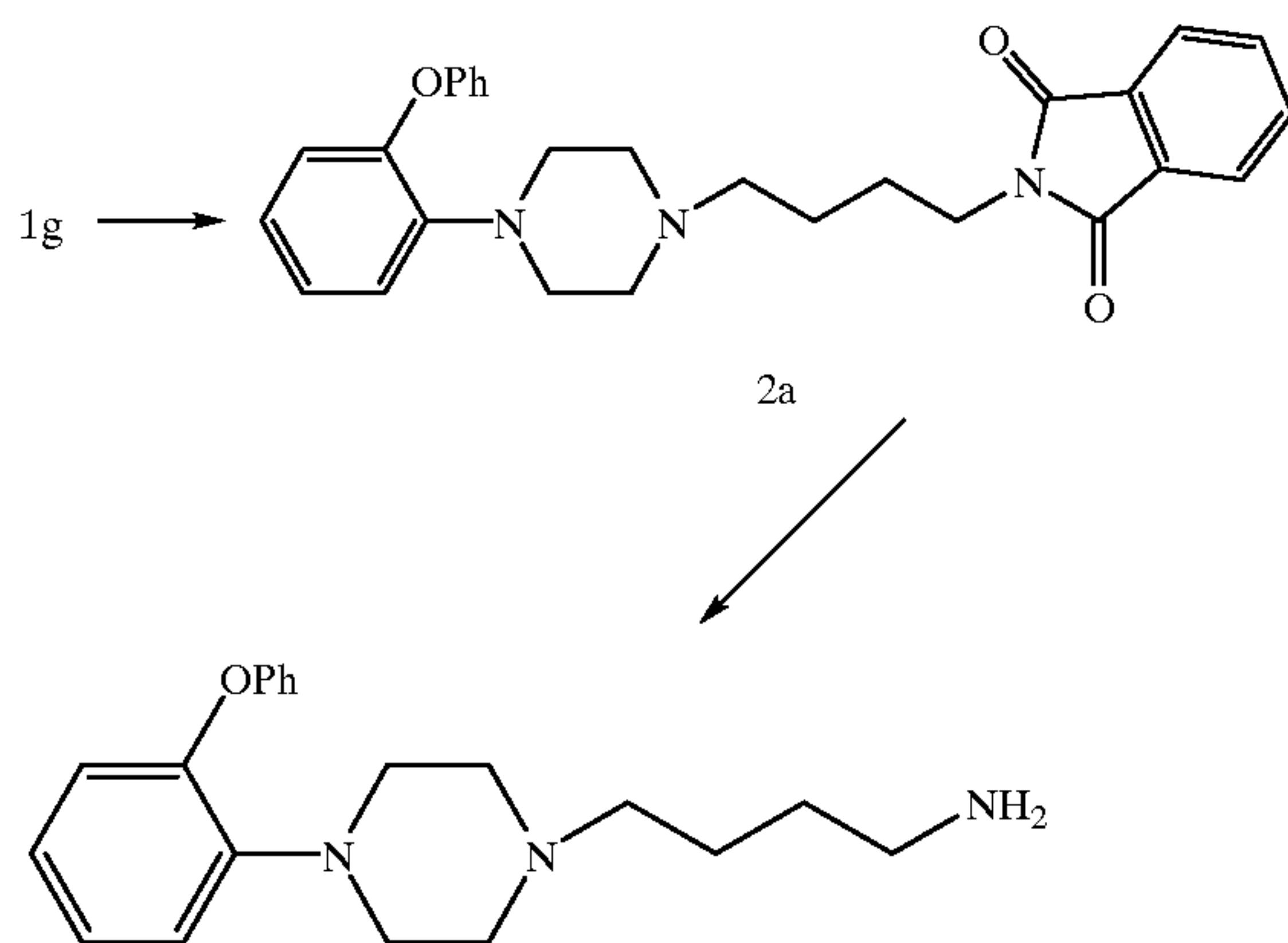
Scheme 2
