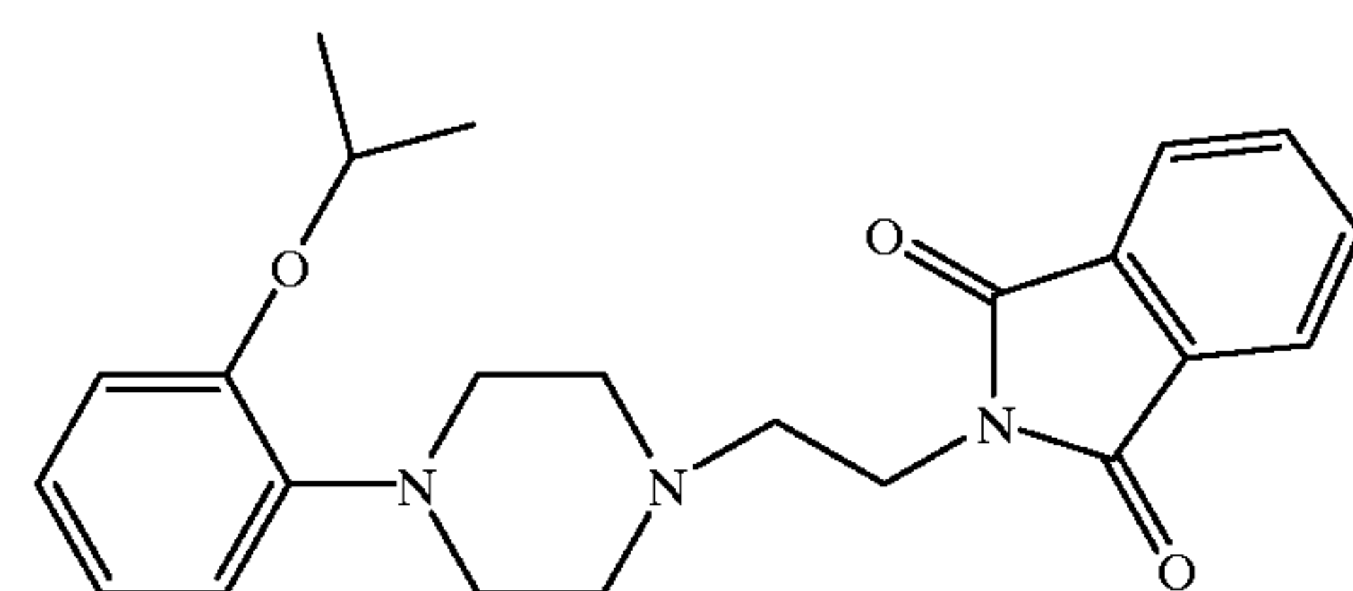
1-(2-phthalimidoethyl)-4-(2-isopropoxyphenyl) piperazine
