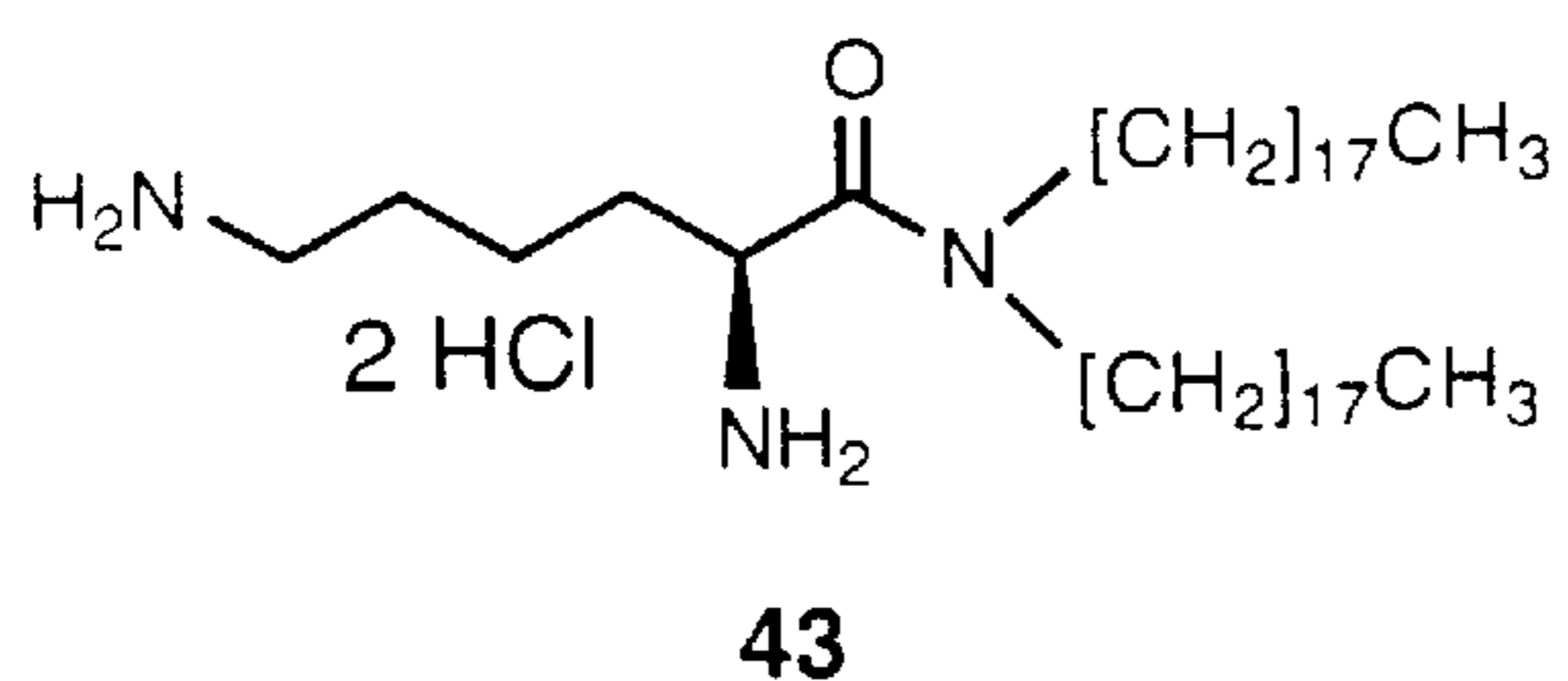
N,N-dioctadecyllysineamide diHCl salt
