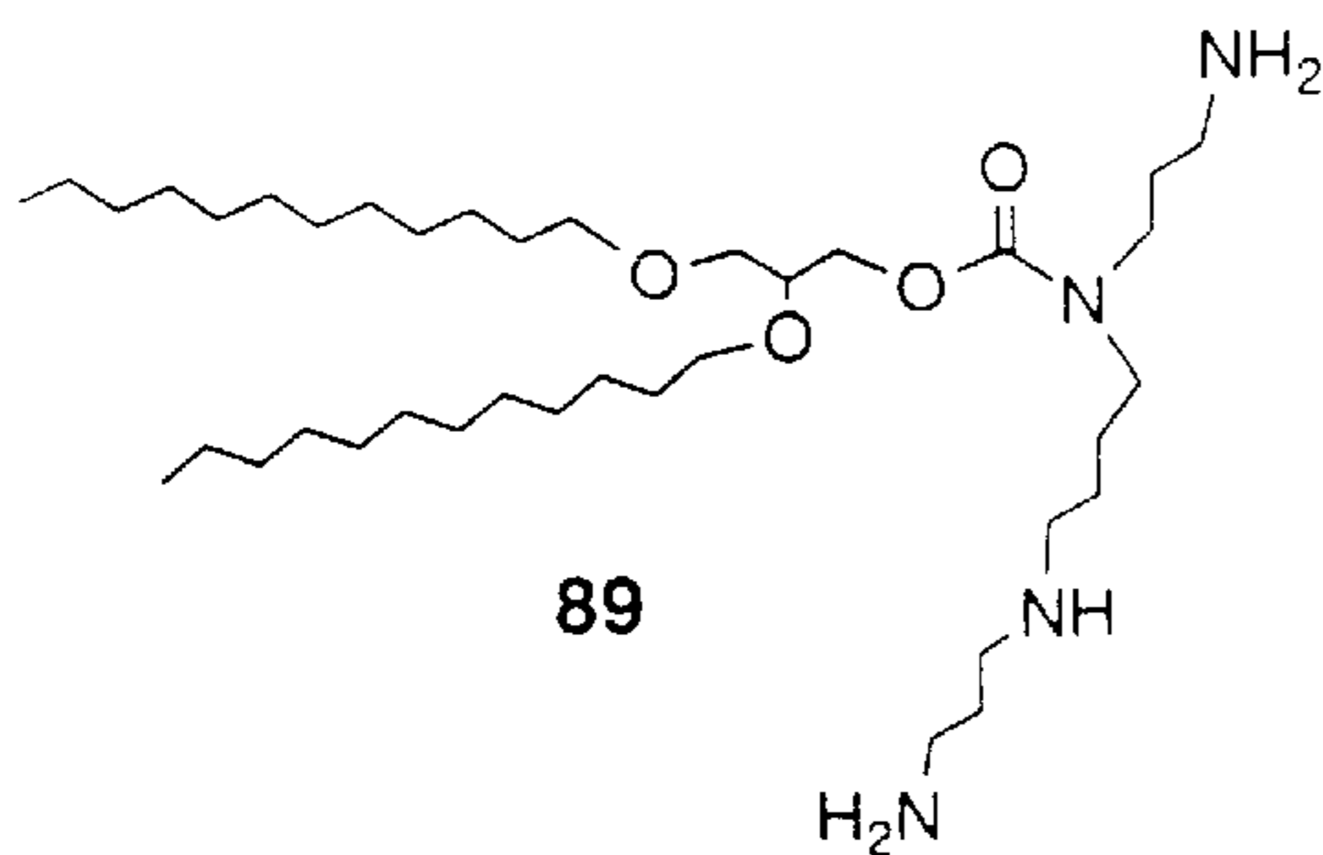
1-(N 4 -spermine)-2,3-dilaurylglycerol carbamate
