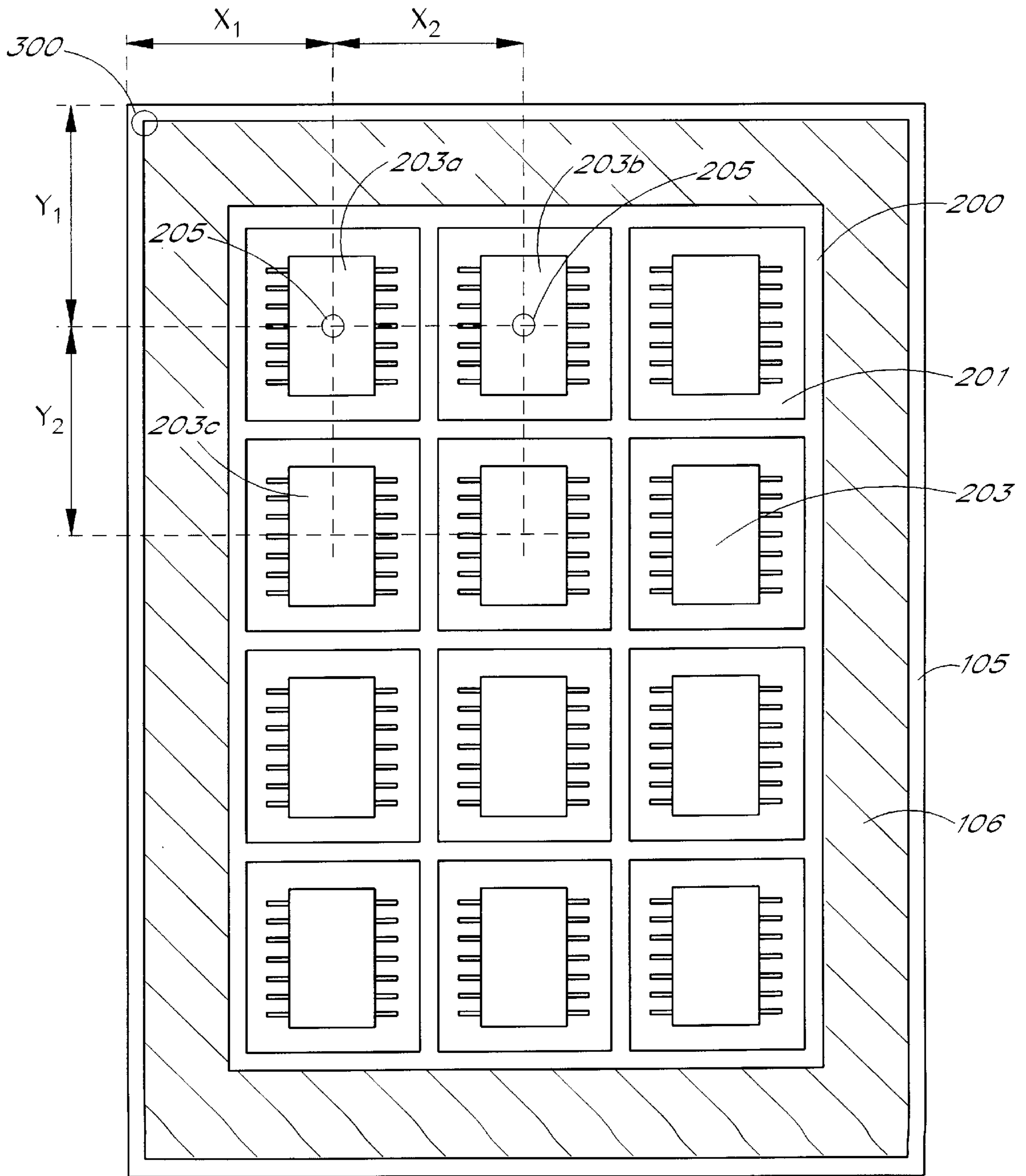
FIG. 4 (PRIOR ART)
