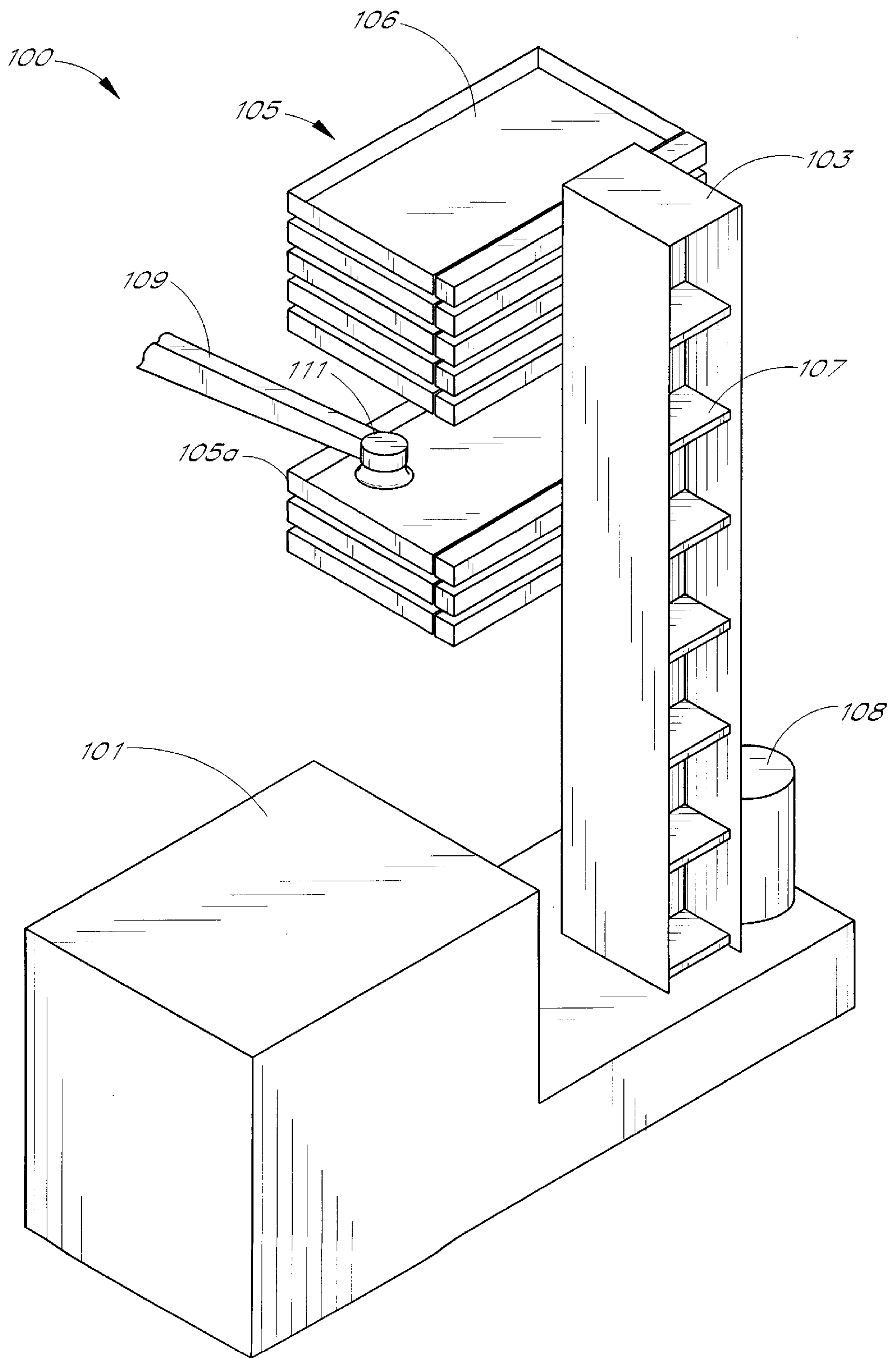
FIG. 1 (PRIOR ART)
