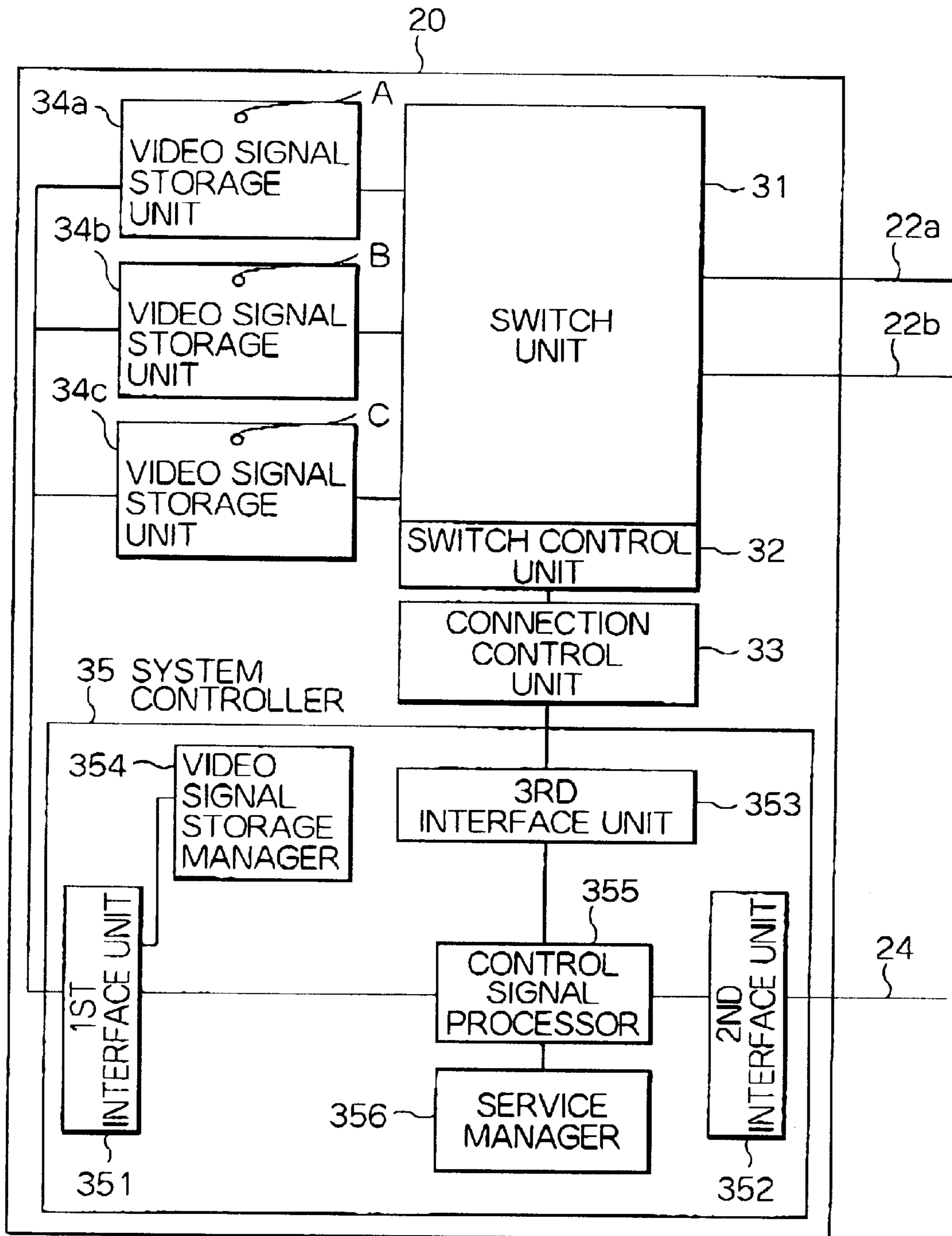
FIG. 2 PRIOR ART
