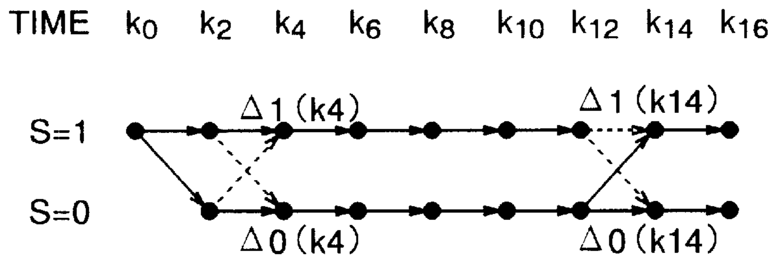
TRELLIS DIAGRAM 1
