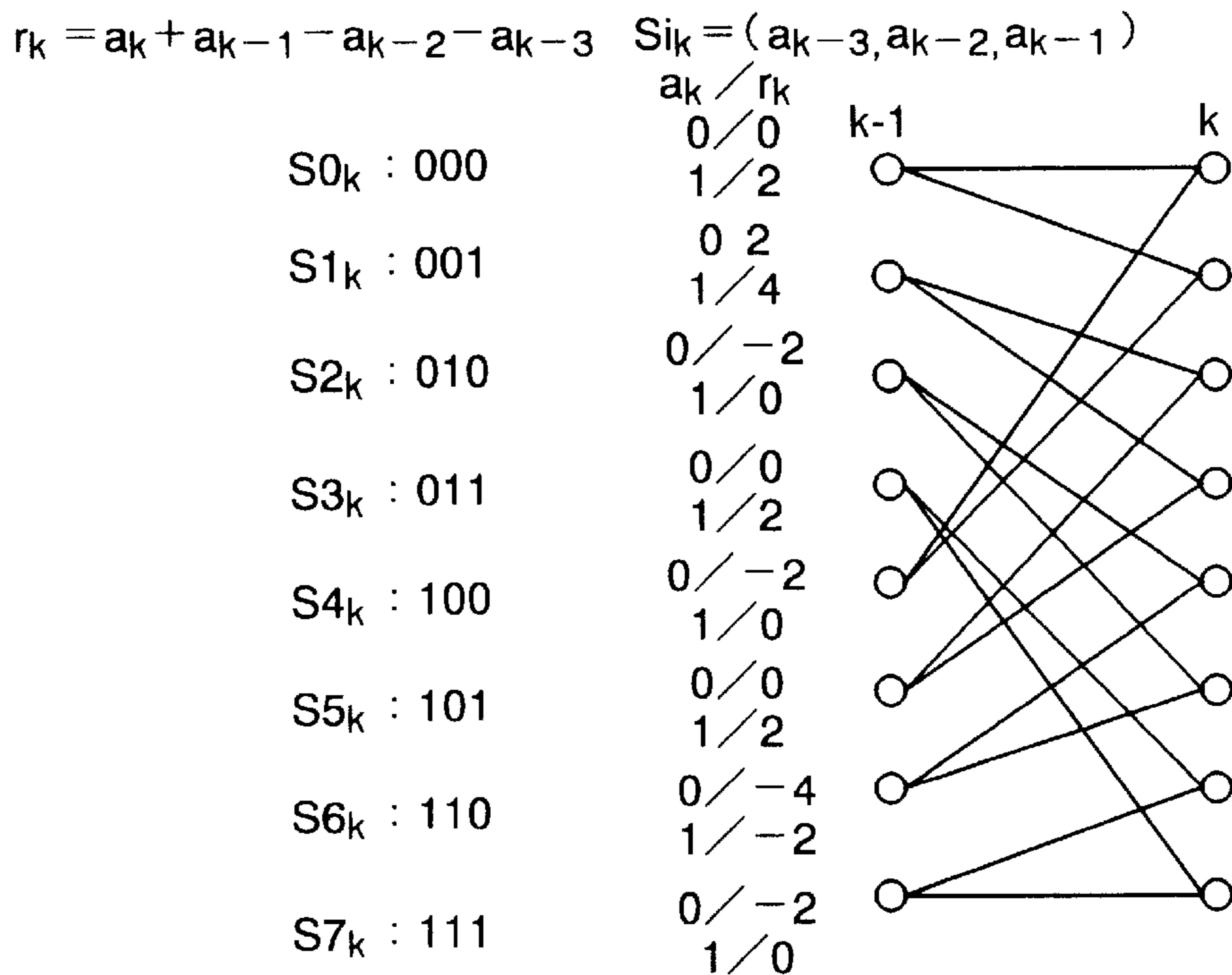
EPRML TRELLIS DIAGRAM
