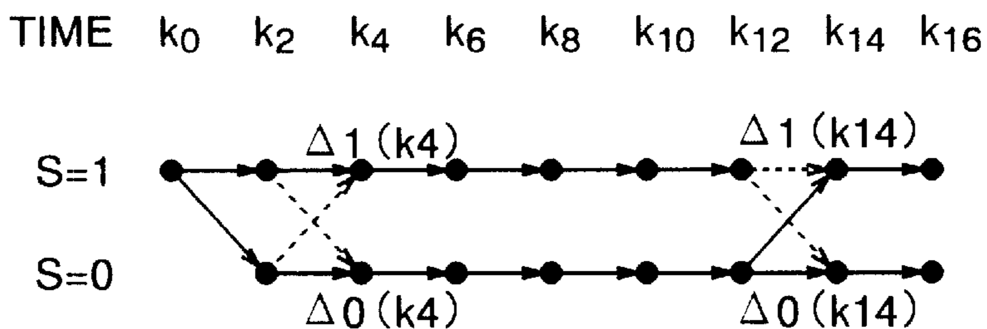
TRELLIS DIAGRAM 1
