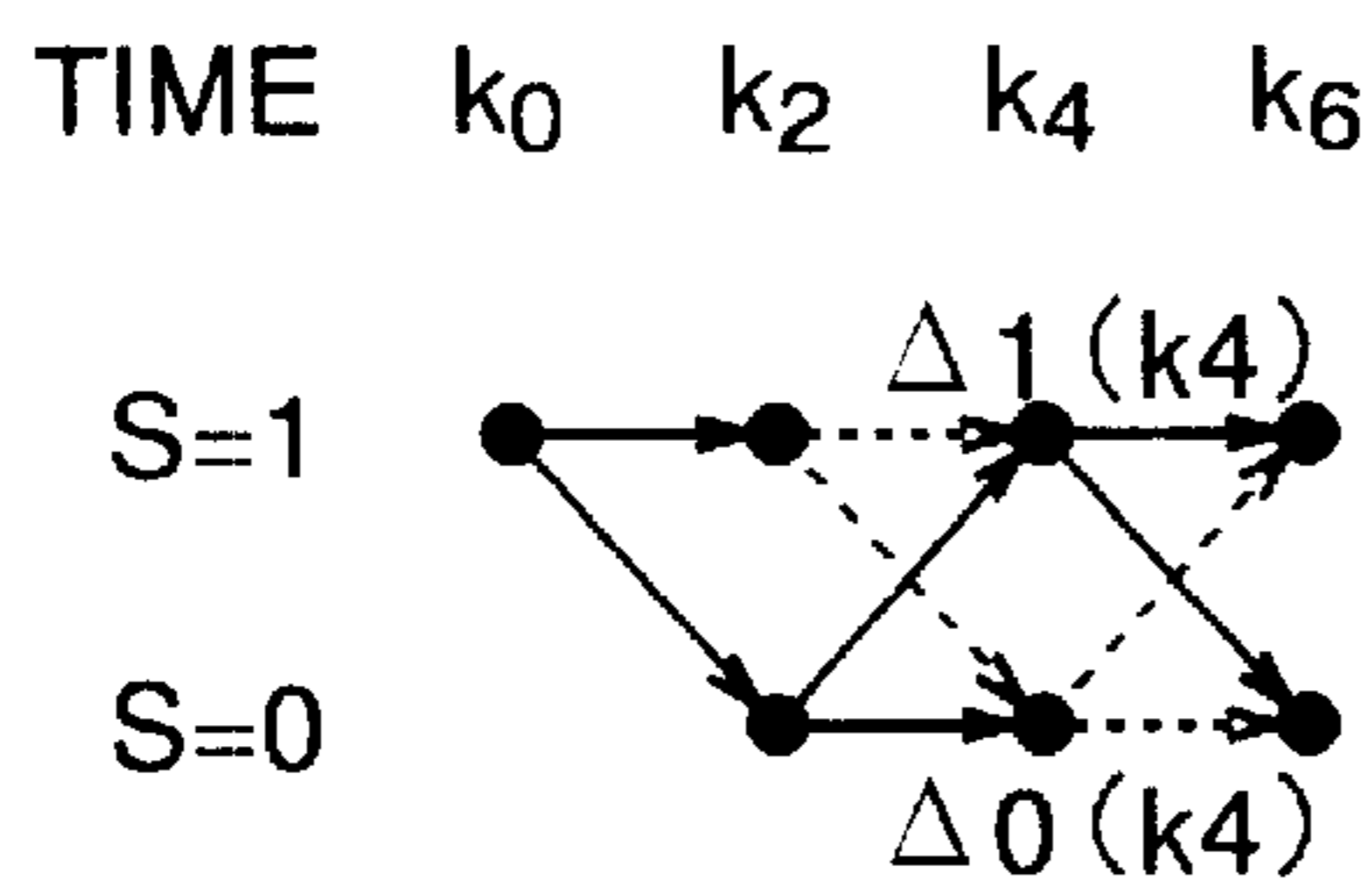
TRELLIS DIAGRAM 2
