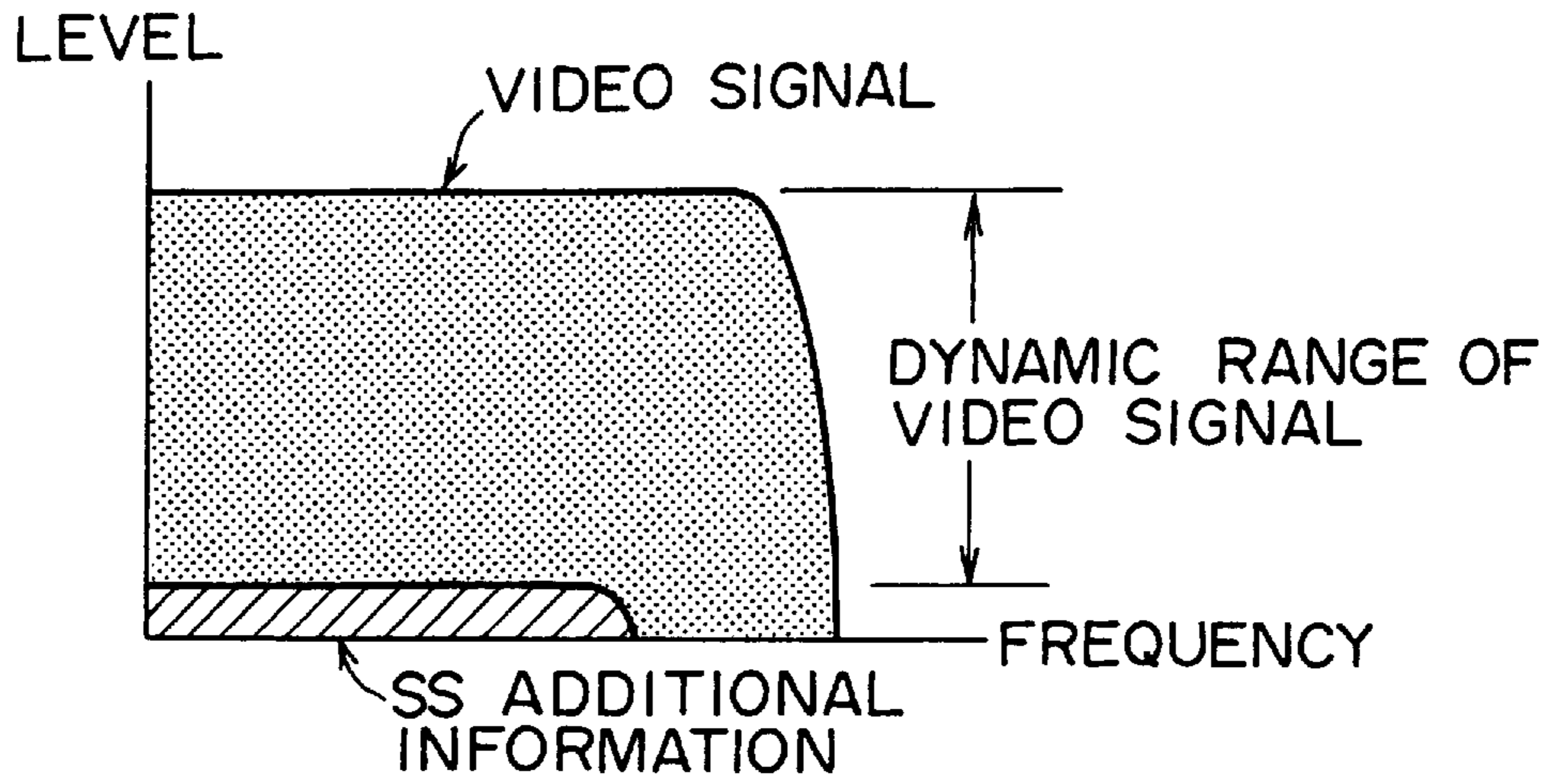
SPECTRUM OF VIDEO SIGNAL HAVING SS ADDITIONAL INFORMATION SUPERIMPOSED THEREON
