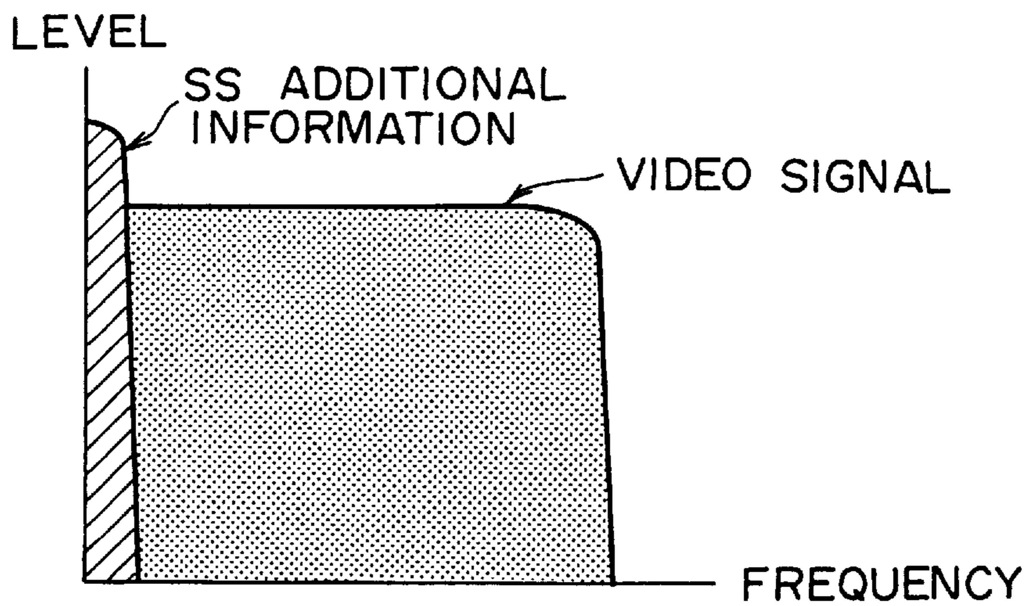
SIGNAL SPECTRUM AFTER INVERSE SPREAD
