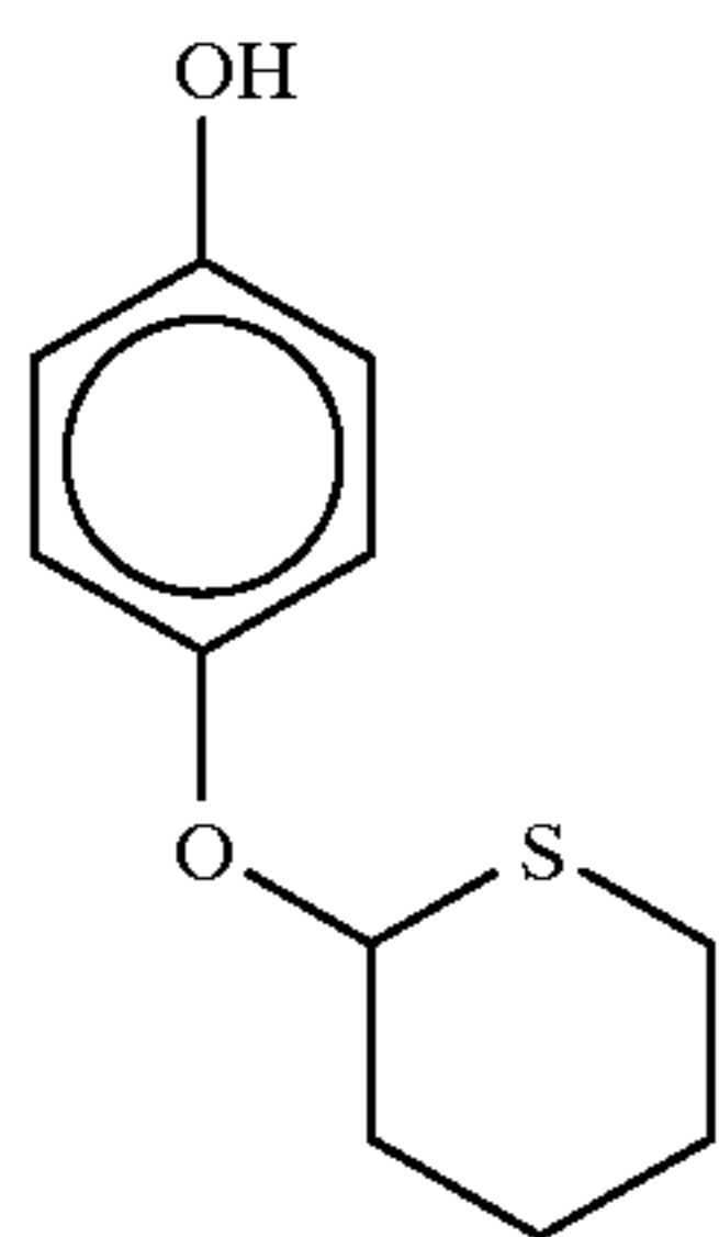
4-[(tetrahydro-2H-thiopyran-2-yl)oxy]phenol
