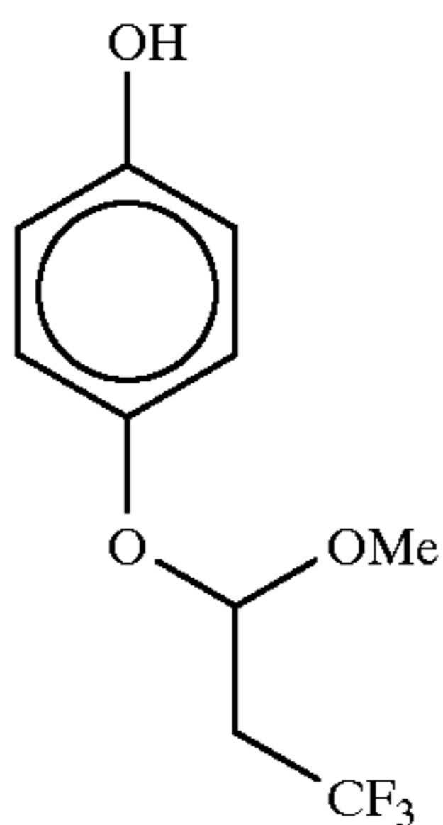
4-[(2-trifluoromethyl-1- methoxyethyl)oxy]phenol
