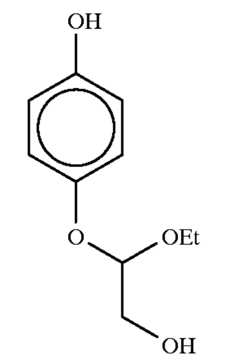
4-[(2-hydroxy-1-ethoxyethyl)oxy]phenol
