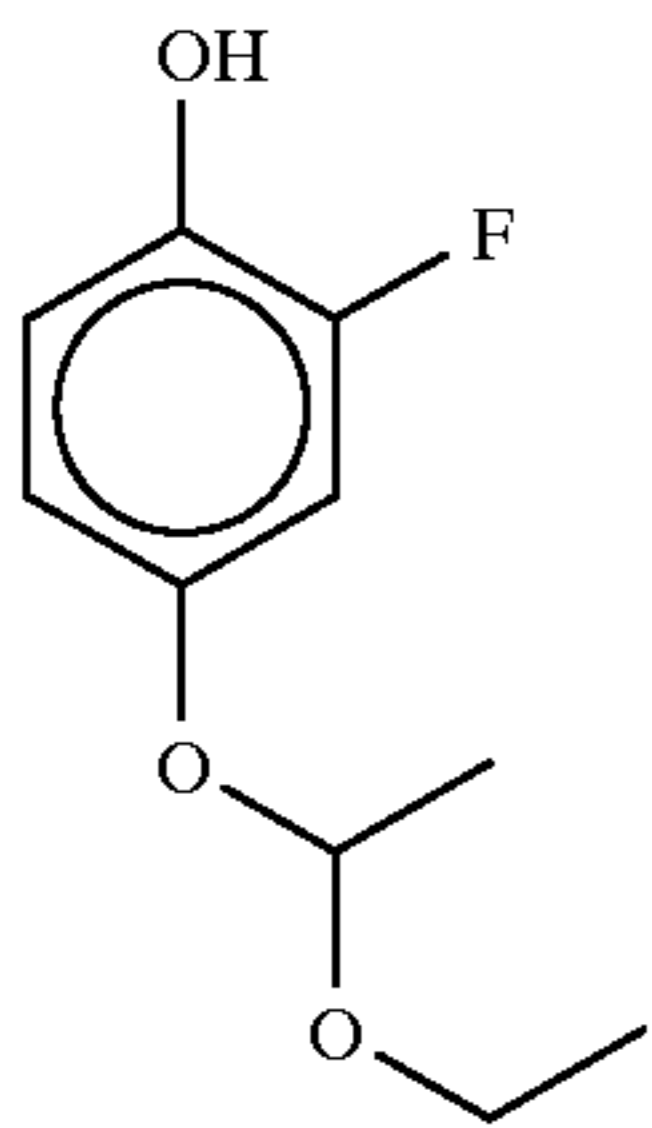
4-[(1-ethoxyethyl)oxy] 2-fluorophenol
