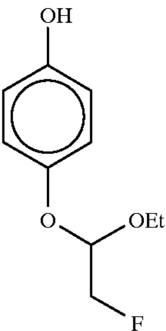
4-[(2-fluoro-1- ethoxyethyl)oxy]phenol
