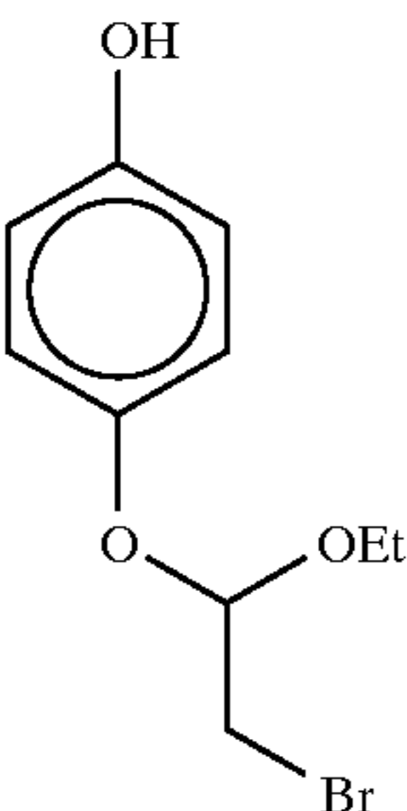
4-[(2-bromo-1- ethoxyethyl)oxy]phenol
