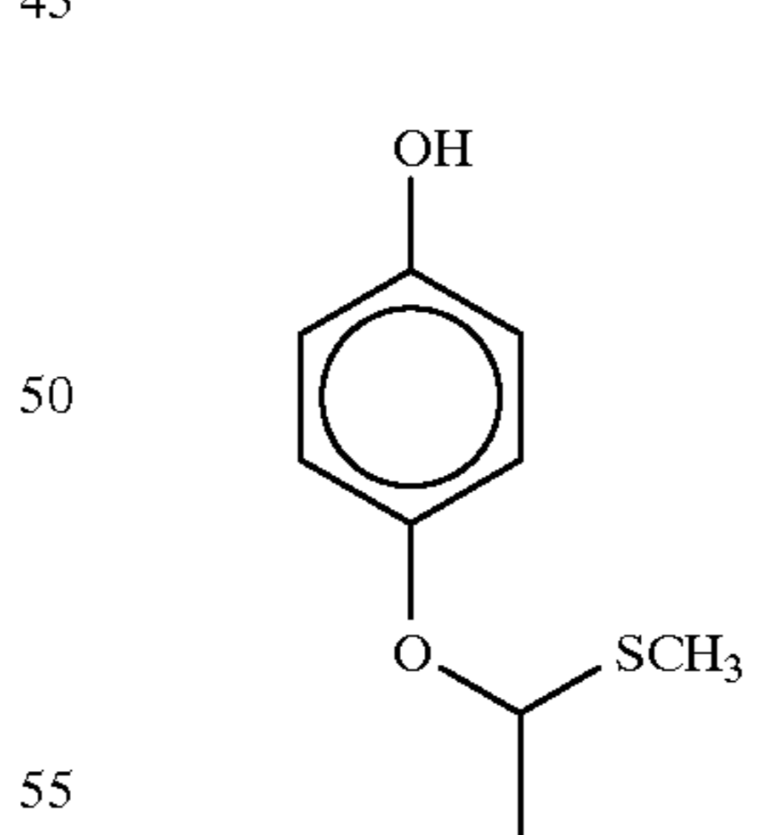
4-(1-methylthioethoxy)phenol
