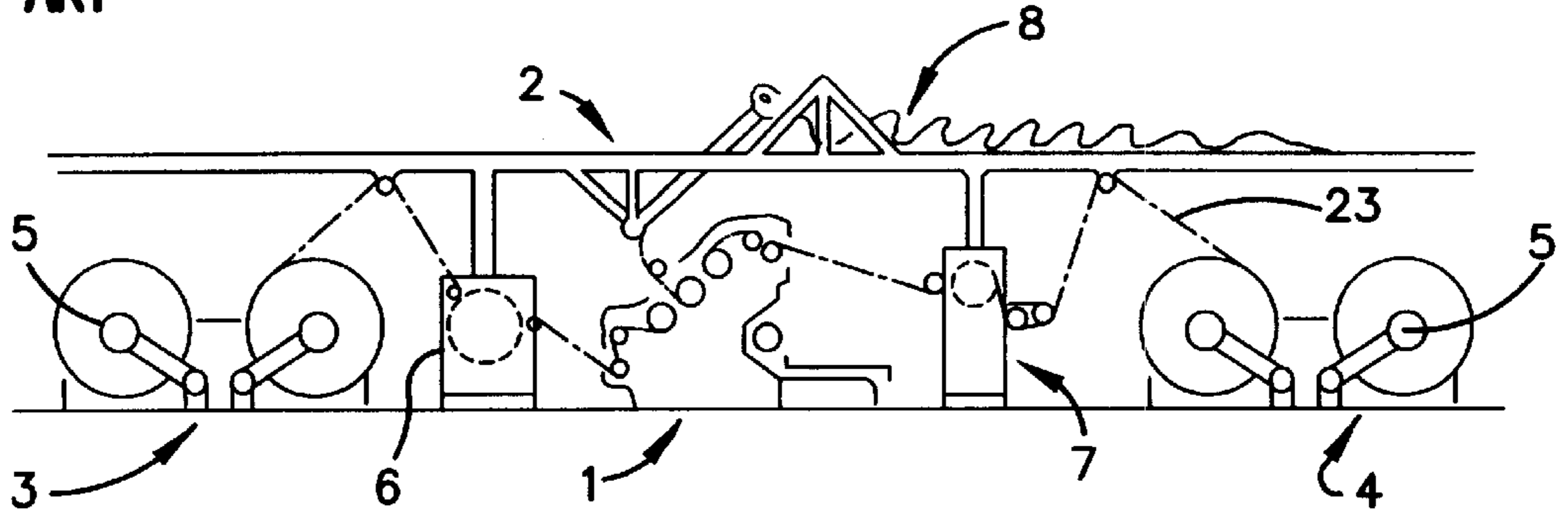
FIG. 1 PRIOR ART
