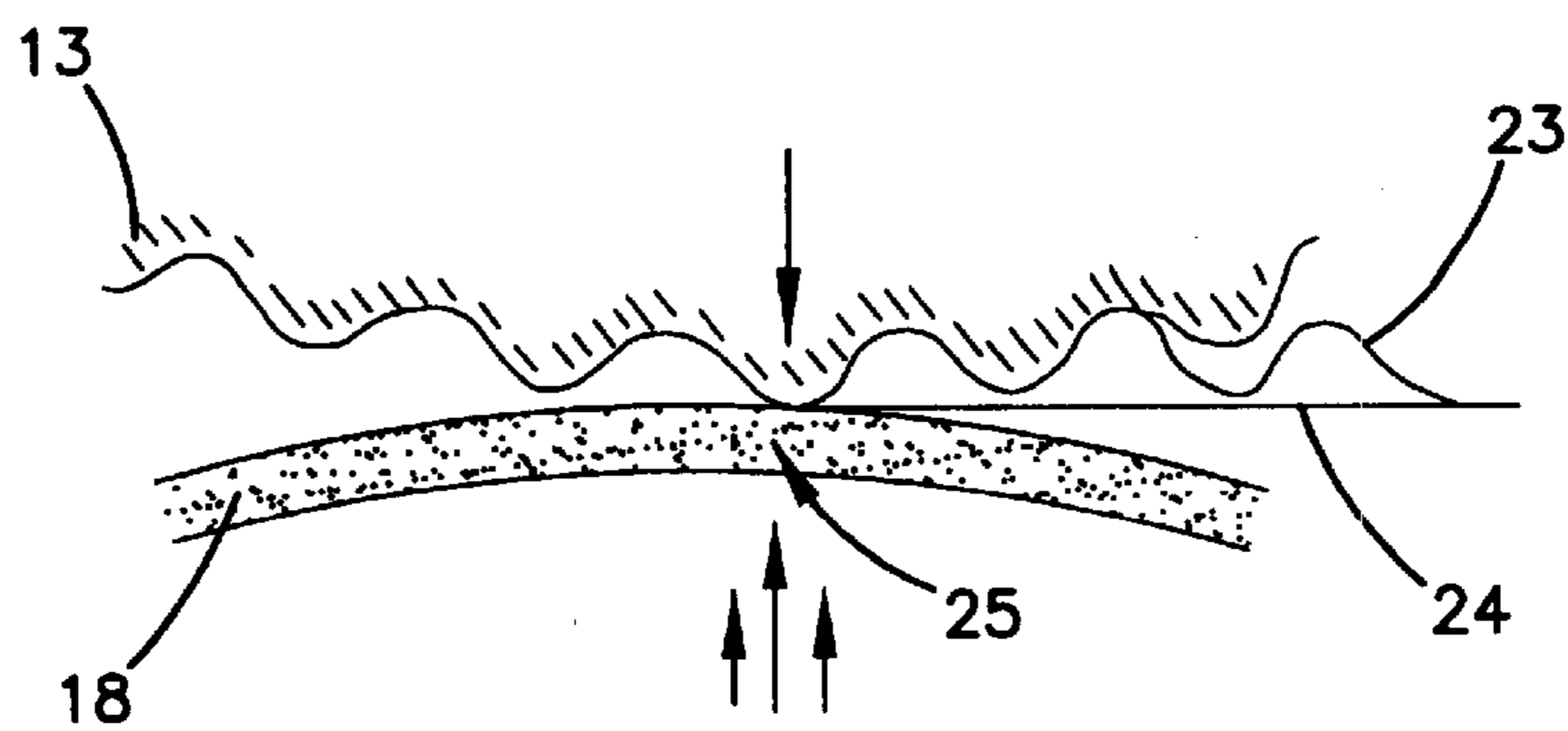
FIG. 3 PRIOR ART
