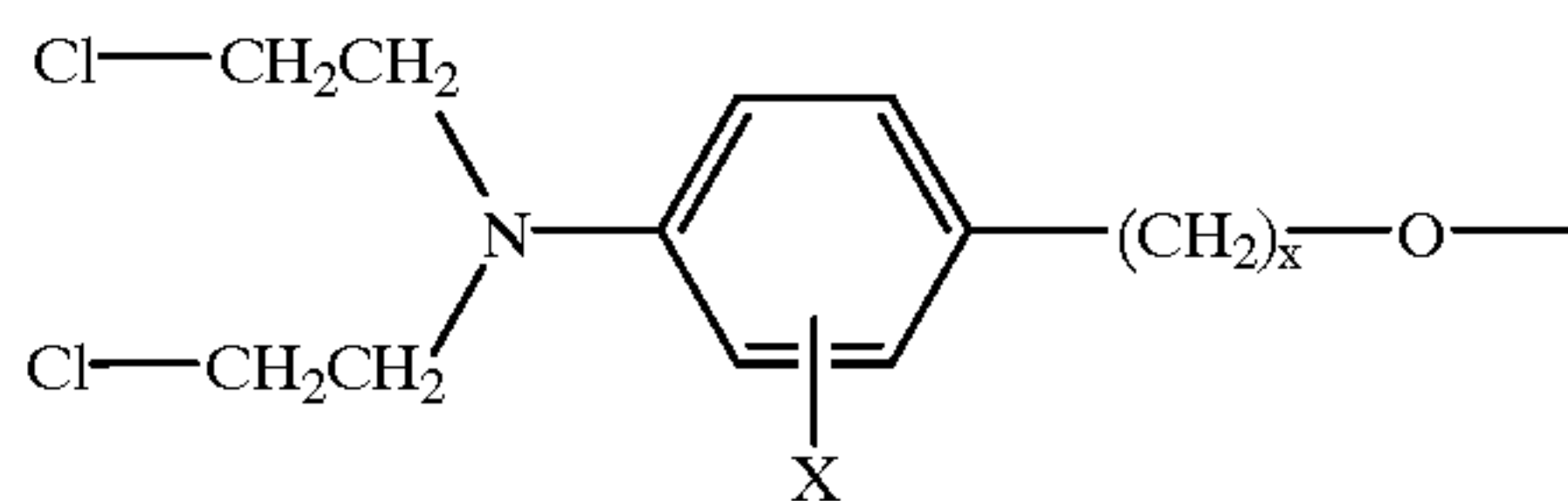
x = 1-18 , X = \text{alkyl, halogen, NO}_2, \text{CN or } -C(=O)R
