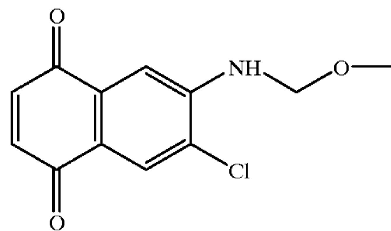
Naphthoquinone conjugate
