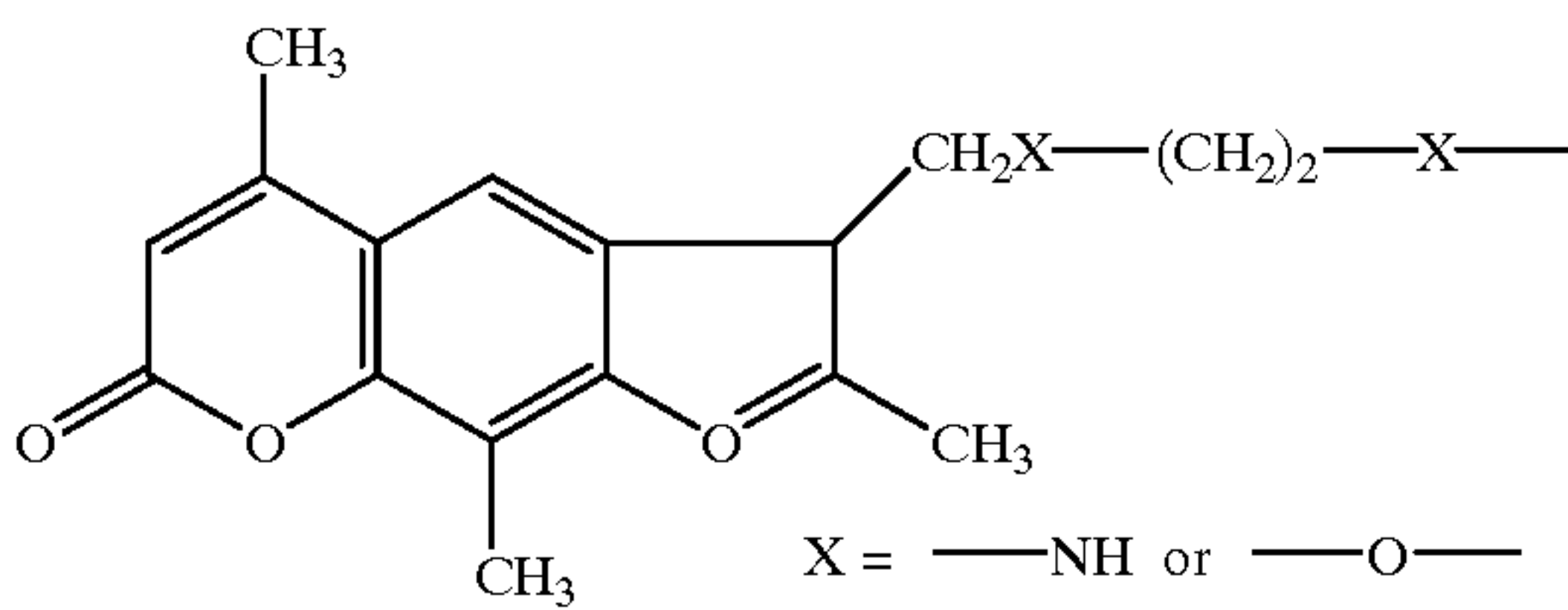
Trimethylpsoralene conjugate (= "psoralene" for X = O )
