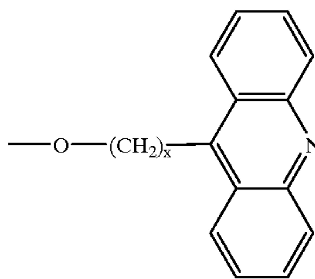
Acridine derivative x = 2-12 , preferably 4
