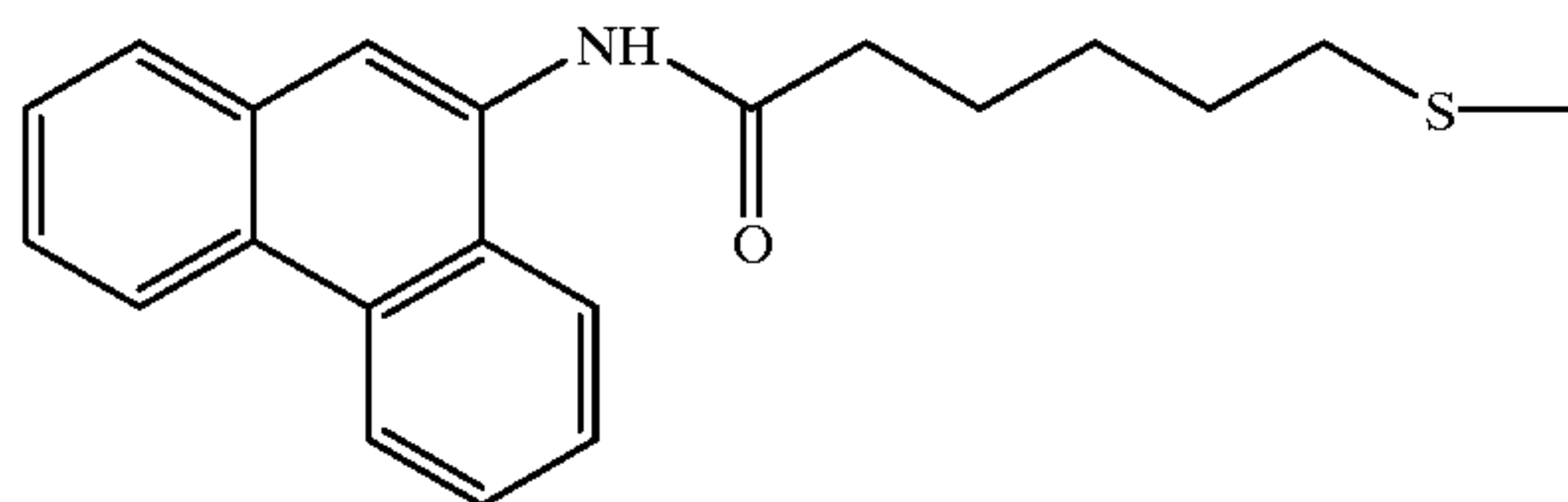
Phenanthroline conjugate
