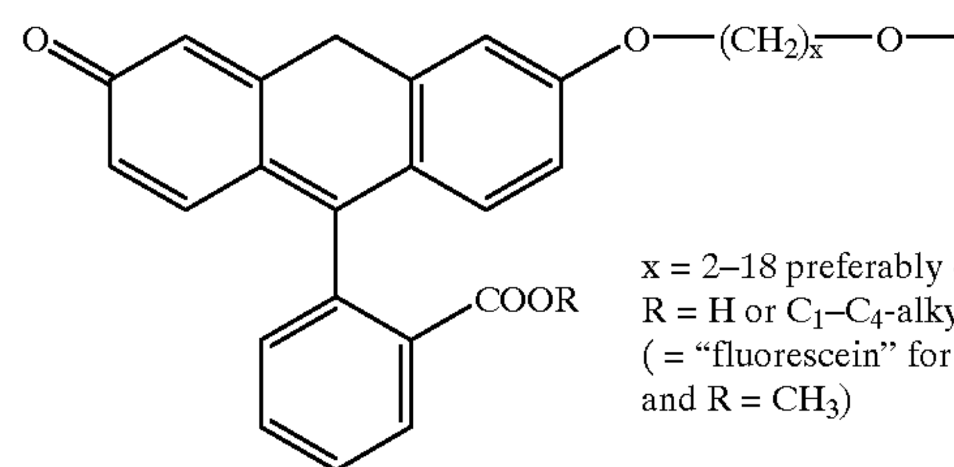
Fluorescein derivative
