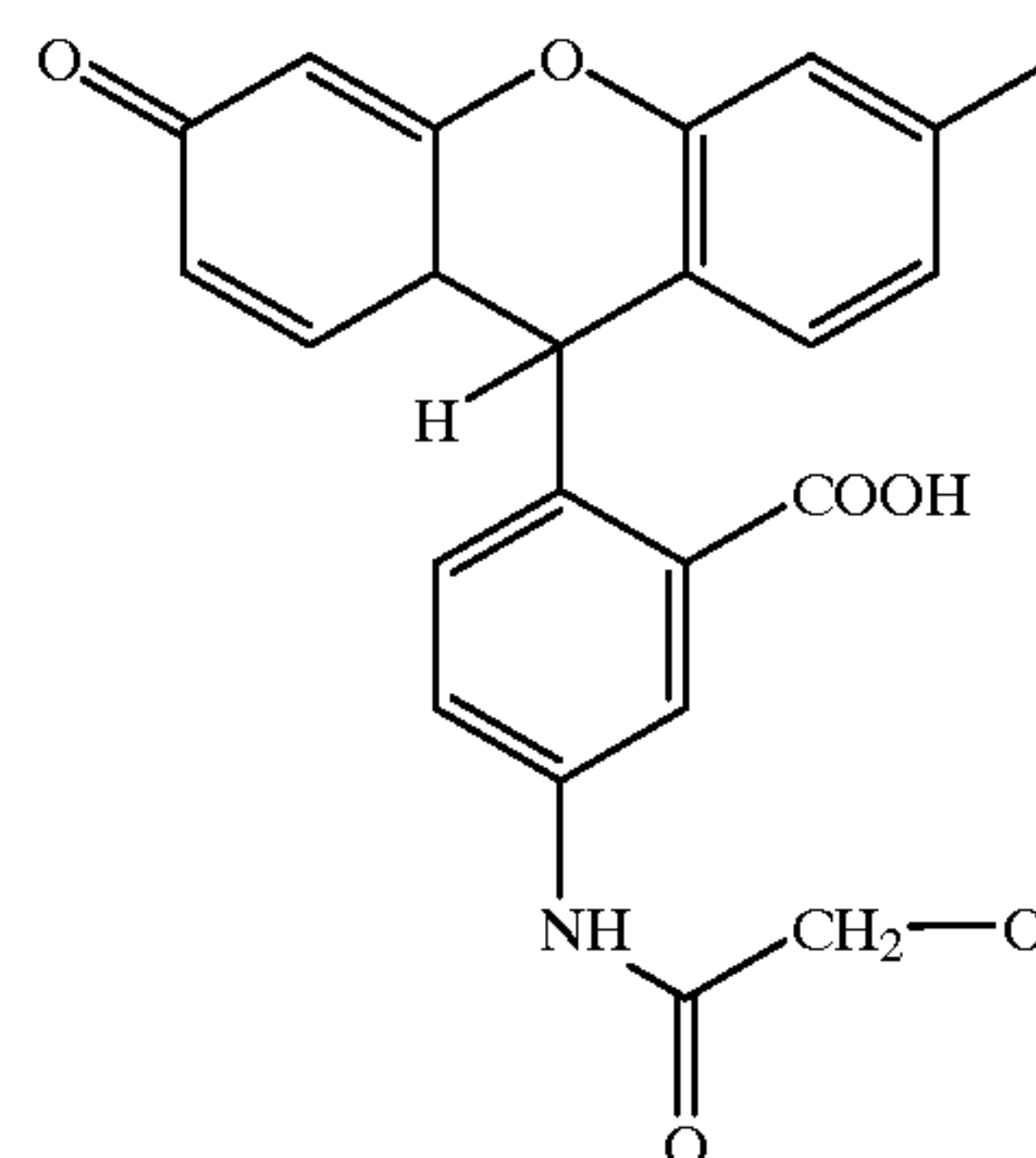
Fluorescein derivative
