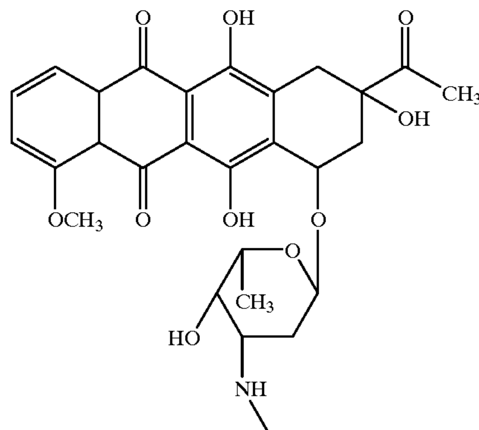
Daunomycin derivative
