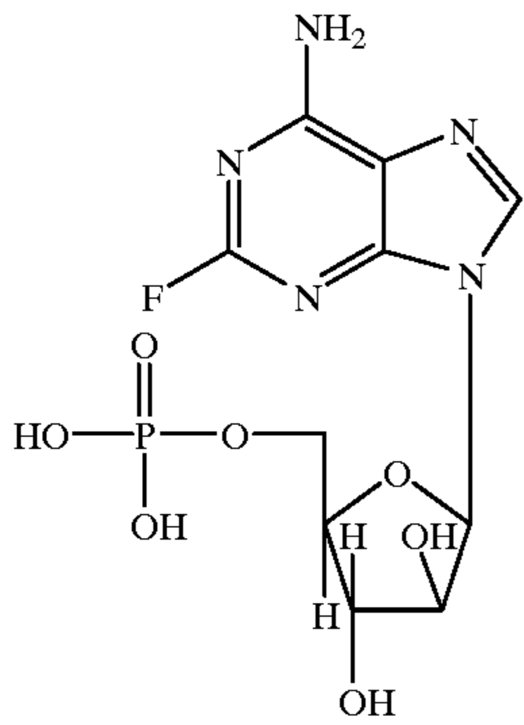
Fludarabine Phosphate
