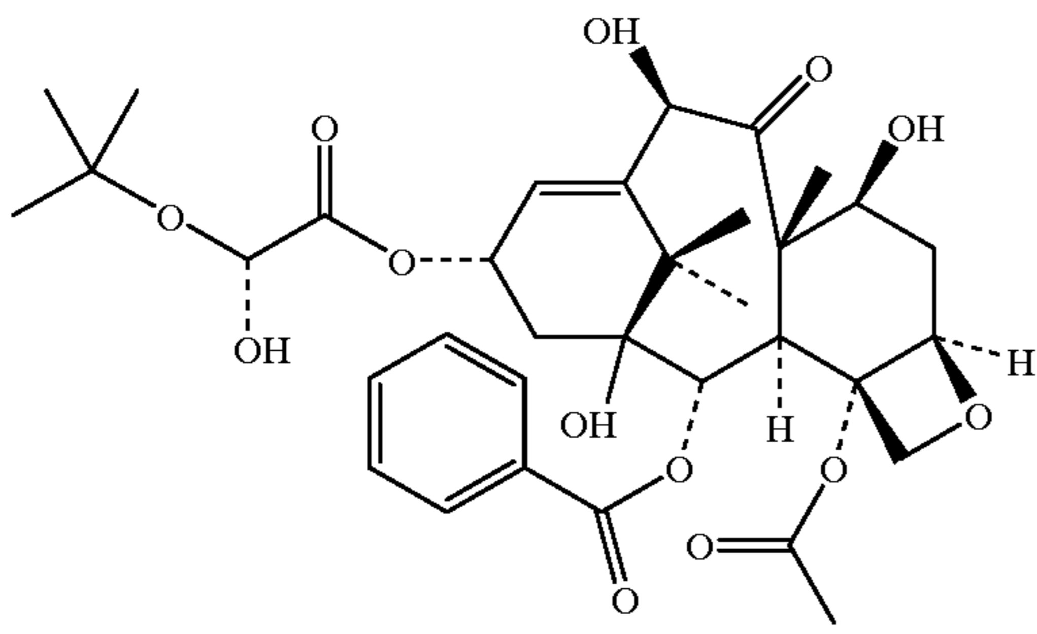
Taxotere
