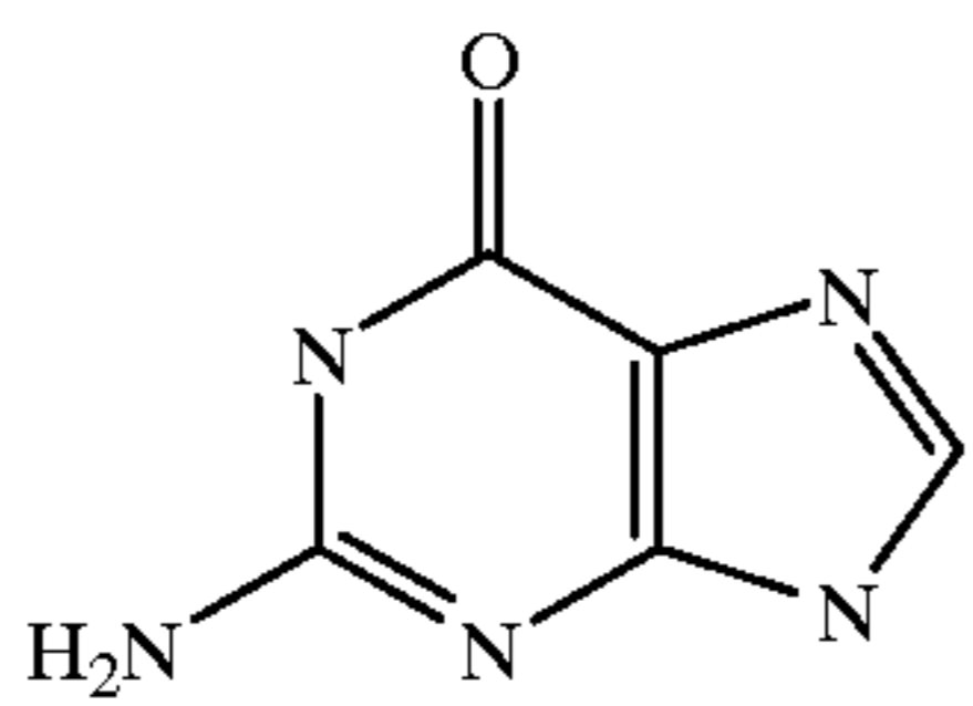
Guanine
