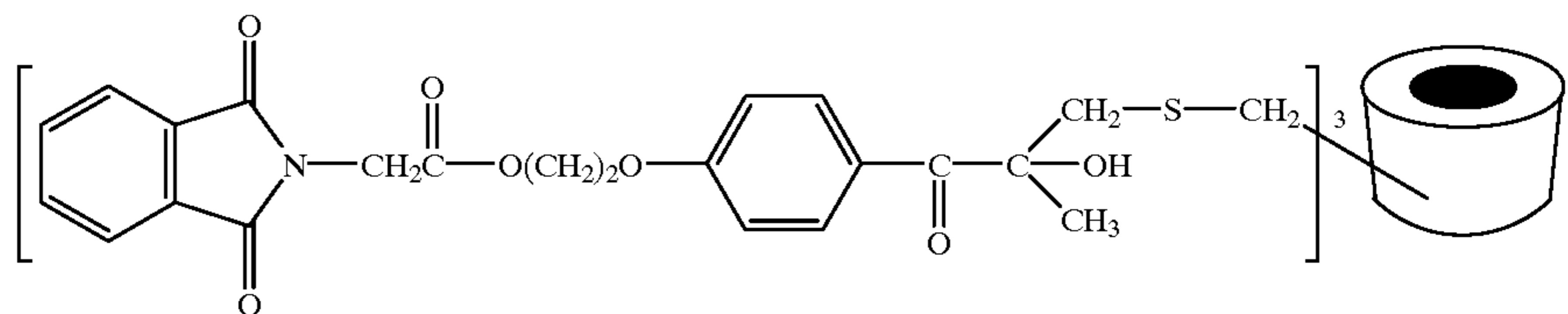
Hydroxy Compound
