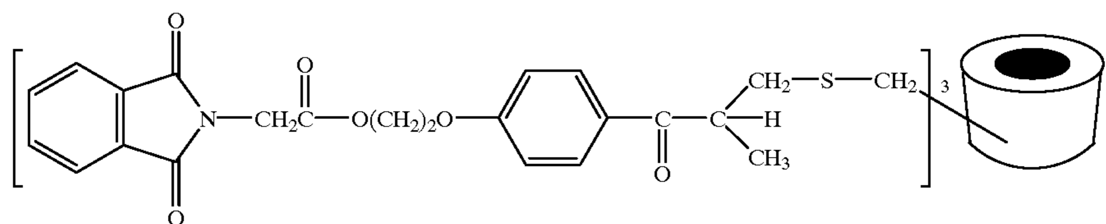
Dehydroxy Compound
