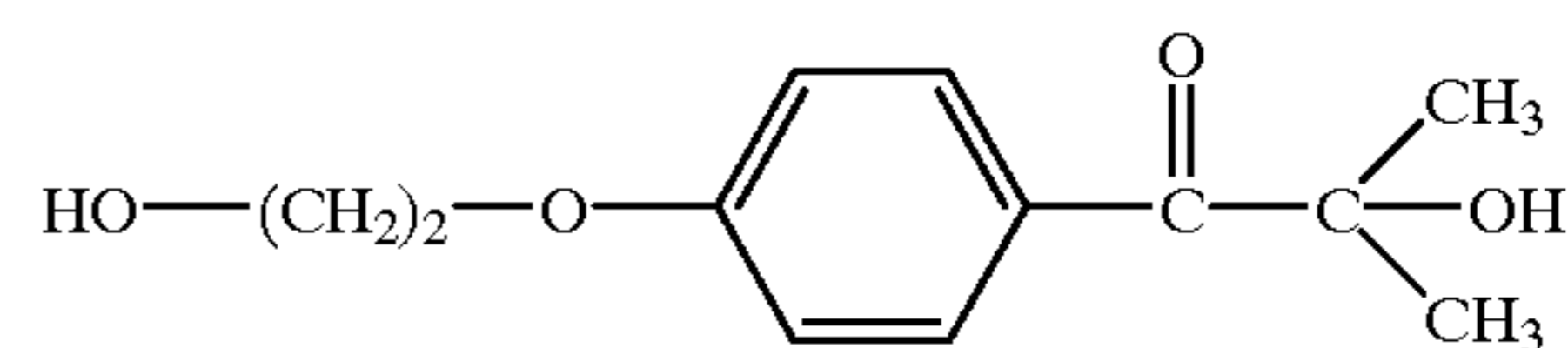
Unmodified DARCUR 2959®
