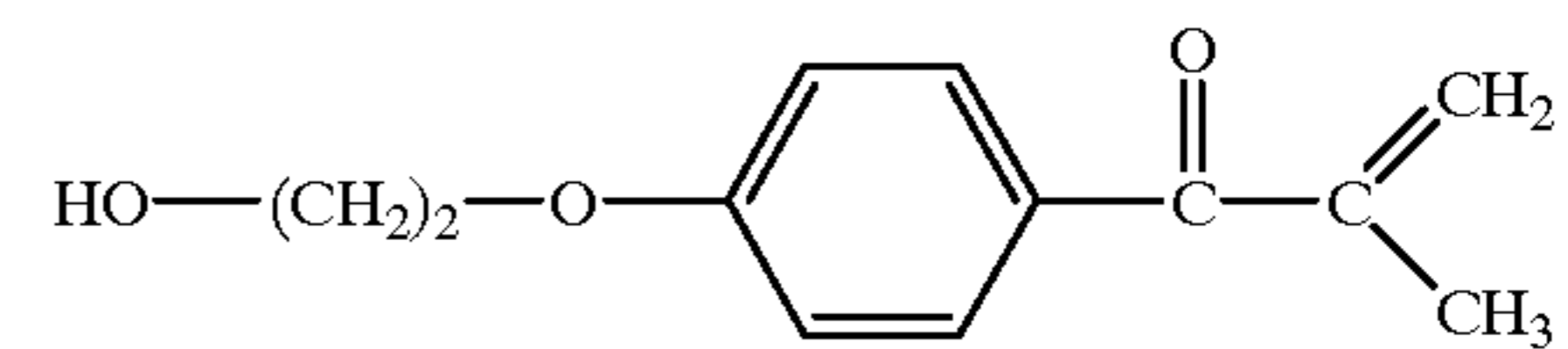
Dehydrated DARCUR 2959®
