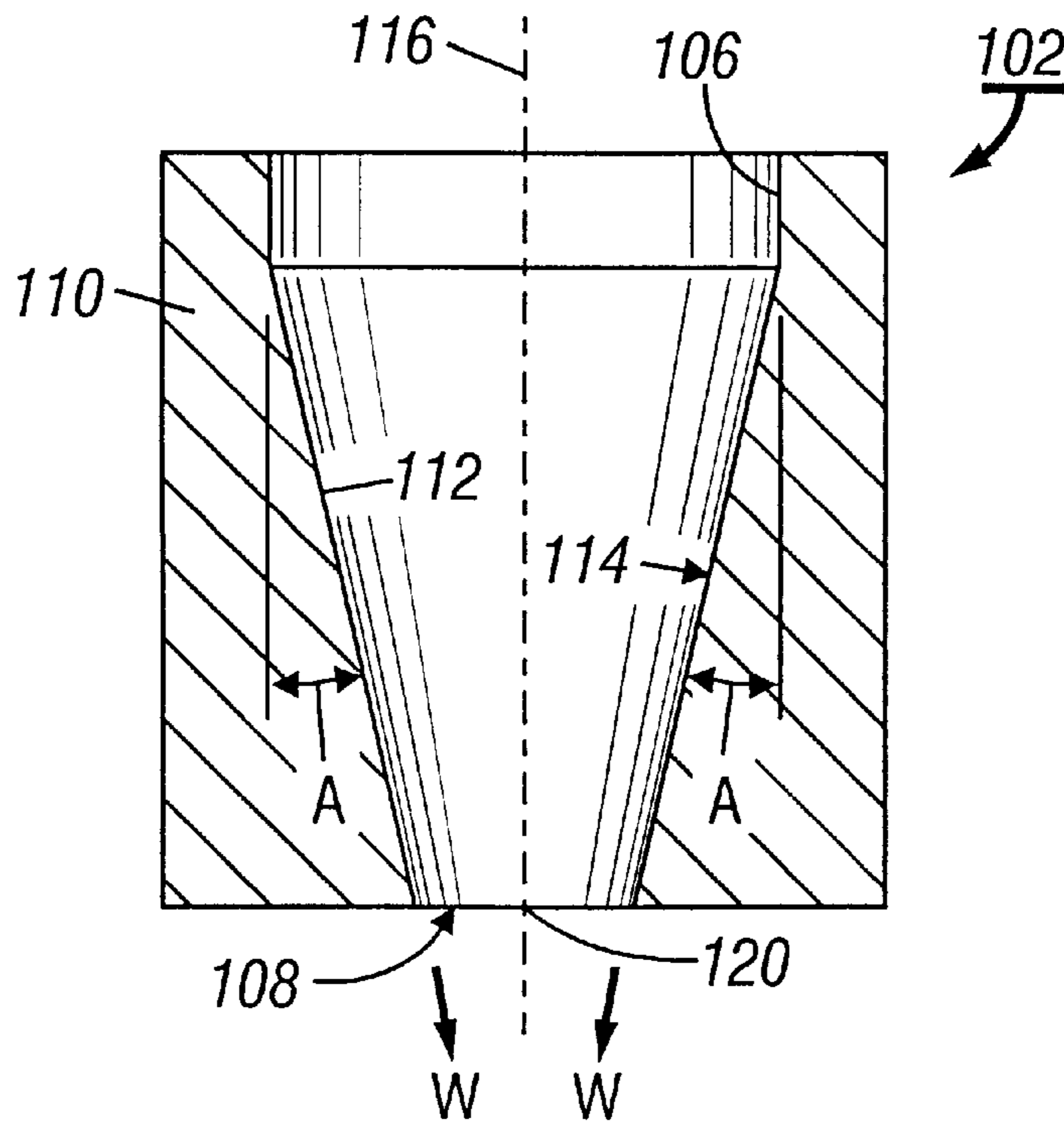
FIG. 1 (Prior Art)
