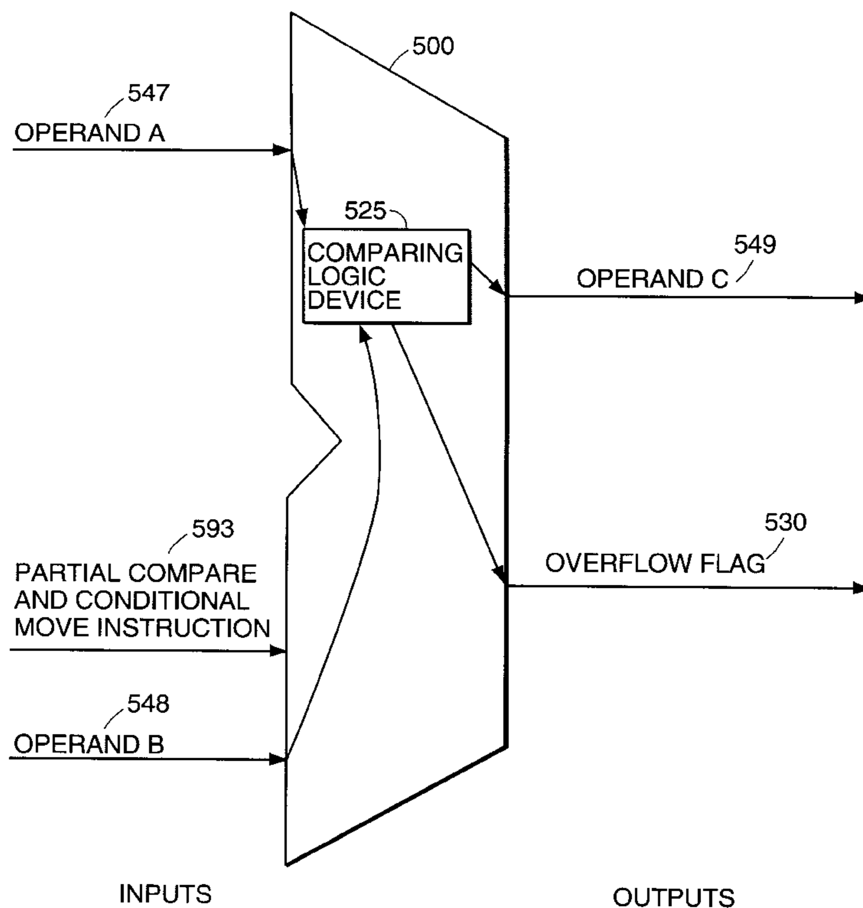
PARTIAL COMPARE AND CONDITIONAL MOVE
