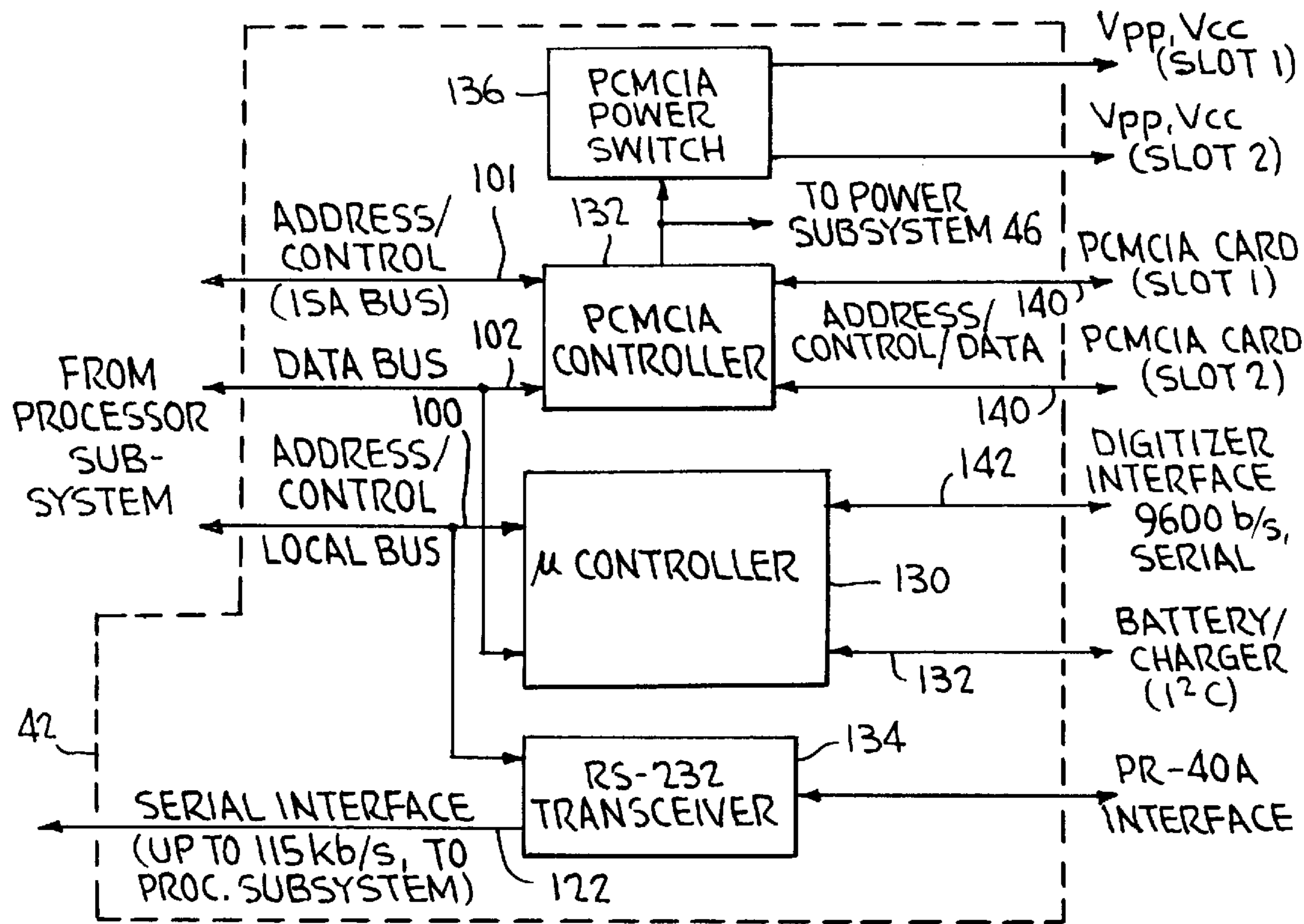
FIG. 4 COMMUNICATION SUBSYSTEM
