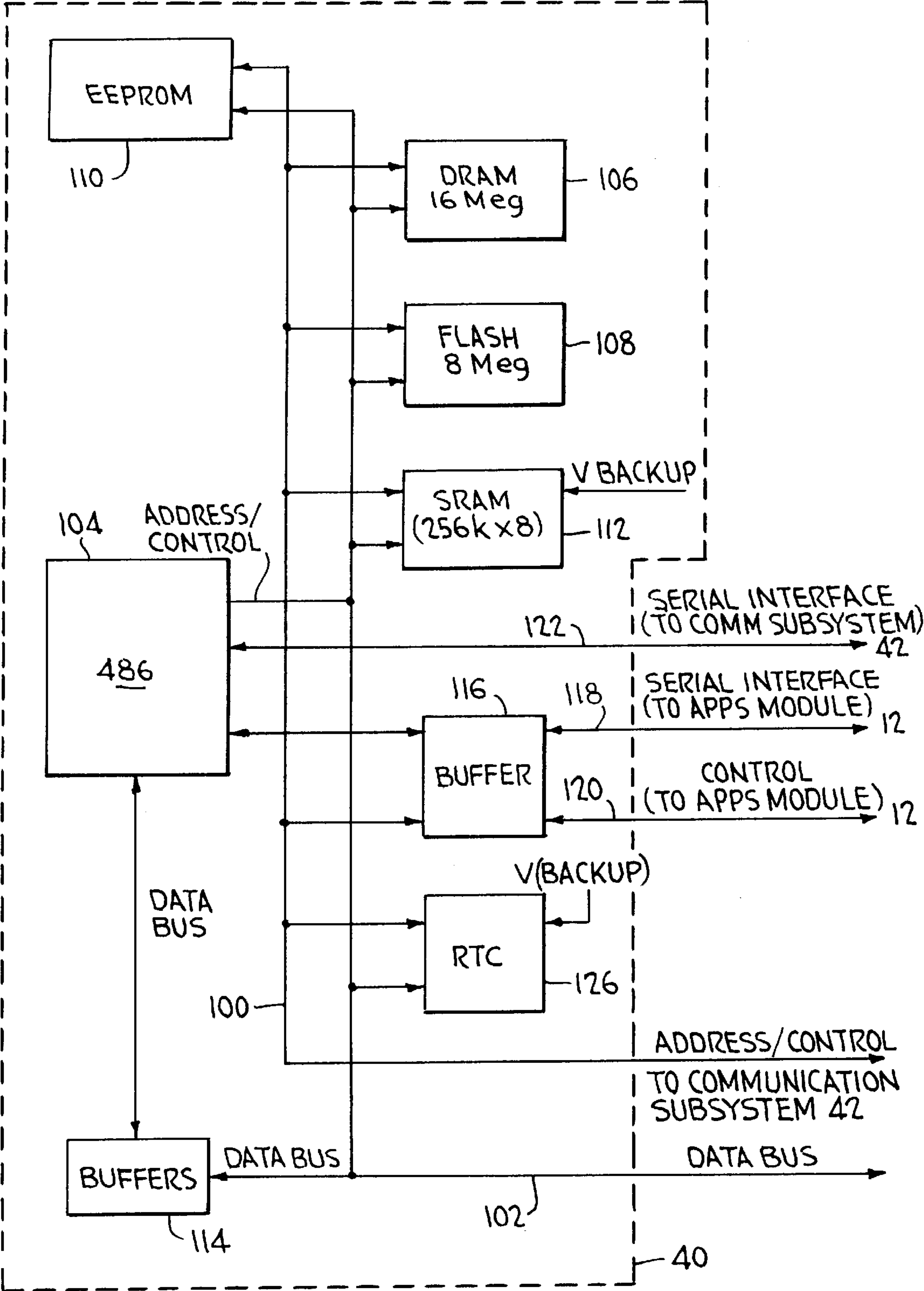
FIG. 3 PROCESSOR SUBSYSTEM
