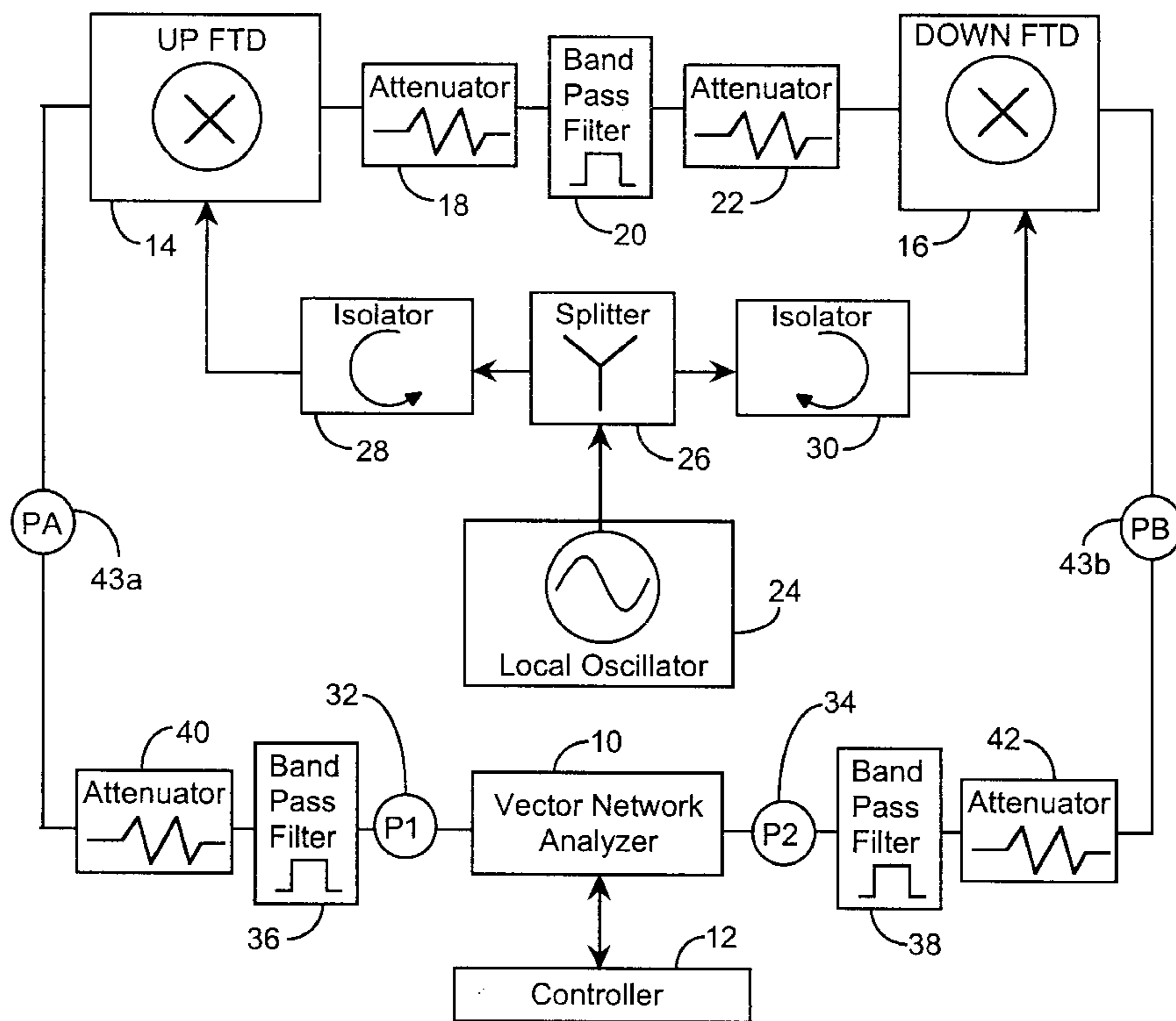
SSB FTD Test Diagram
