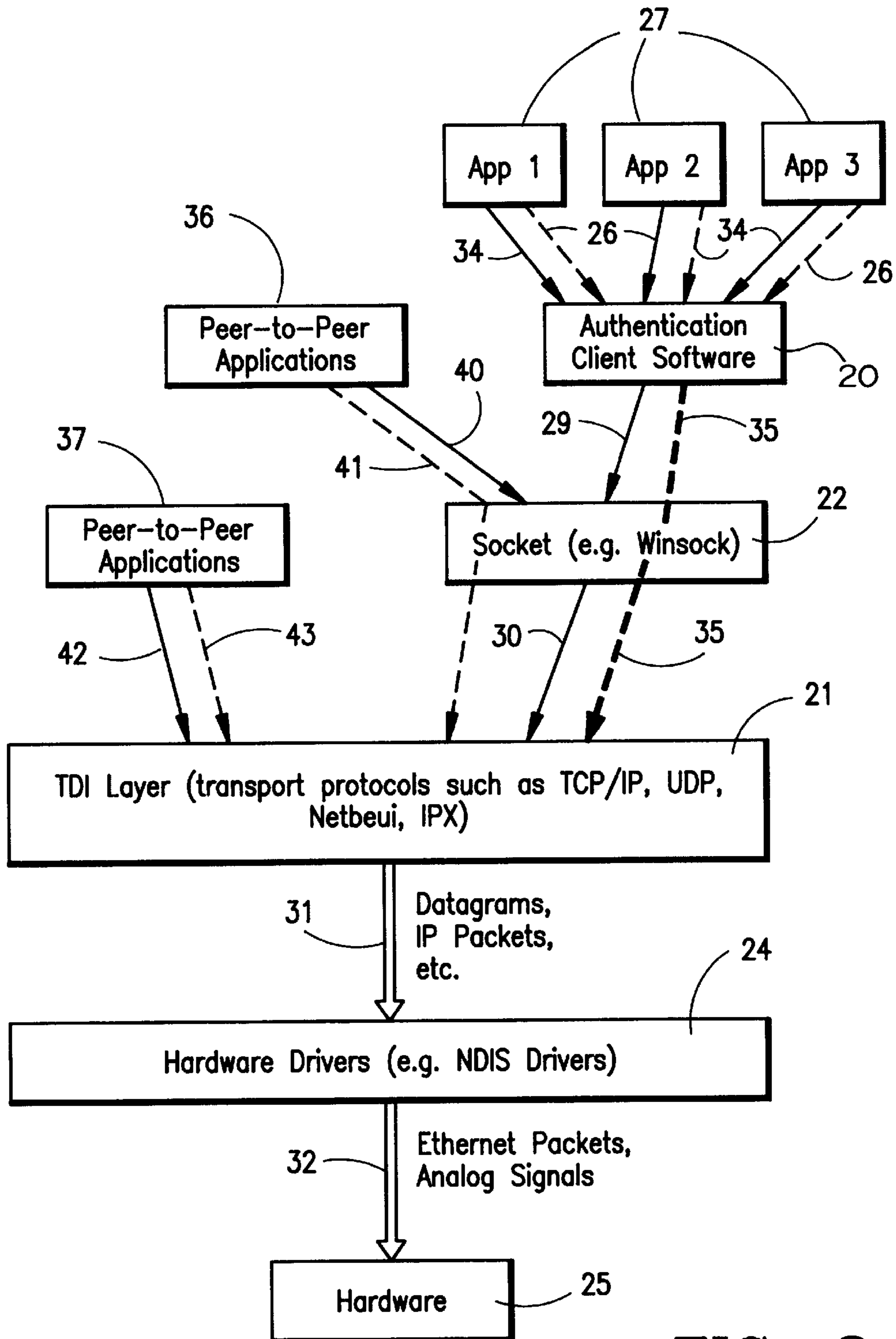
FIG. 2 (PRIOR ART)
