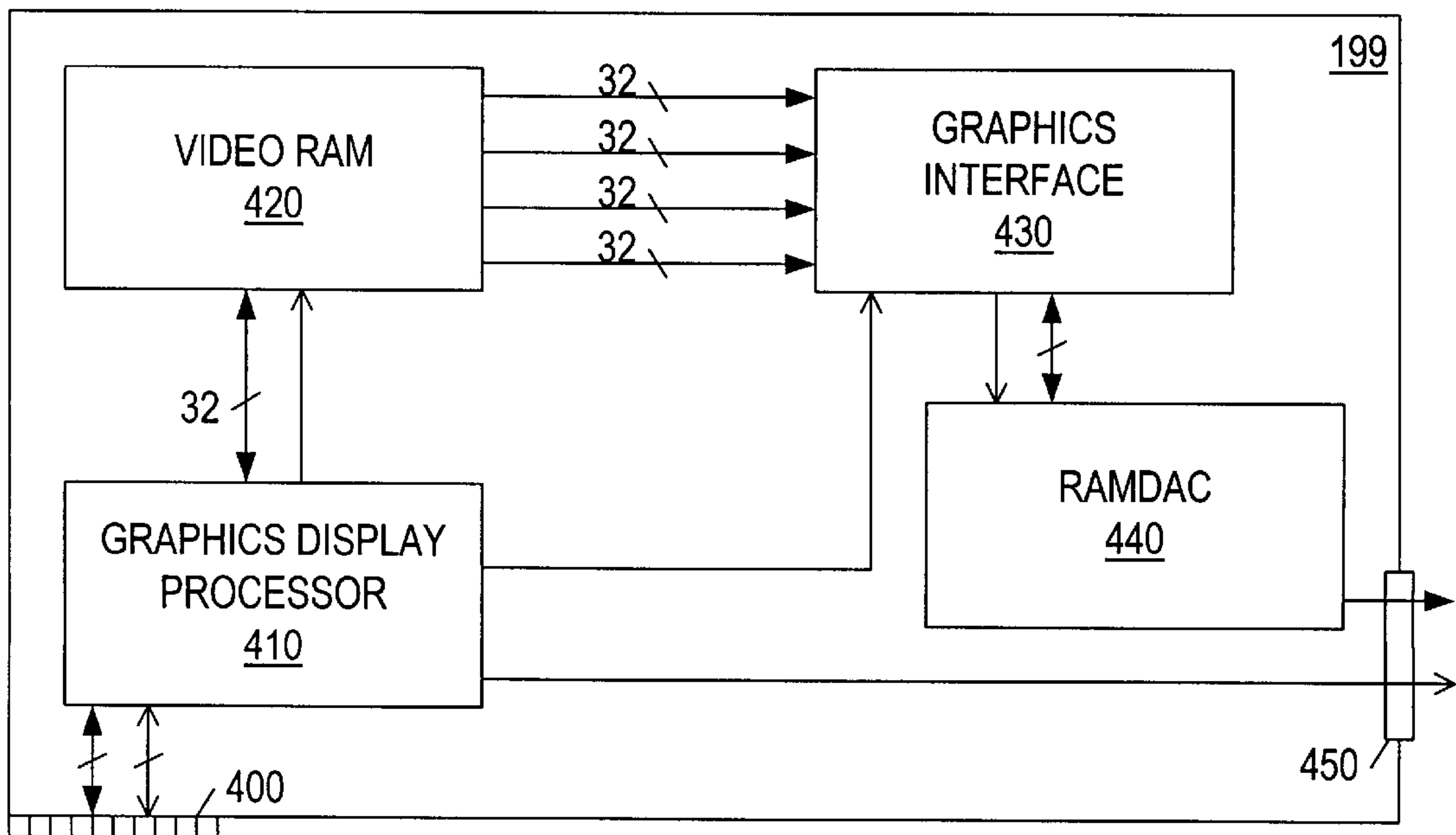
FIG. 4 (PRIOR ART)
