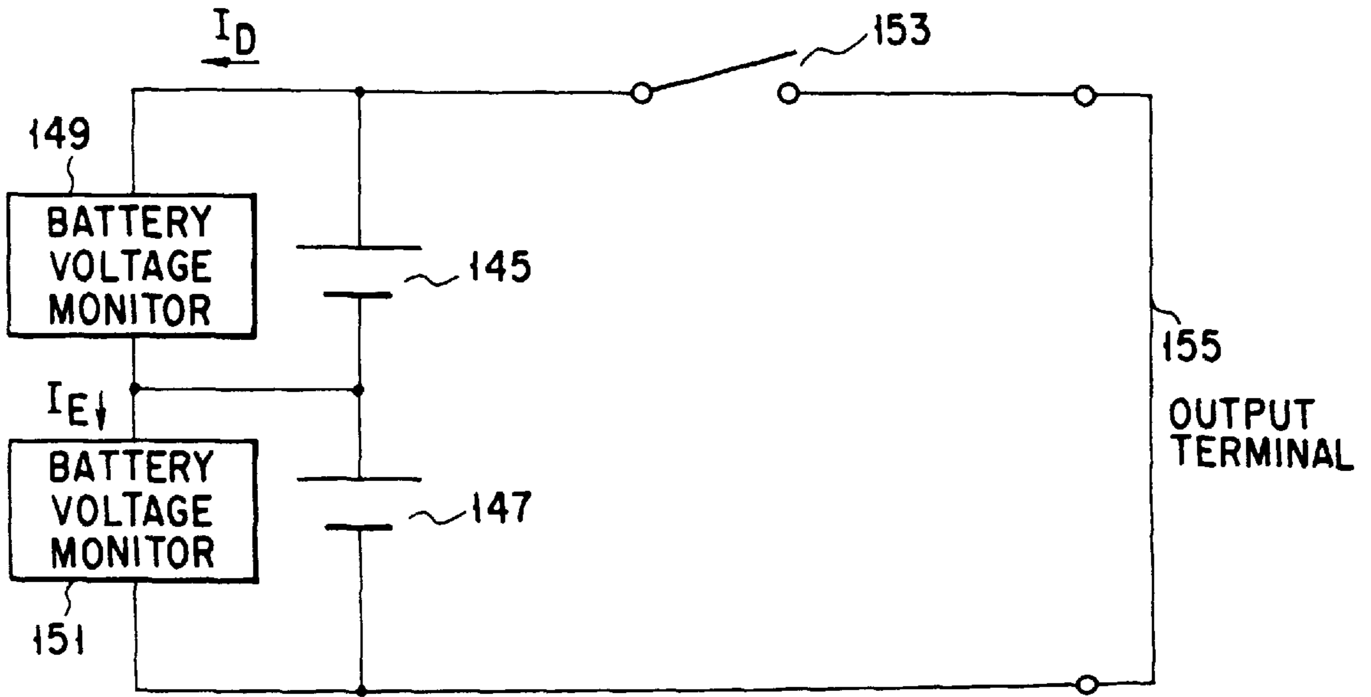
FIG. 13 (PRIOR ART)
