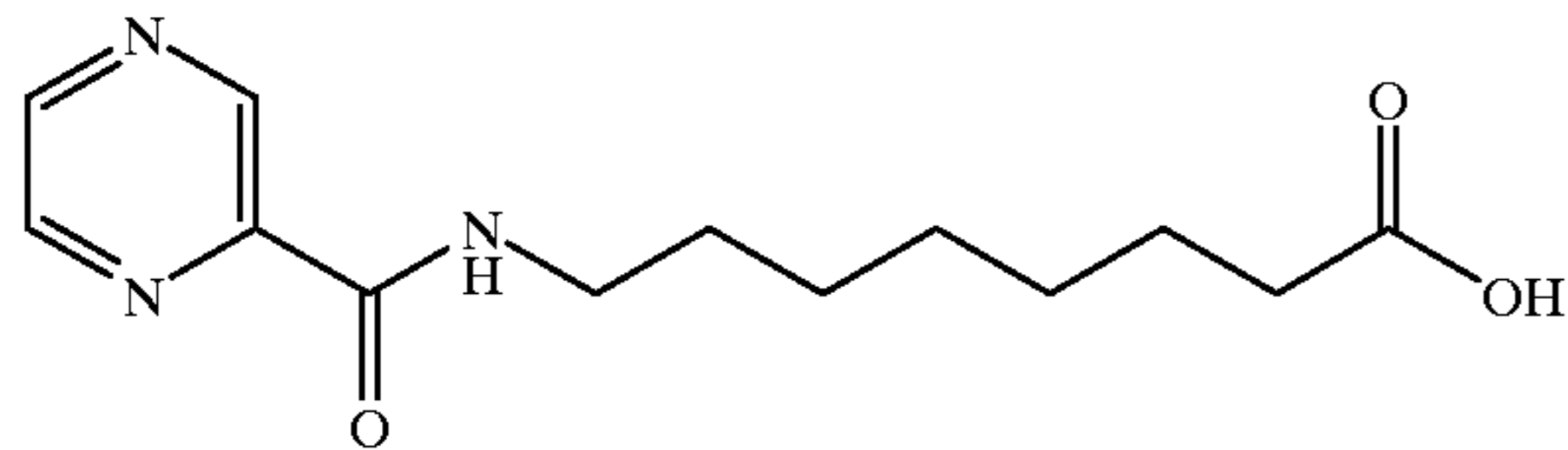
8-(2-pyrazinecarbonyl)aminocaprylic acid
