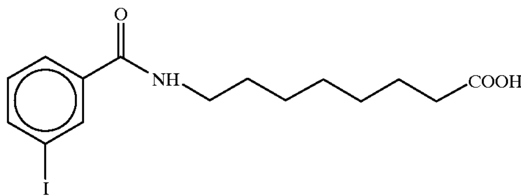
8-N-(3-iodobenzoyl)aminocaprylic acid
