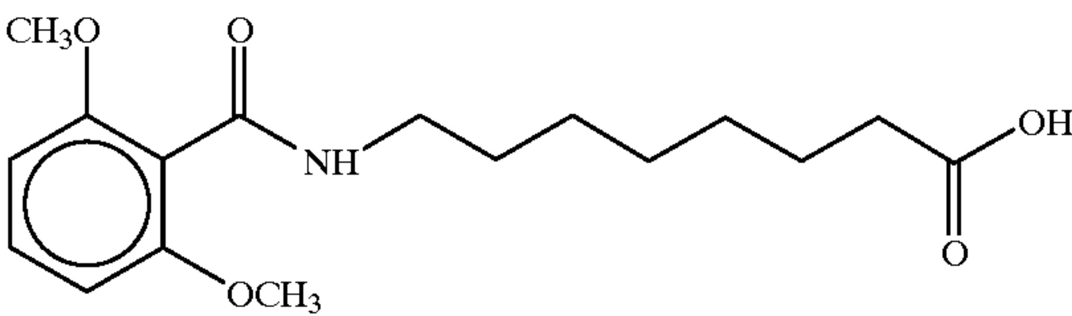
8-(N-2-6-Dimethoxybenzoyl)aminocaprylic acid
