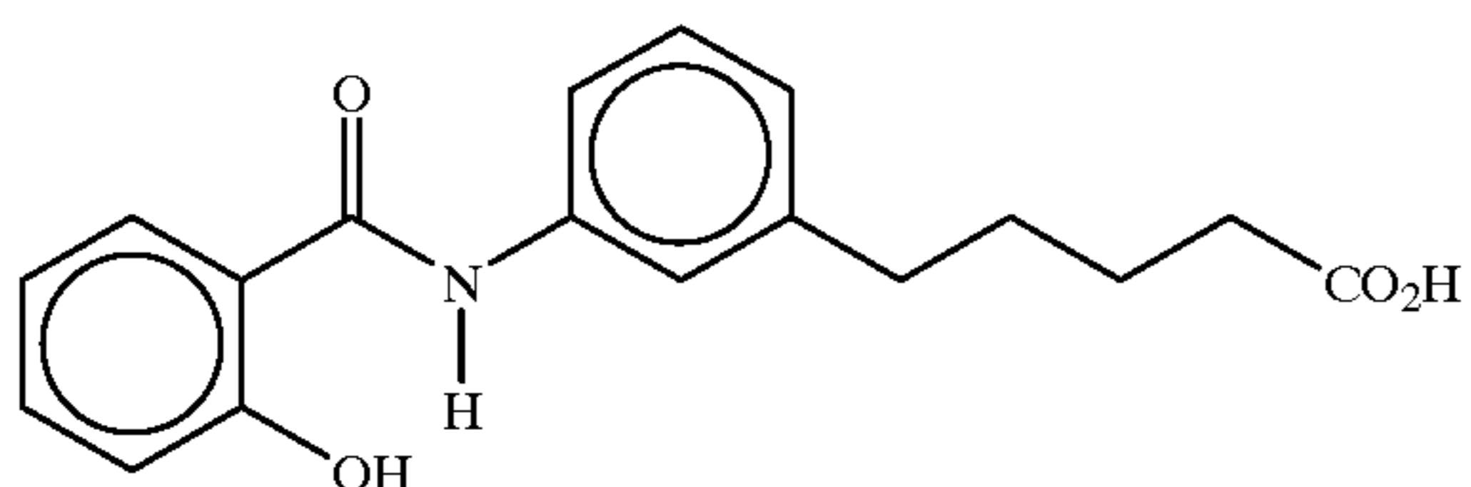
N-salicyloyl-5-(3-aminophenyl)valeric acid
