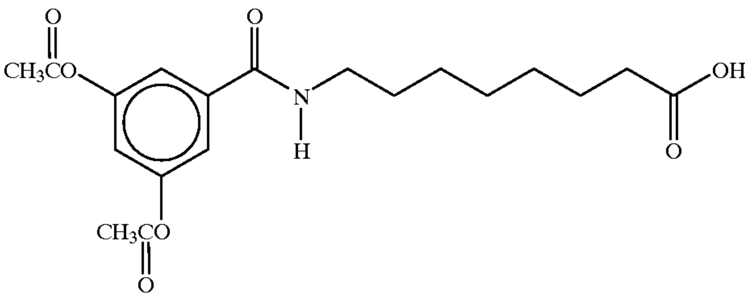
8-(N-3, 5-Diacetyloxybenzoyl)aminocaprylic acid
