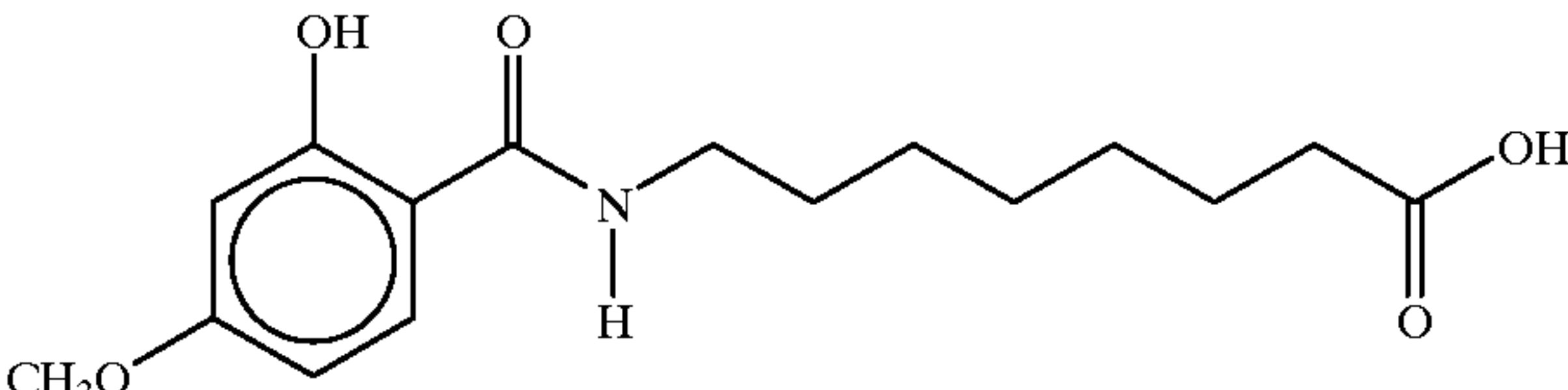
8-(N-2-Hydroxy-4-methoxybenzoyl)aminocaprylic acid
