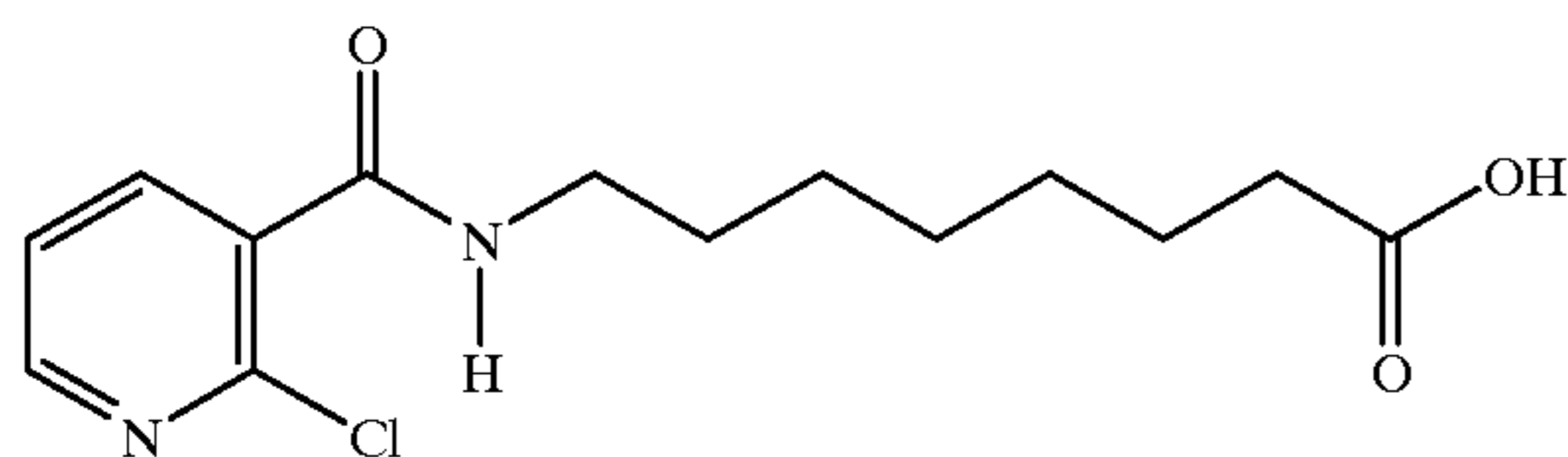
8-(2-chloronicotinoyl)aminocaprylic acid
