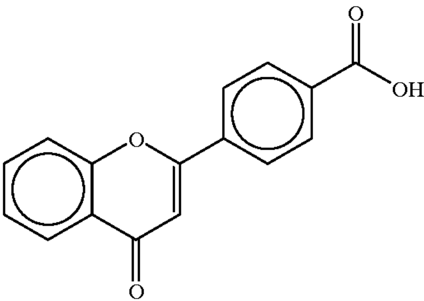
4'-flavonic acid
