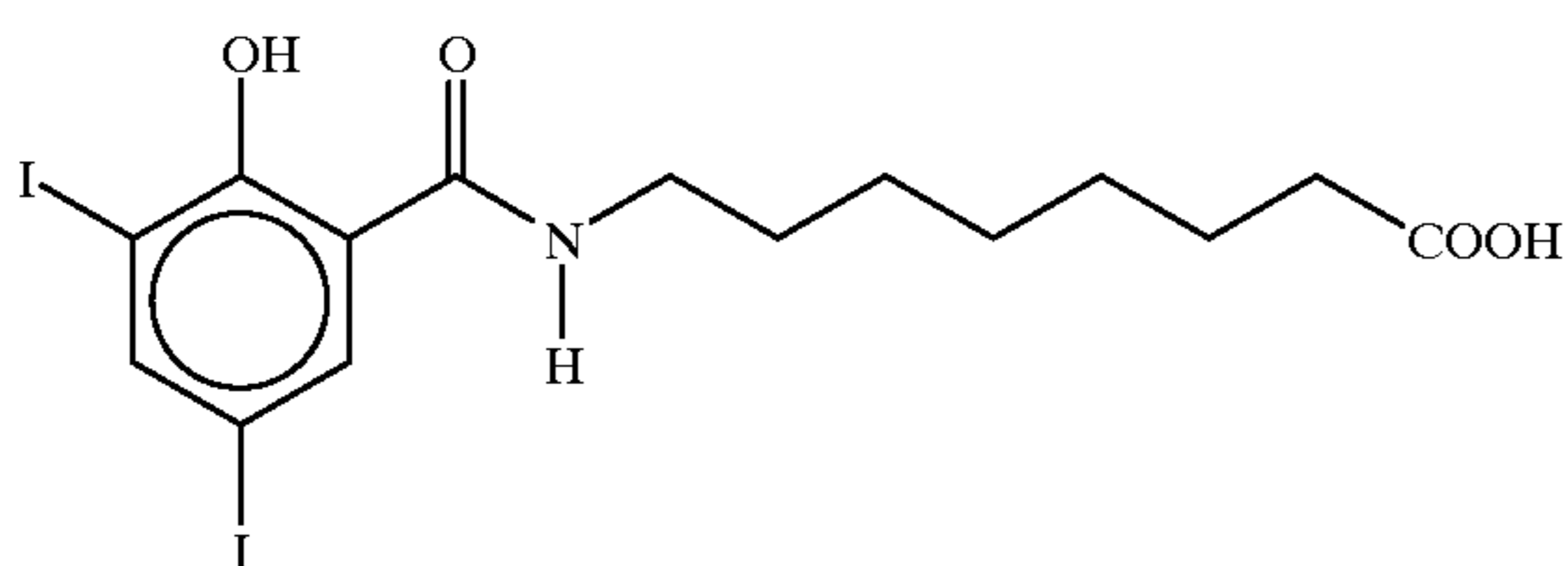
8-(N-2-hydroxy-3,5-diiodobenzoyl)aminocaprylic acid
