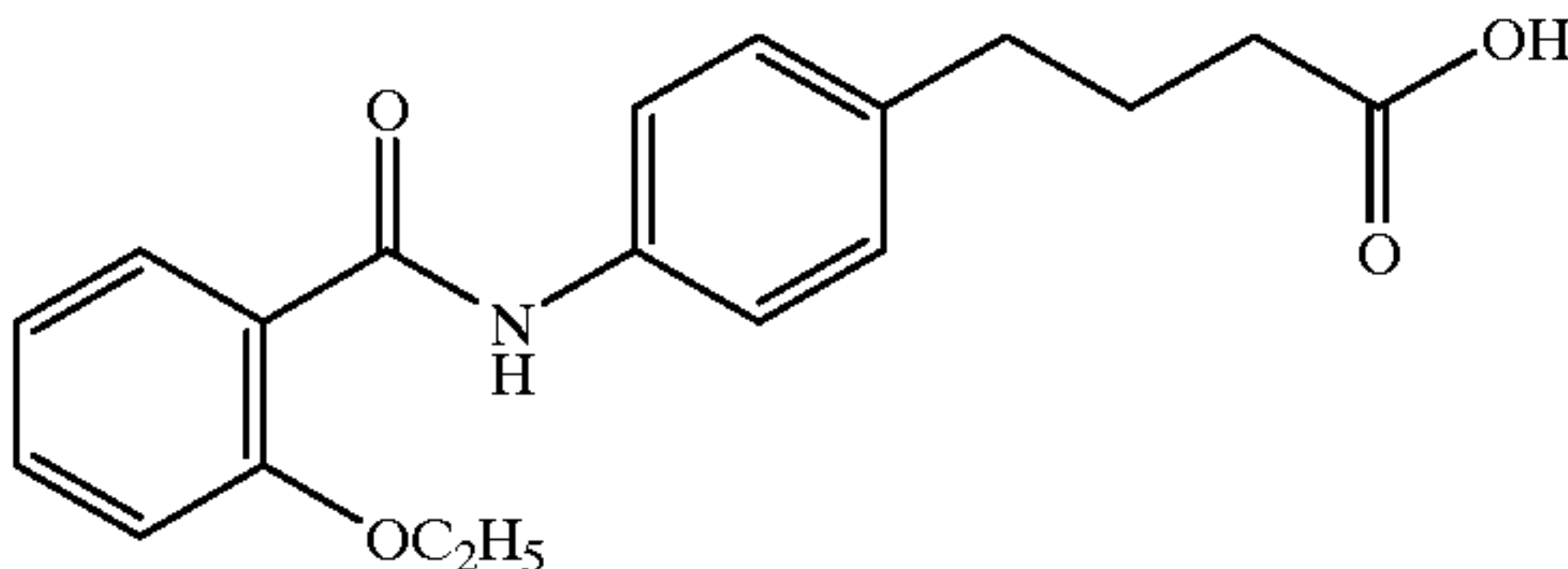
4-(4-(2-ethoxybenzoyl)aminophenyl)butyric acid
