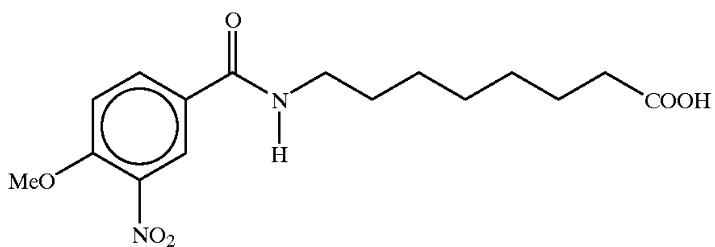
8-N-(4-methoxy-3-nitrobenzoyl)aminocaprylic acid
