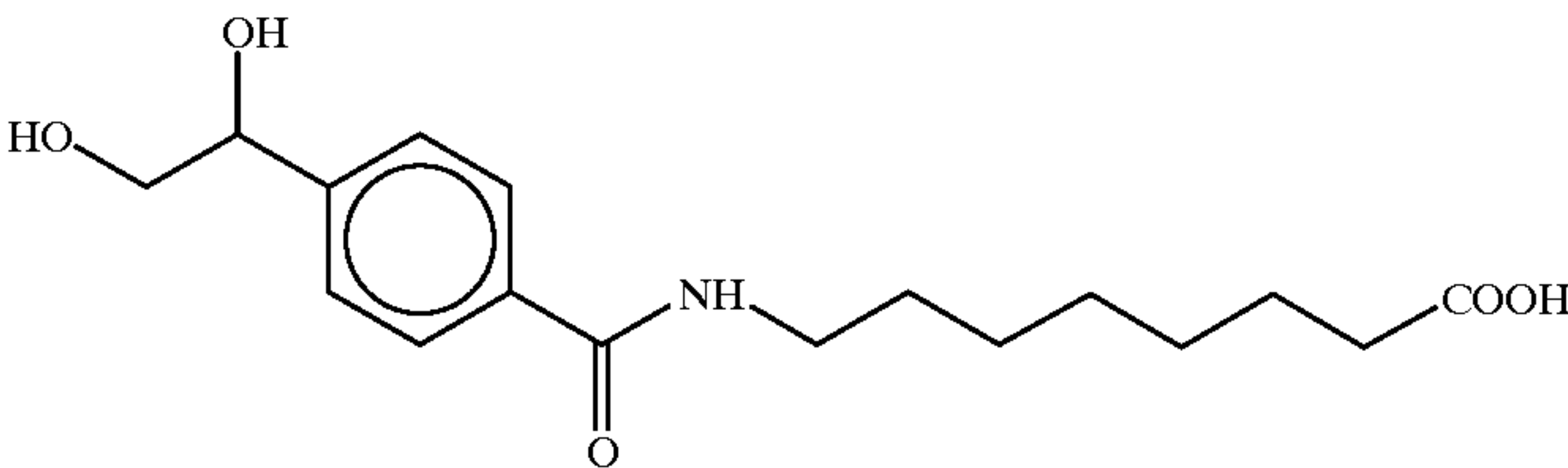
8-(4-(1, 2-dihydroxyethyl)benzoyl)aminocaprylic acid
