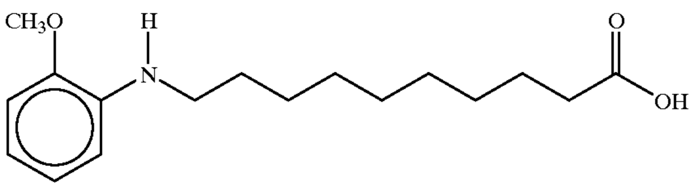
2-Methoxybenzenaminodecanoic acid
