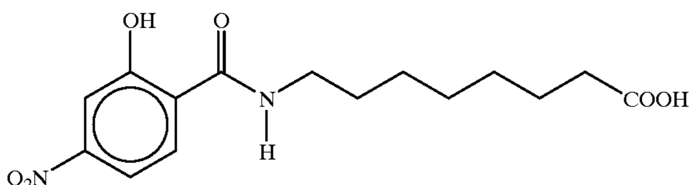
8-(N-2-hydroxy-4-nitrobenzoyl)aminocaprylic acid
