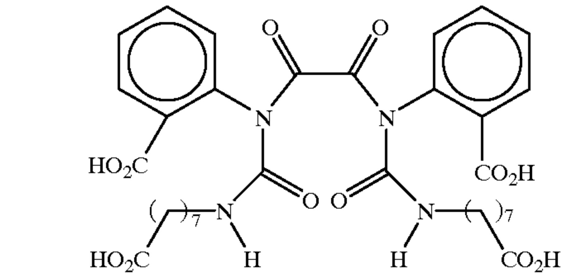
Bis(N-2carboxylphenyl-N-(N'-8-octanoic acid)ureal)oxalyl diamide
