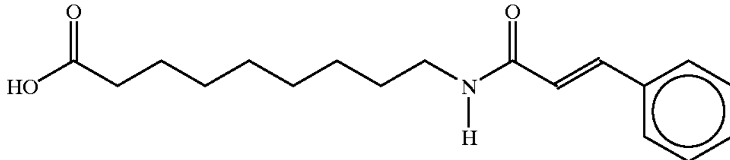
9-(cinnamoylamino)nonanoic acid
