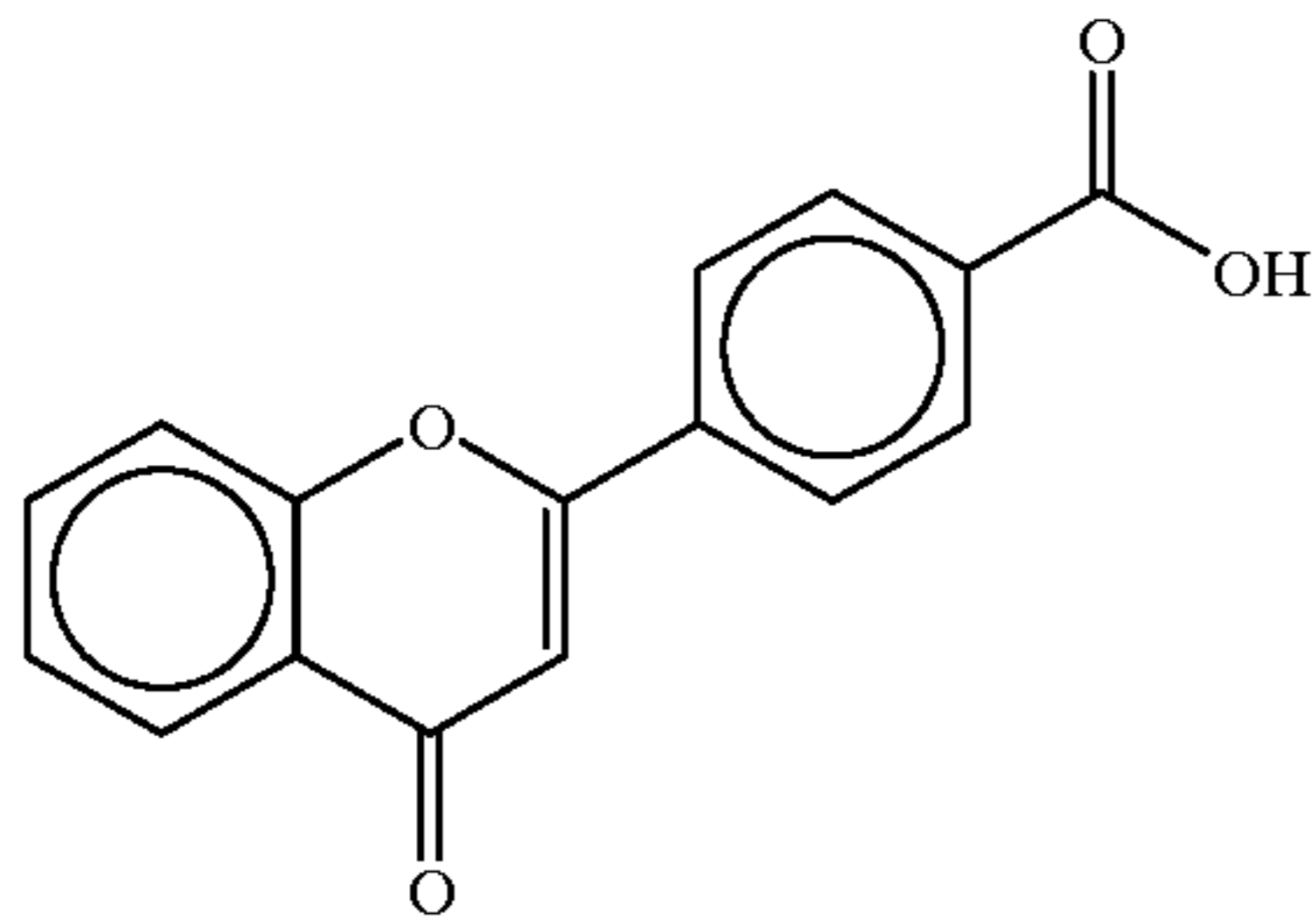
4'-flavonic acid
