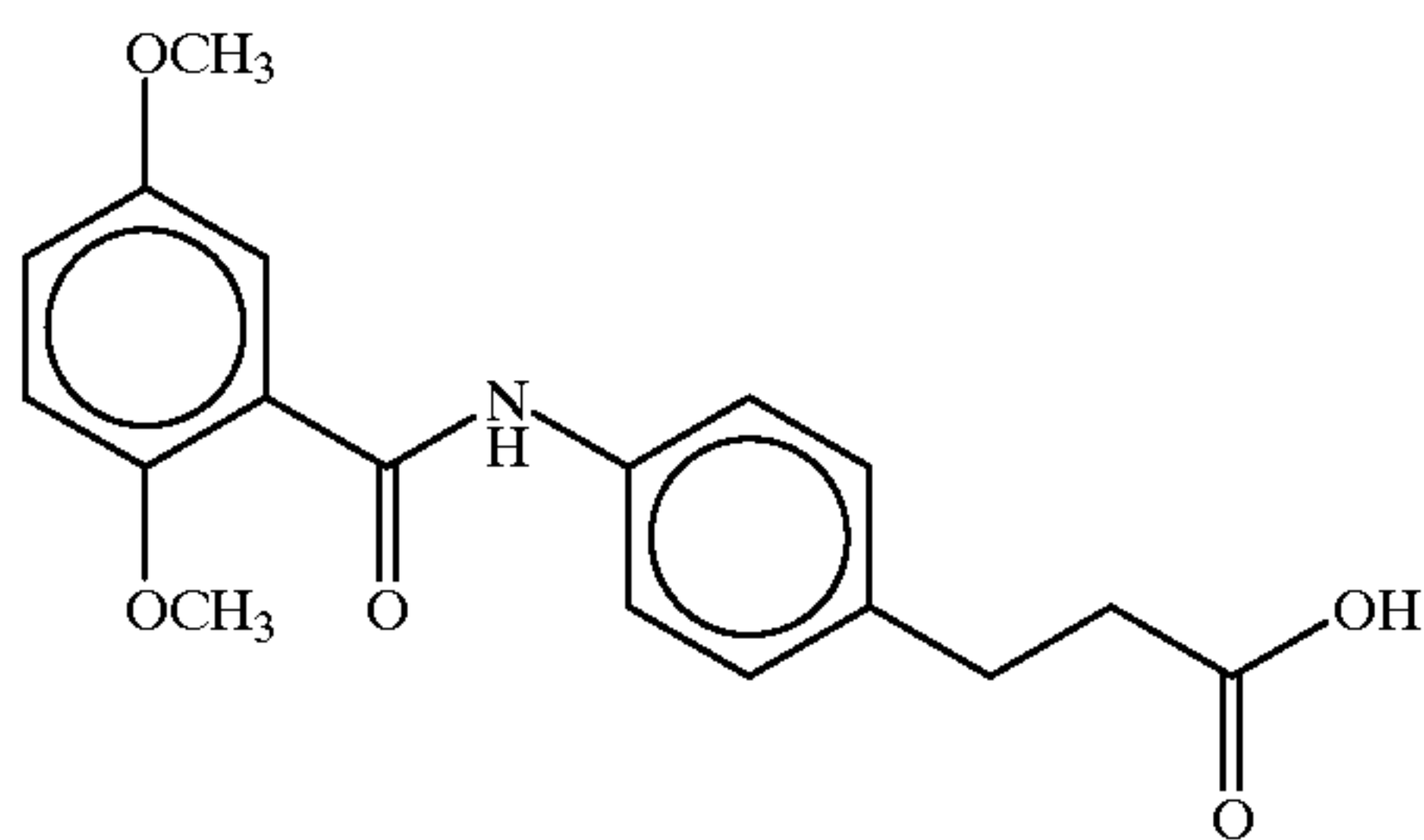
3-(4-(2, 5-dimethoxybenzoyl)aminophenyl)propionic acid
