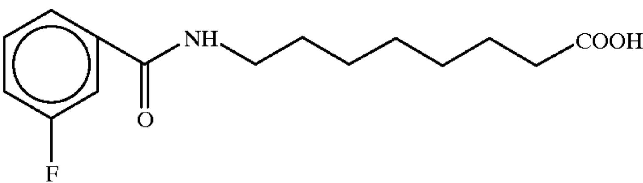
8-[N-(3-fluorobenzoyl)]aminocaprylic acid
