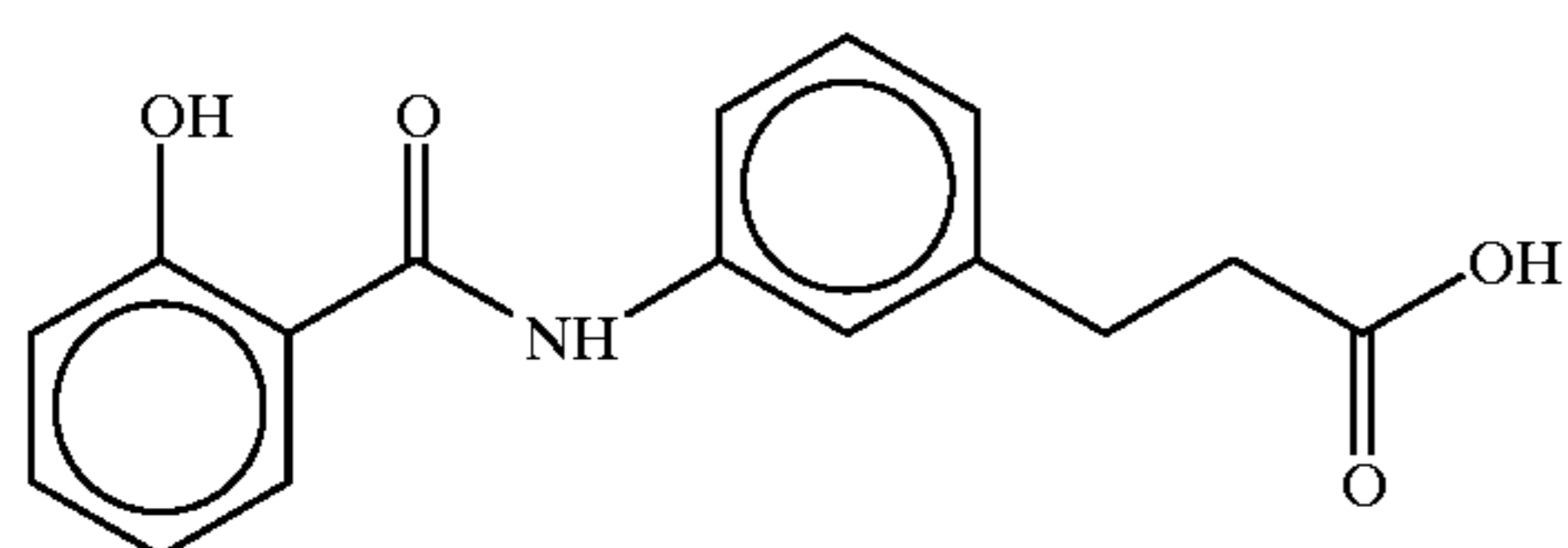
3-(3-(salicyloyl)aminophenyl)propionic acid
