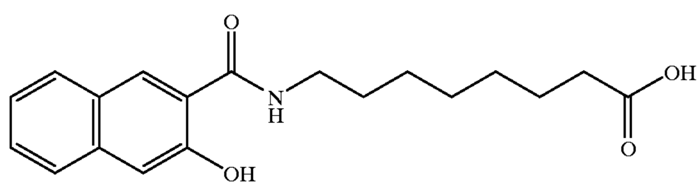
8-(3-hydroxy-2-naphthoyl)aminocaprylic acid
