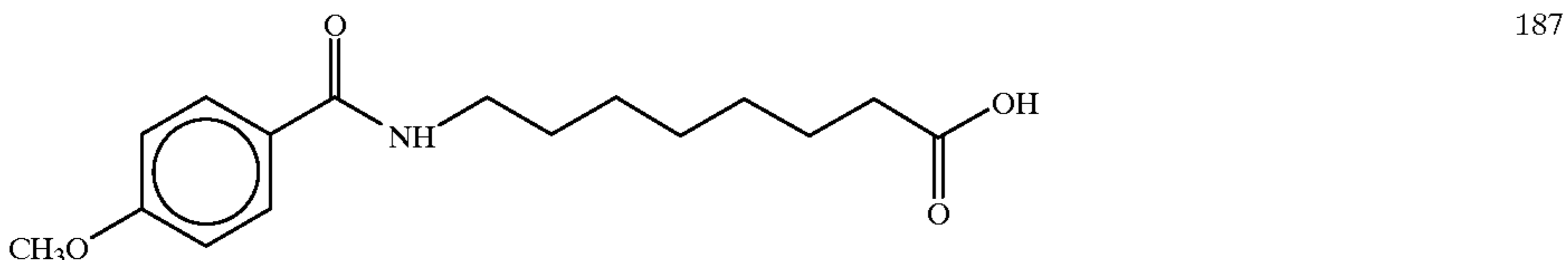
8-(p-anisoyl)aminocaprylic acid
