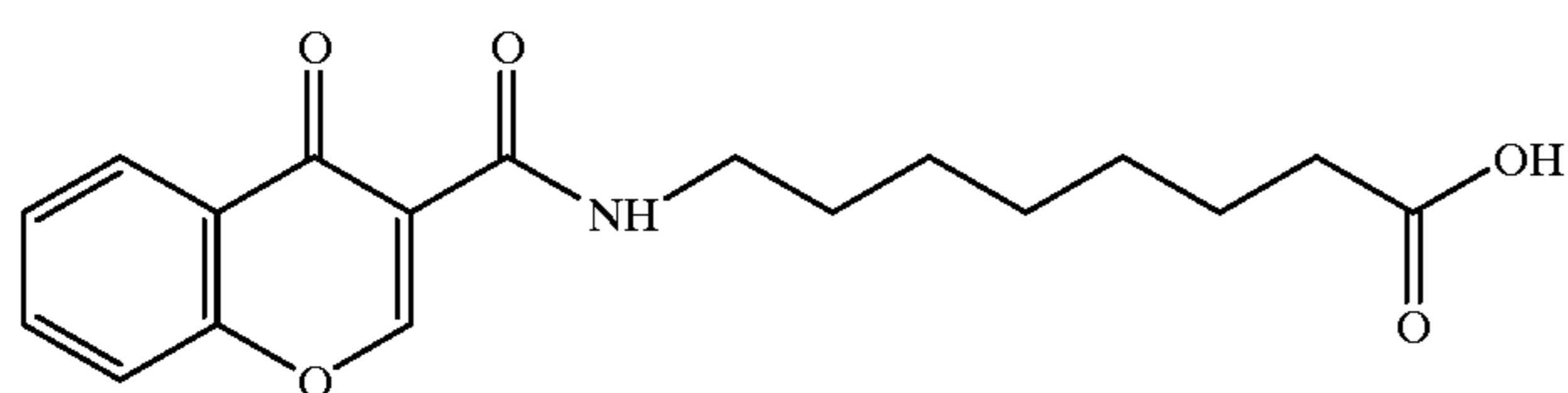
8-(chromone-3-carbonyl)aminocaprylic acid
