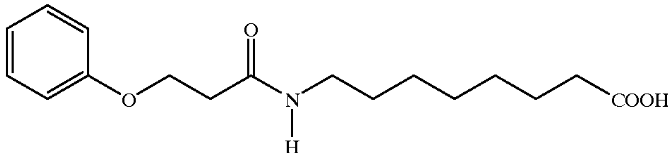
8-(3-Phenoxypropionylamino)caprylic acid
