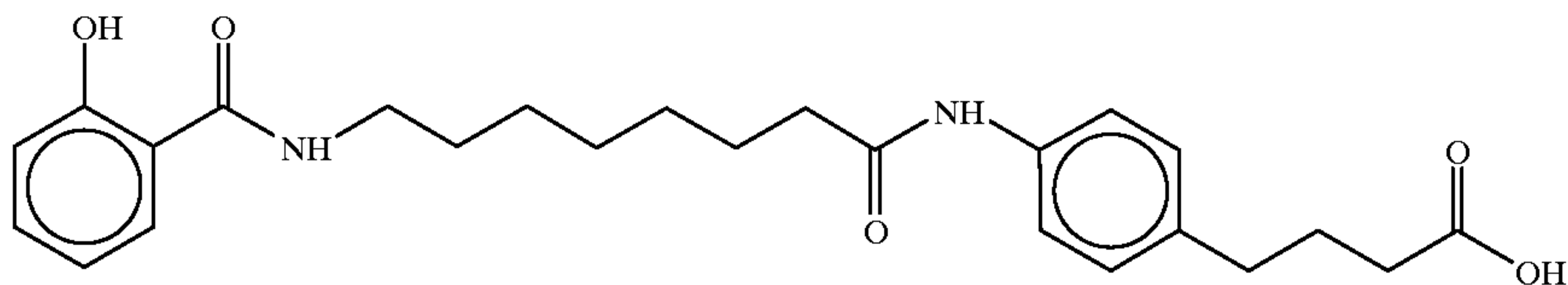
4-(4-(N-8(N-Salicyloyl)aminocaprylic)aminophenyl)butyric acid
