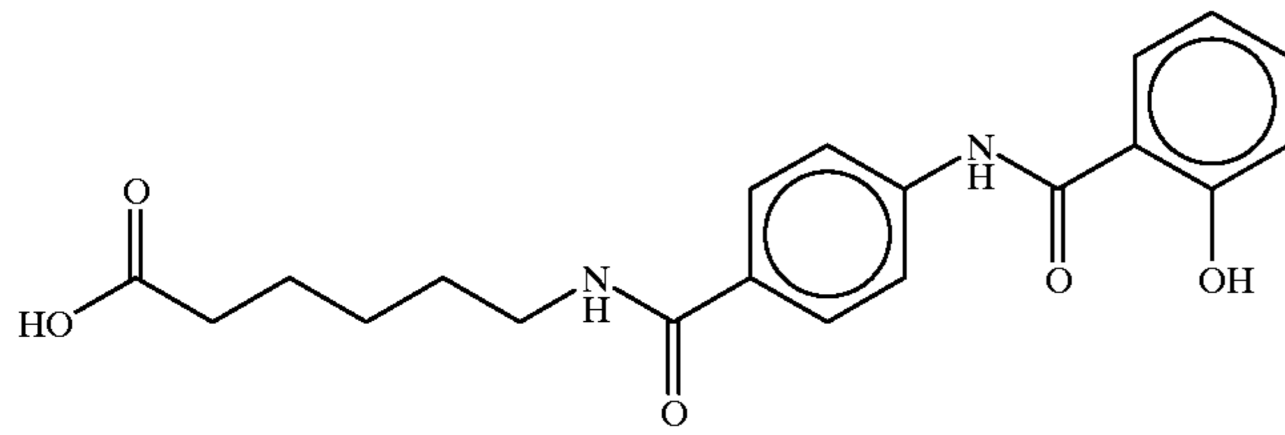
N-(4-salicyloylamino)-6-caproic acid
