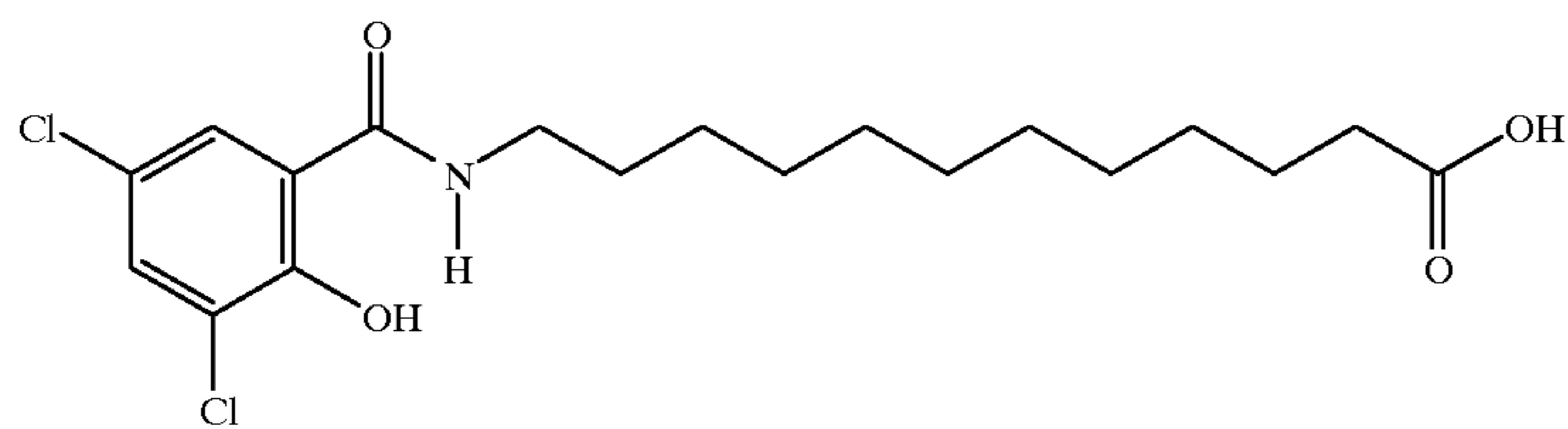
12-N-(3,5-dichloro-2-hydroxybenzoyl)aminododecanoic acid
