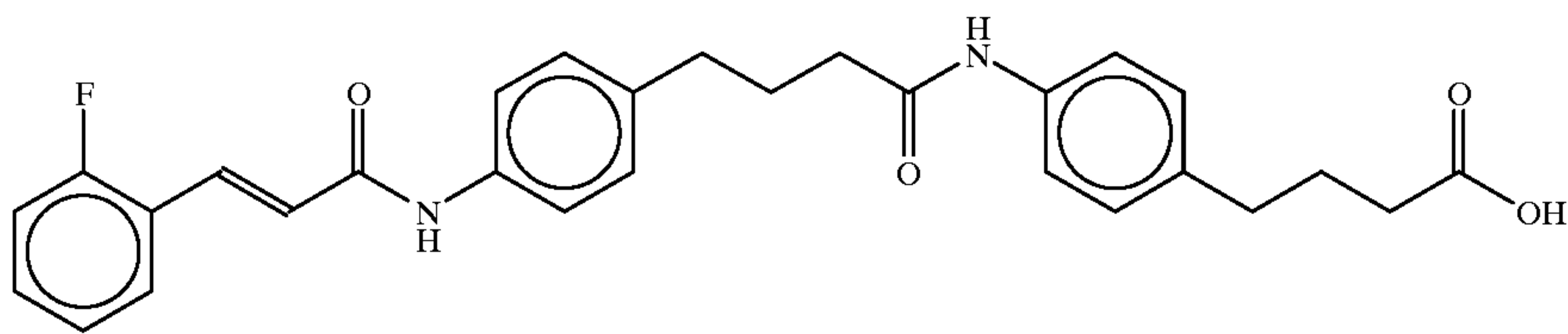
4-(4-(N-(2-Fluorocinnamoyl))aminophenyl) butyric
