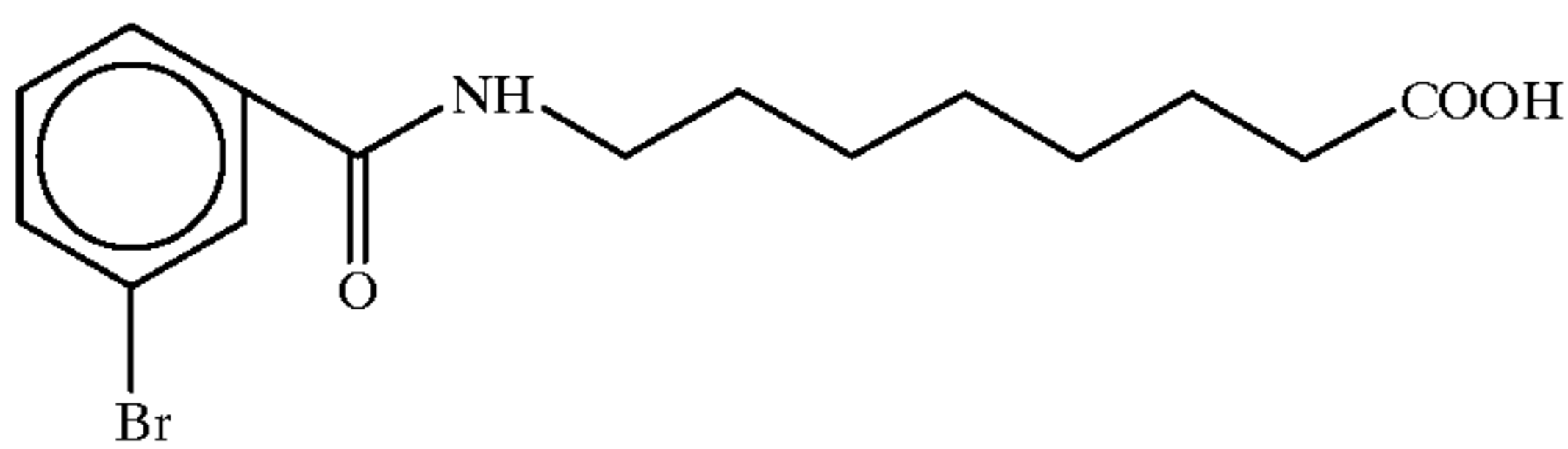
8-[N-(3-bromobenzoyl)]aminocaprylic acid
