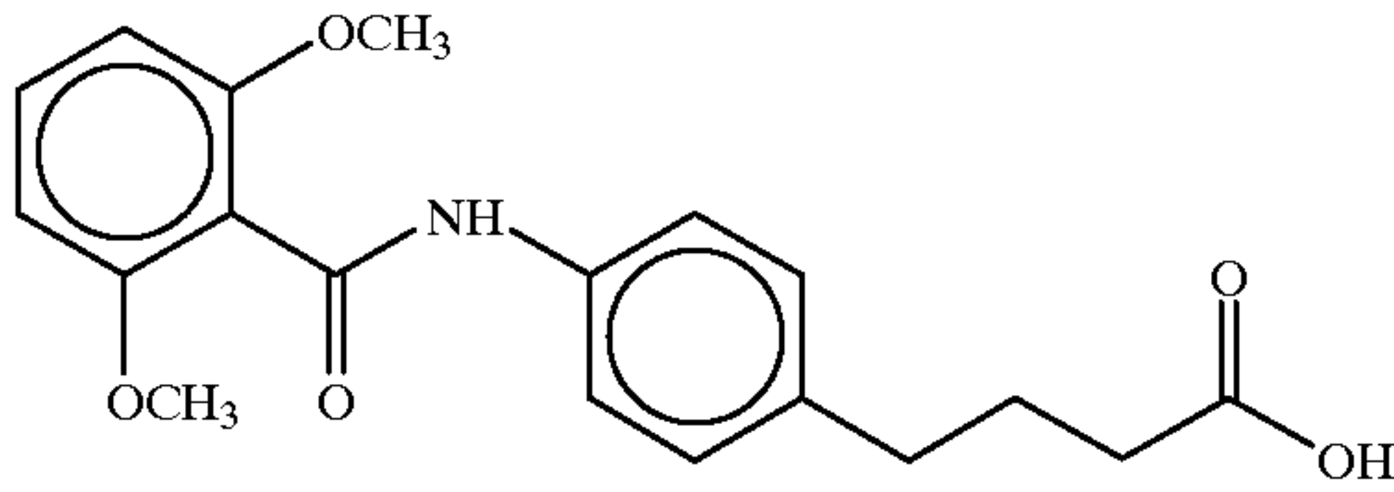
4-(4-(2, 6-dimethoxybenzoyl)aminophenyl)butyric acid
