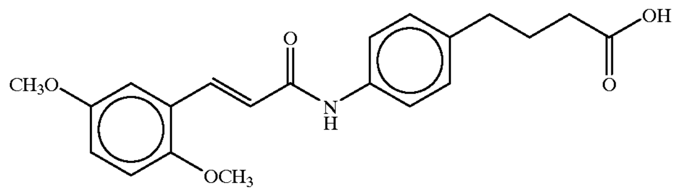
4-(4-(2,5-dimethoxycinnamoyl)aminophenyl)butyric acid
