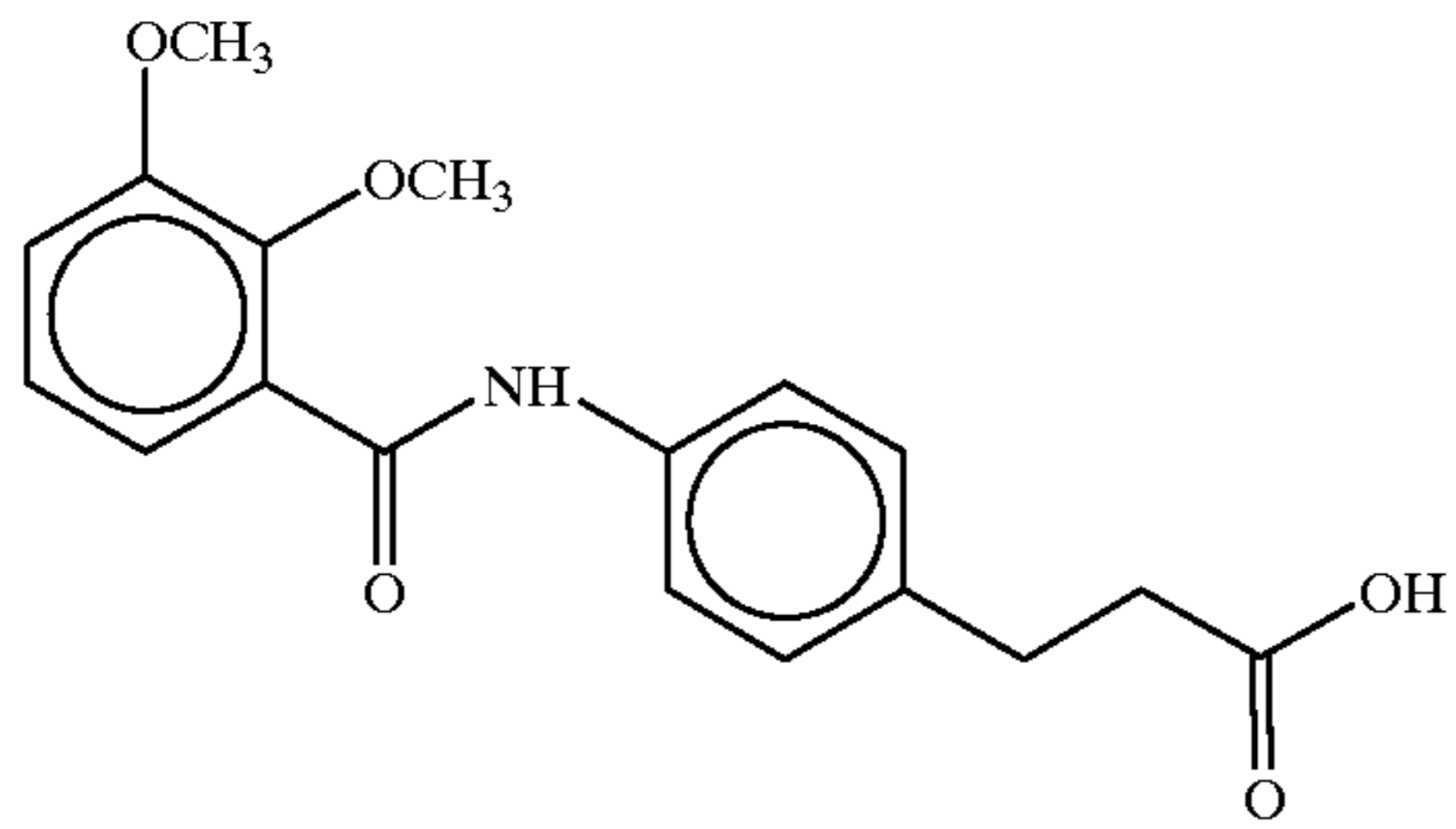
3-[4-(2,3-dimethoxybenzoyl)aminophenyl]propionic acid
