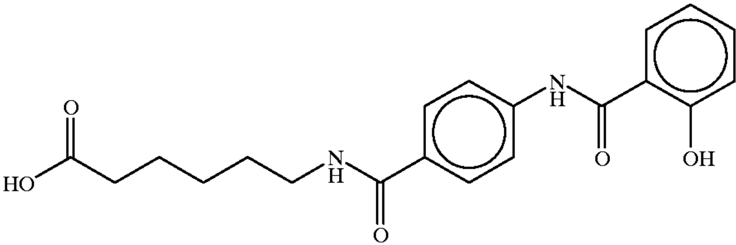
N-(4-salicyloylamino)-6-caproic acid
