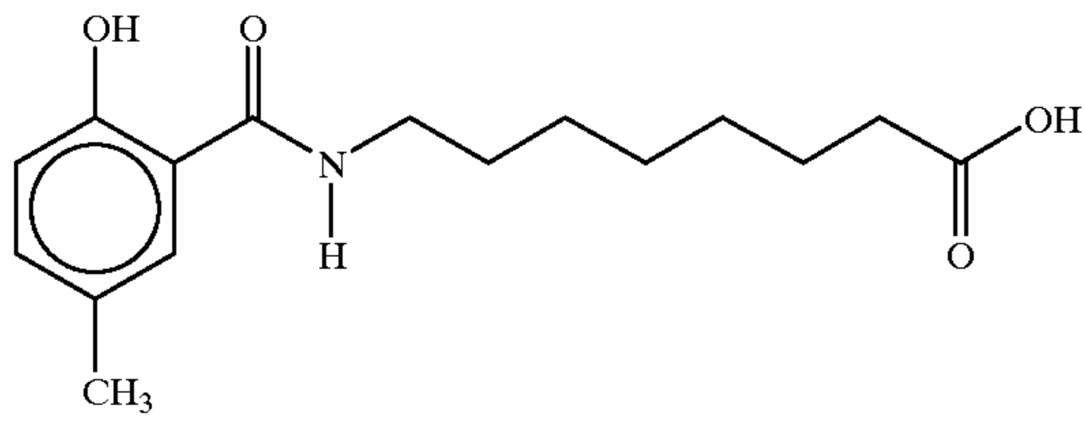
8-(N-5-methylsalicyloyl)aminocaprylic acid
