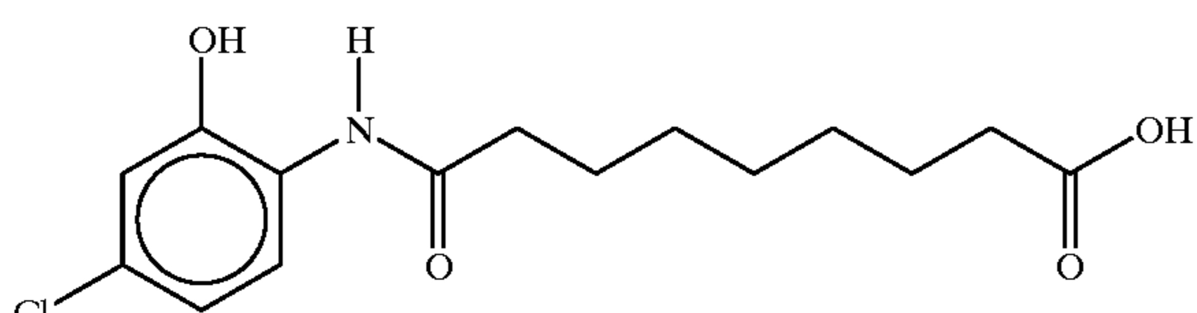
8-(2-hydroxy-5-chloroanilincarbonyl)octanoic acid
