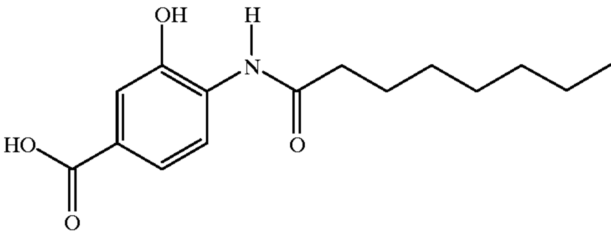
4-octanoylamino-3-hydroxybenzoic acid
