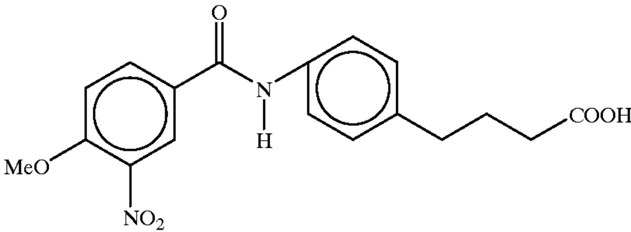
4-[4 N-(4-methoxy-3-nitrobenzoyl)aminophenyl]butyric acid
