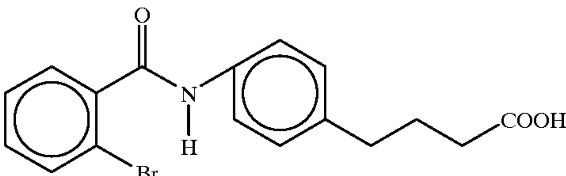
4-{4-[N-2-bromobenzoyl]} aminophenyl} butyric acid
