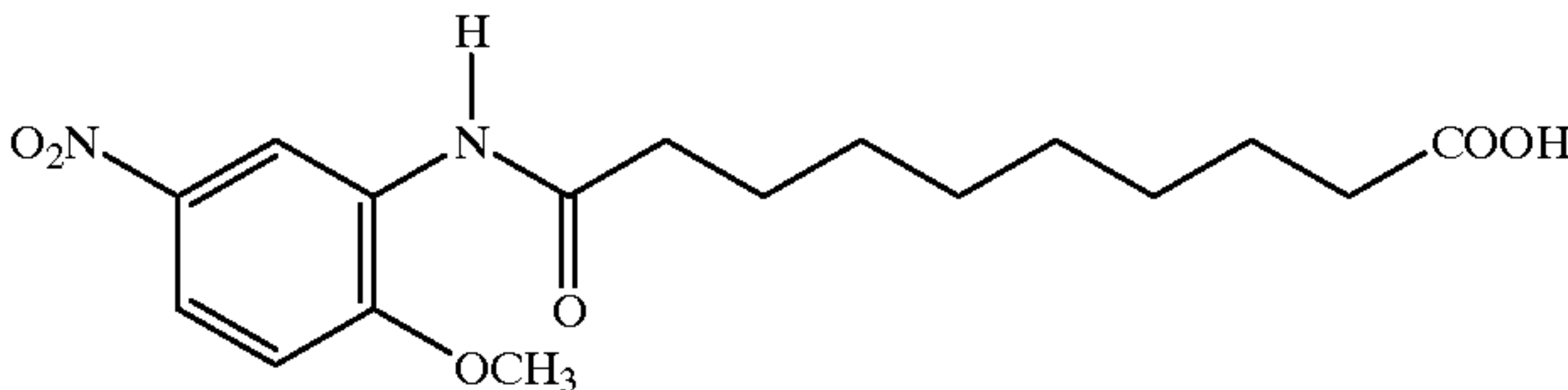
N-(2-methoxy-5-nitrophenyl) sebecoyl amide acid
