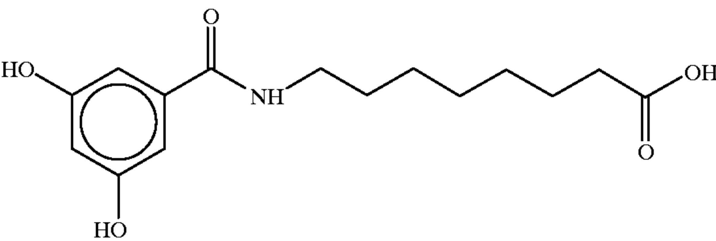
8-(N-3, 5 Dihydroxybenzoyl)aminocaprylic acid
