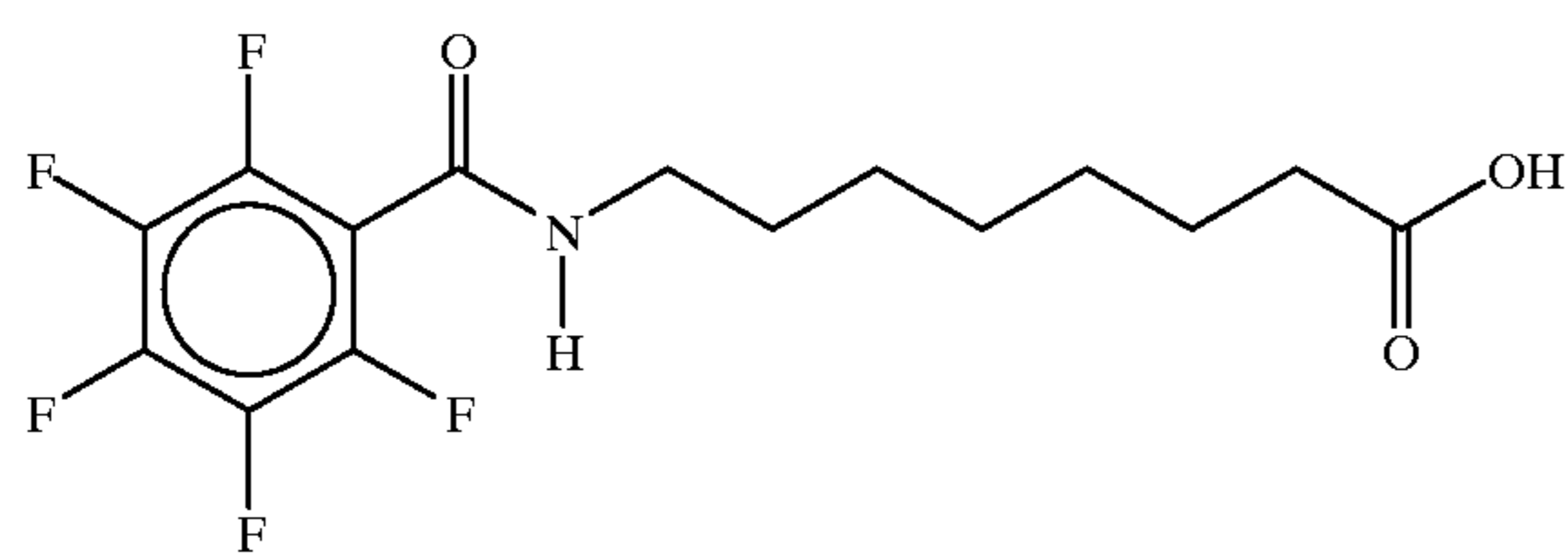
8-(pentafluorobenzoyl)aminocaproic acid
