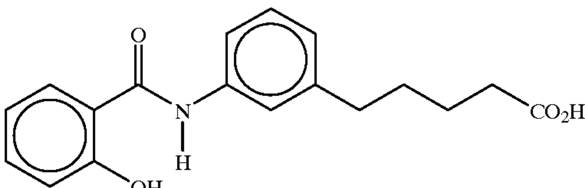
N-Salicyl-5-(3-aminophenyl)valeric acid
