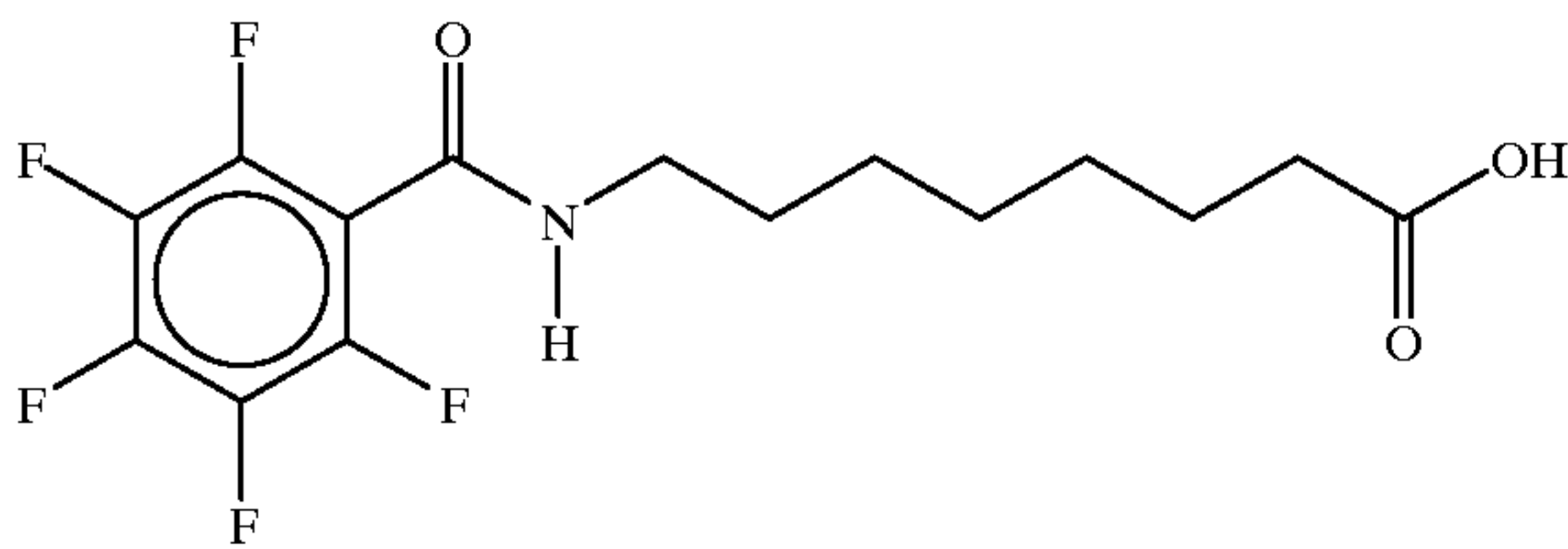
8-(pentafluorobenzoyl)aminocaprylic acid
