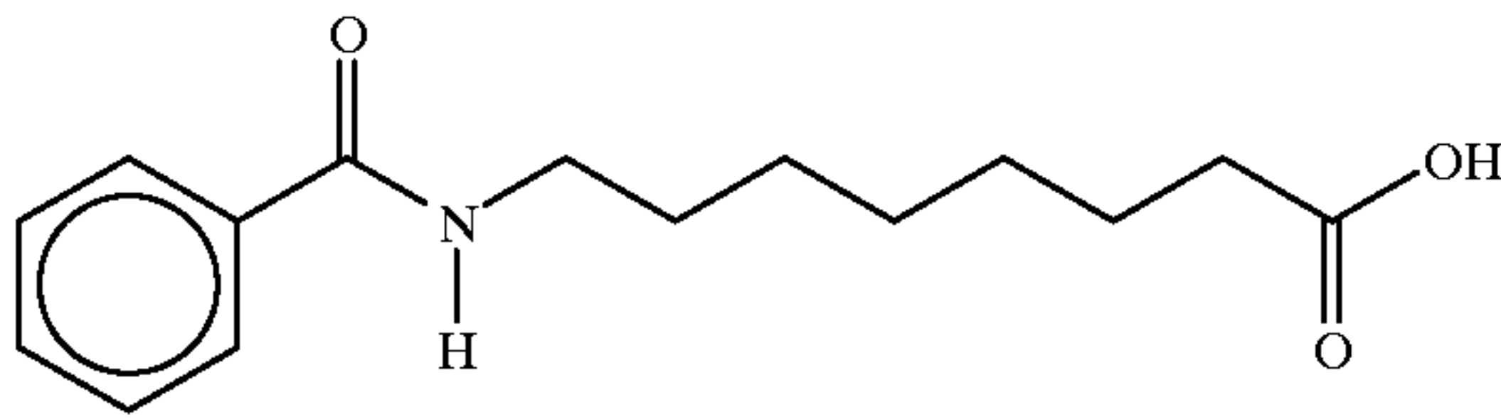
8-(N-benzoyl)aminocaprylic acid
