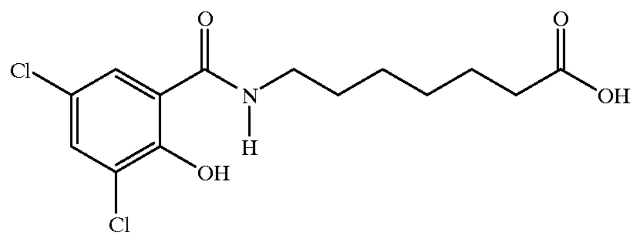
7-N-(3,5-dichloro-2-hydroxybenzoyl)aminoheptanoic acid
