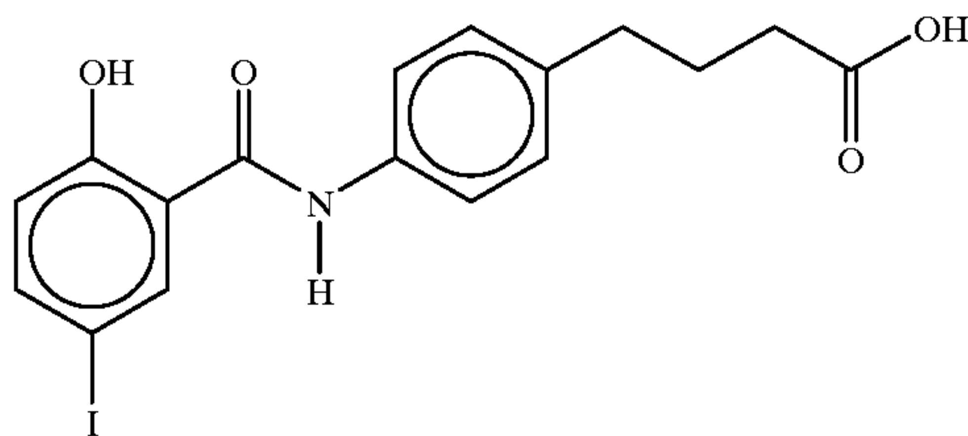
4-{-[N-(2-hydroxy-5-iodobenzoyl)]aminophenyl}butyric acid
