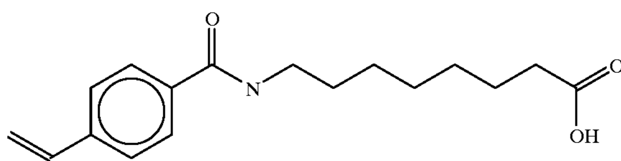
8-(vinylbenzoyl)aminocaprylic acid
