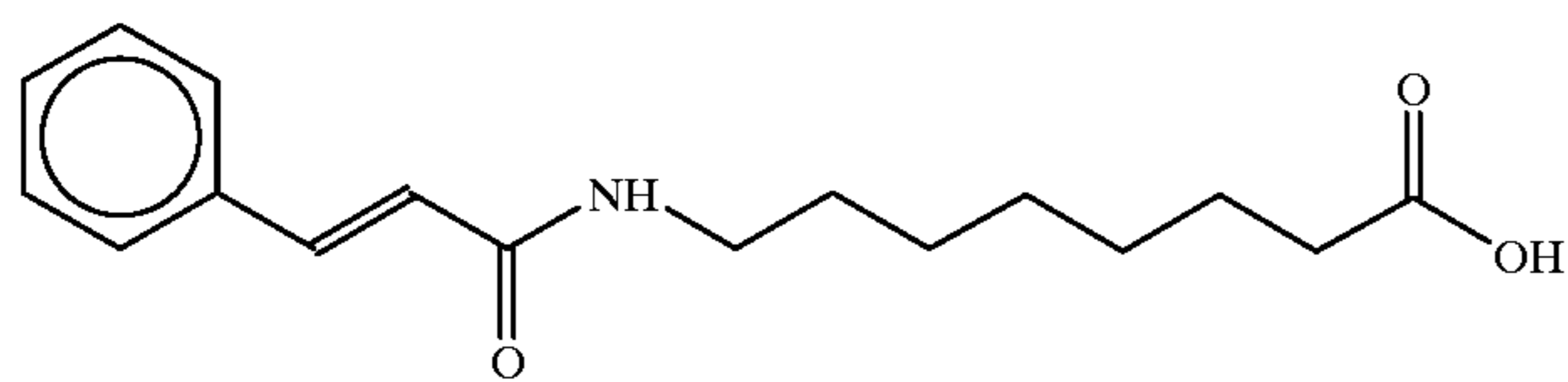
8-cinnamoylaminocaprylic acid
