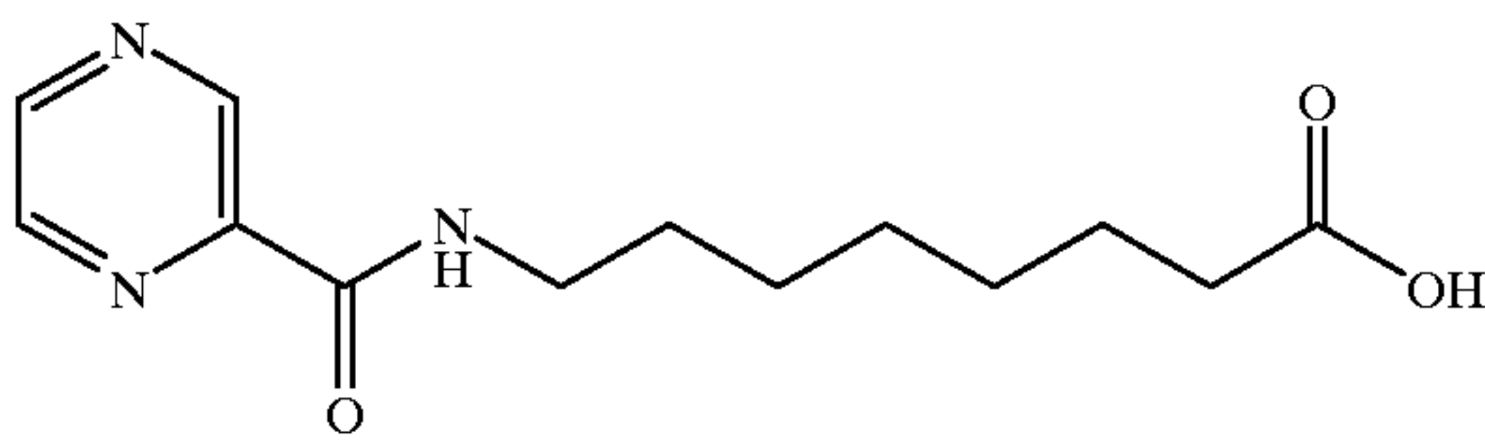
8-(2-pyrazinecarbonyl)aminocaprylic acid
