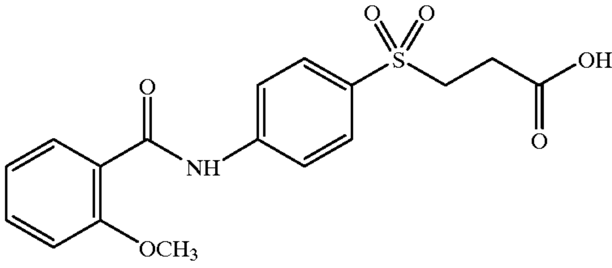
4-(2-methoxybenzoyl)amino 3-carboxypropylsulfone
