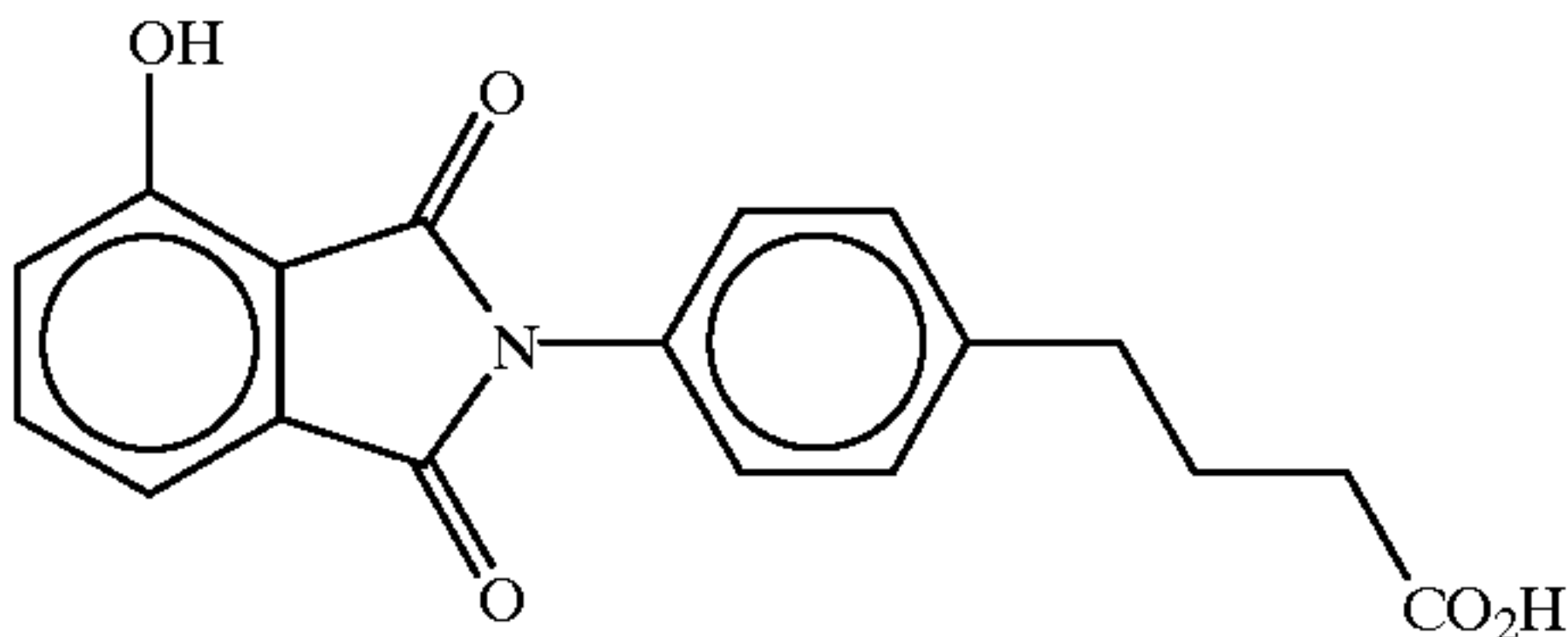
4-(4-(3-hydroxyphthalimido)phenyl)butyric acid
