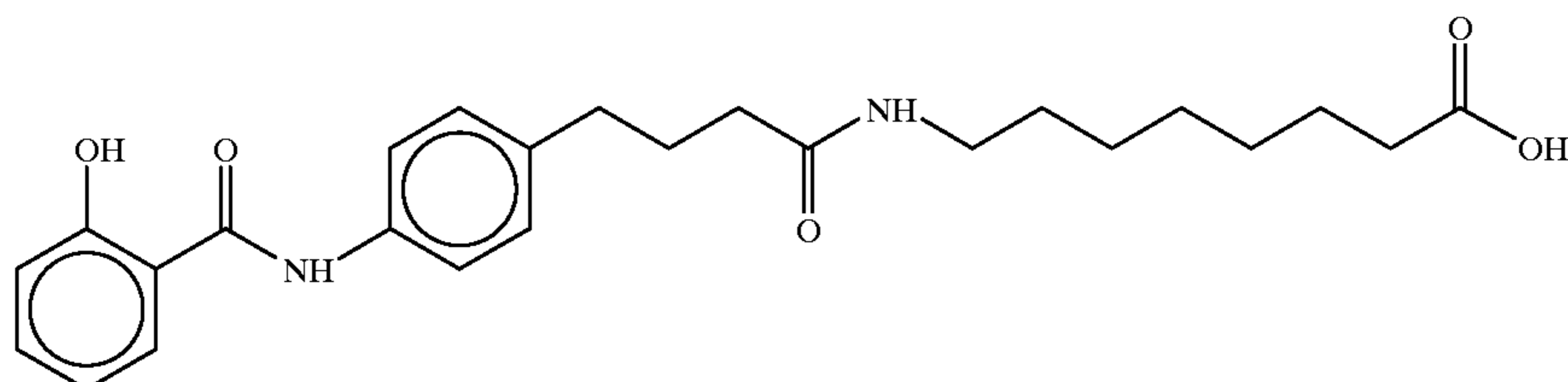
8-(4-(N-Salicyloyl-4aminophenyl)butyric)aminocaproic acid
