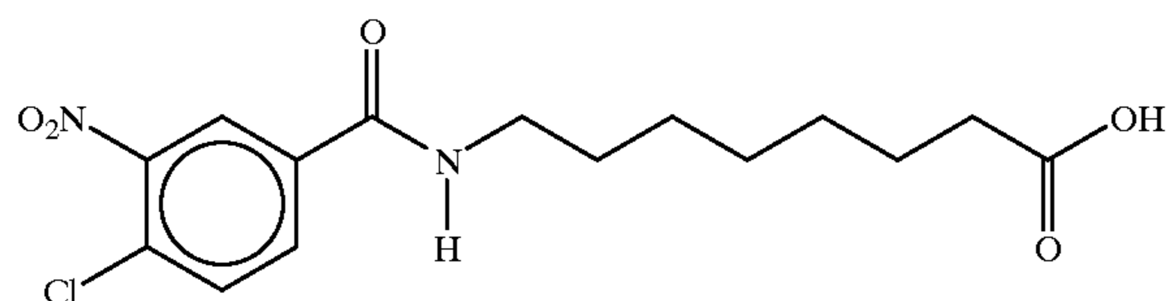
8-(4-chloro-3-nitrobenzoyl)aminocaprylic acid
