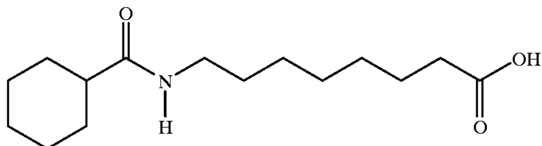
8-N-cyclohexanoylaminovaleric acid
