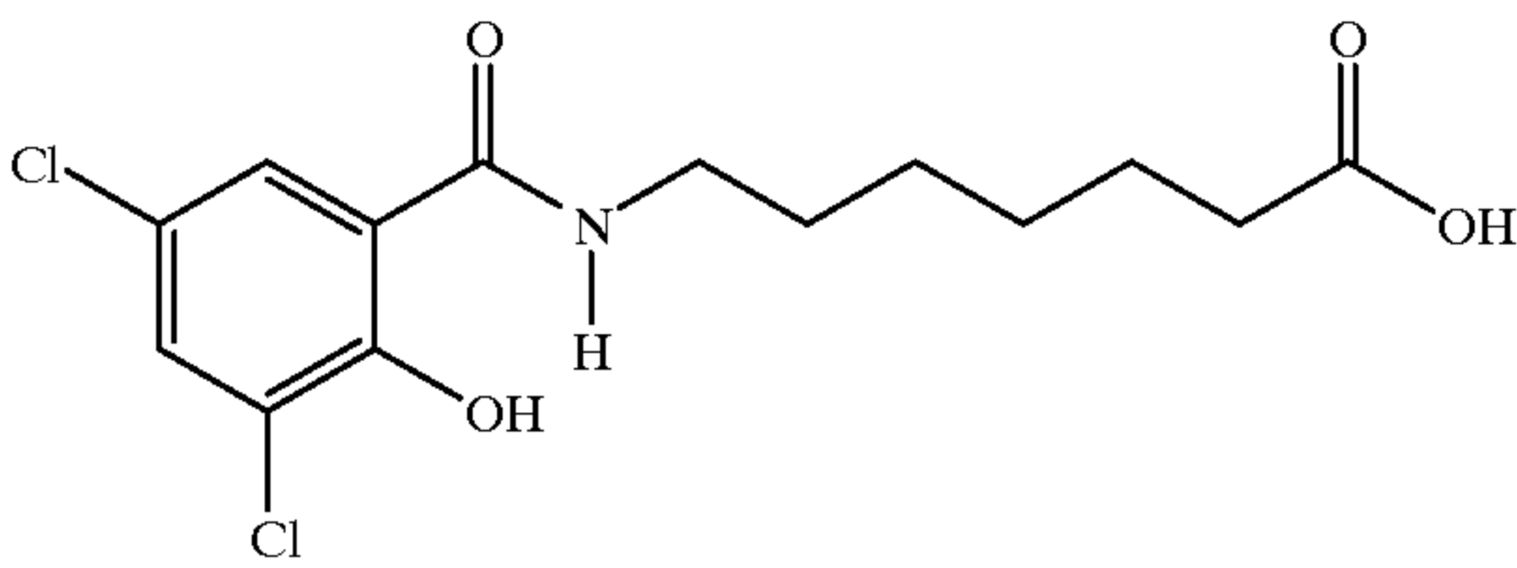
7-N-(3, 5-dichloro-2-hydroxybenzoyl)aminoheptanoic acid
