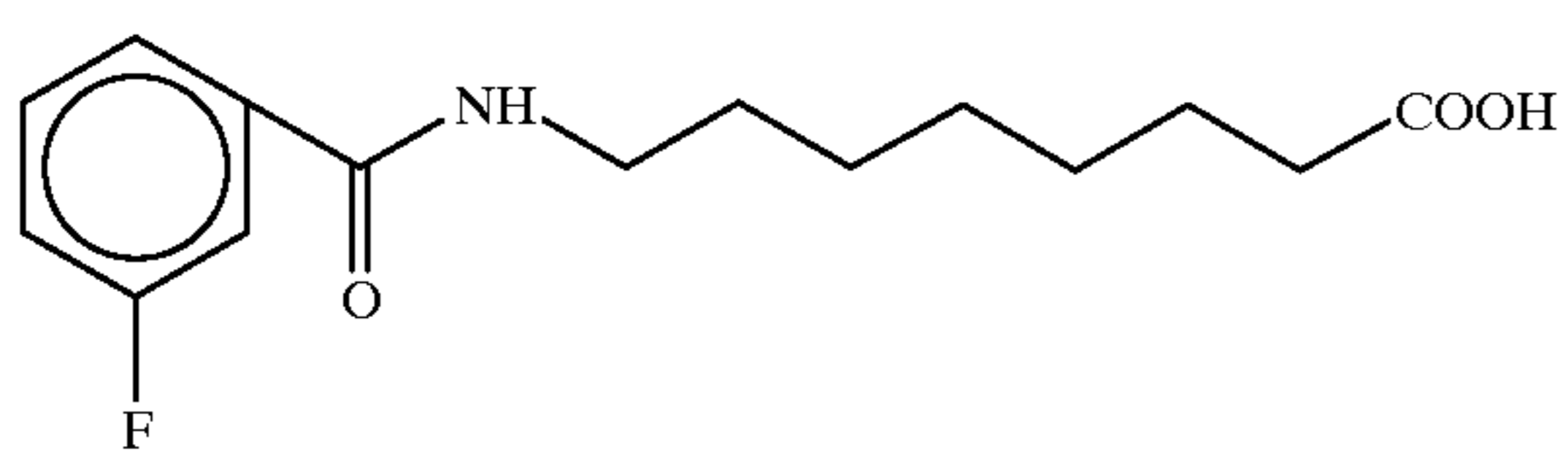
8-[N-(3-fluorobenzoyl)]aminocaproic acid
