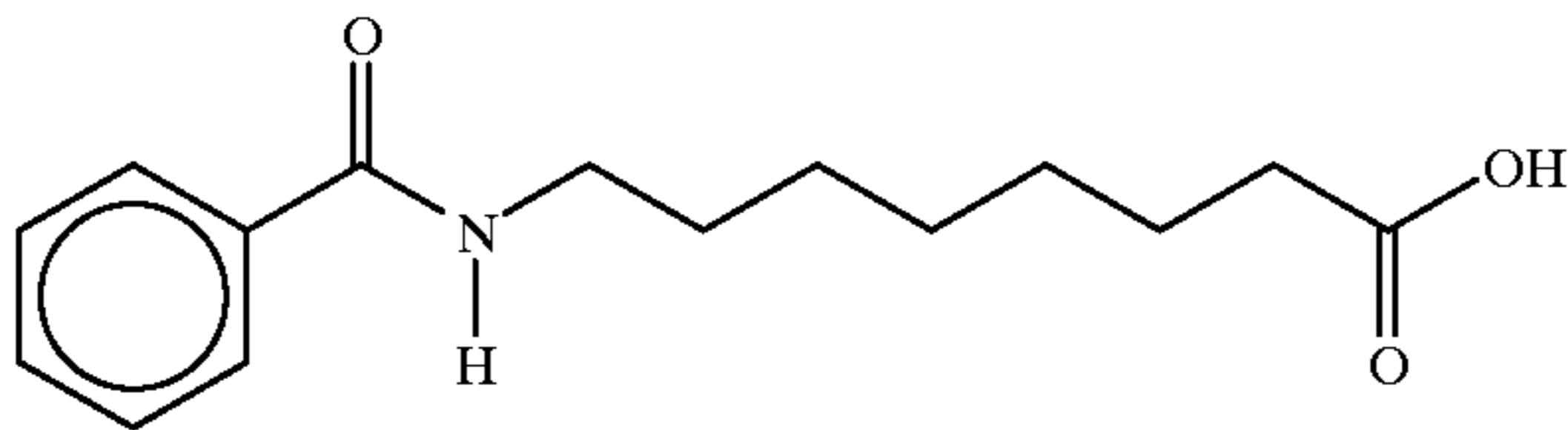
8-(N-benzoyl)aminocaprylic acid
