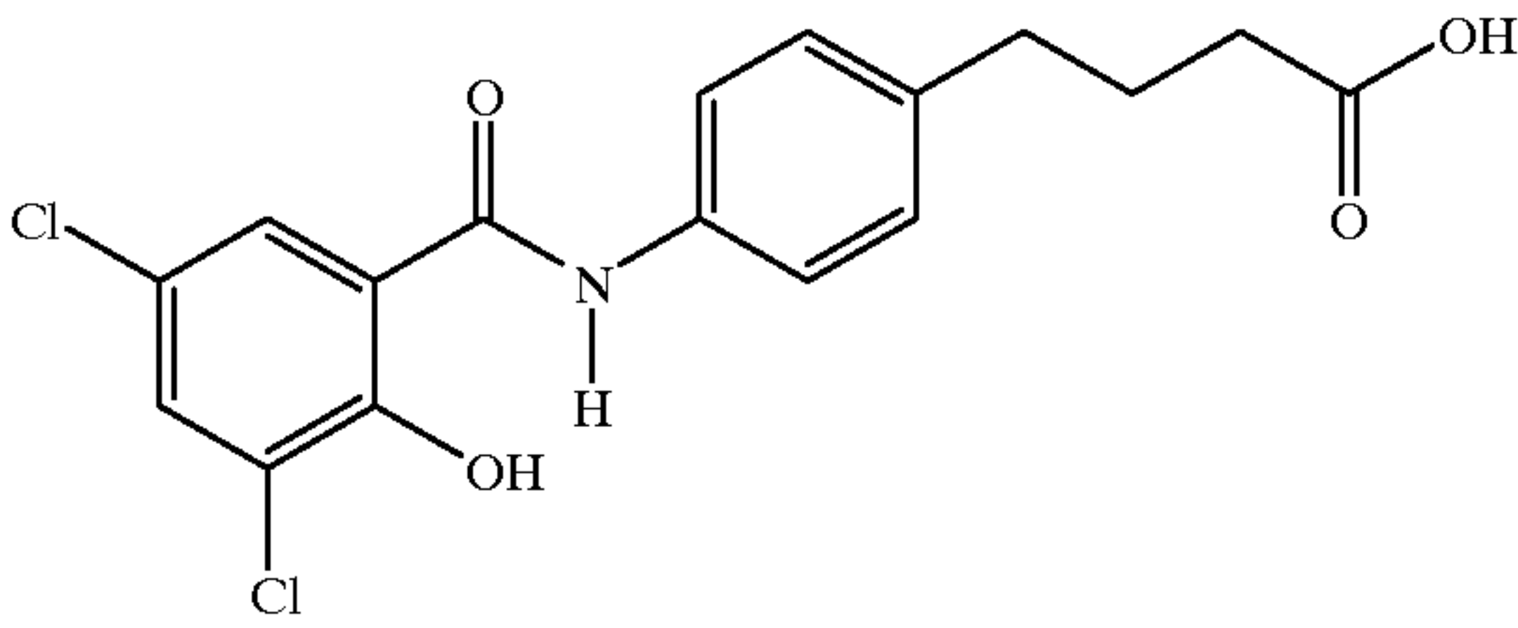
N-[3, 5-dichloro-2-hydroxybenzoyl-4(4-aminophenyl)]butyric acid
