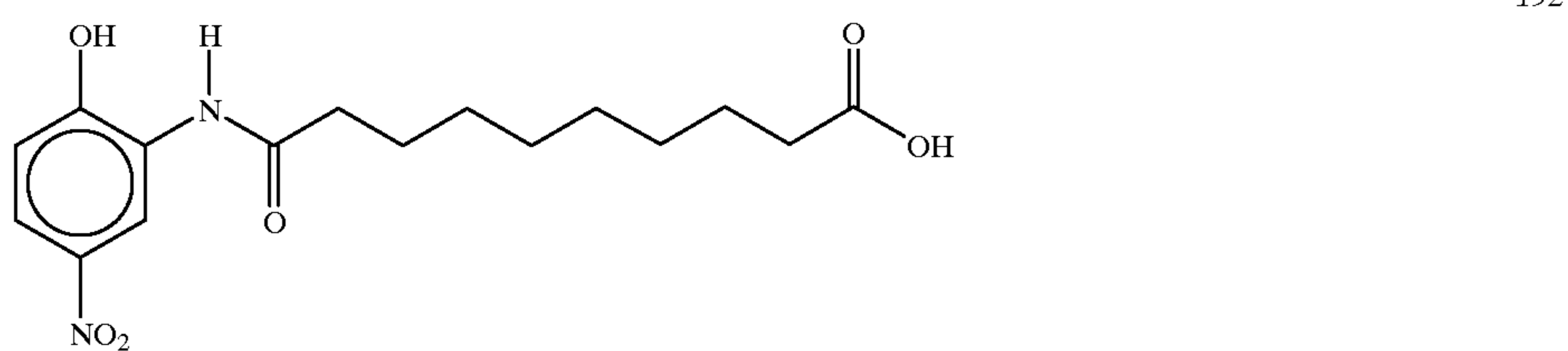
N-10-(2-hydroxy-5-nitroanilino)decanoic acid
