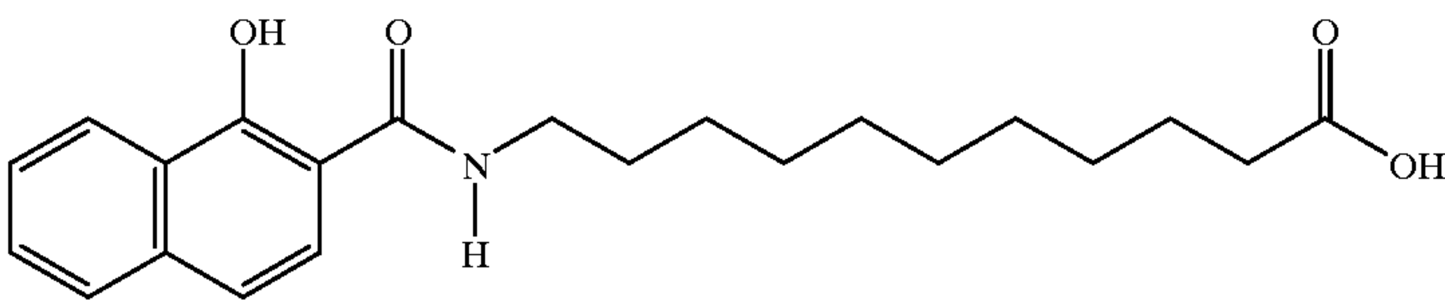
11-N-(1-hydroxy-2-naphthoyl)aminoundecanoic acid
