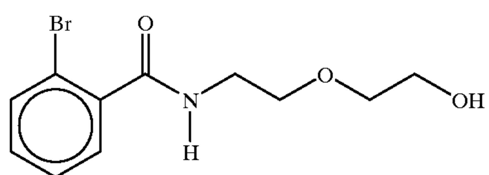
2-[N-(2-bromobenzoyl)aminoethoxy]ethanol
