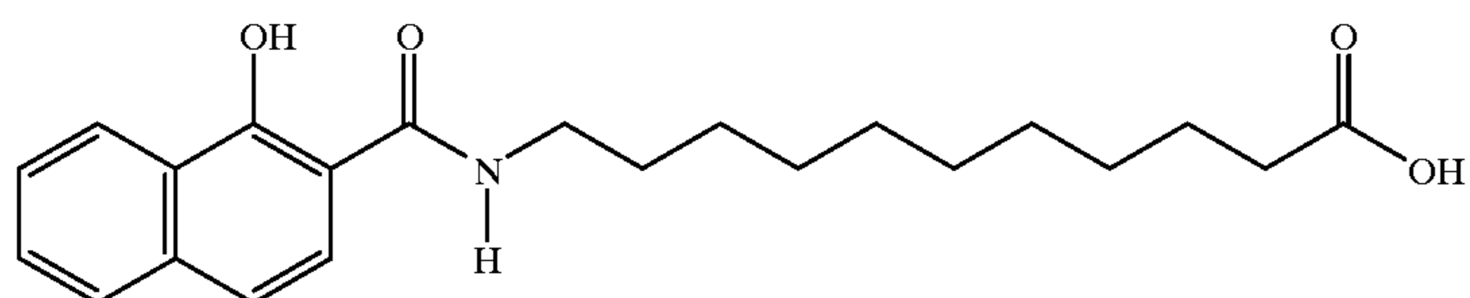
11-N-(1-hydroxy-2-naphthoyl)aminoundecanoic acid
