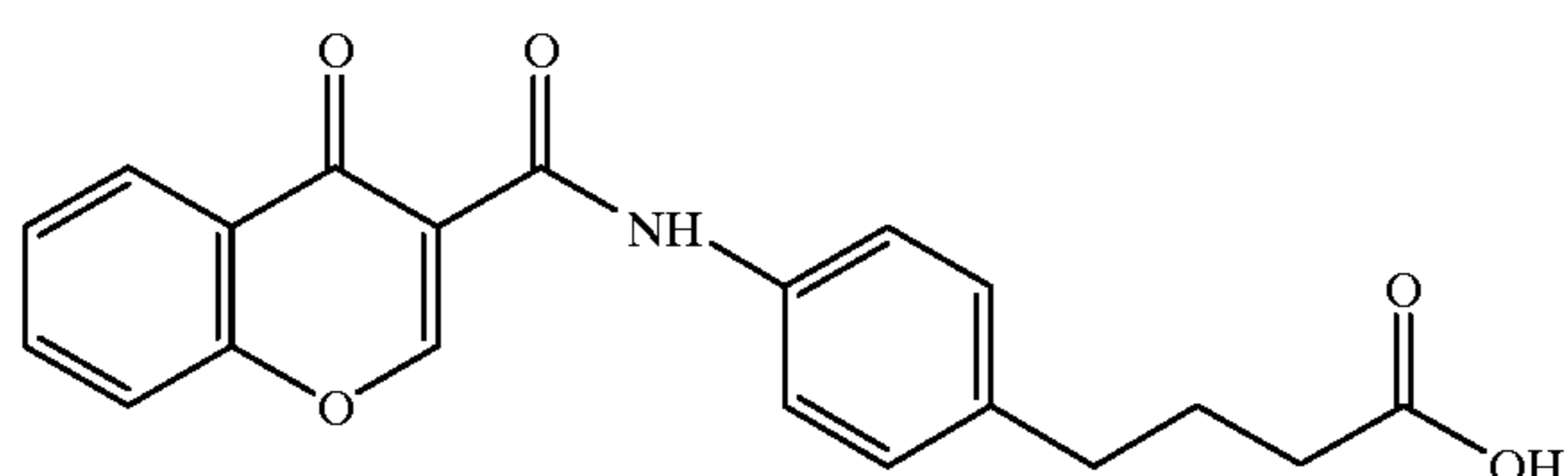
4-(4-(chromone-3-carbonyl)aminophenyl)butyric acid
