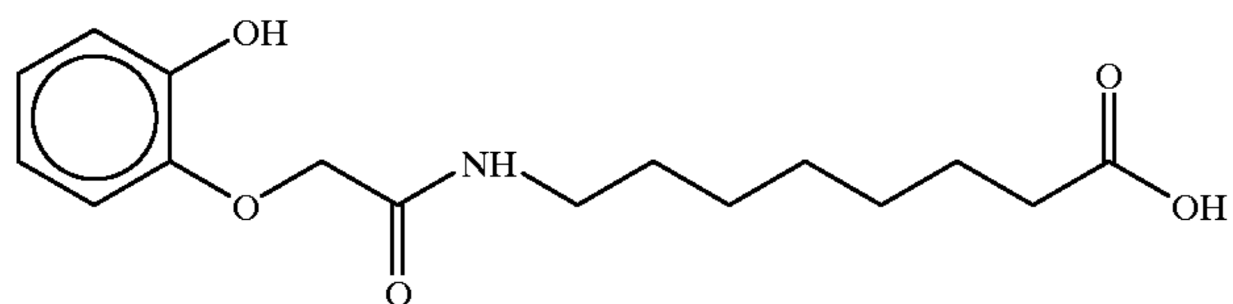
7-(2-hydroxyphenoxyacetyl)aminocaproic acid
