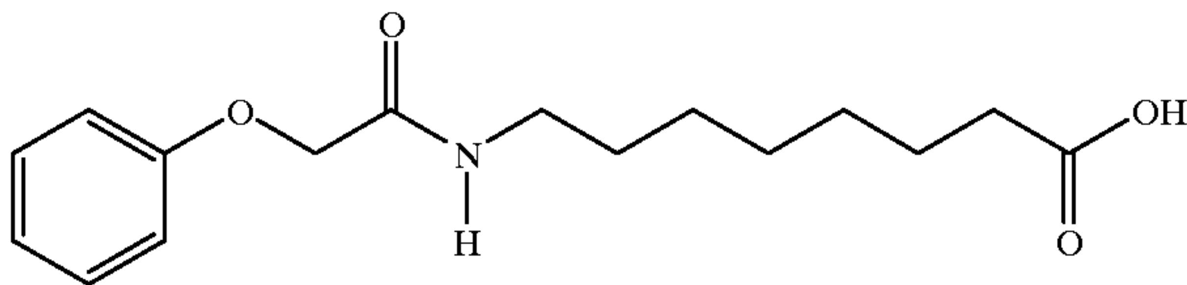
8-(Phenoxyacetyl)amino caprylic acid
