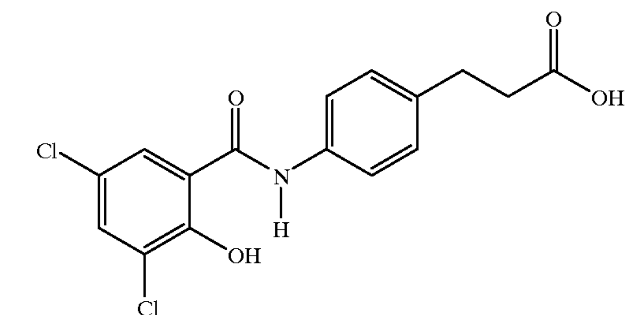
N-[3,5-dichloro-2-hydroxybenzoyl-3-(4-aminophenyl)]propionic acid
