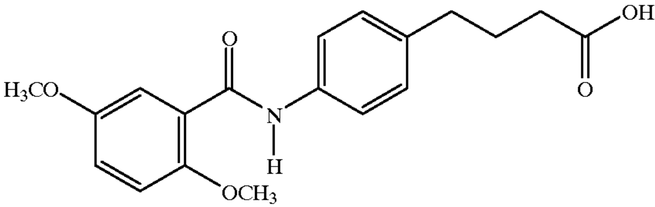
4-(4-(2, 5-dimethoxybenzoyl)aminophenyl)butyric acid
