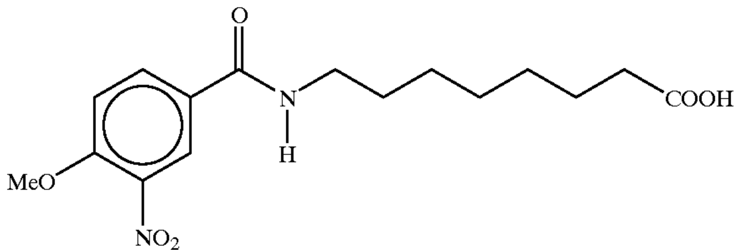
8-N-(4-methoxy-3-nitrobenzoyl)aminocaprylic acid
