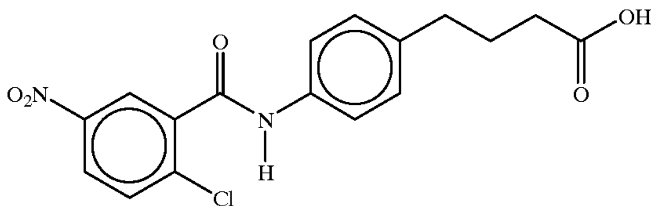
4-(4-(2-chloro-5-nitrobenzoyl)aminophenyl)butyric acid
