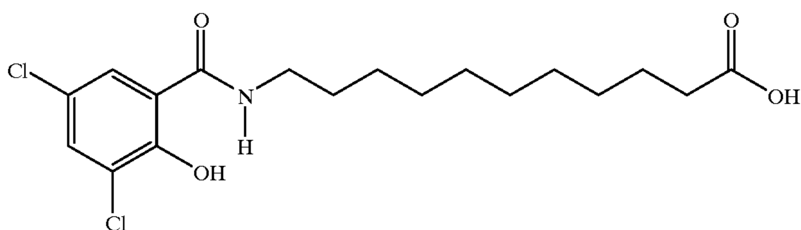
11-N-(3,5-dichloro-2-hydroxybenzoyl)aminoundecanoic acid
