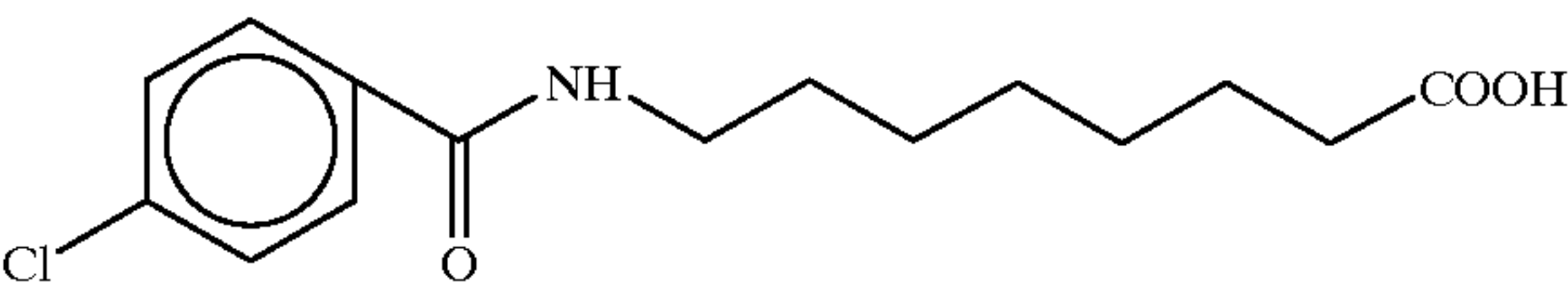
8-[N-(4-chlorobenzoyl)]aminocaprylic acid
