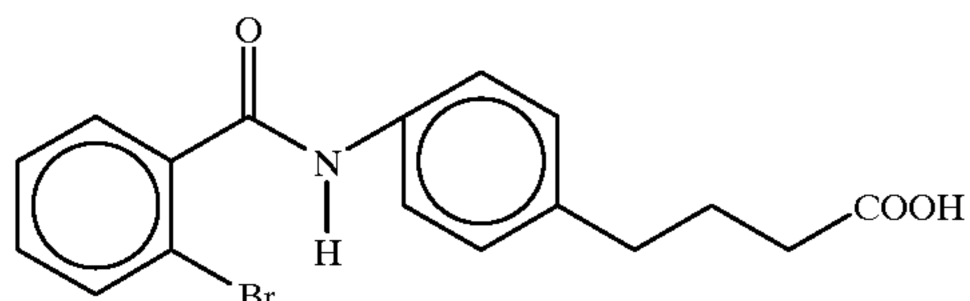
4-[4-[N-(2-bromobenzoyl)]aminophenyl]butyric acid
