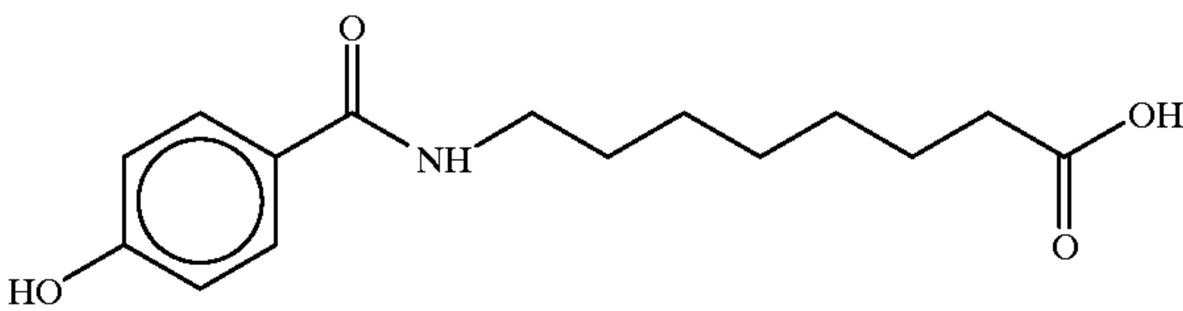
8-(4-Hydroxybenzoyl)aminocaprylic acid
