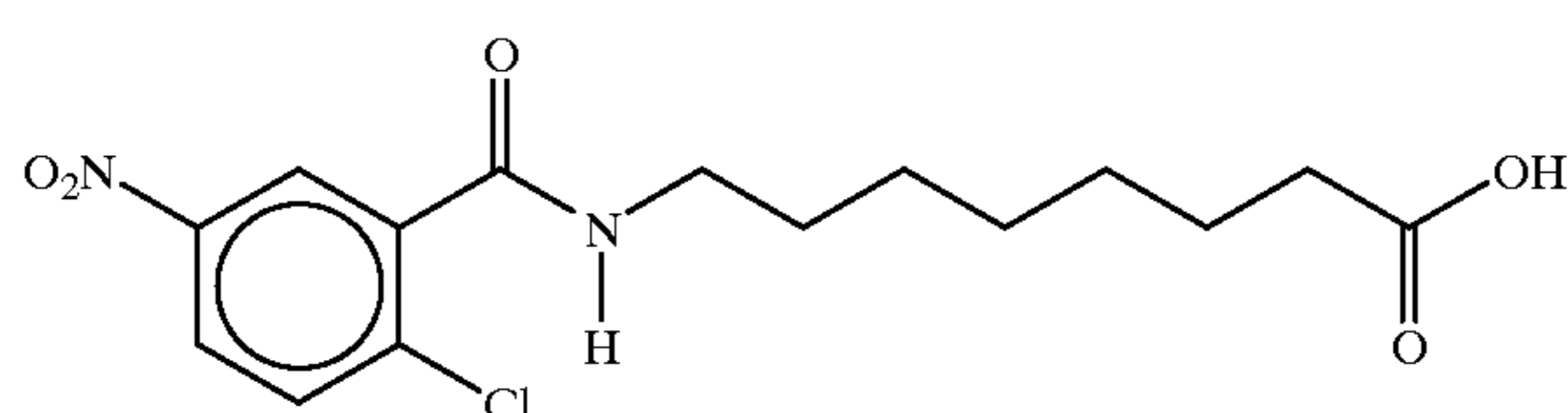
8-(2-chloro-5-nitrobenzoyl)aminocaprylic acid
