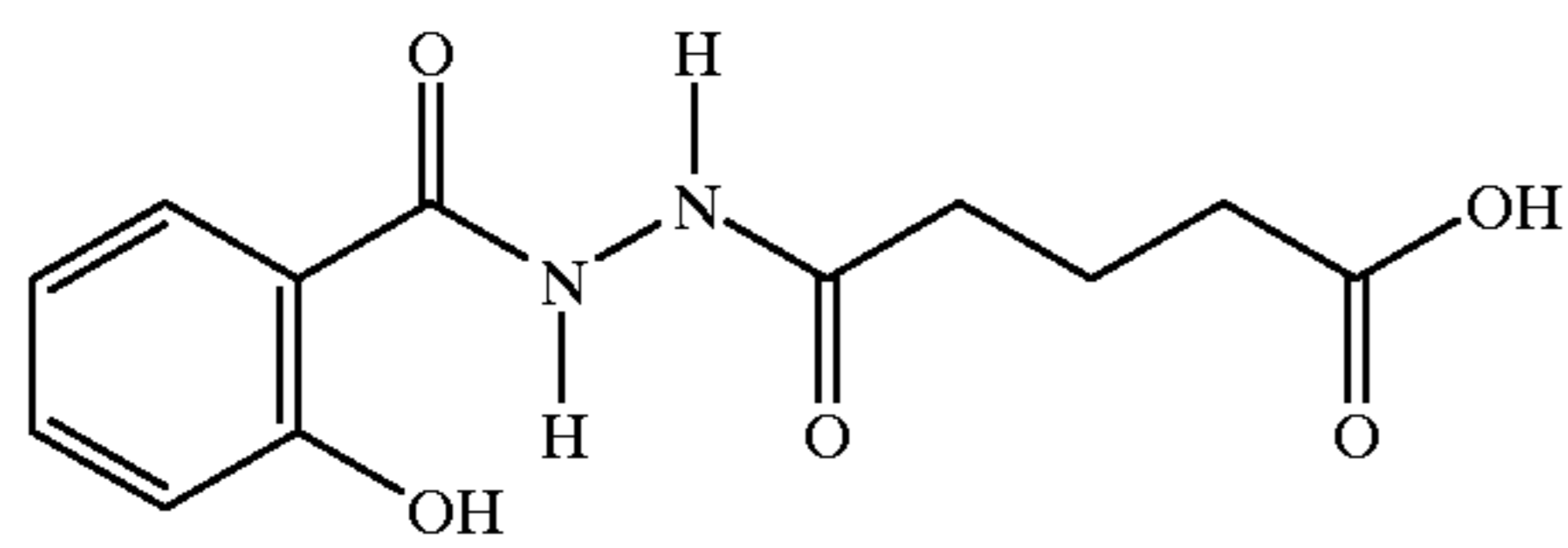
1-salicyloyl-2-glutaryl hydrazide
