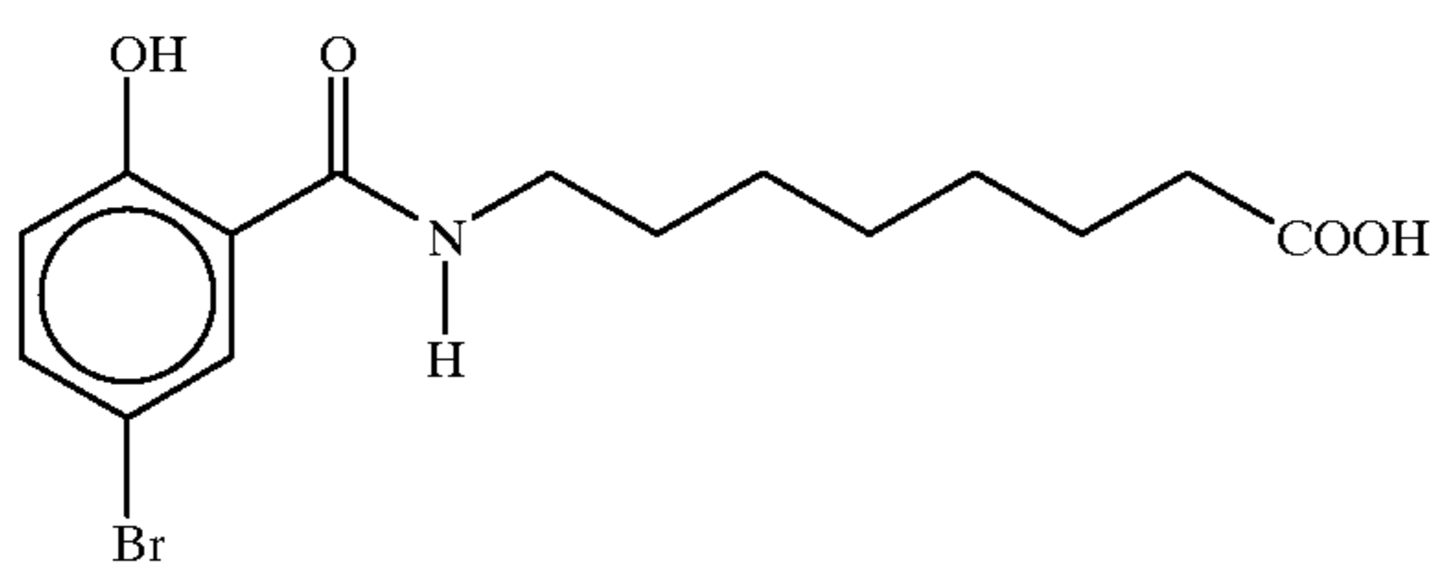
8-(N-(2-hydroxy-5-bromobenzoyl)aminocaprylic acid
