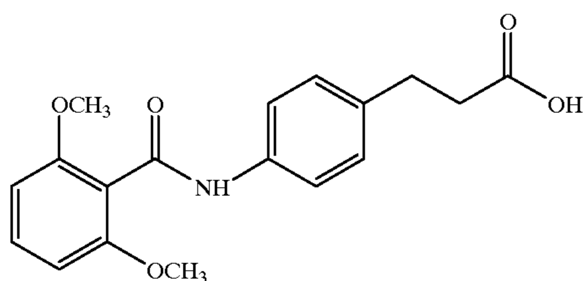
3-(4-(2,6-dimethoxybenzoyl)aminophenyl)propionic acid
