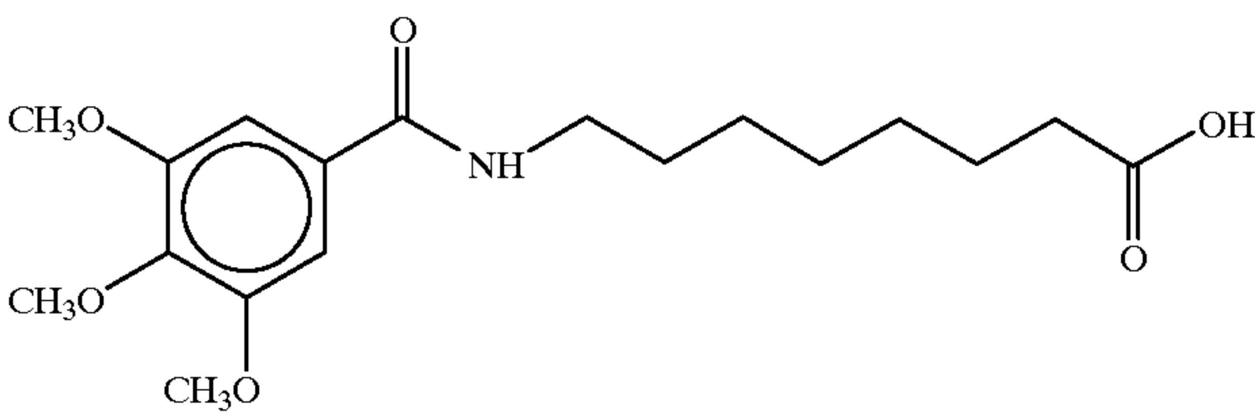
8-(3, 4, 5-Trimethoxybenzoyl)aminocaprylic acid
