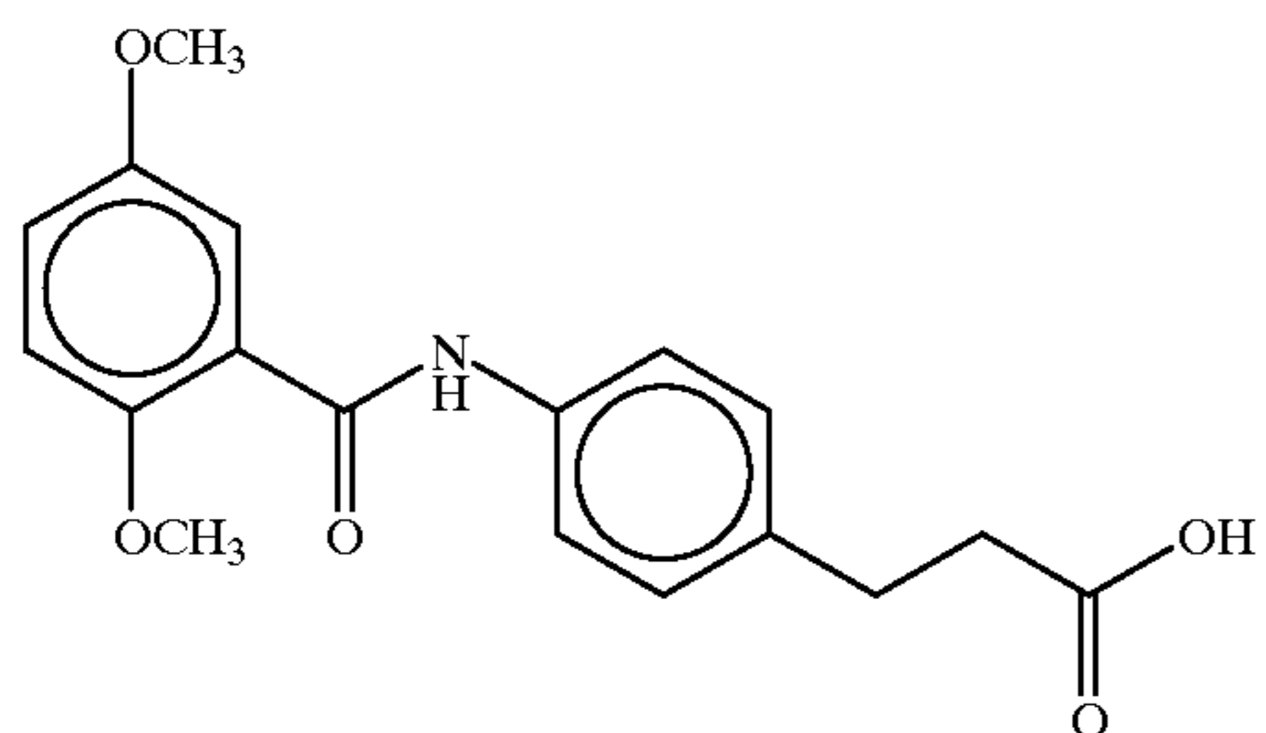
3-(4-(2,5-dimethoxybenzoyl)aminophenyl)propionic acid
