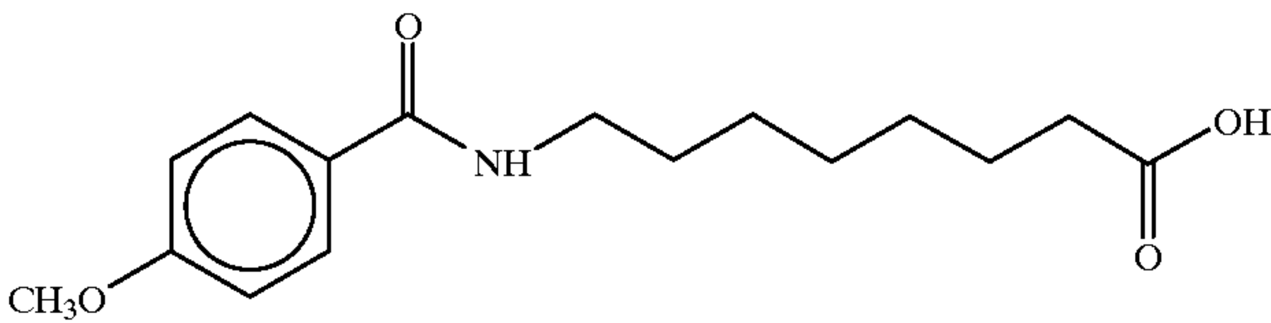
8-(p-anisoyl)aminocaprylic acid
