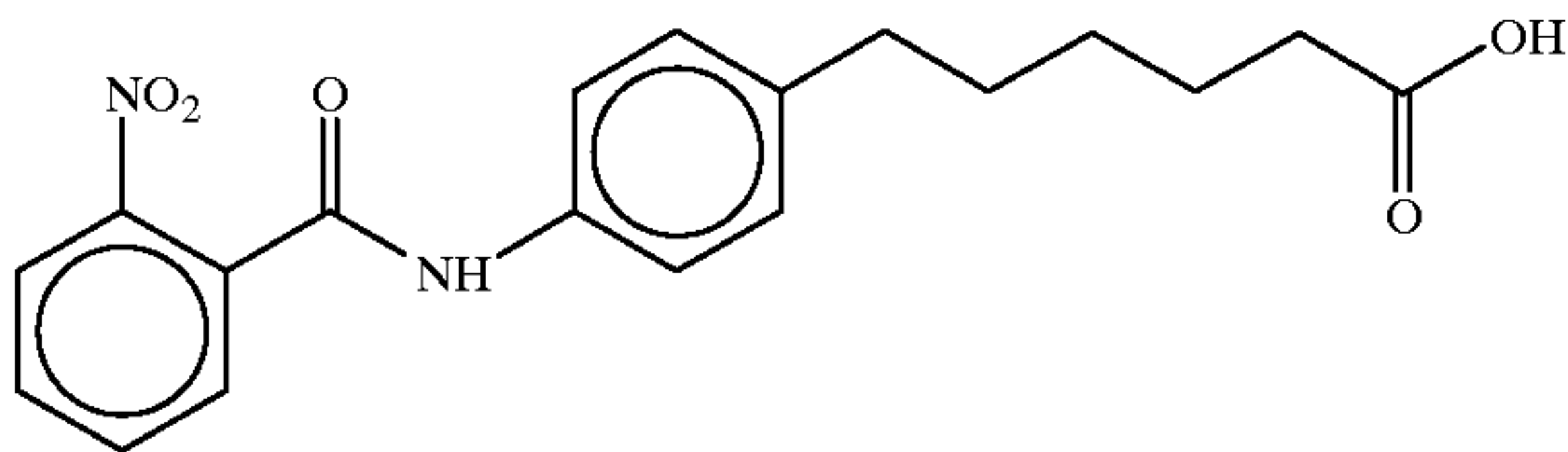
6-(4-(N-2-Nitrobenzoyl)aminophenyl)hexanoic acid
