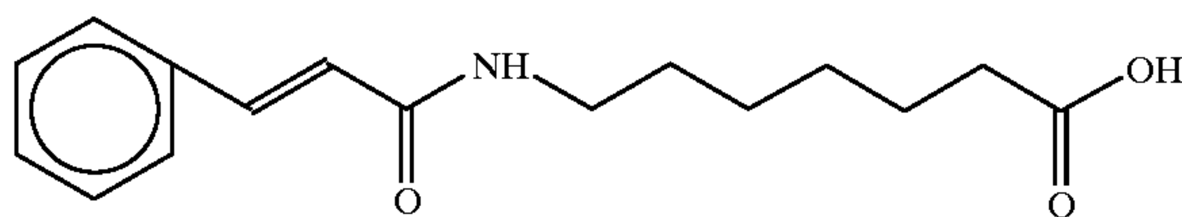
7-cinnamoylaminoheptanoic acid
