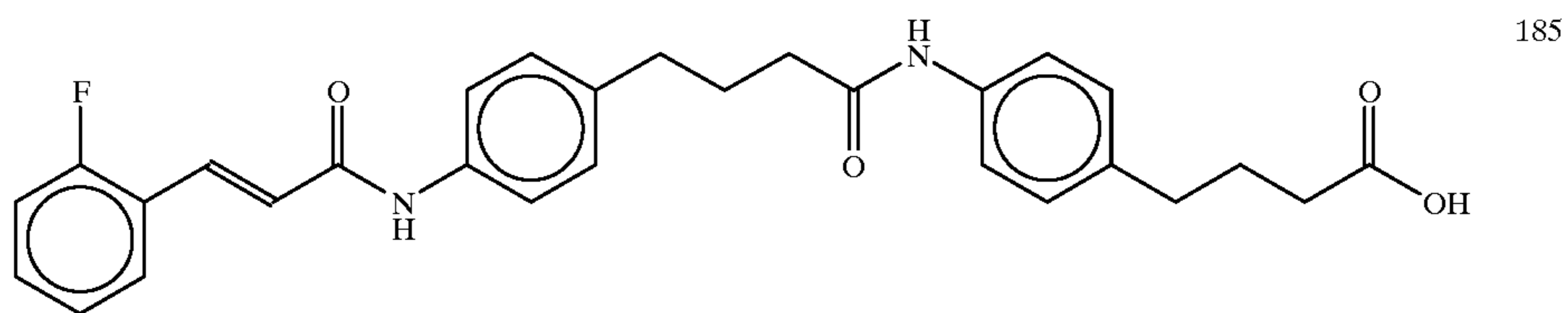
4-(4-(N-(2-Fluorocinnamoyl))aminophenyl)butyric
