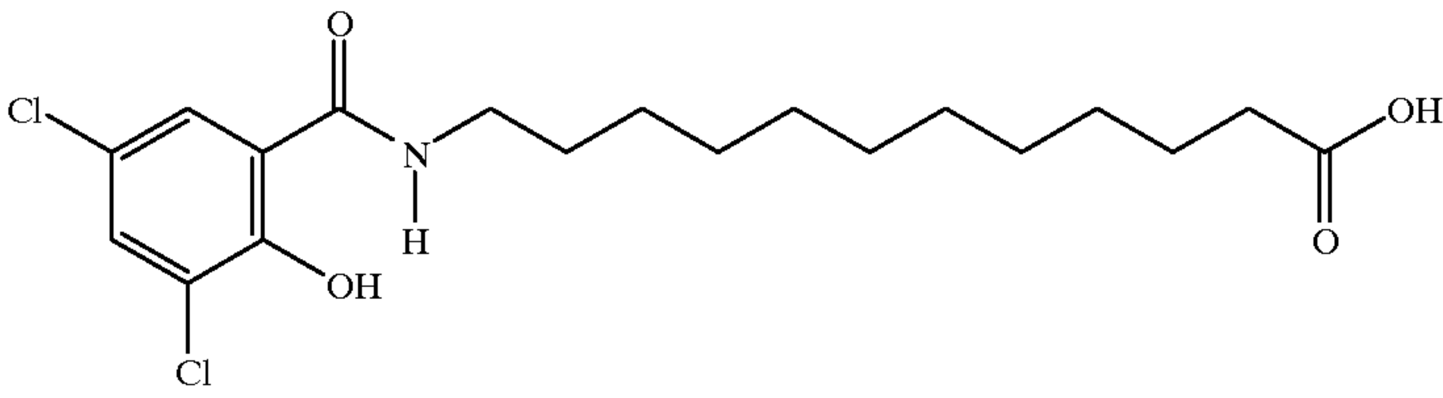
12-N-(3, 5-dichloro-2-hydroxybenzoyl)aminododecanoic acid
