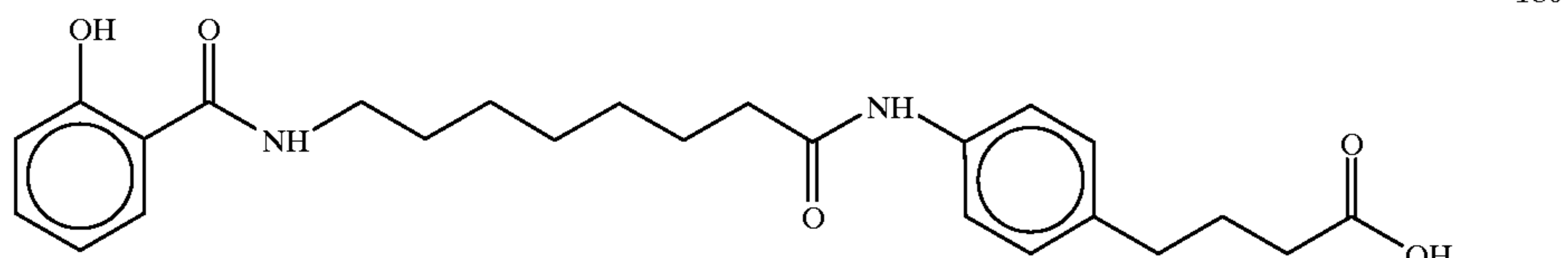
4-(4-(N-8(N-Salicyloyl)aminocaprylic)aminophenyl)butyric acid
