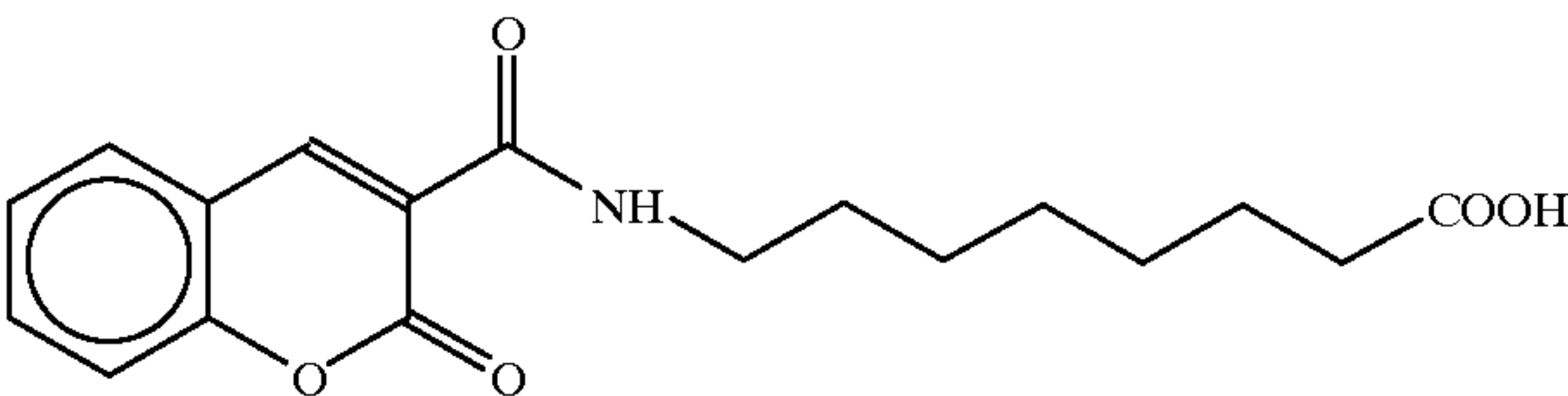
8-[N-(3-coumarincarbonyl)]aminocaprylic acid
