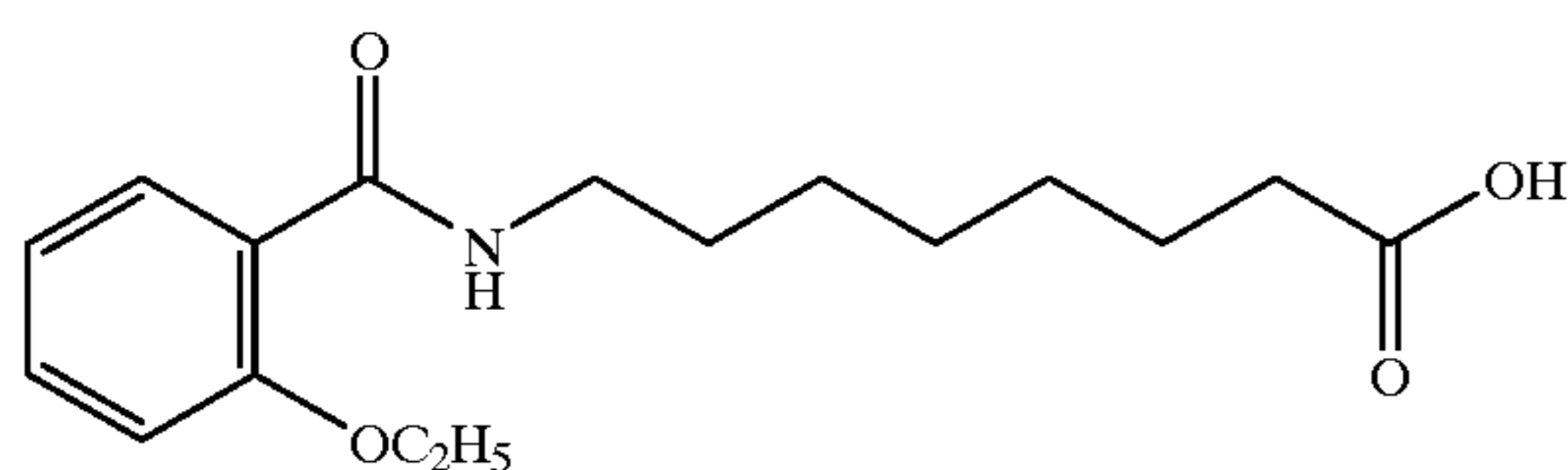
8-(2-ethoxybenzoyl)aminocaproic acid
