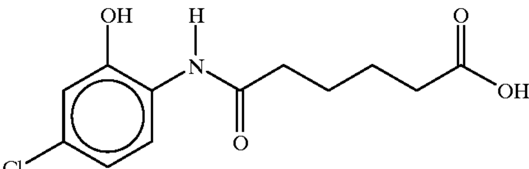
5-(4-chloro-2-hydroxyanilino)valeric acid
