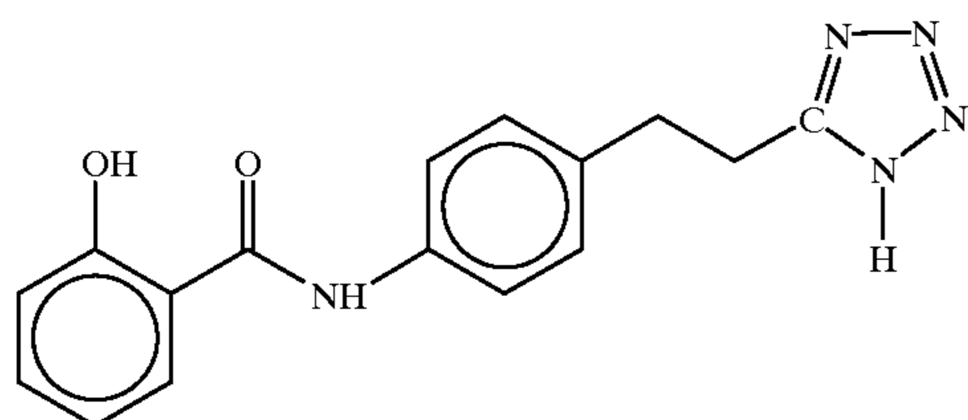
4-(Salicyloyl)aminophenylethyltetrazole
