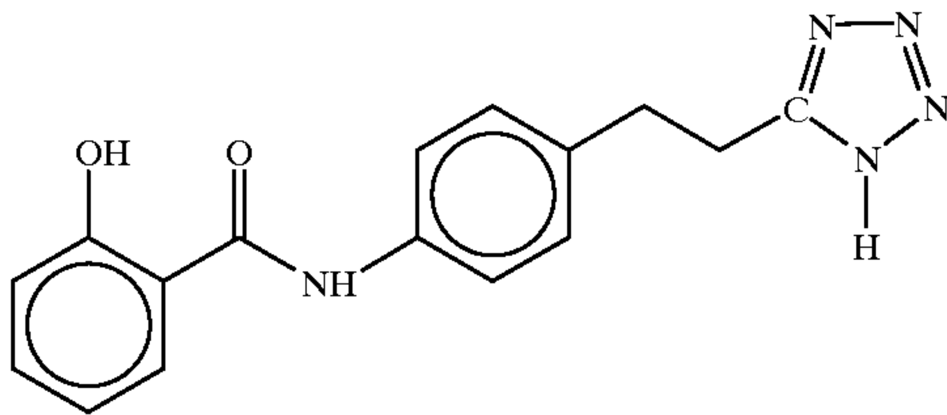
4-(Salicyloyl)aminophenylethyltetrazole
