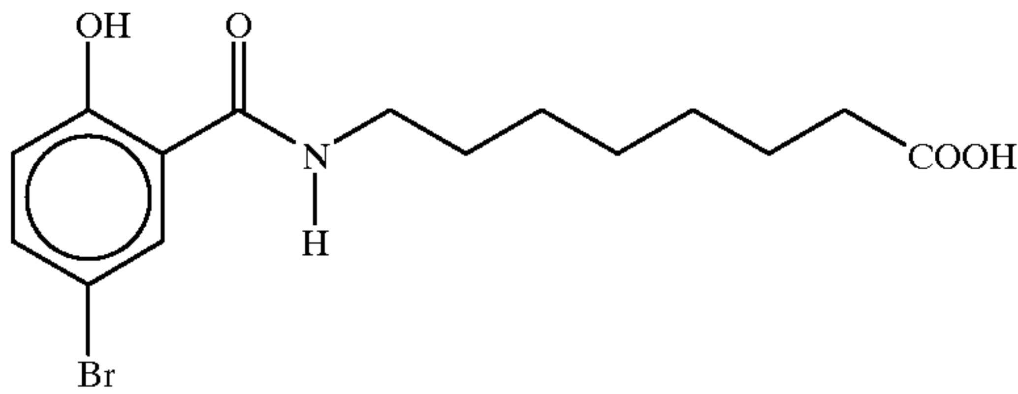
8-(N-2-hydroxy-5-bromobenzoyl)aminocaprylic acid
