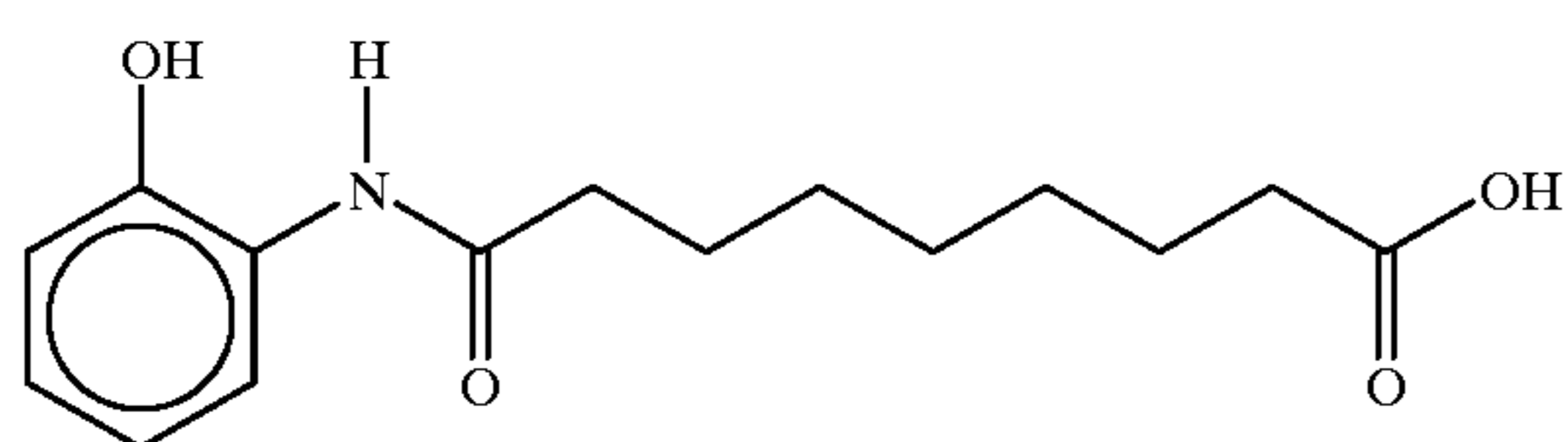
9-(2-hydroxybenzamido)nonanic acid
