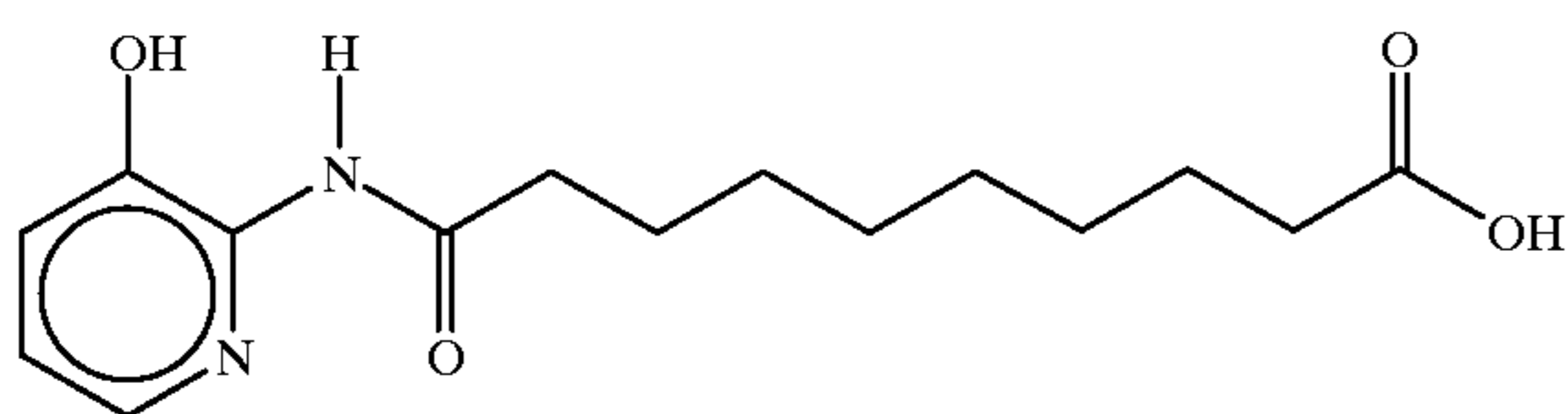
9-[2-(3-hydroxy)pyridylamino]nonanoic acid
