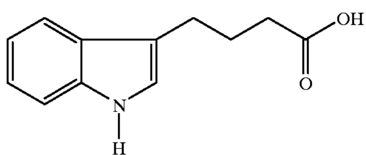
3-Indolebutyric acid
