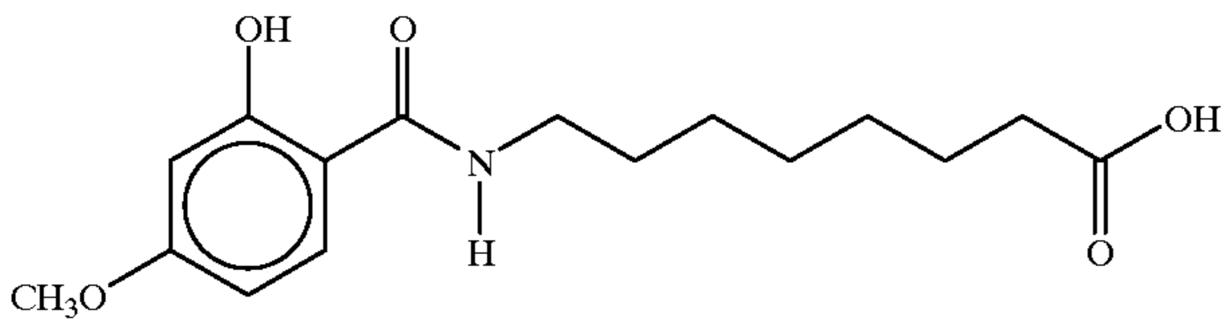
8-(N-2-Hydroxy-4-methoxybenzoyl)aminocaprylic acid
