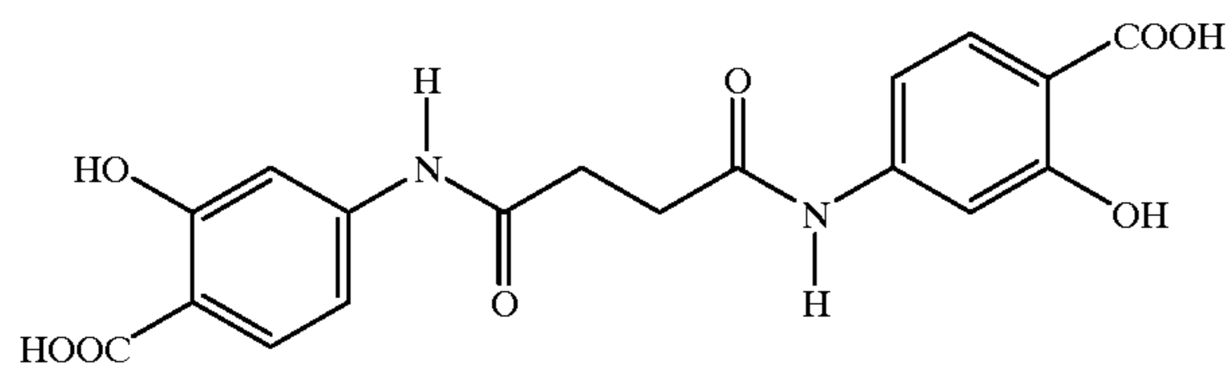
Succinyl-4-aminosalicylic acid
