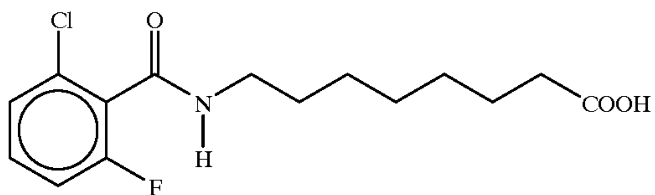
8-N-(2-chloro-6-fluorobenzoyl)aminocaprylic acid
