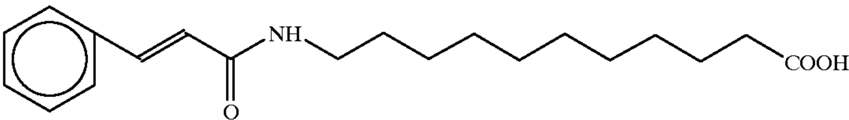
11-cinnamoylamino undecanoic acid
