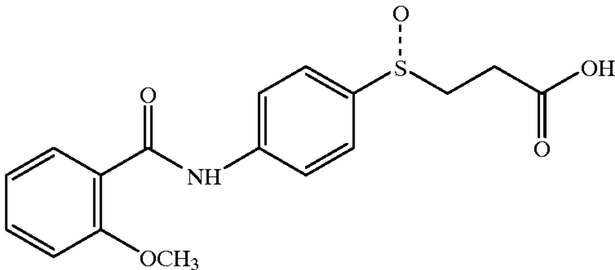
4-(2-methoxybenzoyl)amino 3-carboxysulfoxide
