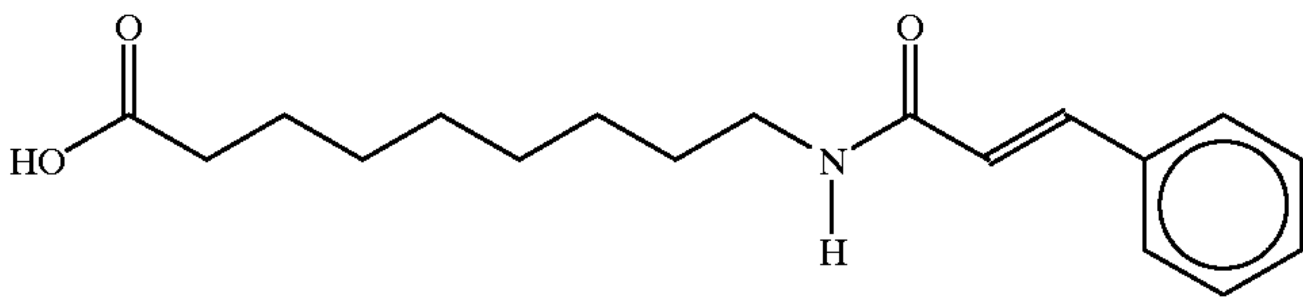
9-(cinnamoylamino)nonanoic acid
