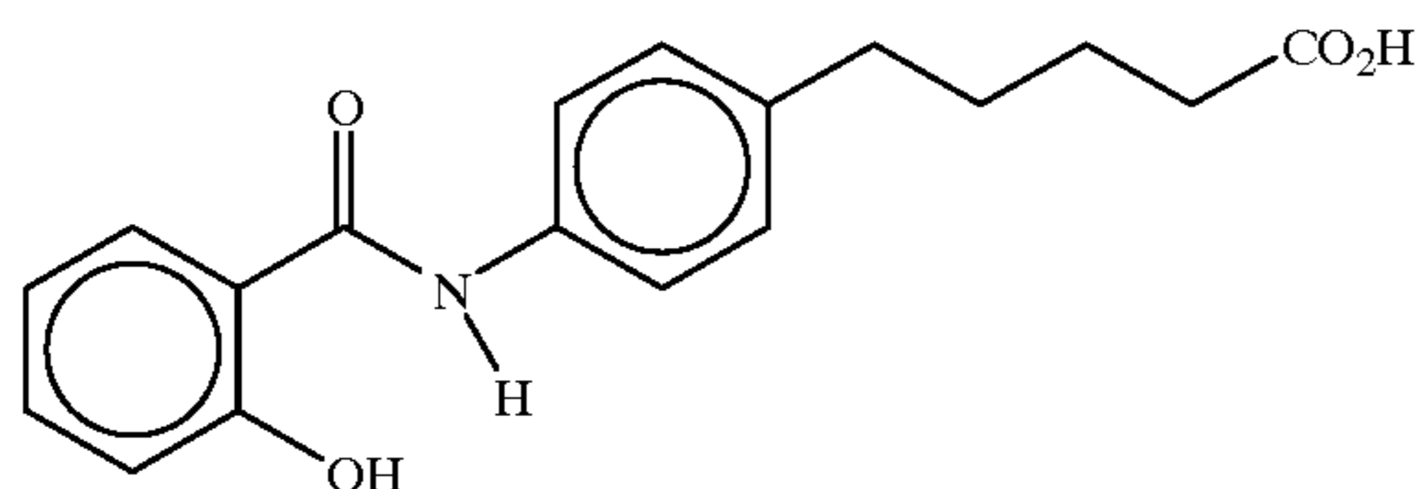
N-salicyloyl-5-(4-aminophenyl)valeric acid
