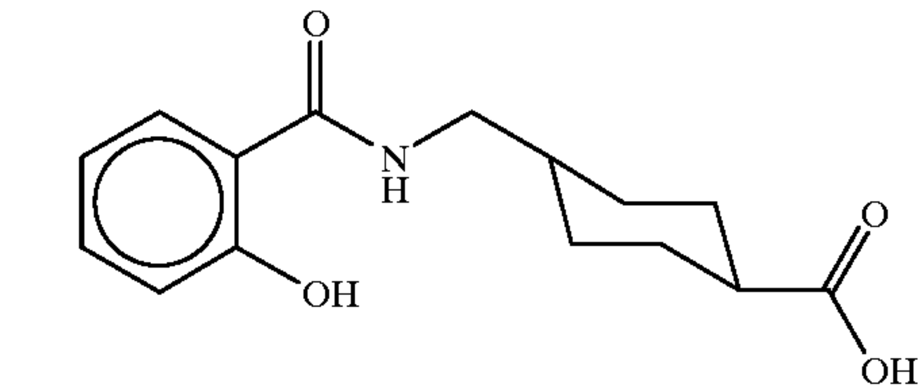
trans-4-(N-salicyloylaminomethyl)cyclohexane carboxylic acid
