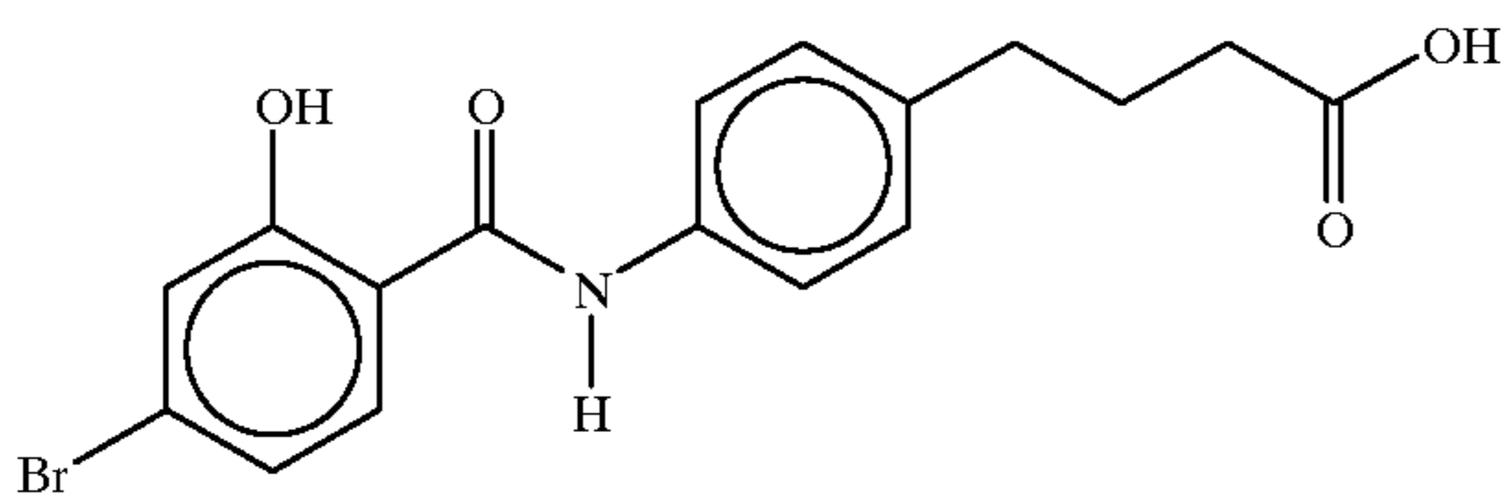
4-[N-(2-hydroxy-4-bromobenzoyl)aminophenyl]butyric acid
