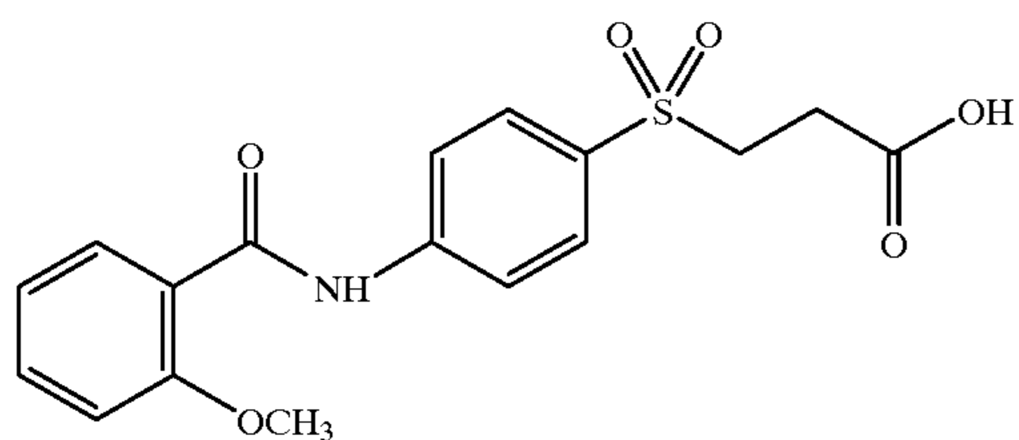
4-(2-methoxybenzoyl)amino 3-carboxypropylsulfone
