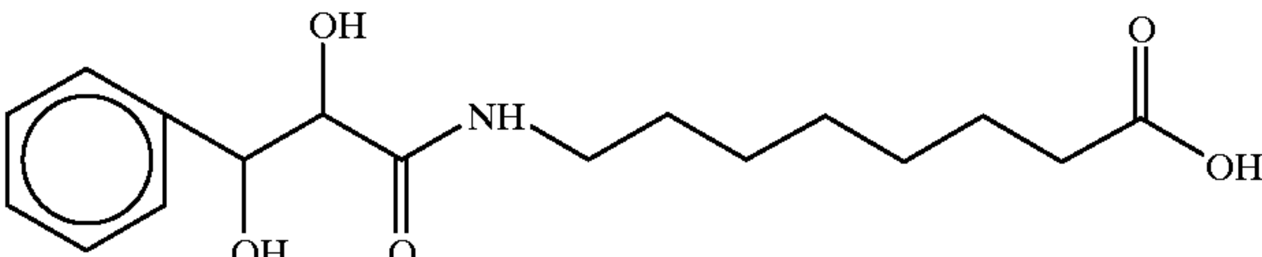
(3-phenyl-2,3-dihydroxypropanoyl) 8-aminocaprylic acid
