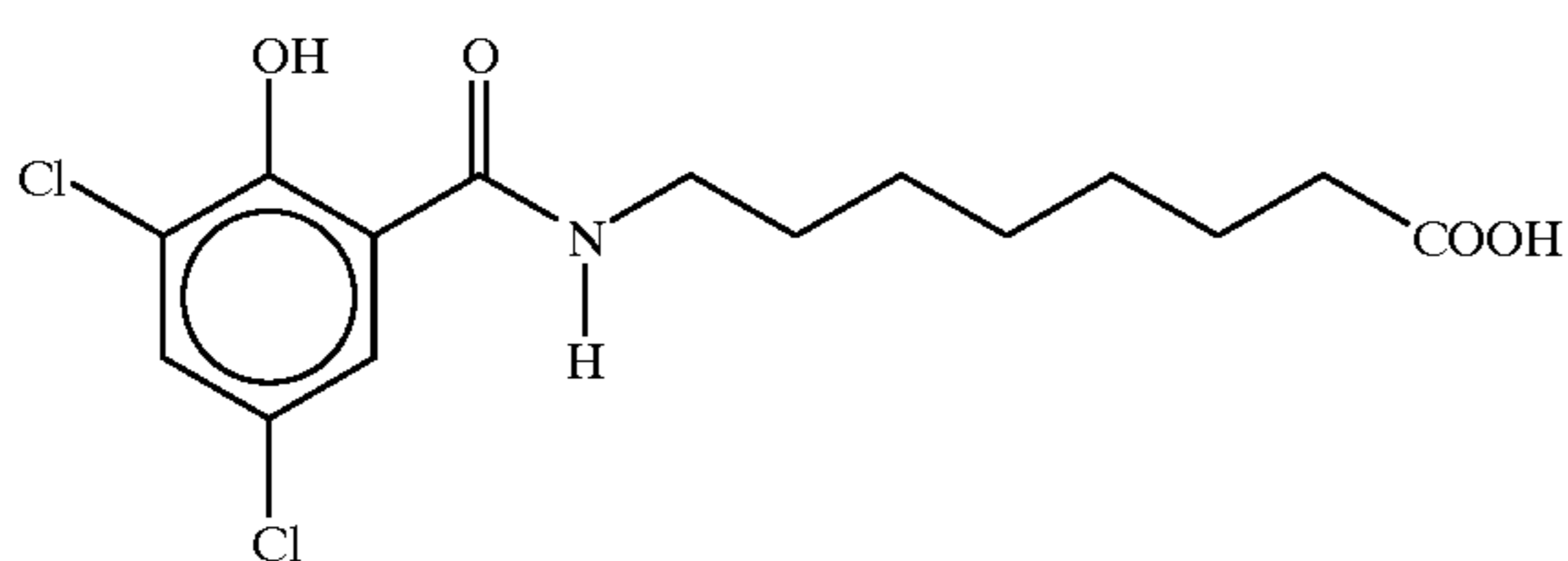
8-[N-(2-acetoxy-3,5-dichlorobenzoyl)]aminocaprylic acid
