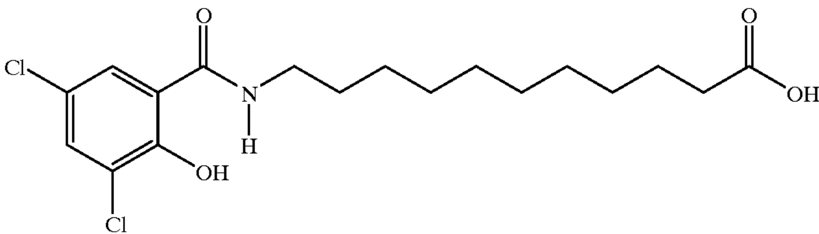
11-N-(3, 5-dichloro-2-hydroxybenzoyl)aminoundecanoic acid
