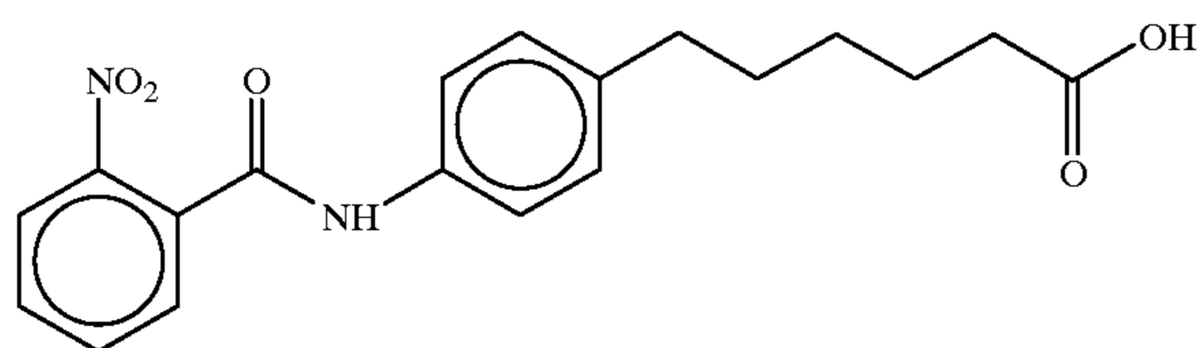
6-(4-(N-2-Nitrobenzoyl)aminophenyl)hexanoic acid
