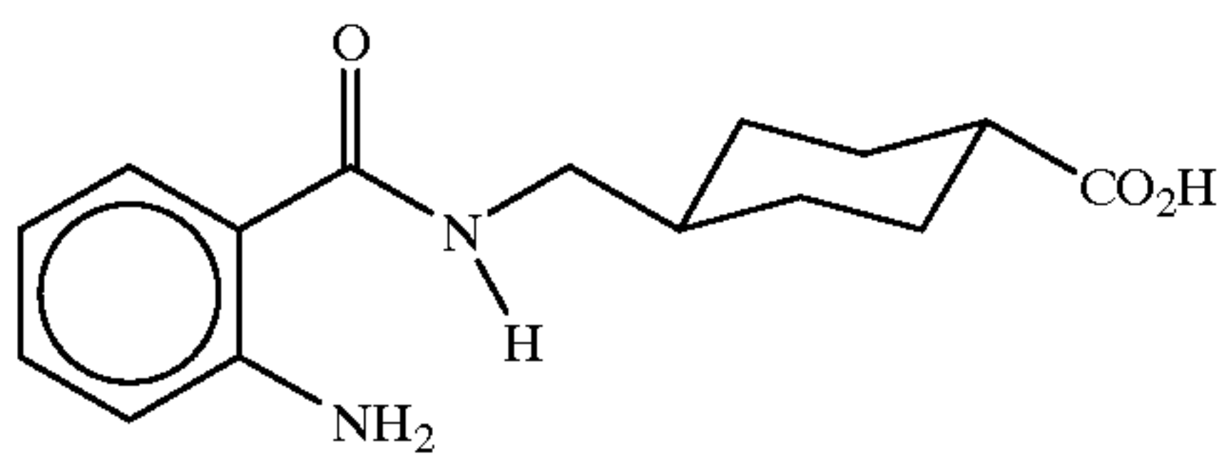
trans-4-(2-aminobenzamidomethyl)cyclohexanecarboxylic acid
