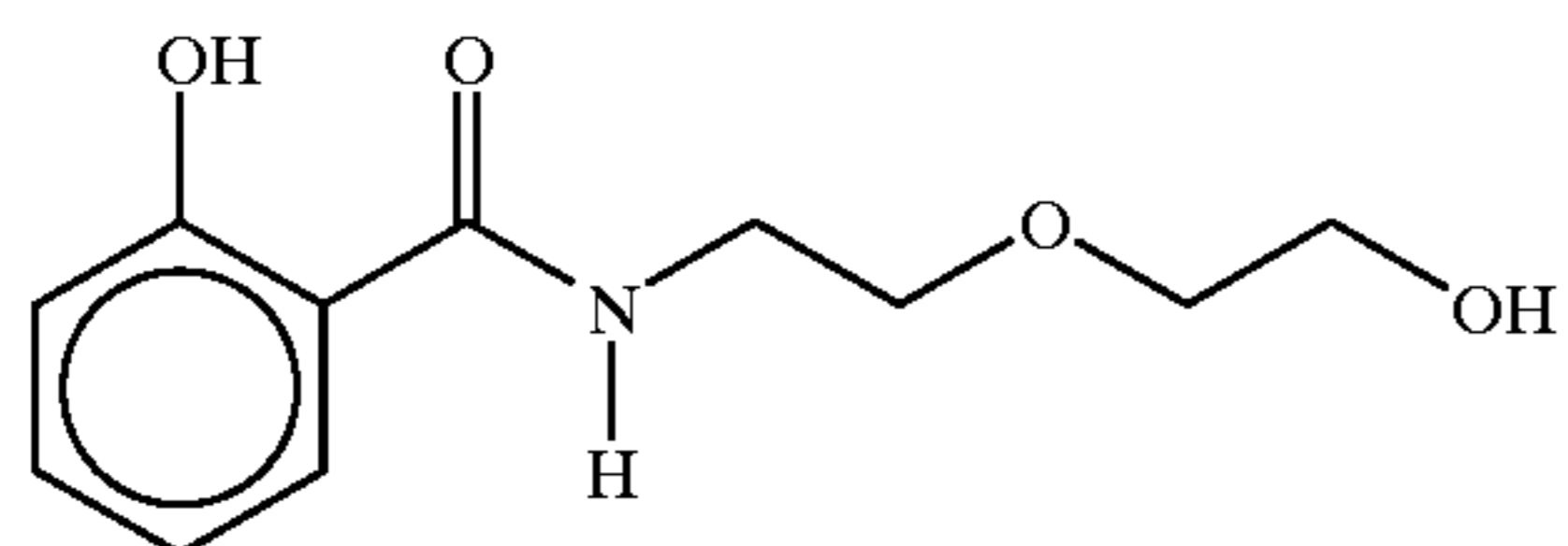
2-[N-(2-hydroxybenzoylamino)ethoxy]ethanol
