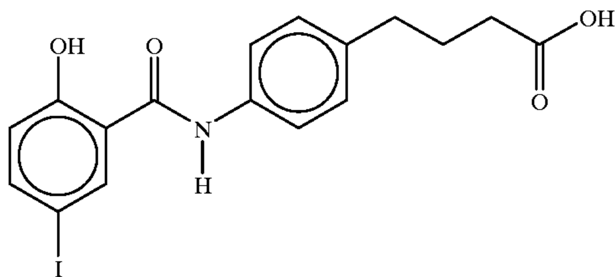
4-[-[N-(2-hydroxy-5-iodobenzoyl)]aminophenyl]butyric acid
