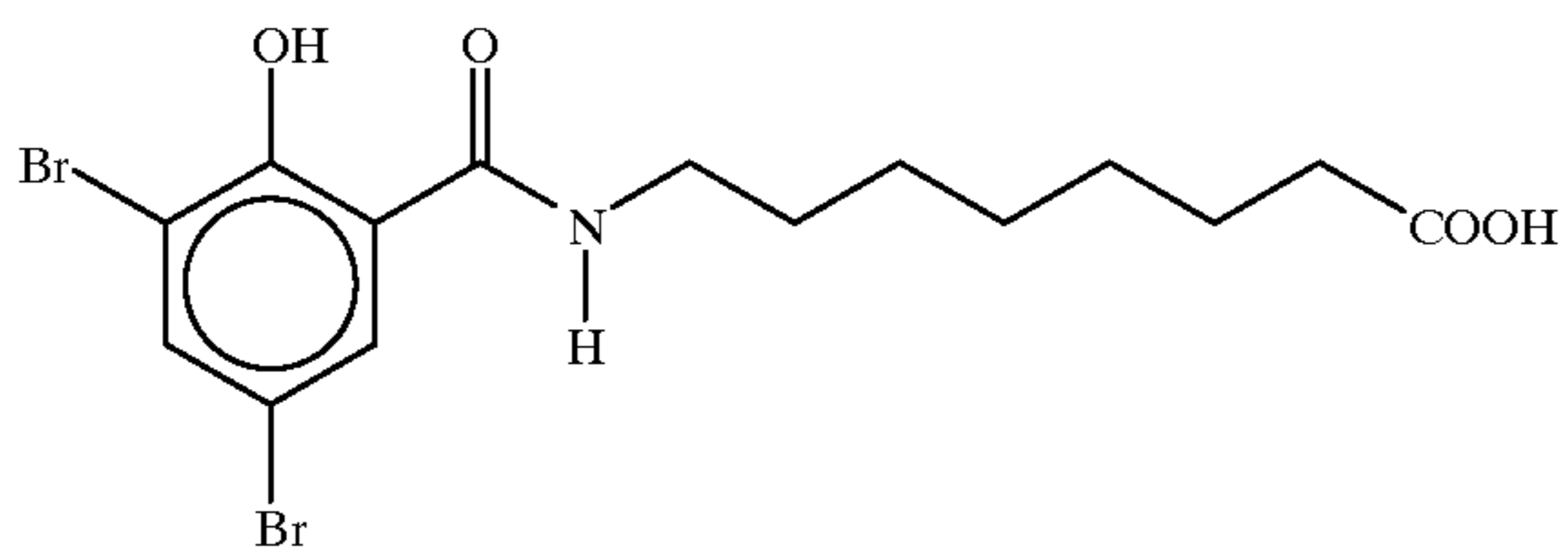
8-[N-(2-acetoxy-3,5-dibromobenzoyl)]aminocaprylic acid
