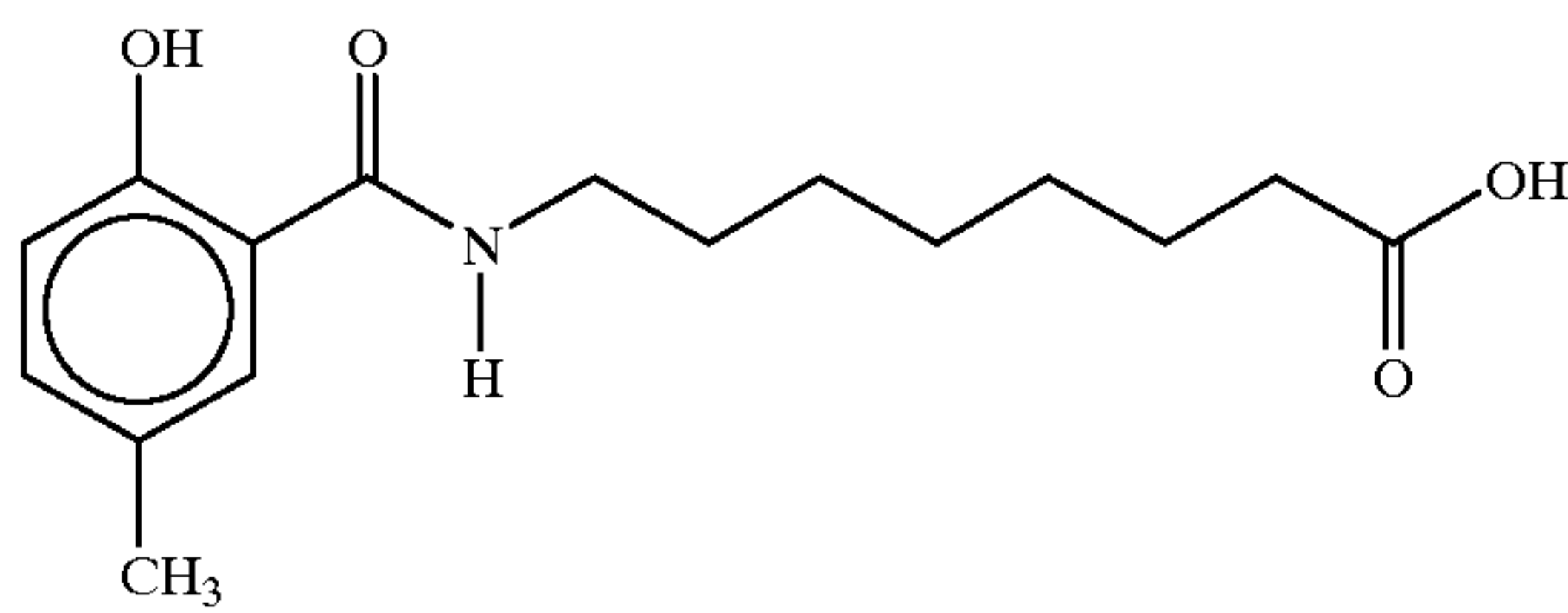
8-(N-5-methylsalicyloyl)aminocaprylic acid
