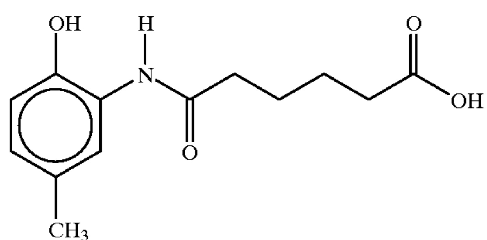
5-(2-hydroxy-5-methylanilincarbonyl)valeric acid
