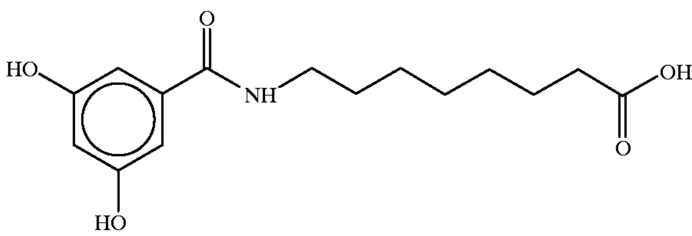
8-(N-(3,5-Dihydroxybenzoyl)aminocaprylic acid
