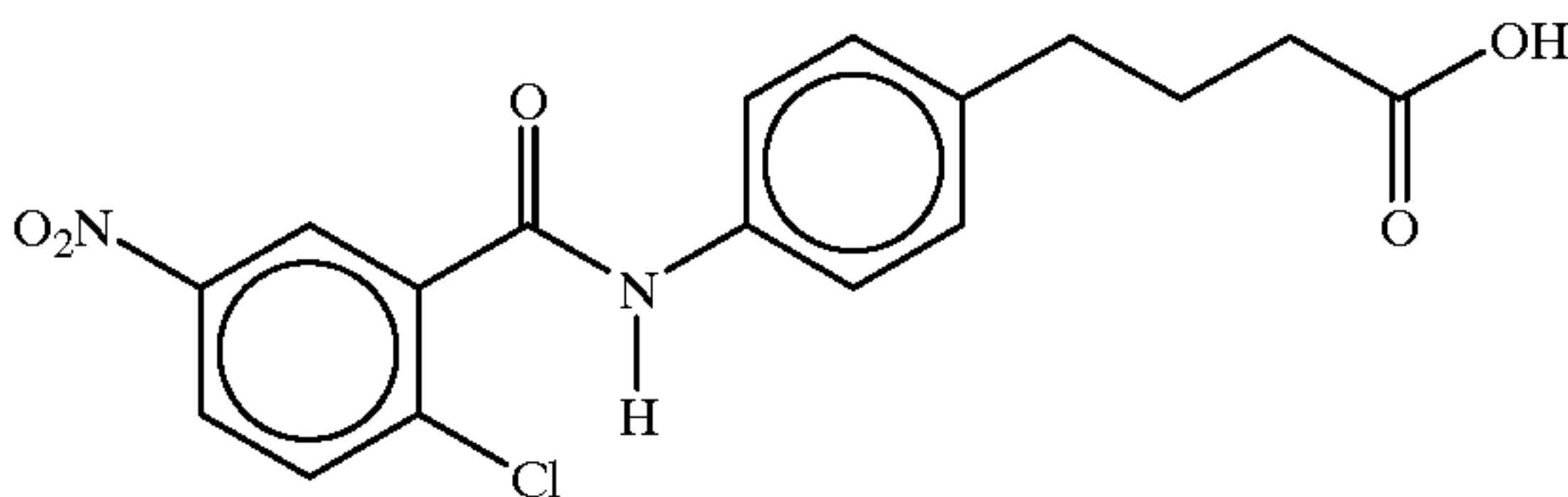
4-(4-(2-chloro-5-nitrobenzoyl)aminophenyl)butyric acid
