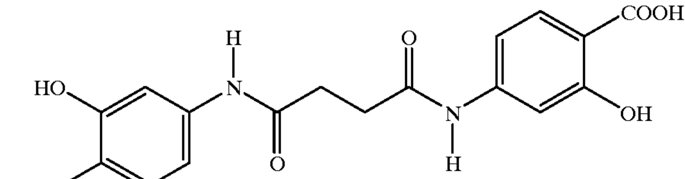
Succinyl-4-aminosalicylic acid
