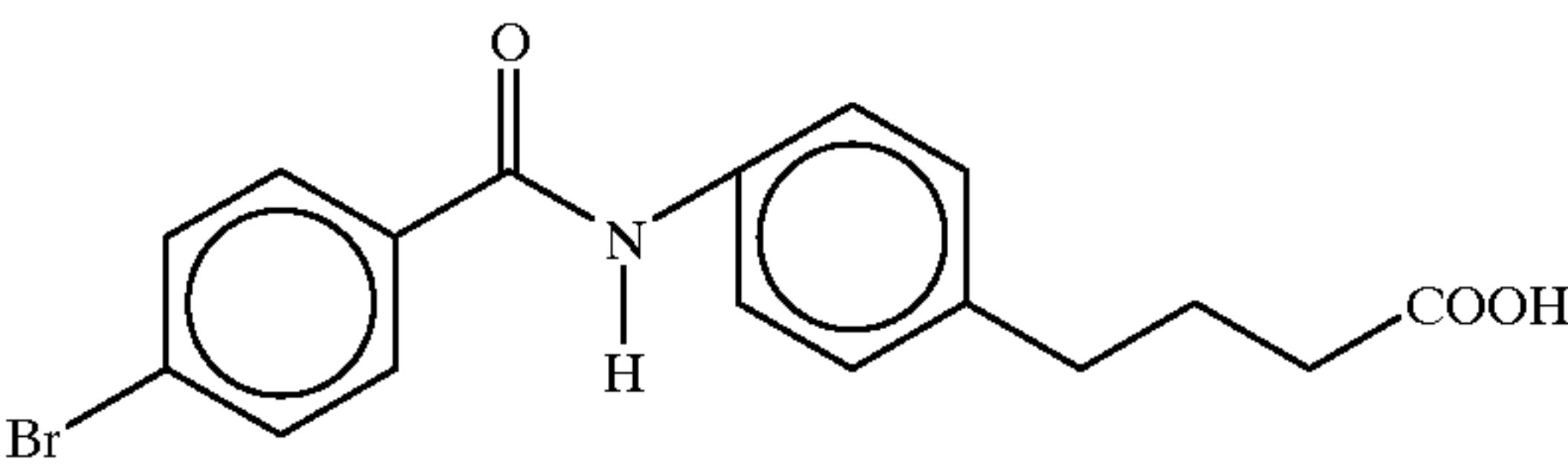
4-{4-[N-(4-bromobenzoyl)aminophenyl]}butyric acid
