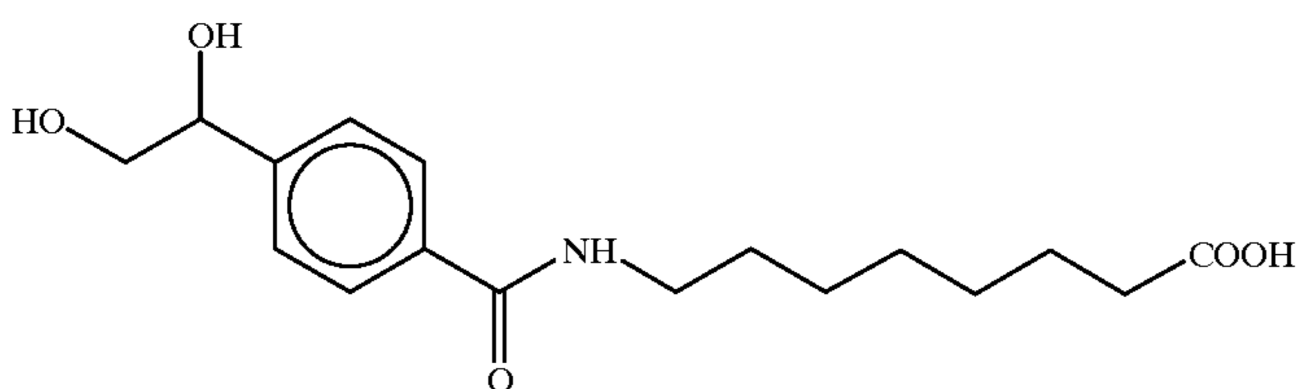
8-(4-(1,2-dihydroxyethyl)benzoyl)aminocaprylic acid
