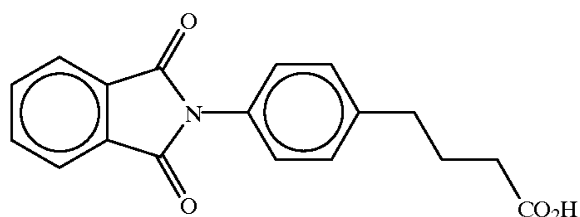
4-(4-phthalimidophenyl)butyric acid
