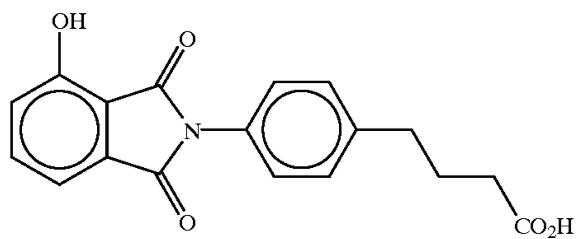
4-(4-(3-hydroxyphthalimido)phenyl)butyric acid
