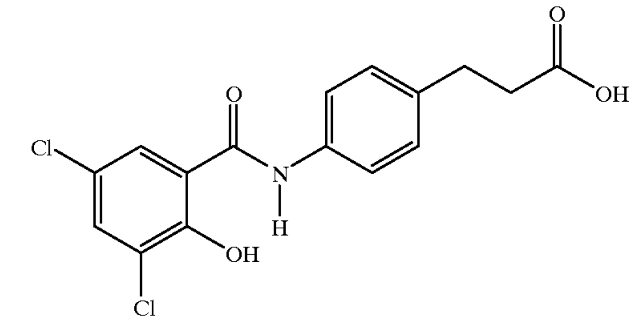
N-[3, 5-dichloro-2-hydroxybenzoyl-3-(4-aminophenyl)]propionic acid
