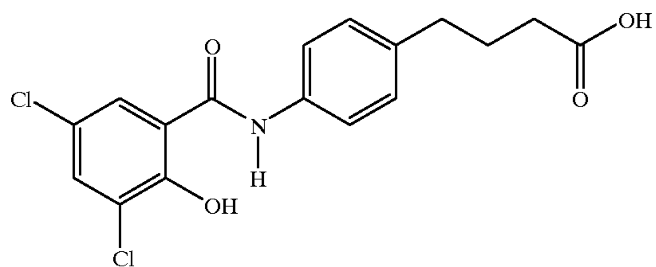
N-[3,5-dichloro-2-hydroxybenzoyl-4(4-aminophenyl)]butyric acid
