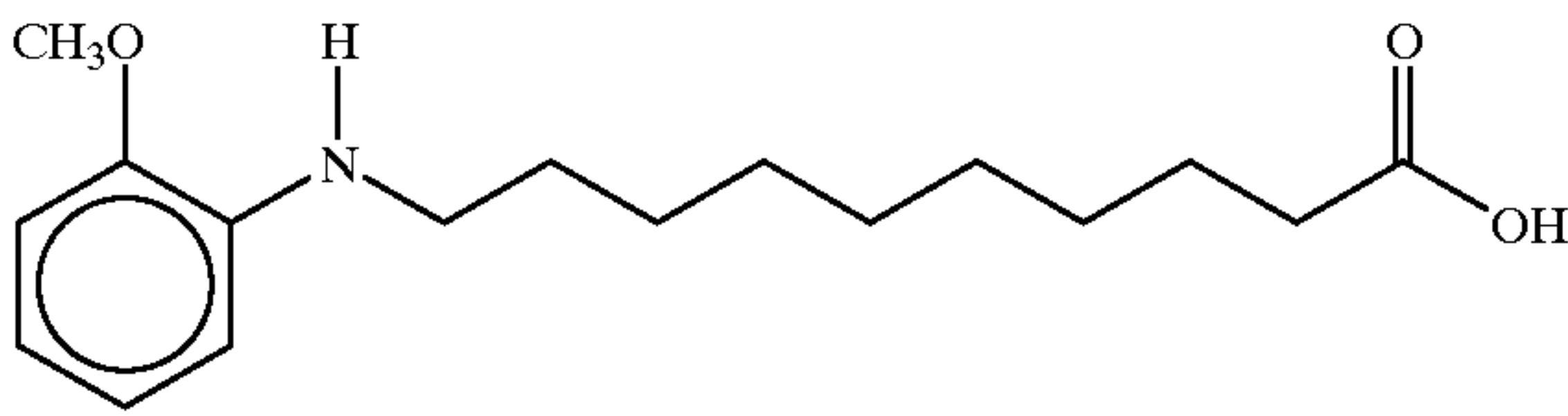
2-Methoxybenzenaminodecanoic acid
