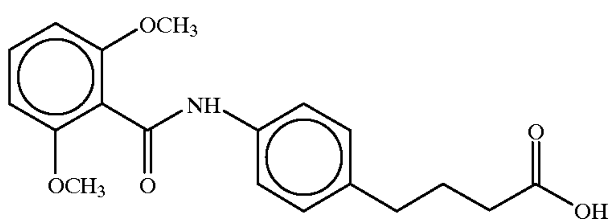
4-(4-(2,6-dimethoxybenzoyl)aminophenyl)butyric acid
