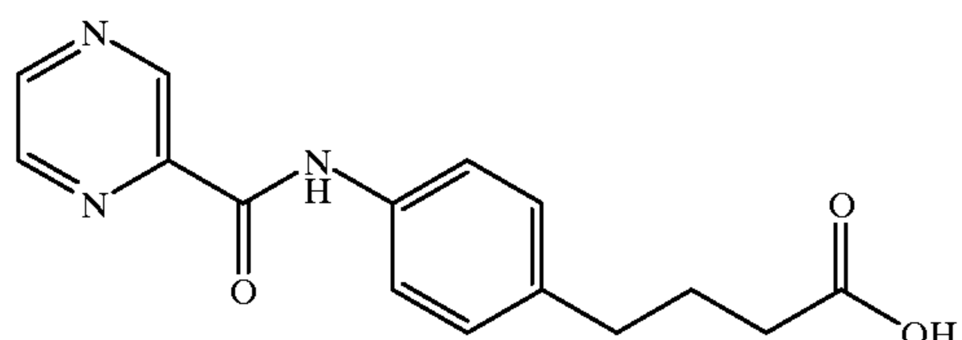
4-(4-(2-pyrazinecarbonyl)aminophenyl)butyric acid
