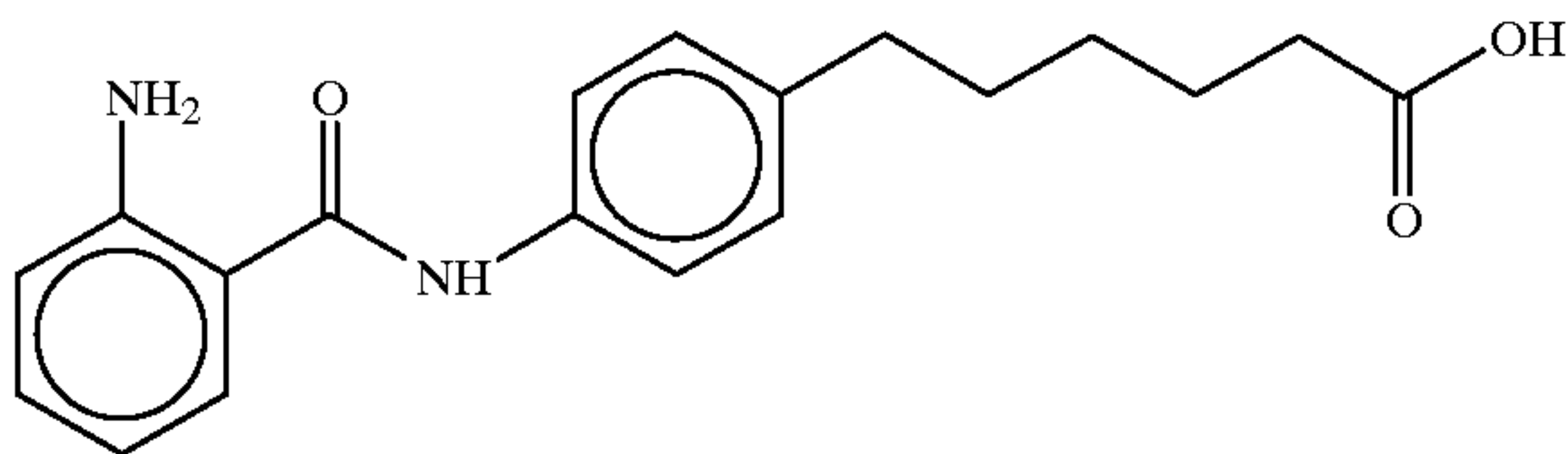
6-(4-(N-2-aminobenzoyl)aminophenyl)hexanoic acid
