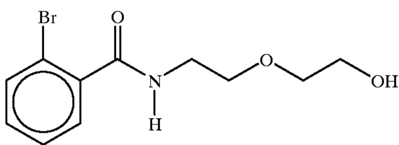
2-[N-(2-bromobenzoyl)aminoethoxy]ethanol
