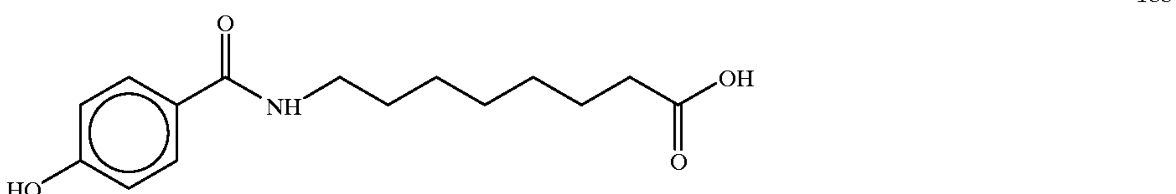
8-(4-Hydroxybenzoyl)aminocaprylic acid
