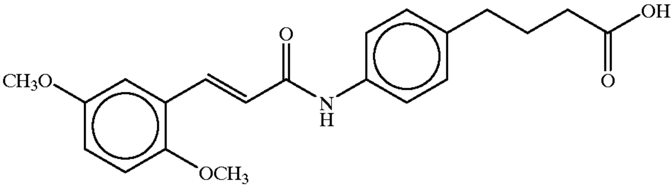
4-(4-(2, 5-dimethoxycinnamoyl)aminophenyl)butyric acid
