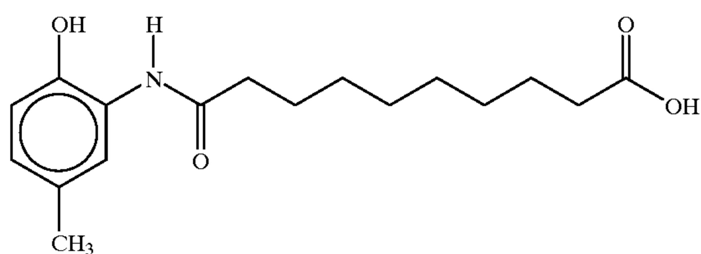
9-(2-hydroxy-5-methylanilincarbonyl)nonanoic acid
