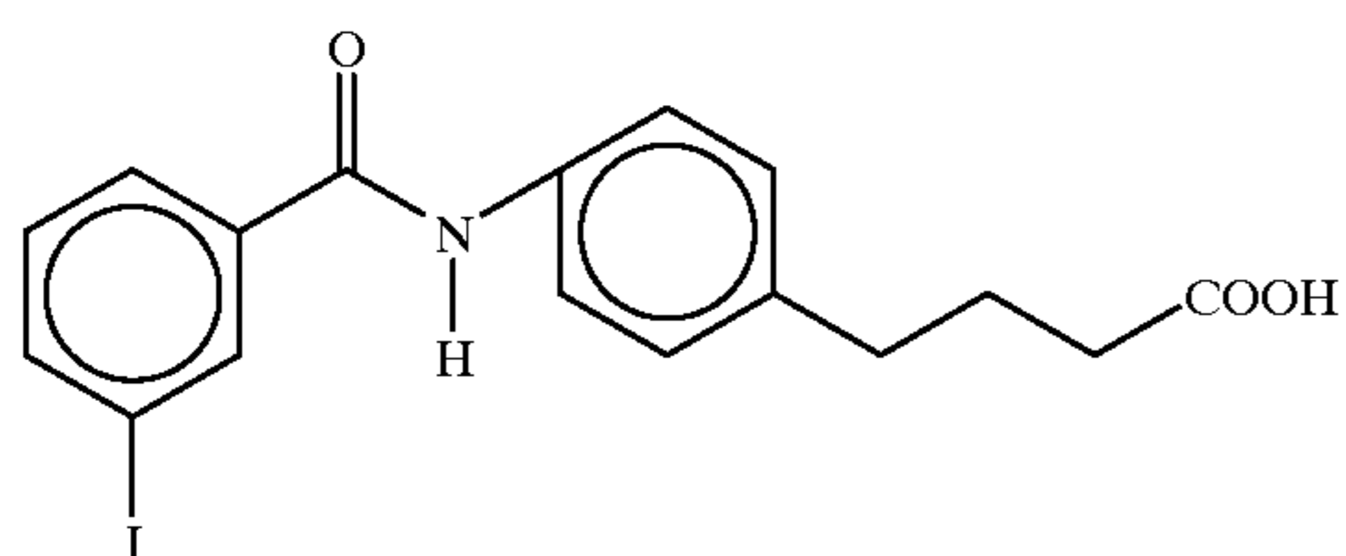
4-{N-[4-(3-iodobenzoyl)aminophenyl]}butyric acid
