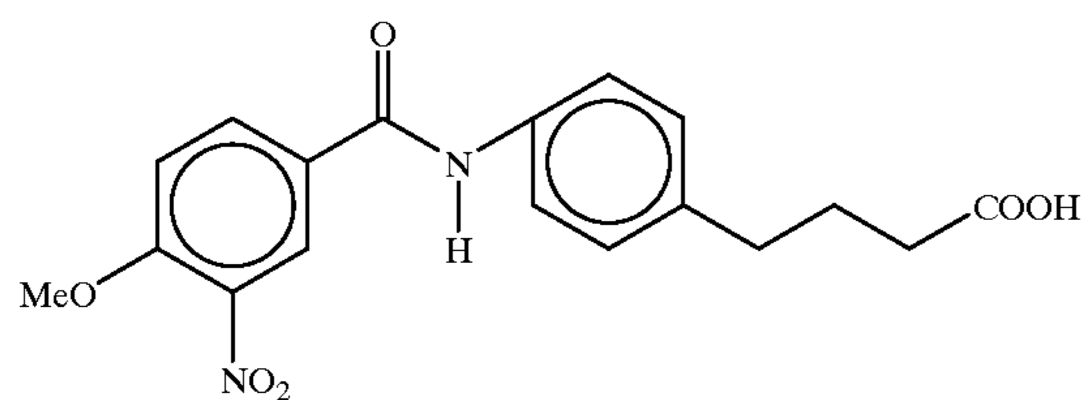
4-[4-N-(4-methoxy-3-nitrobenzoyl)aminophenyl]butyric acid
