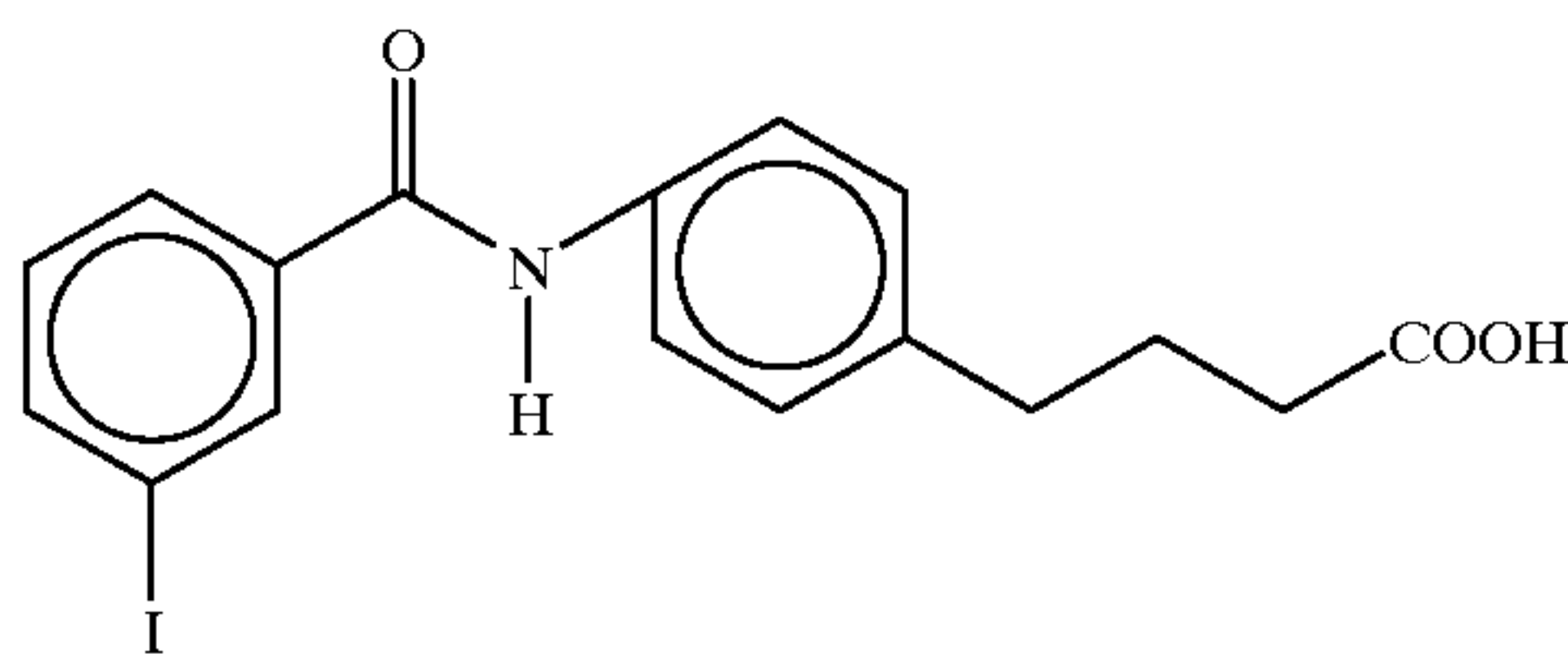
4-{N-[4-(3-iodobenzoyl)aminophenyl]}butyric acid
