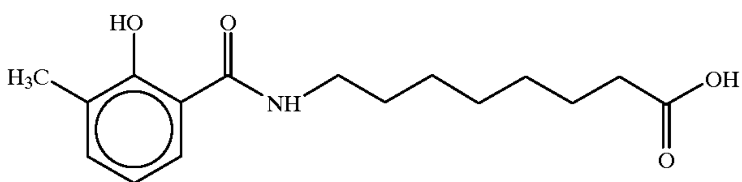
8-(N-3-methylsalicyloyl)aminocaprylic acid
