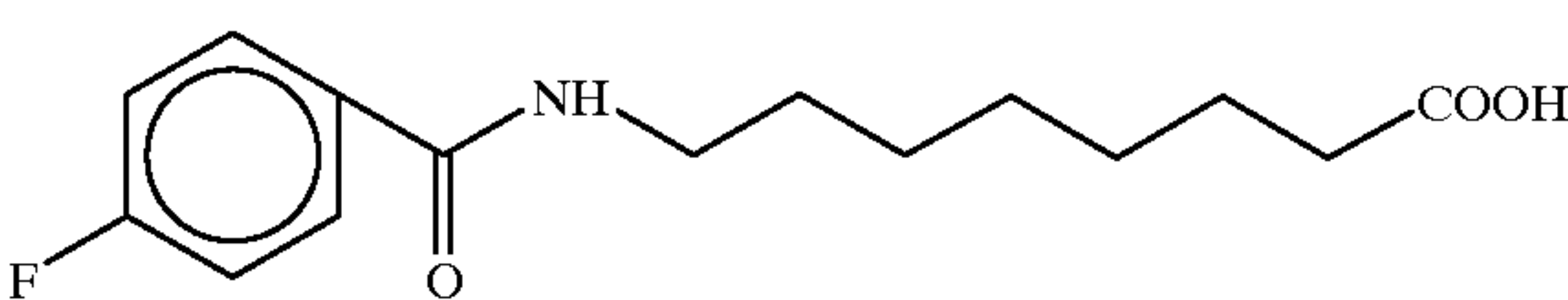
8-[N-(4-fluorobenzoyl)]aminocaprylic acid
