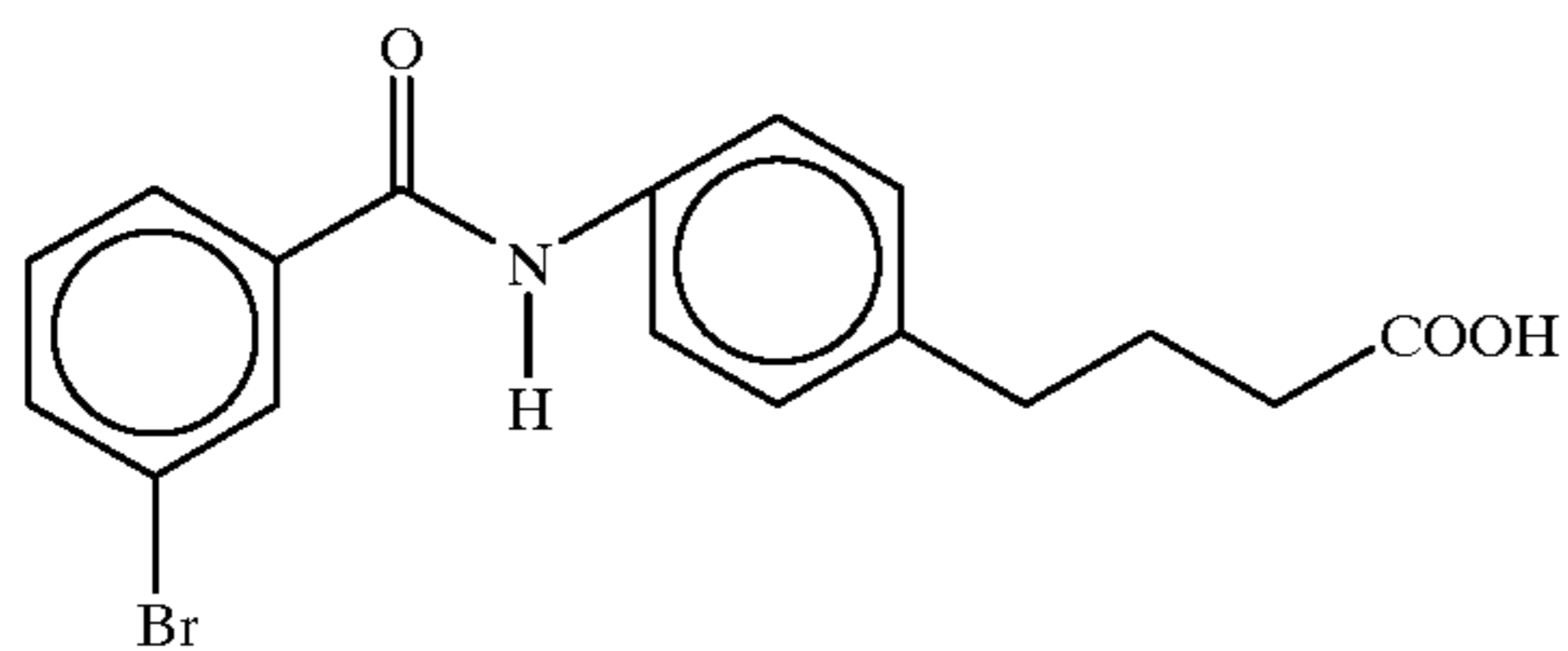
4-[4-[N-(3-bromobenzoyl)]aminophenyl]butyric acid
