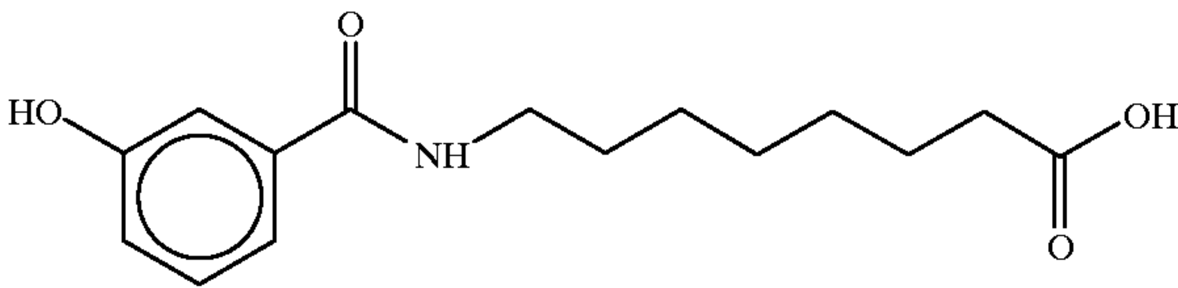
8-(3-Hydroxybenzoyl)aminocaprylic acid
