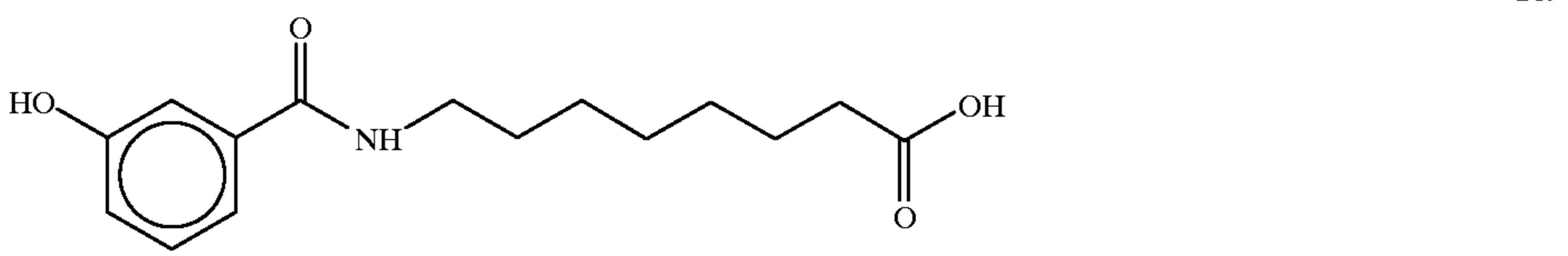
8-(3-Hydroxybenzoyl)aminocaprylic acid
