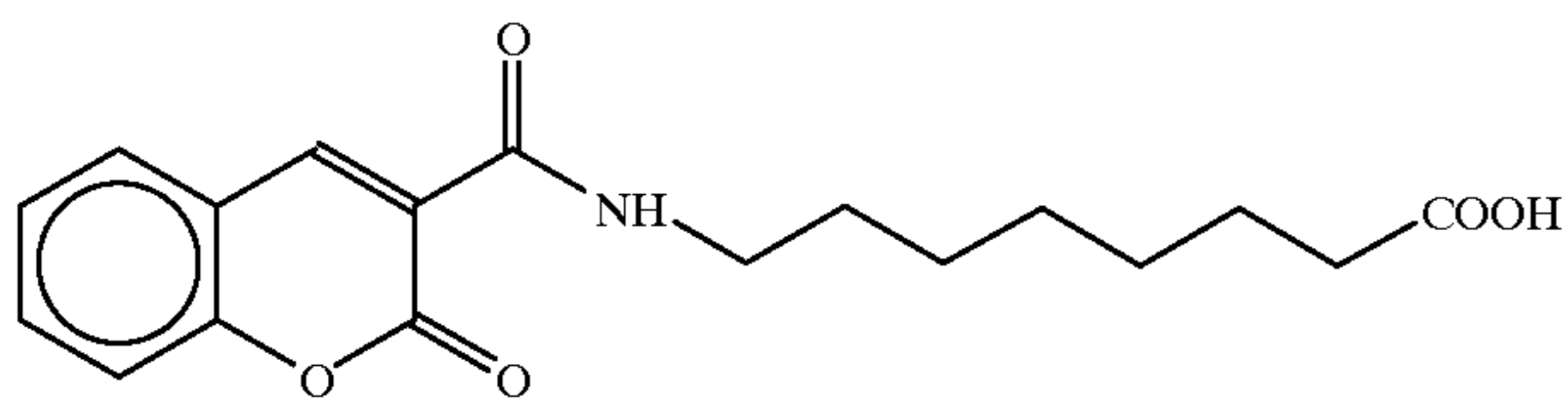
8-[N-(3-coumarinyl)]aminocaproic acid
