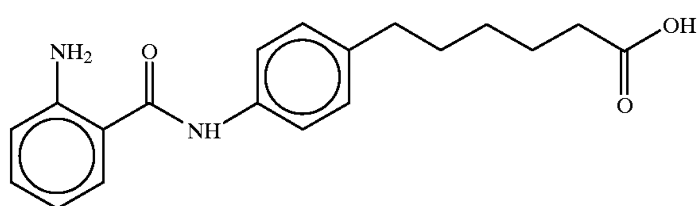
6-(4-(N-2-aminobenzoyl)aminophenyl)hexanoic acid
