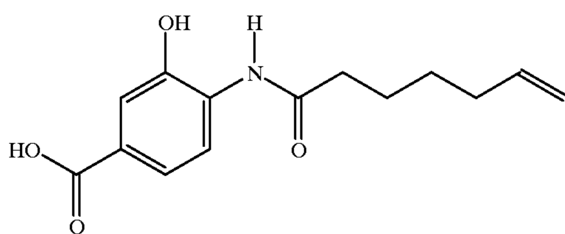
N-(2-hydroxy-4-carboxy)-6-heptenamide
