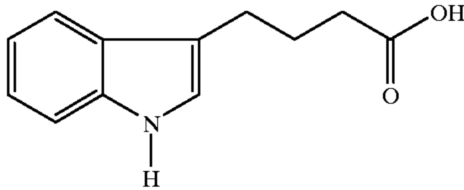
3-Indolebutyric acid
