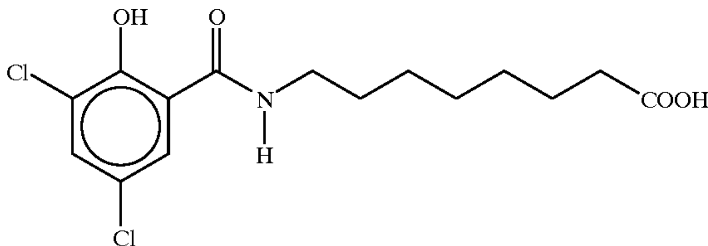
8-[N-(2-acetoxy-3, 5-dichlorobenzoyl)]aminocaprylic acid
