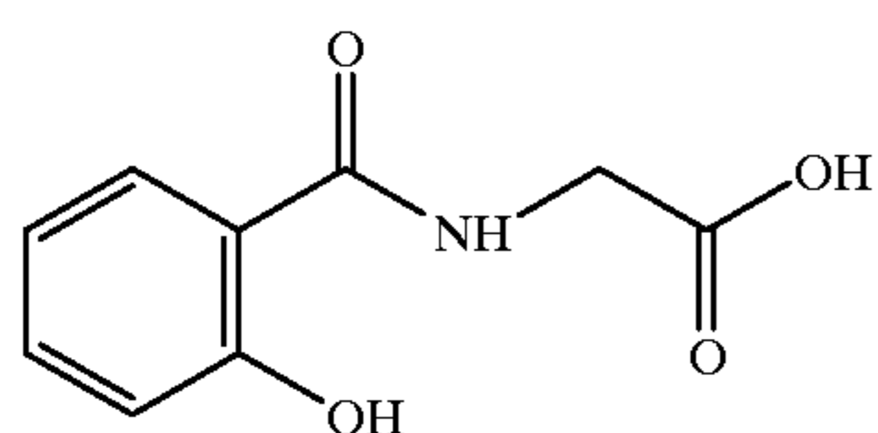
salicyloylglycine
