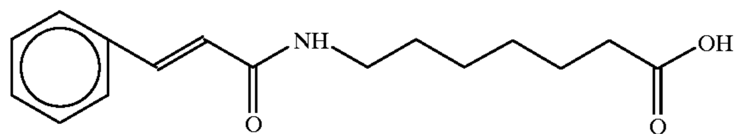
7-cinnamoylaminoheptanoic acid
