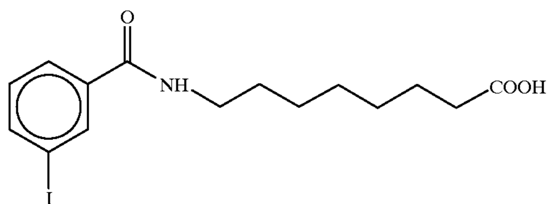
8-N-(3-iodobenzoyl)aminocaprylic acid
