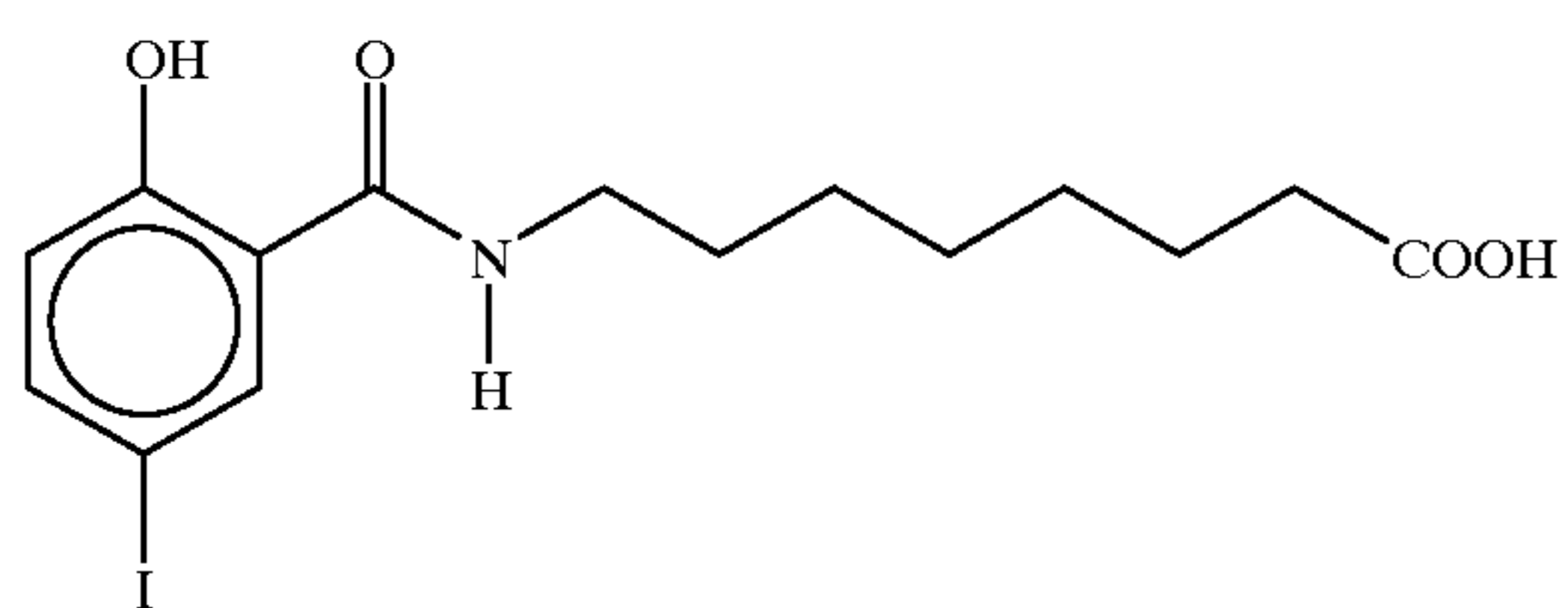
8-(N-2-hydroxy-5-iodobenzoyl)aminocaprylic acid
