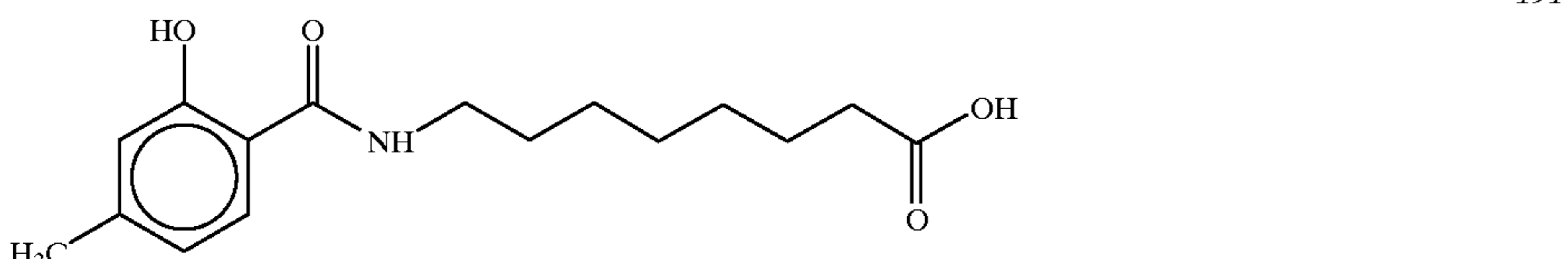
8-(N-4-Methylsalicyloyl)aminocaprillic acid
