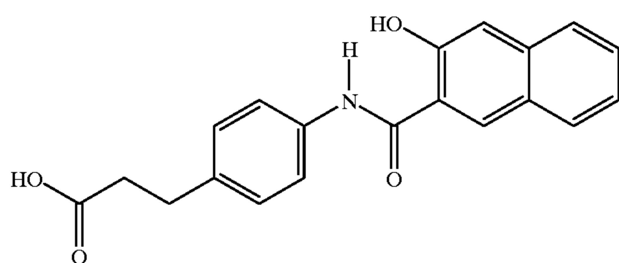
4-{4-[N-(3-hydroxy-2-naphthoyl)aminophenyl]}propanoic acid
