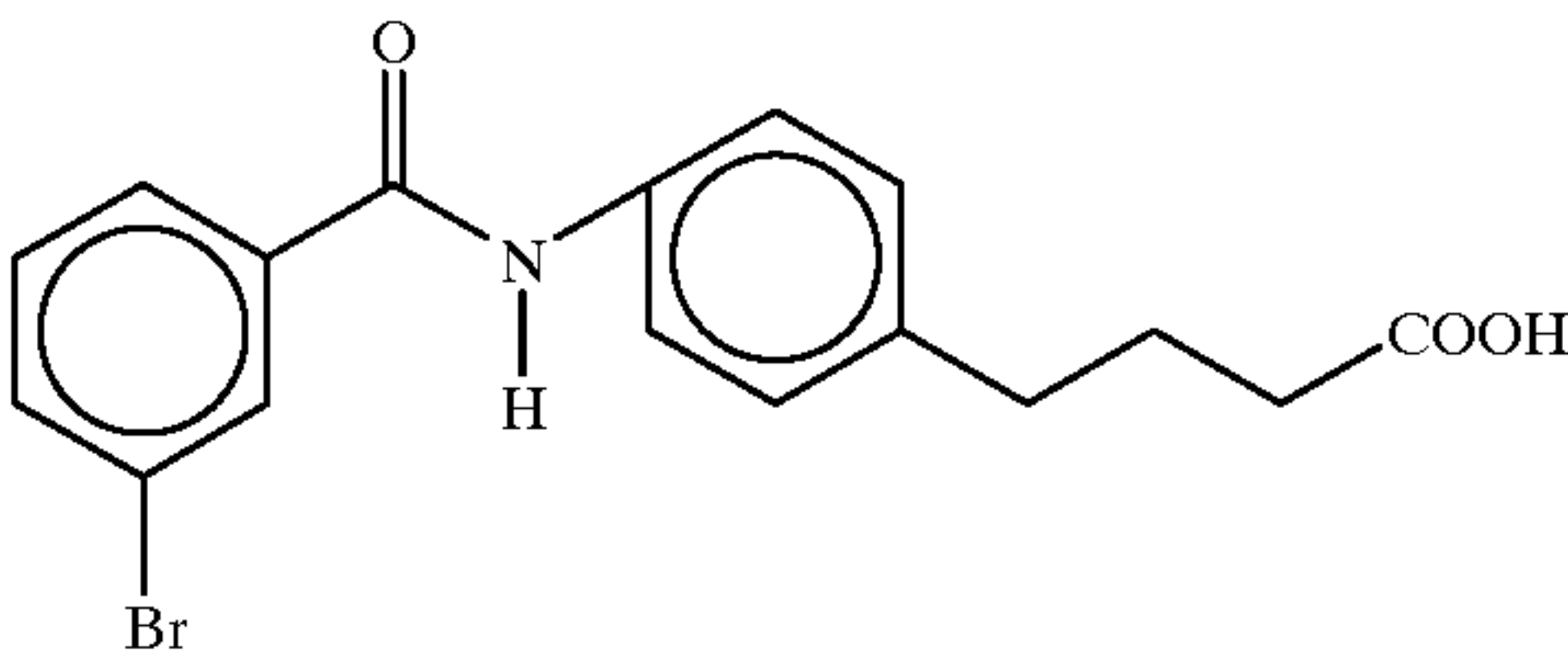
4-{4-[N-3-bromobenzoyl] aminophenyl}} butyric acid
