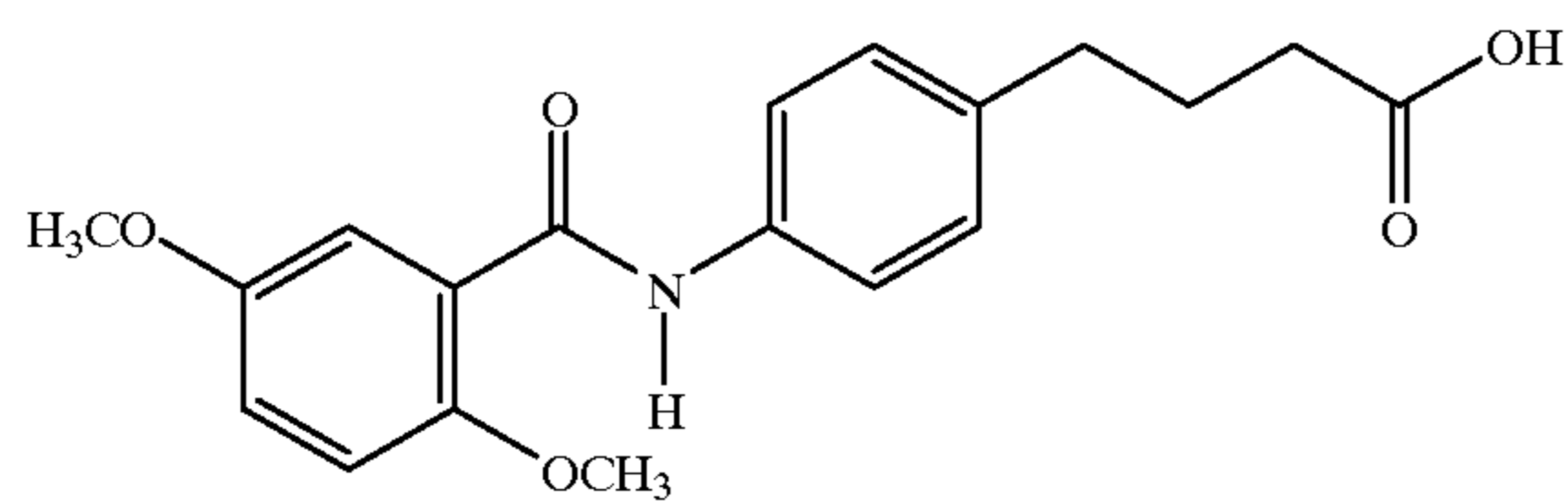
4-(4-(2,5-dimethoxybenzoyl)aminophenyl)butyric acid
