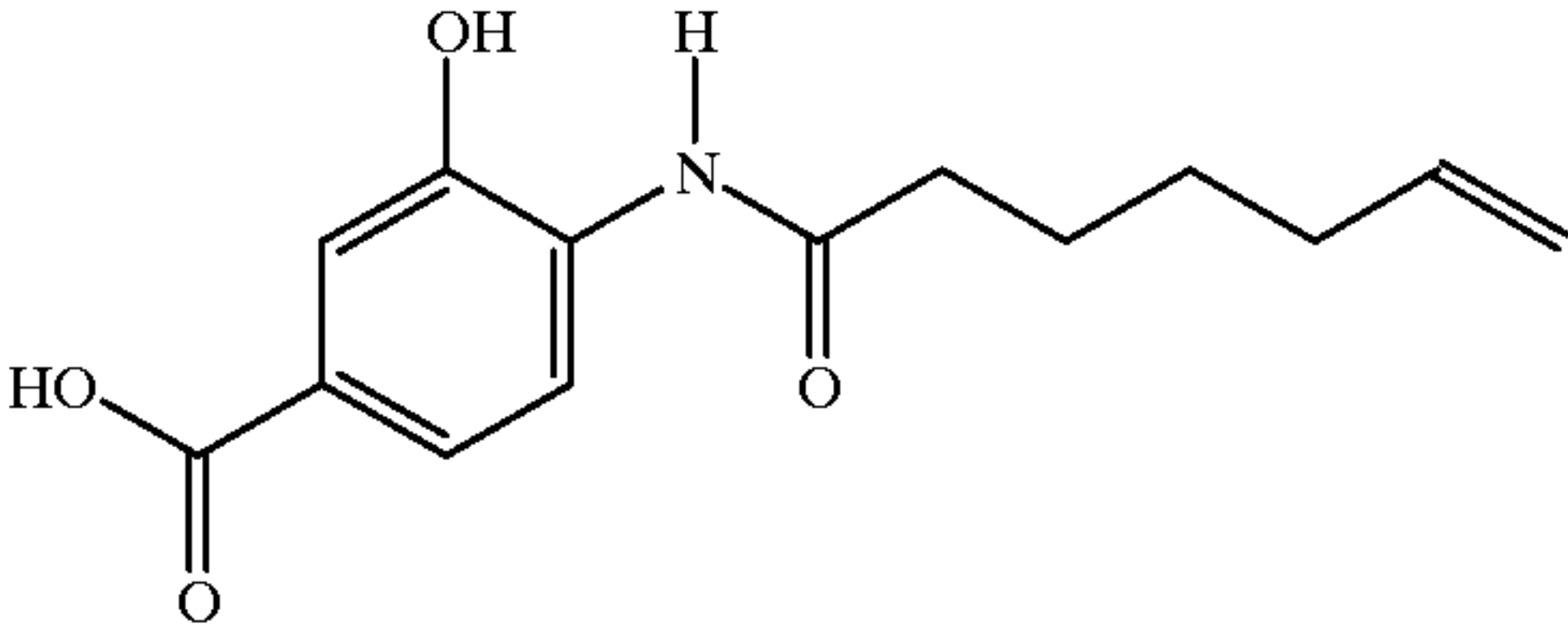
N-(2-hydroxy-4-carboxy)-6-heptenamide
