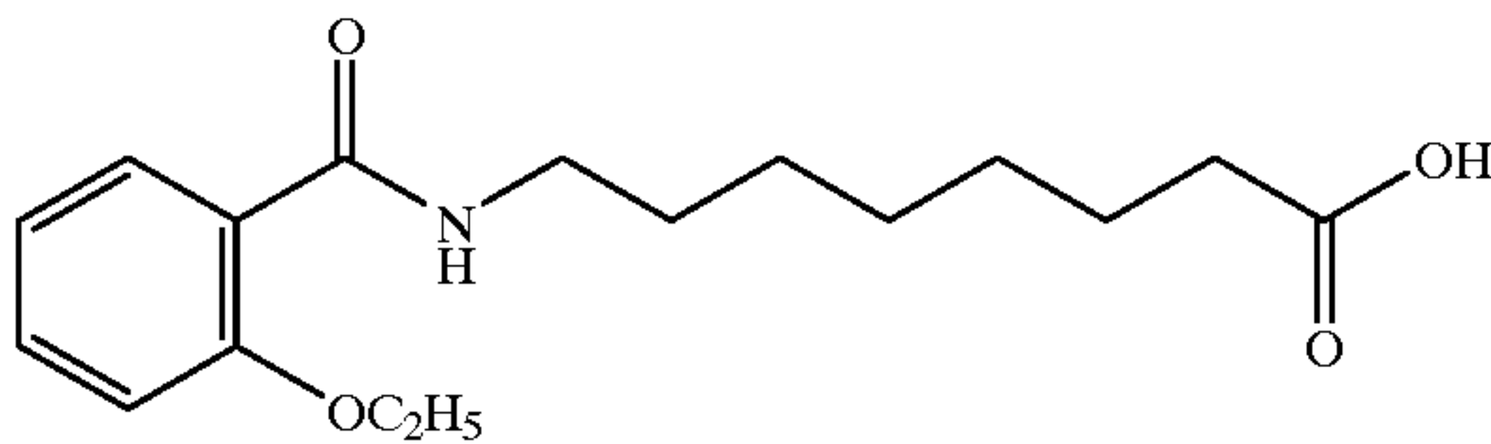
8-(2-ethoxybenzoyl)aminocaprylic acid
