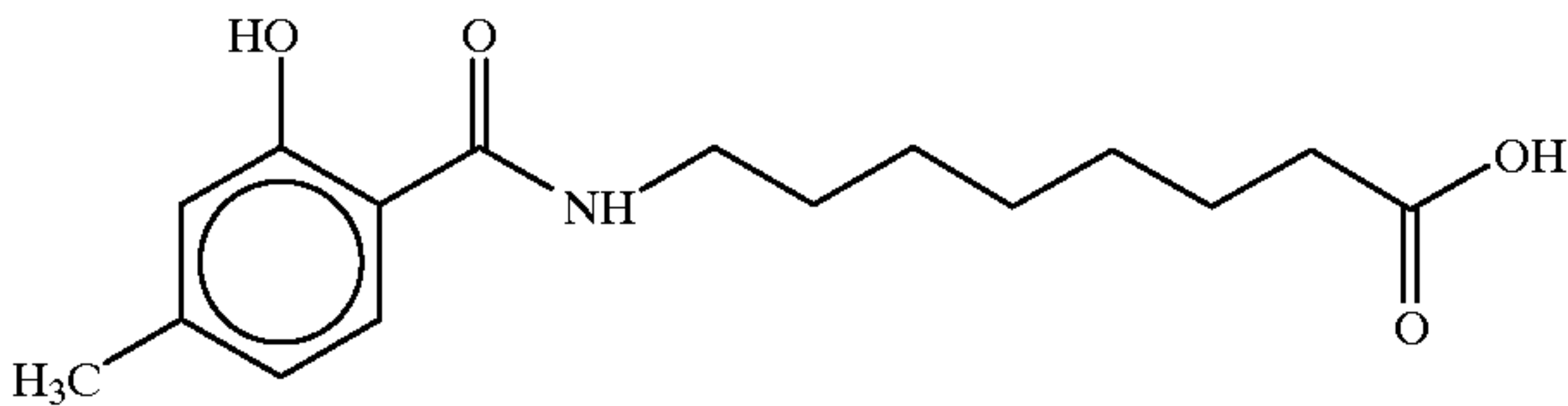
8-(N-4-Methylsalicyloyl)aminocaprillic acid
