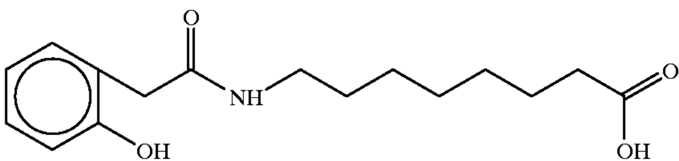
8-(2-hydroxyphenoxy)-aminocaproic acid
