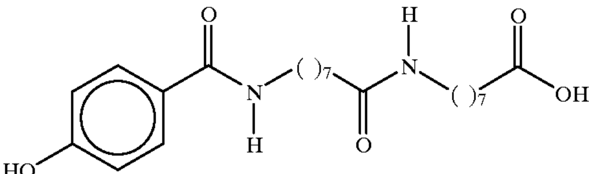
8-(N-4-Hydroxybenzoyl)aminocaprylic acid (dimer)
