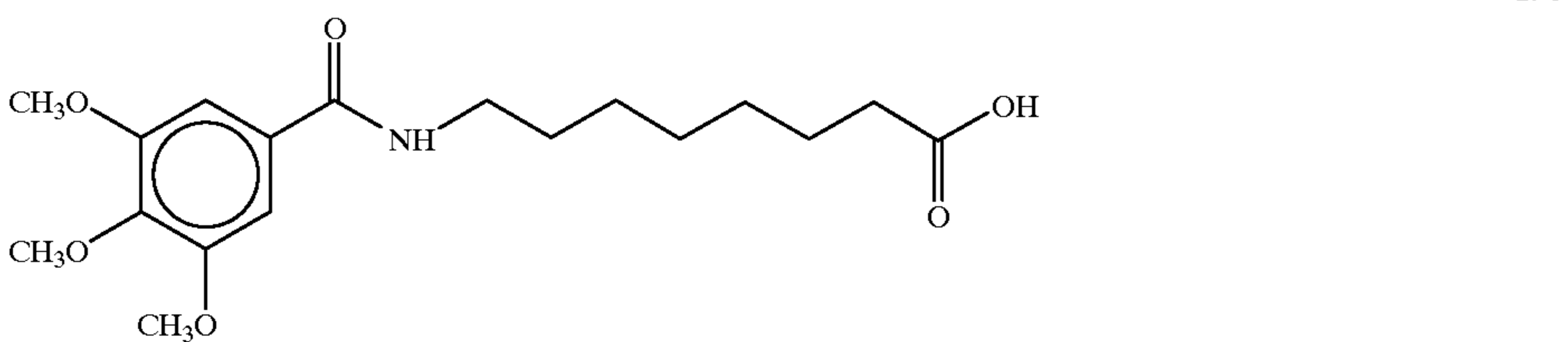
8-(3, 4, 5-Trimethoxybenzoyl)aminocaprylic acid
