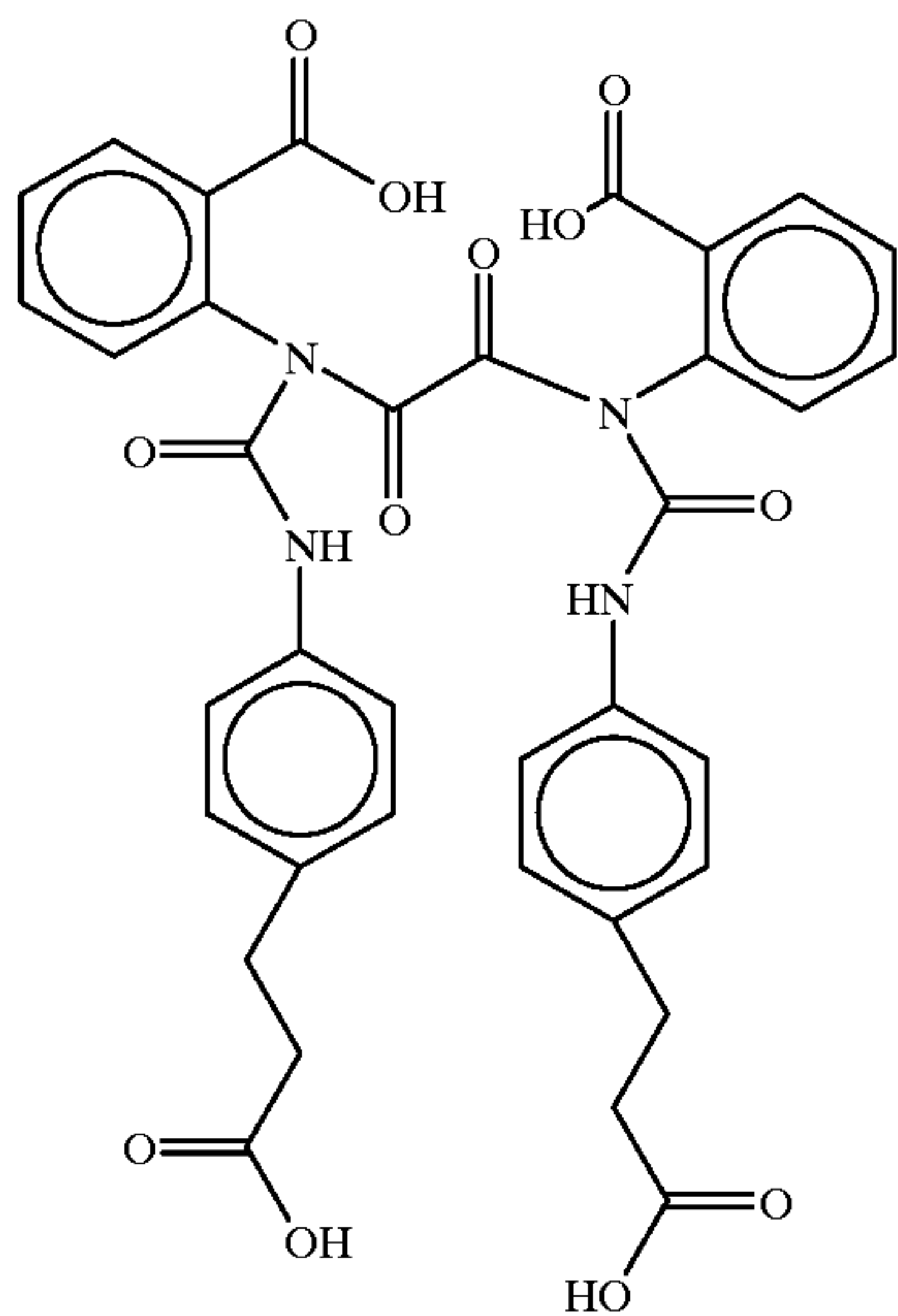
Bis(N-2-carboxyphenyl-N-(N'-3(4-aminophenyl)propionic acid)urea)oxaylyl diamide
