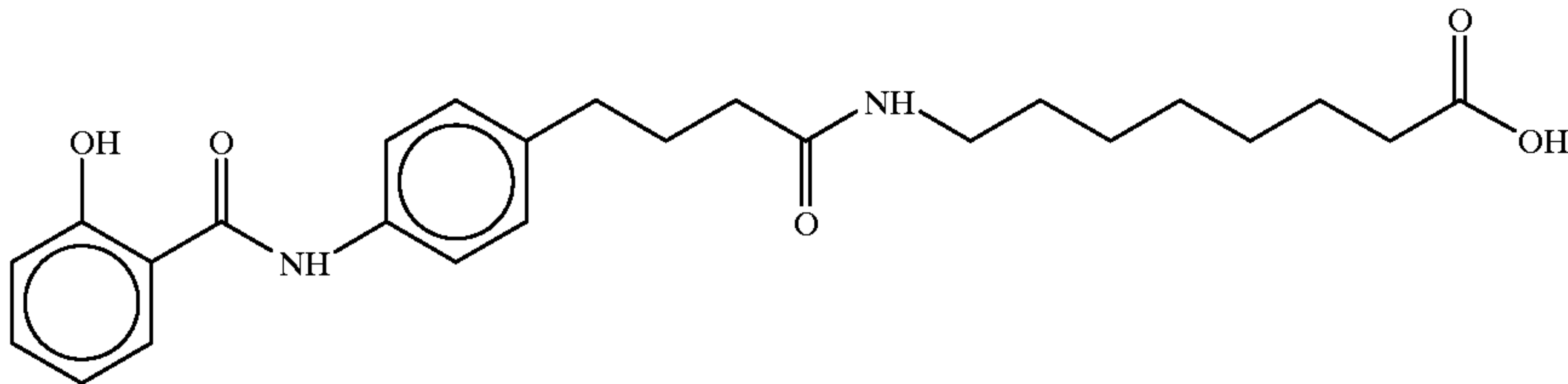
8-(4-(N-Salicyloyl-4aminophenyl)butyric)aminocaprylic acid
