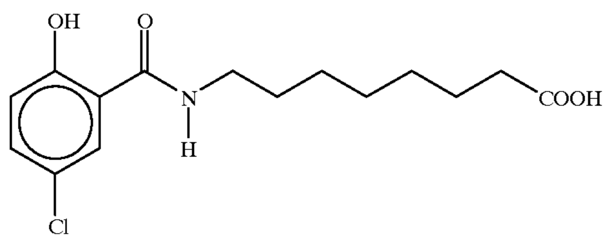
8-(N-2-hydroxy-5-chlorobenzoyl)aminocaprylic acid
