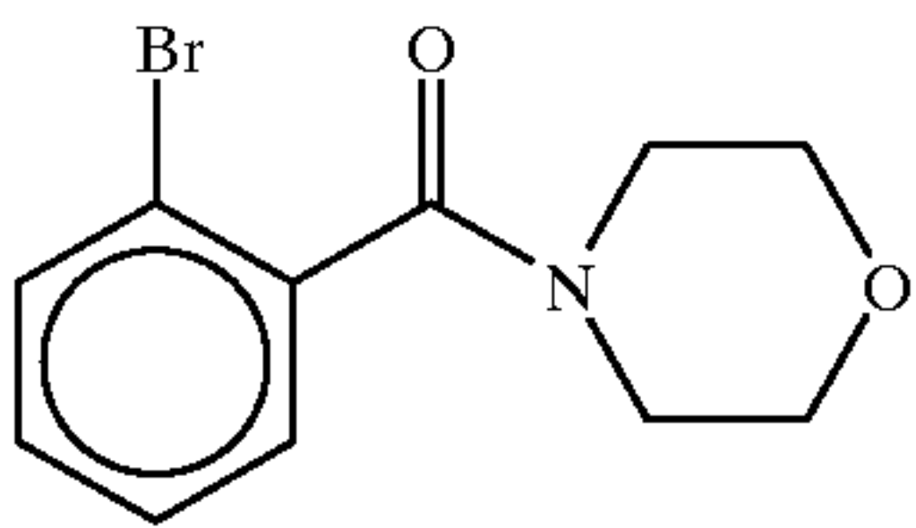
N-(2-bromobenzoyl)morpholine
