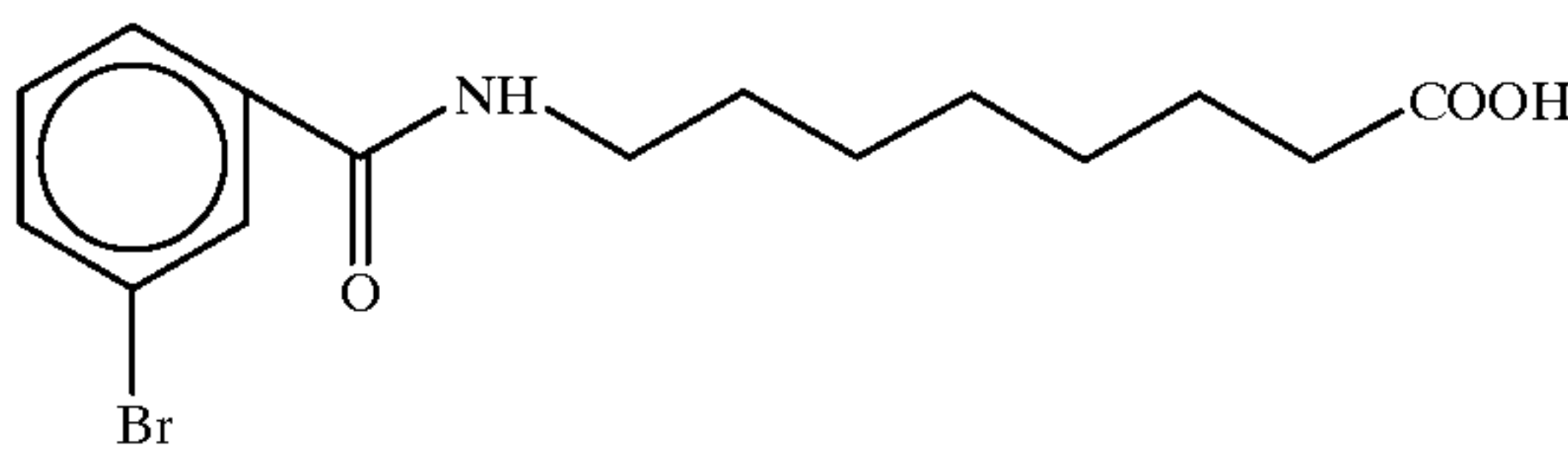
8-[N-(3-bromobenzoyl)]aminocaprylic acid
