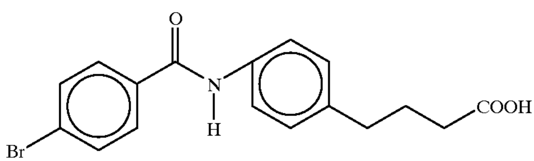
4-[4-[N-(4-bromobenzoyl)aminophenyl]butyric acid
