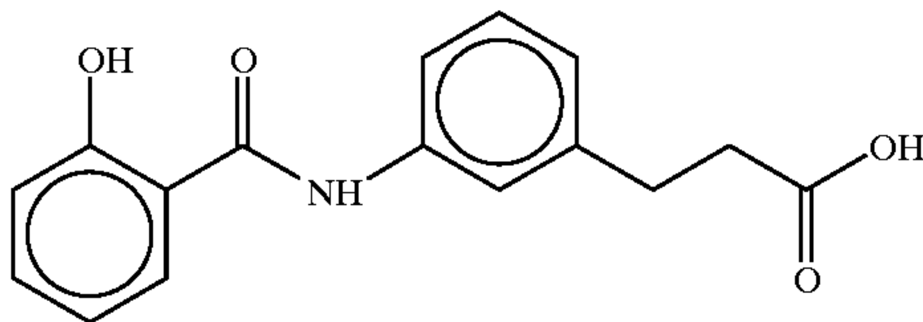
3-(3-(salicyloyl)aminophenyl)propionic acid
