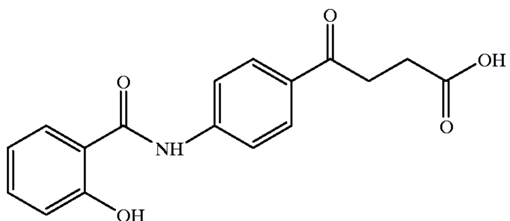
4-(4-salicyloylaminophenyl)-4-oxobutanoic acid
