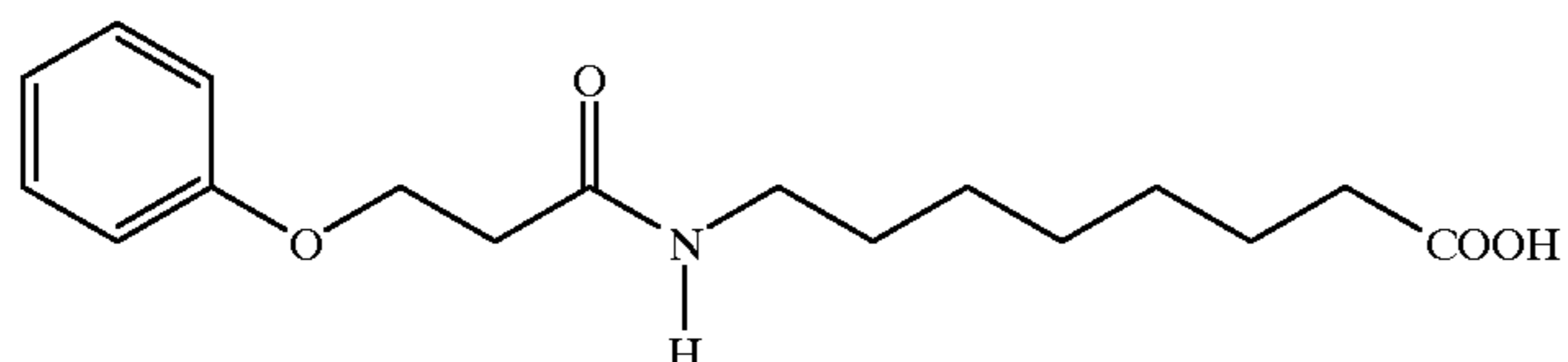
8-(3-Phenoxypropionylamino)caprylic acid
