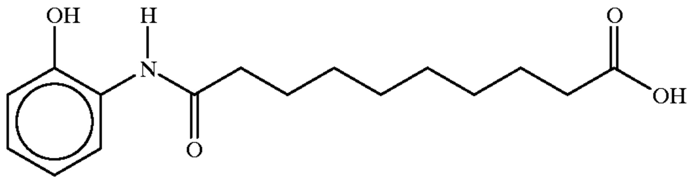
10-(N-2-Hydroxyanilino)sebacic acid
