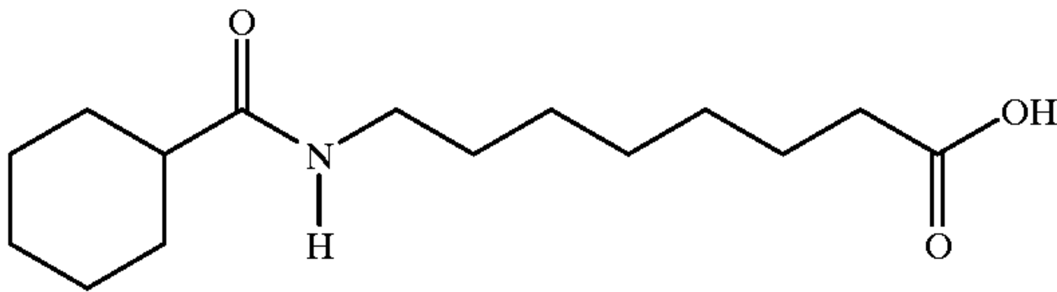
8-N-cyclohexanoylaminovaleric acid
