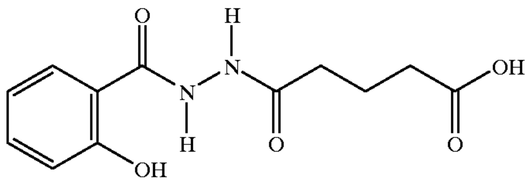
1-salicyloyl-2-glutaryl hydrazide
