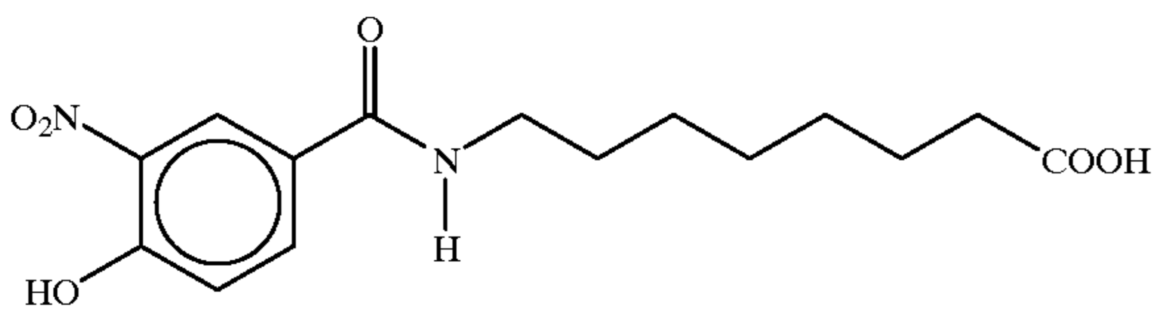
8-N-(4-hydroxy-3-nitrobenzoyl)aminocaprylic acid
