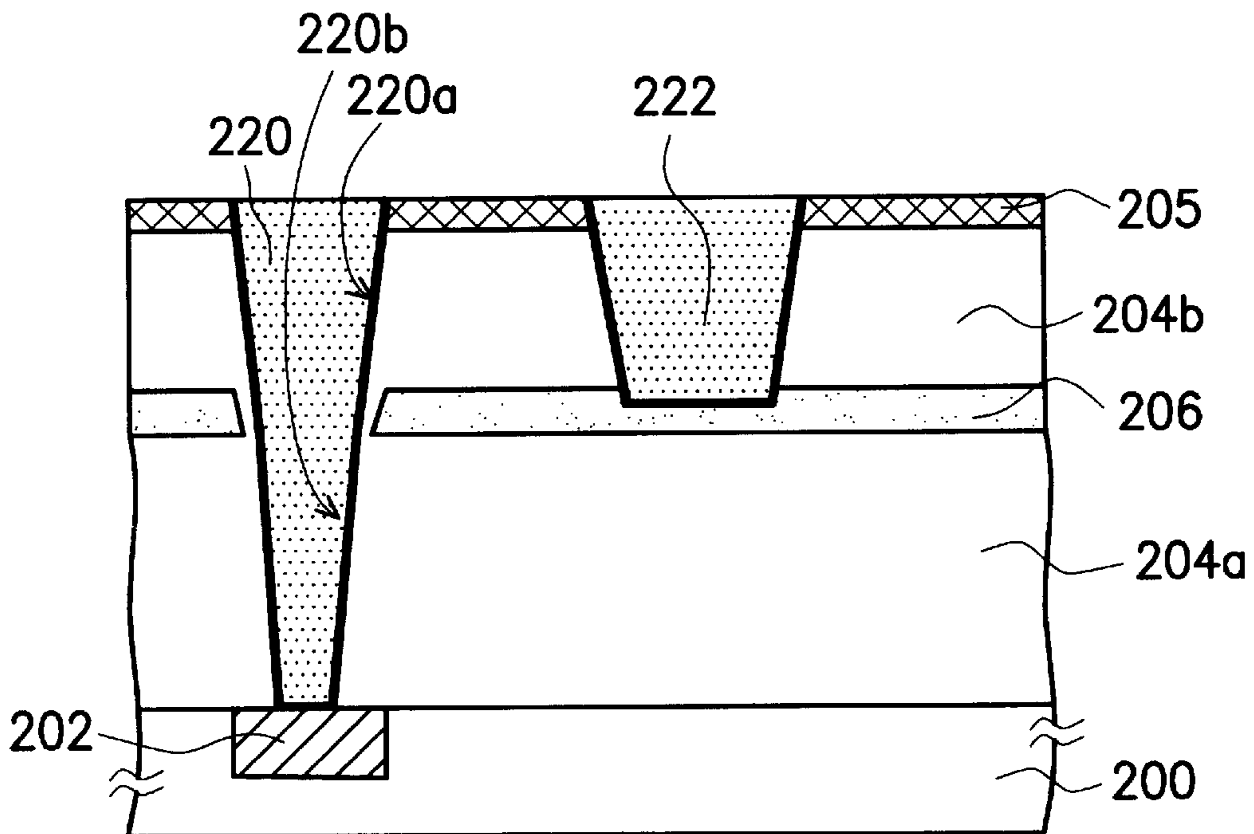
FIG. 4 (PRIOR ART)
