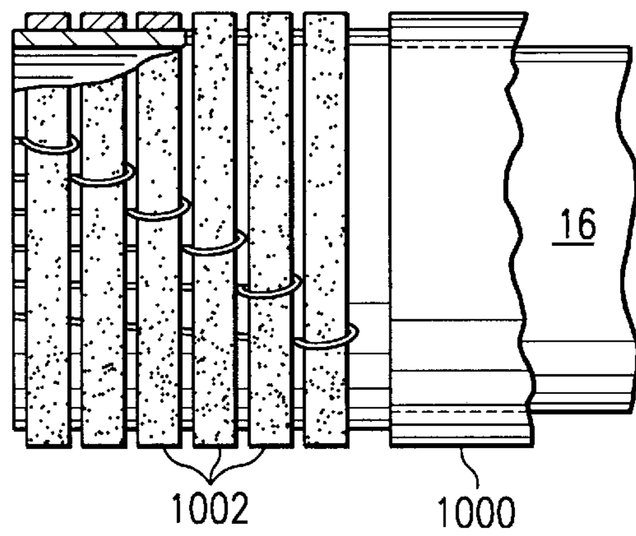
FIG. 3 (PRIOR ART)
