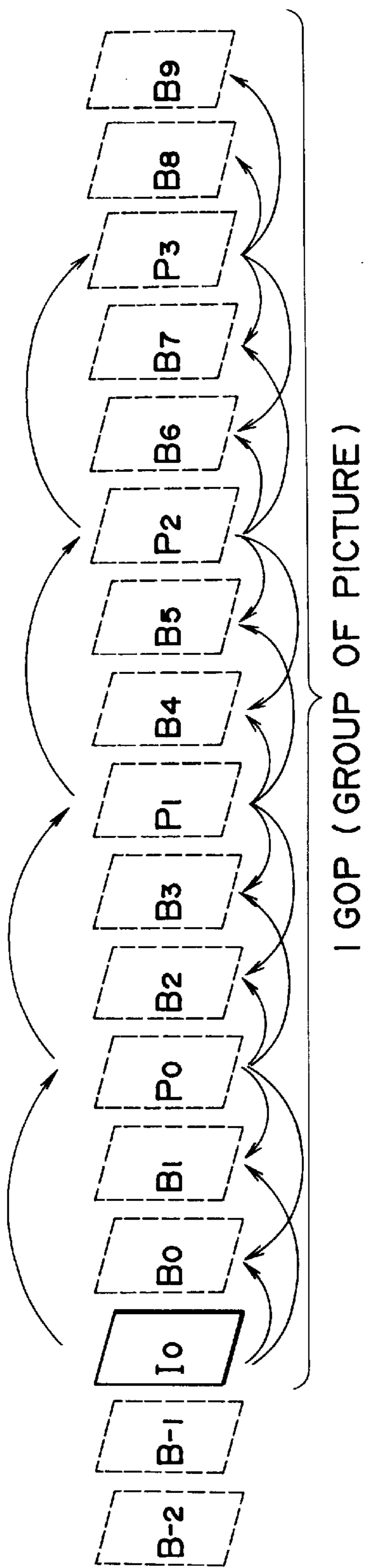
FIG. 10A PREDICTION STRUCTURE OF FRAMES RELATED ART
