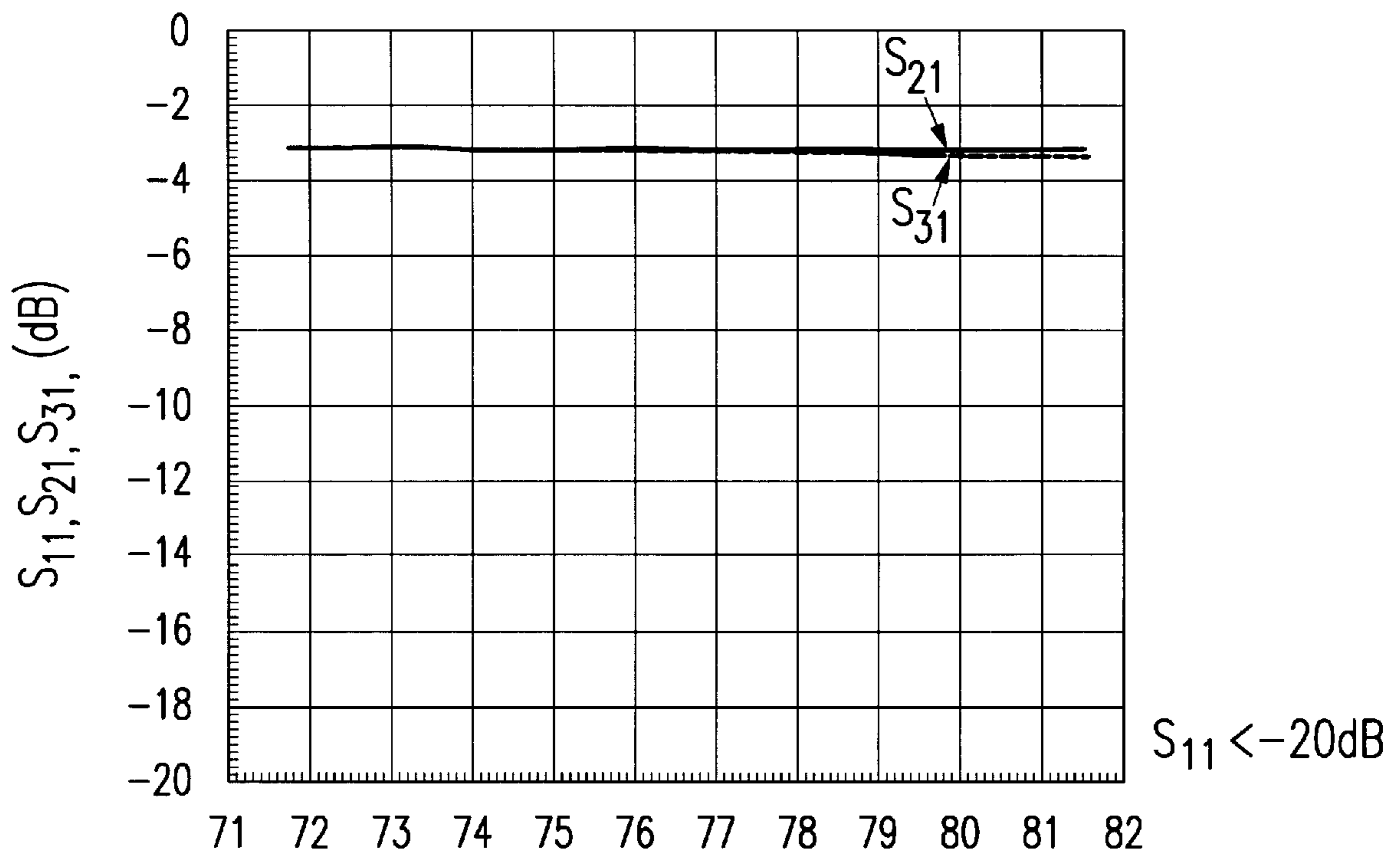
FREQUENCY (GHz) FREQUENCY CHARACTERISTICS
