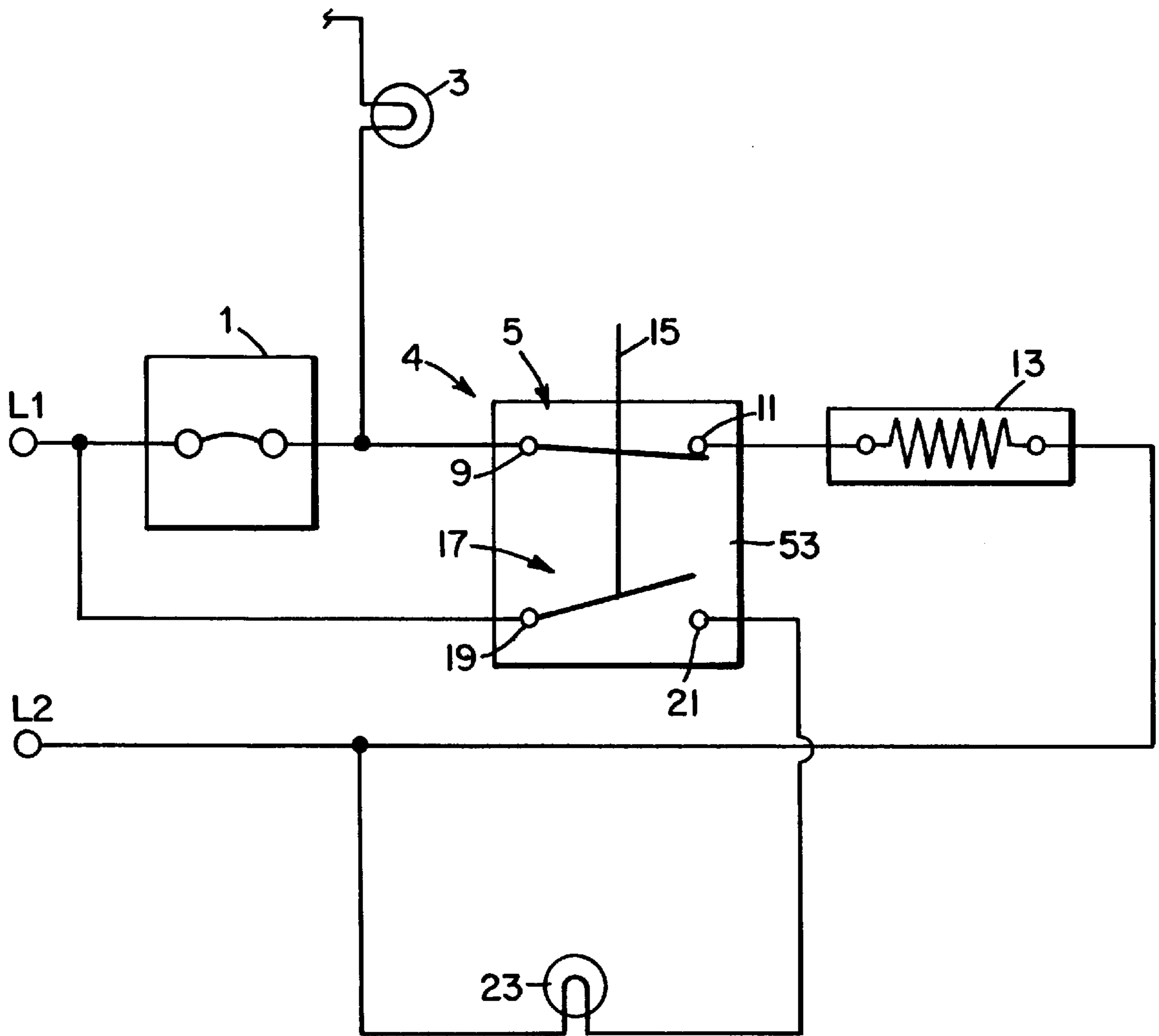
Fig. 1 PRIOR ART
