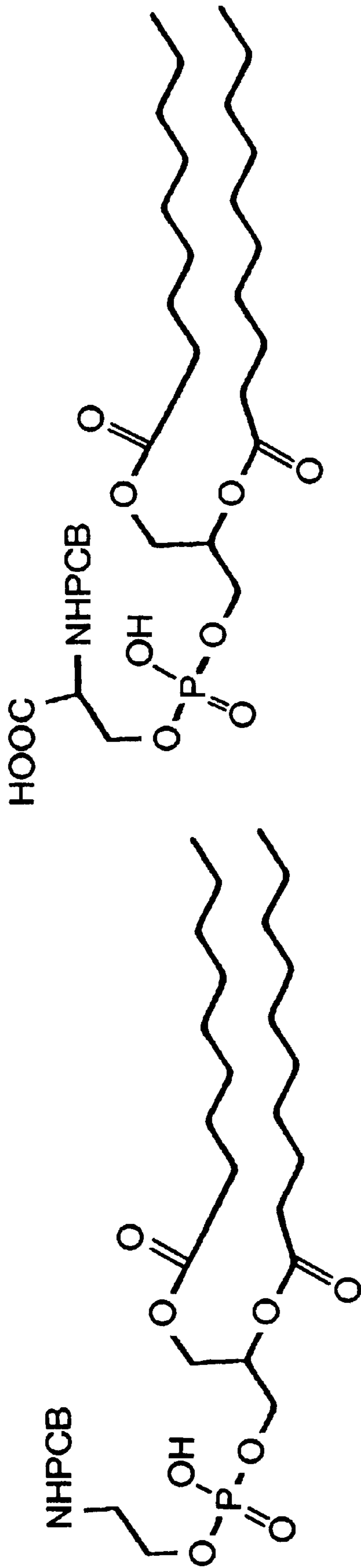
PCB-Phosphatidytserine (PCB-PS)
