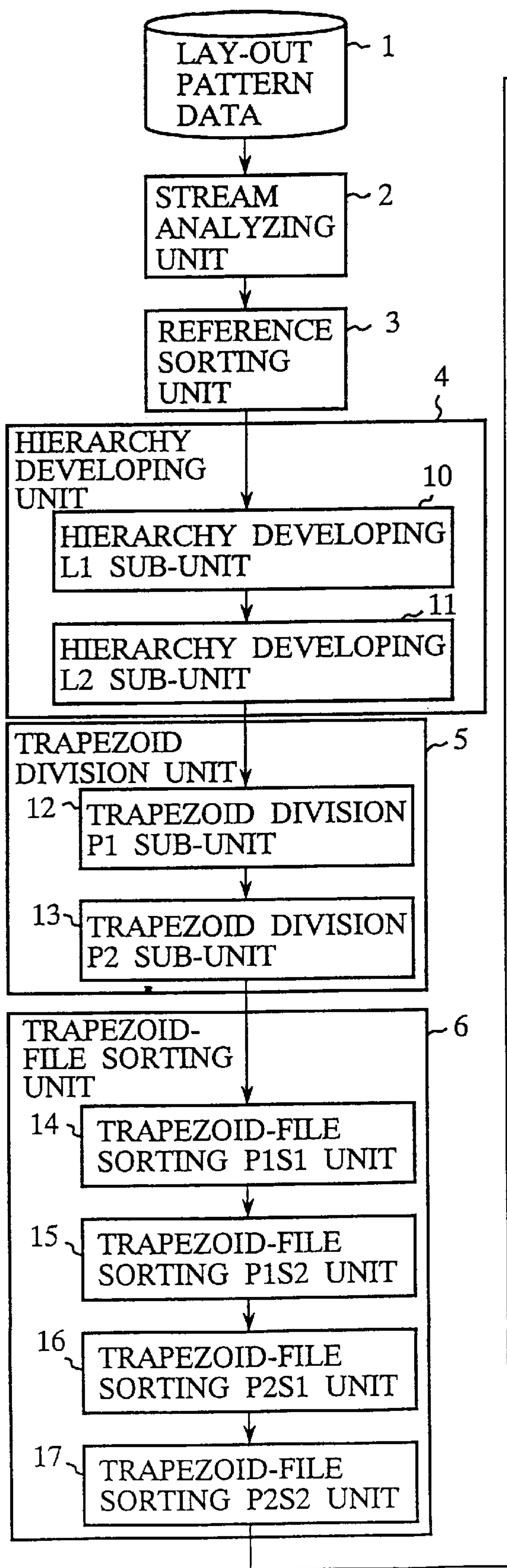
FIG.8 (PRIOR ART)
