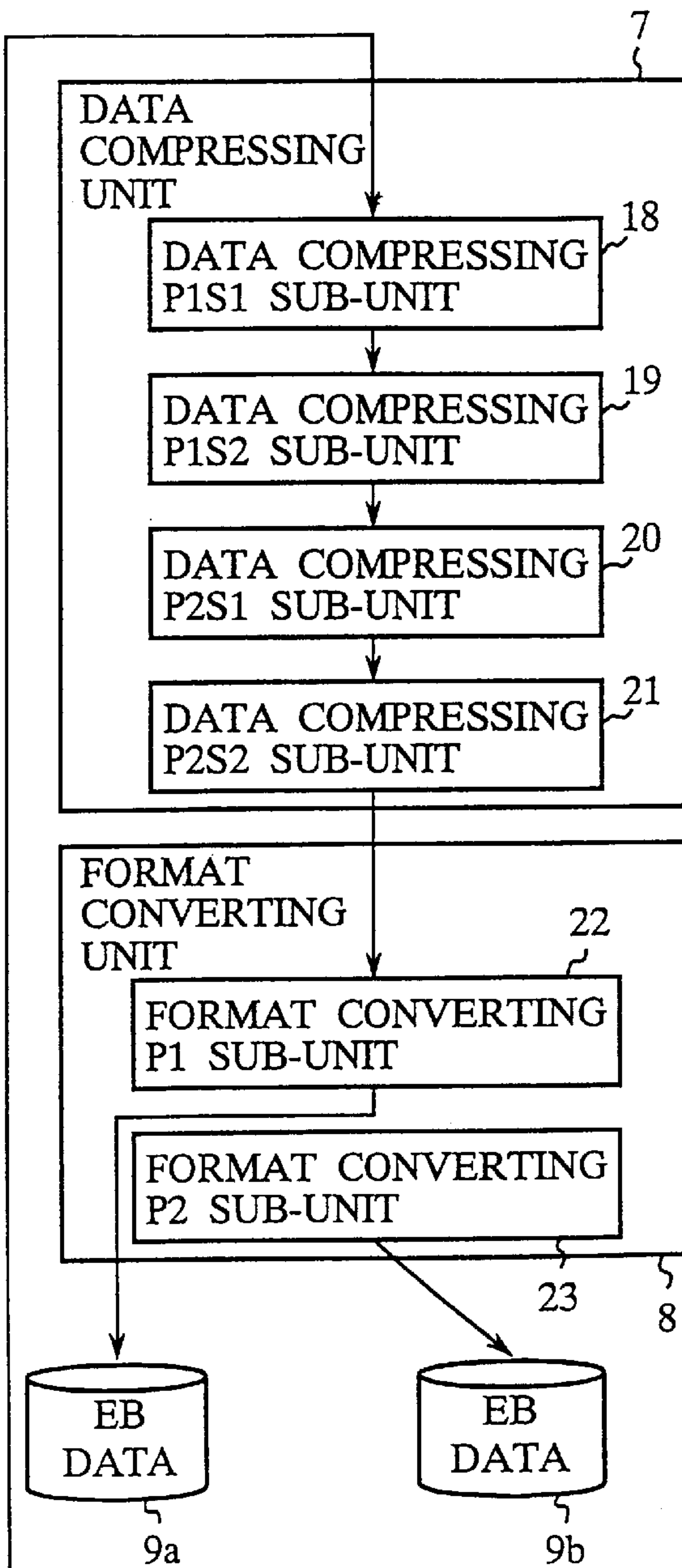
FIG.8 (PRIOR ART)
