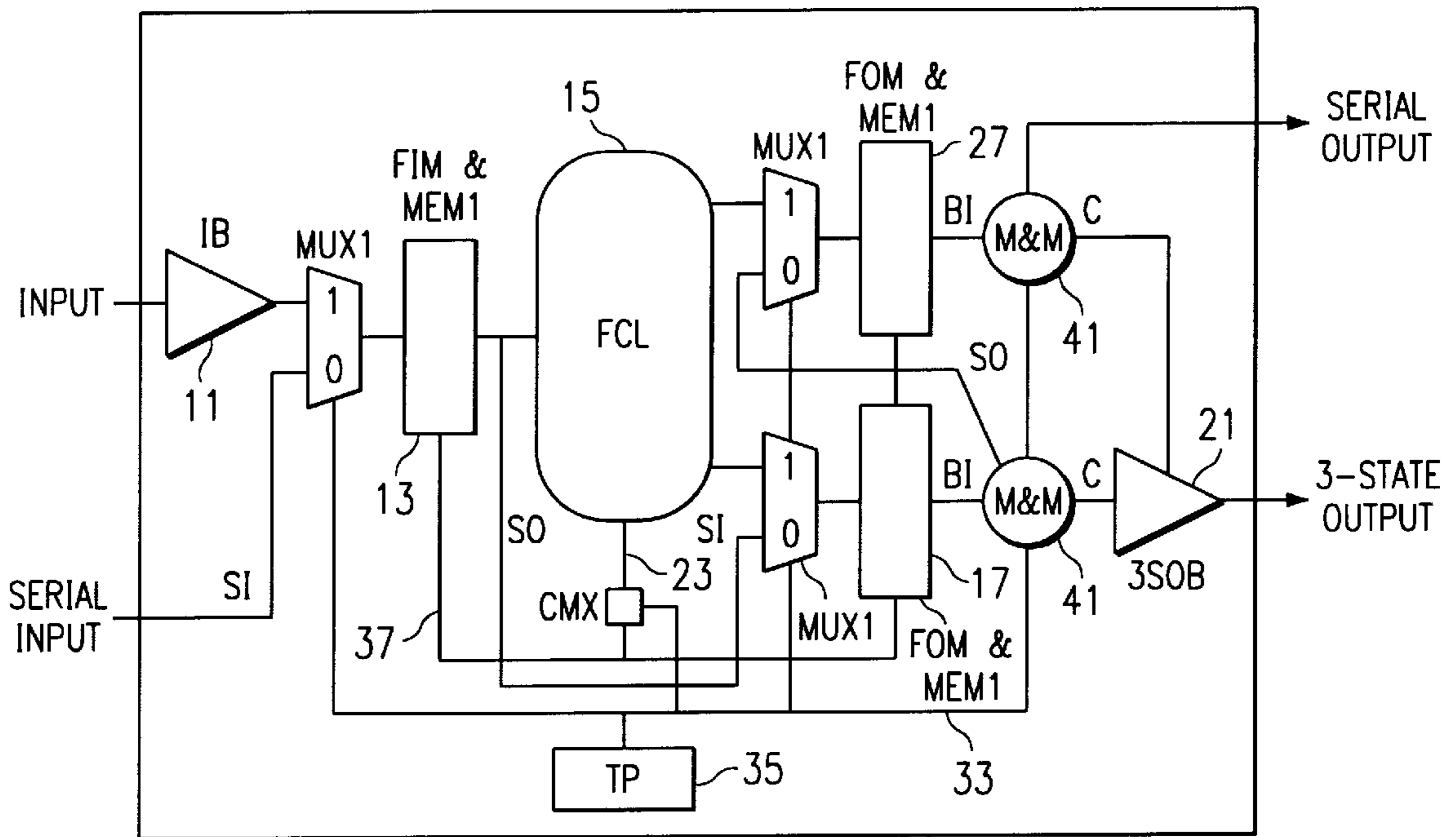
FIG. 6 (PRIOR ART)
