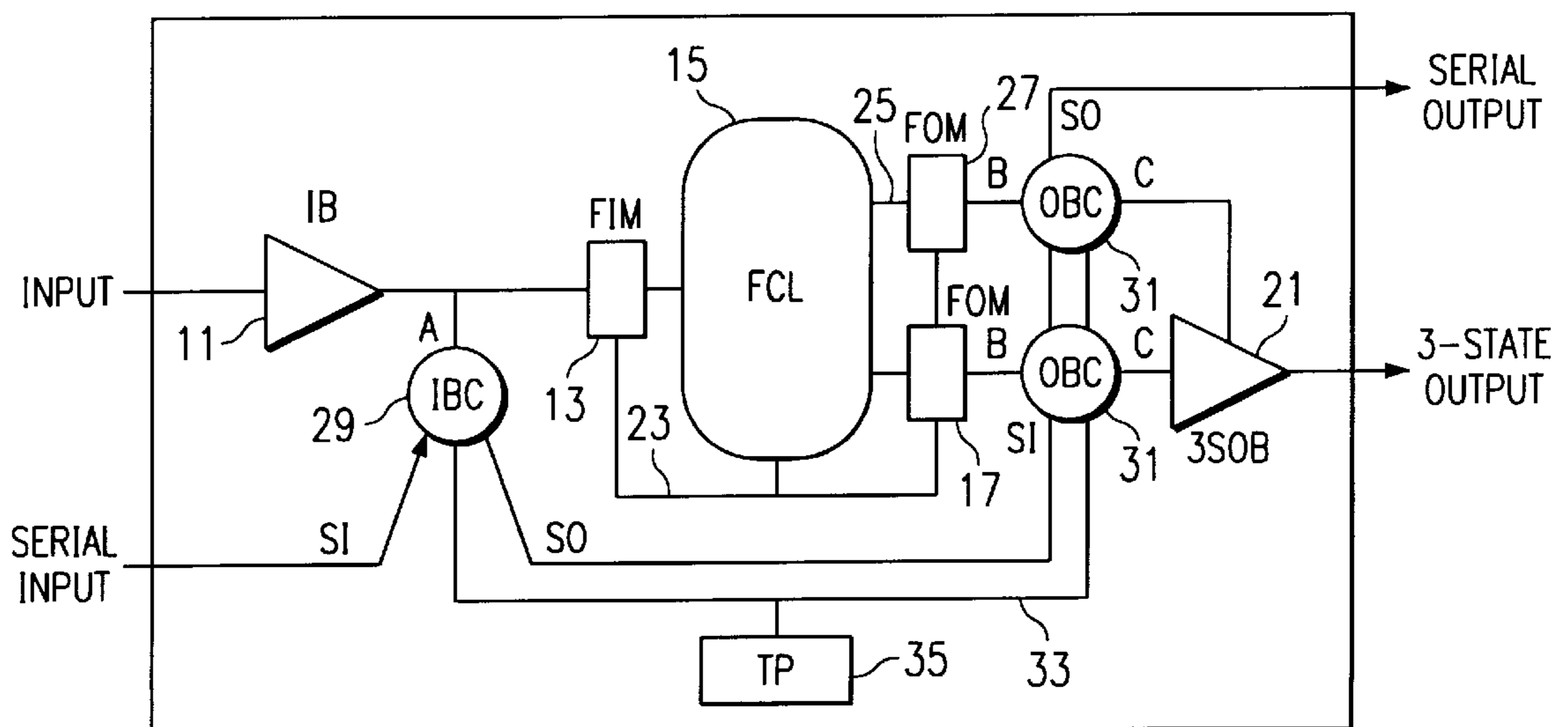
FIG. 4 (PRIOR ART)
