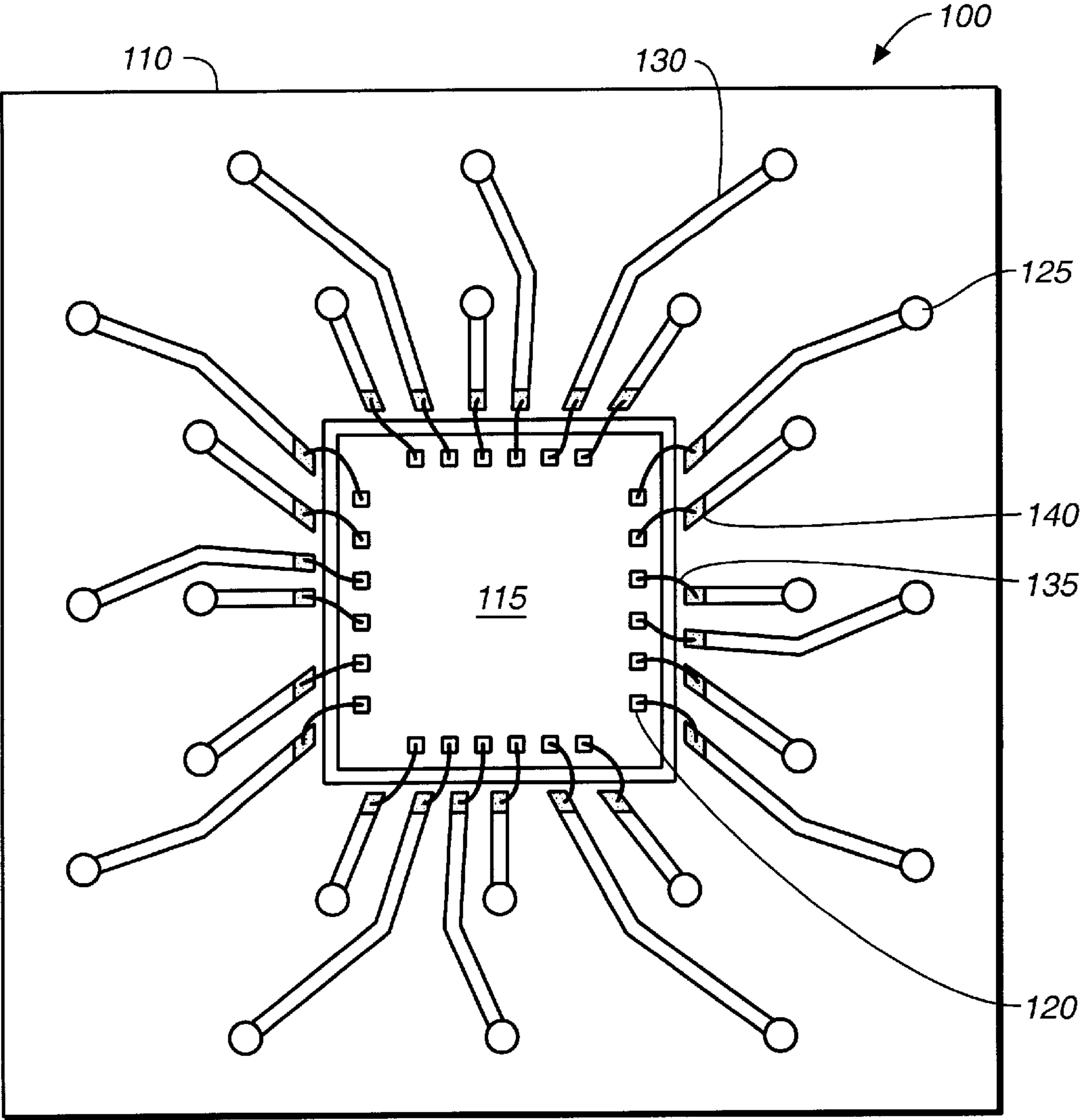
FIG. 1 (PRIOR ART)
