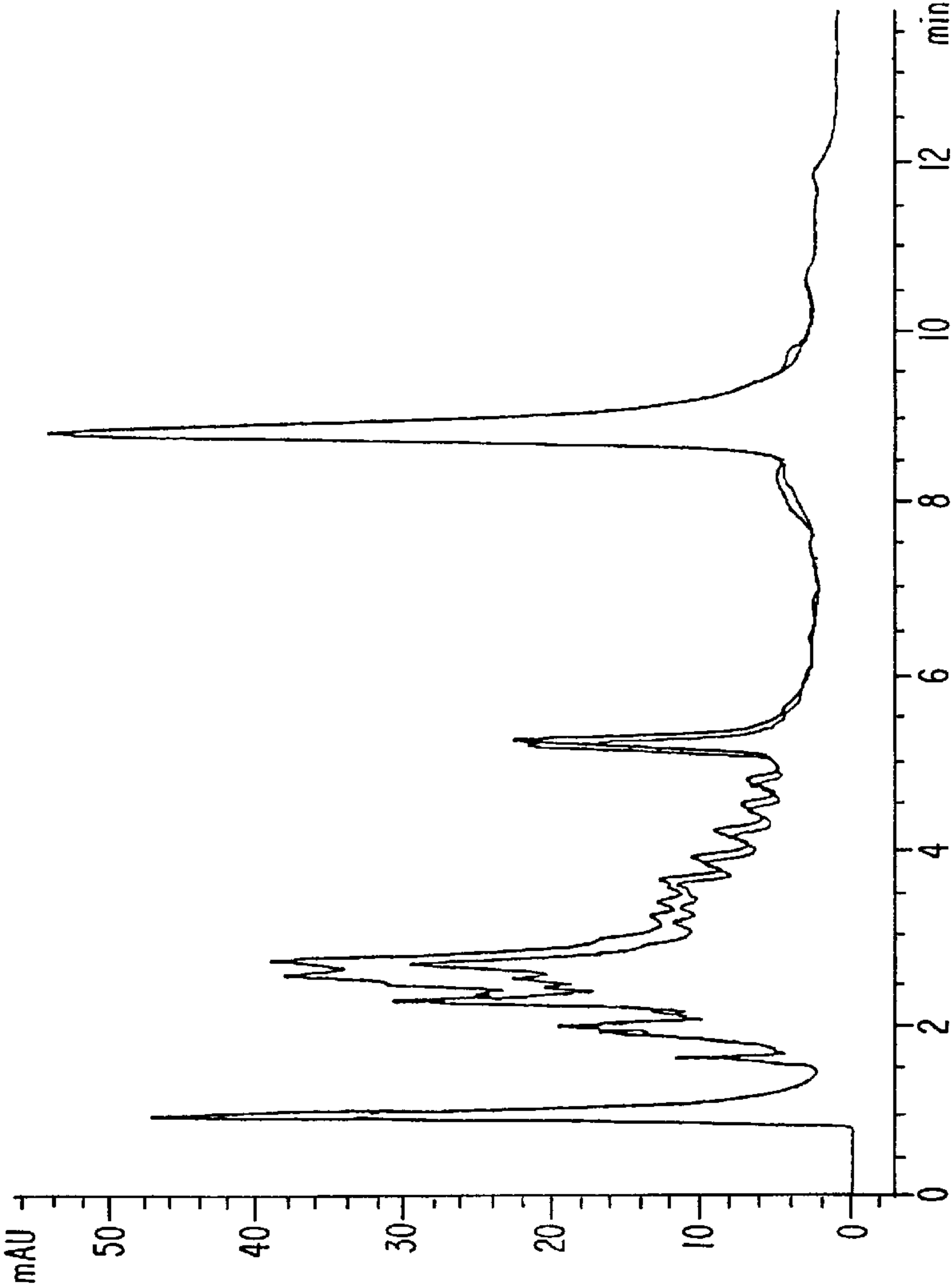
FIG. 3. Overlay of chromatograms of "one-pot" or "two pot" deprotected RPI.3703 ribozyme RPI.3703 g s u s u s u s uc ccu GAu Gag gcc gaa agg ccG aaA uuc uccB 200nmoles scale
