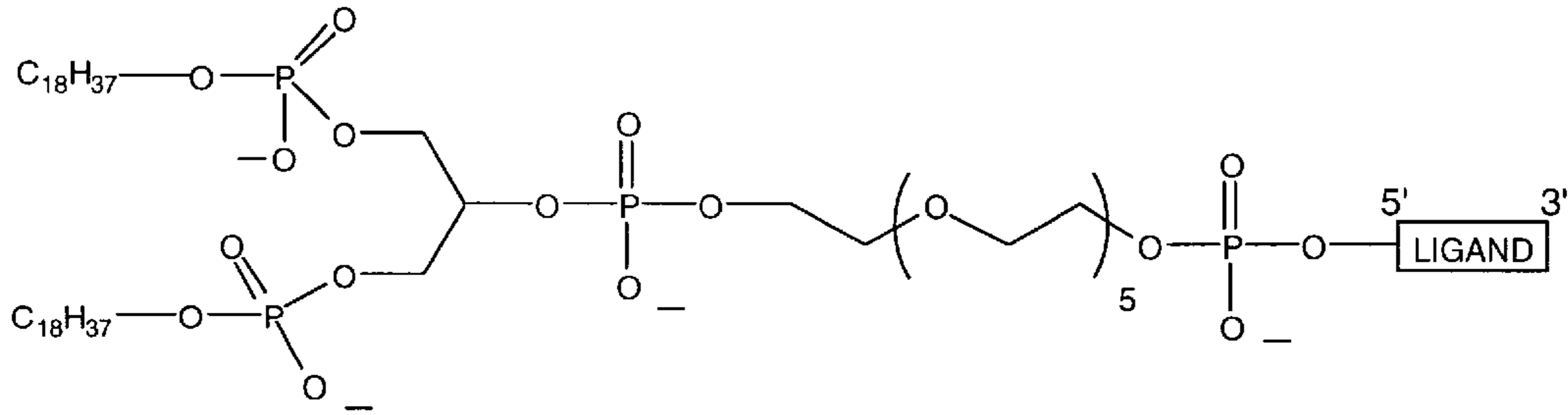
NX31838 - PL
