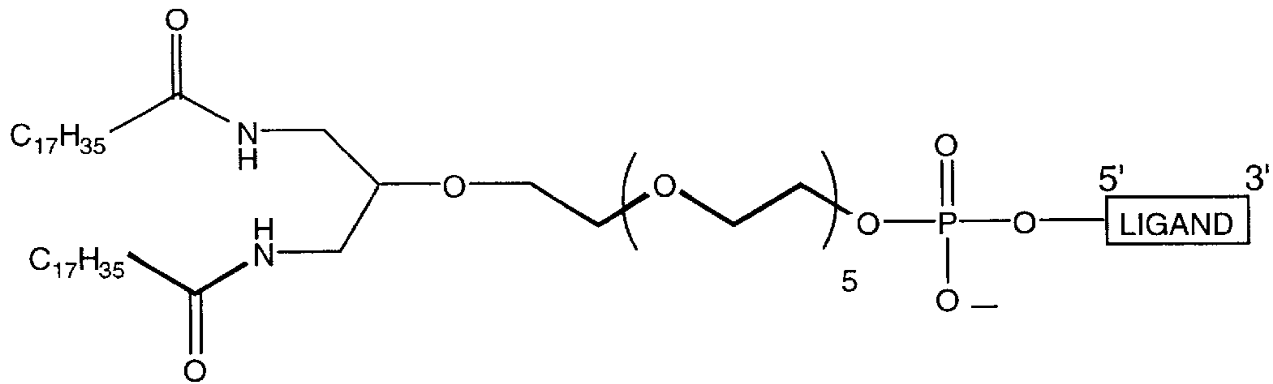
NX31838 Lipid-amide 2
