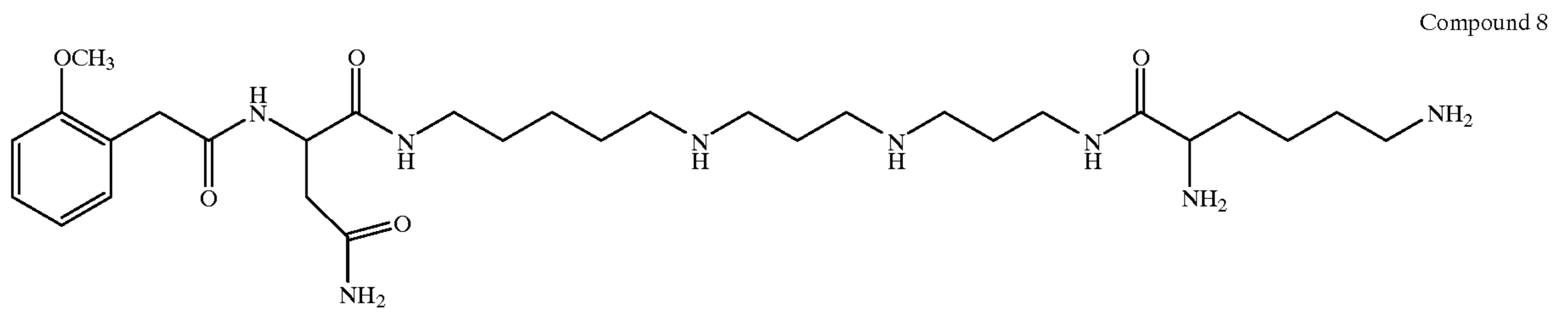
Compound 9
