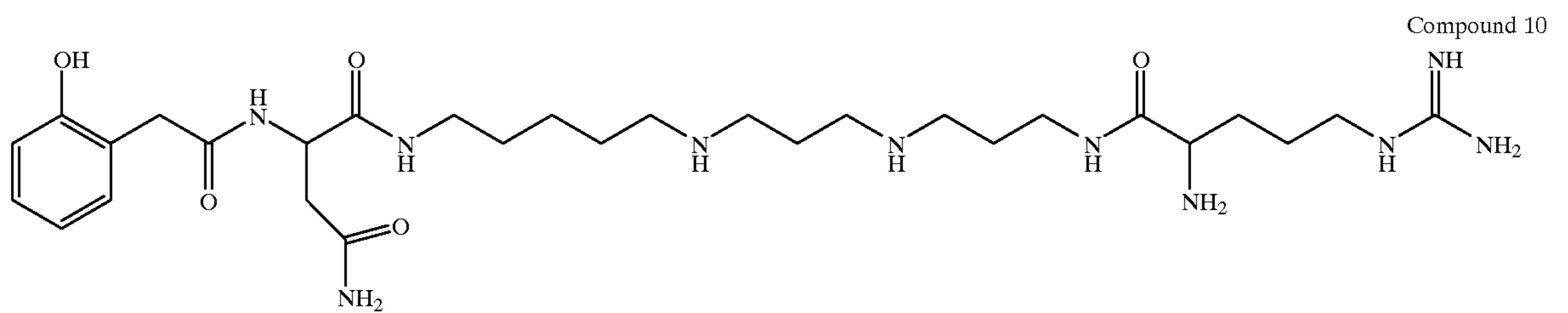
Compound 11
