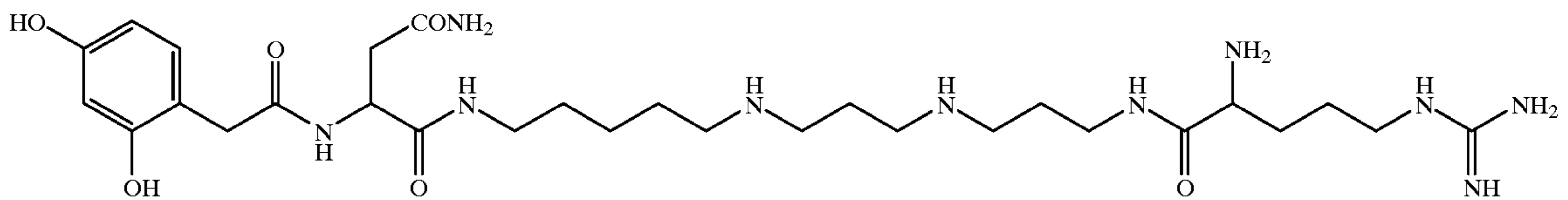
Compound 2
