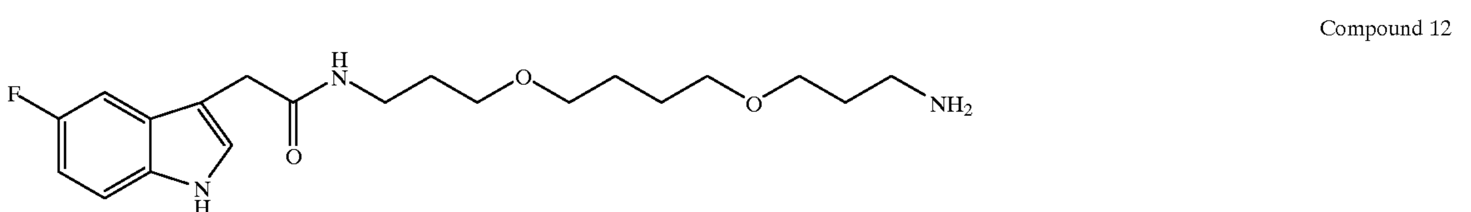
Compound 13
