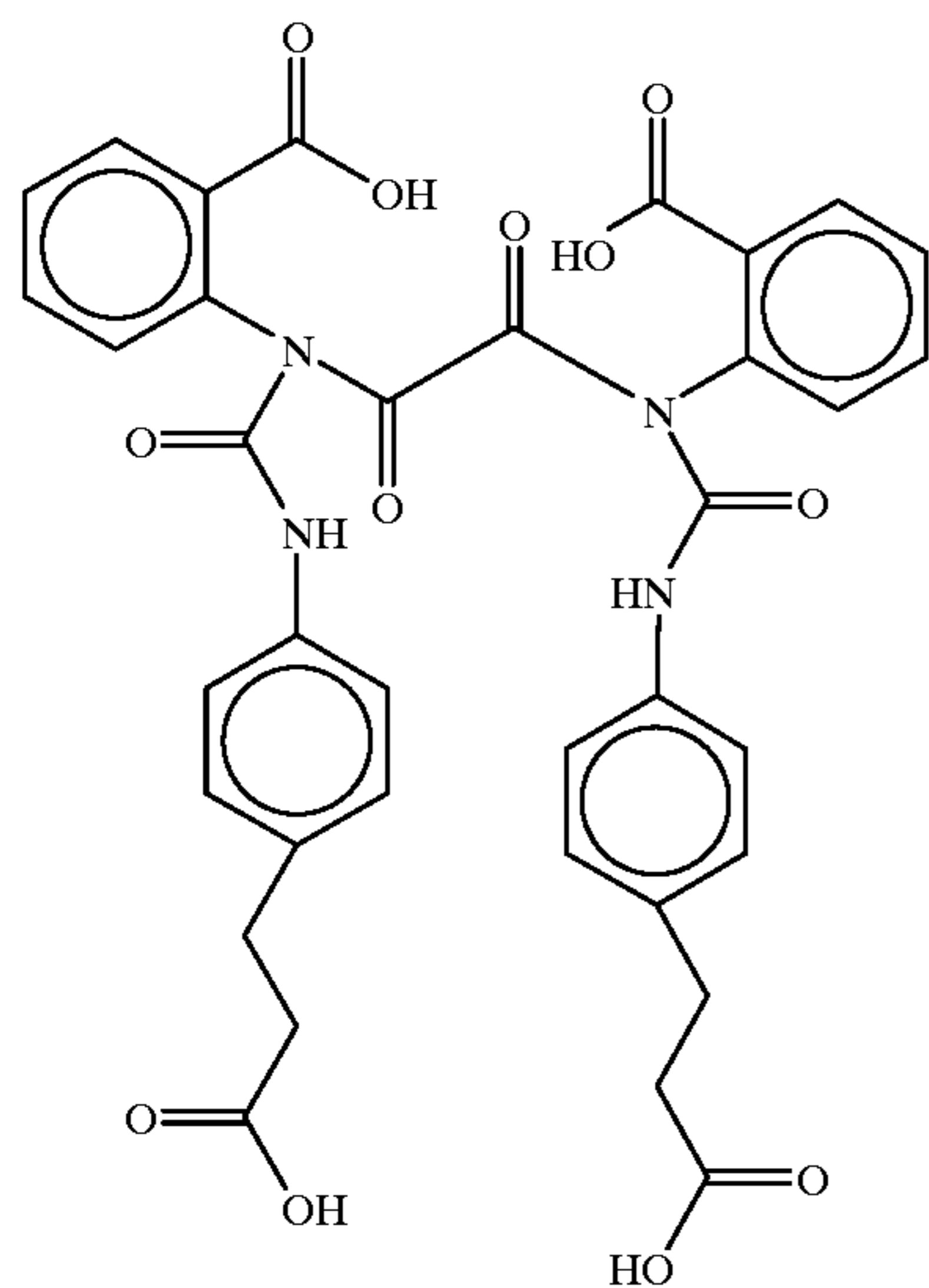
Bis(N-2-carboxyphenyl-N-(N'-3(4-aminophenyl)propionic acid)ureal)oxaylyl diamide
