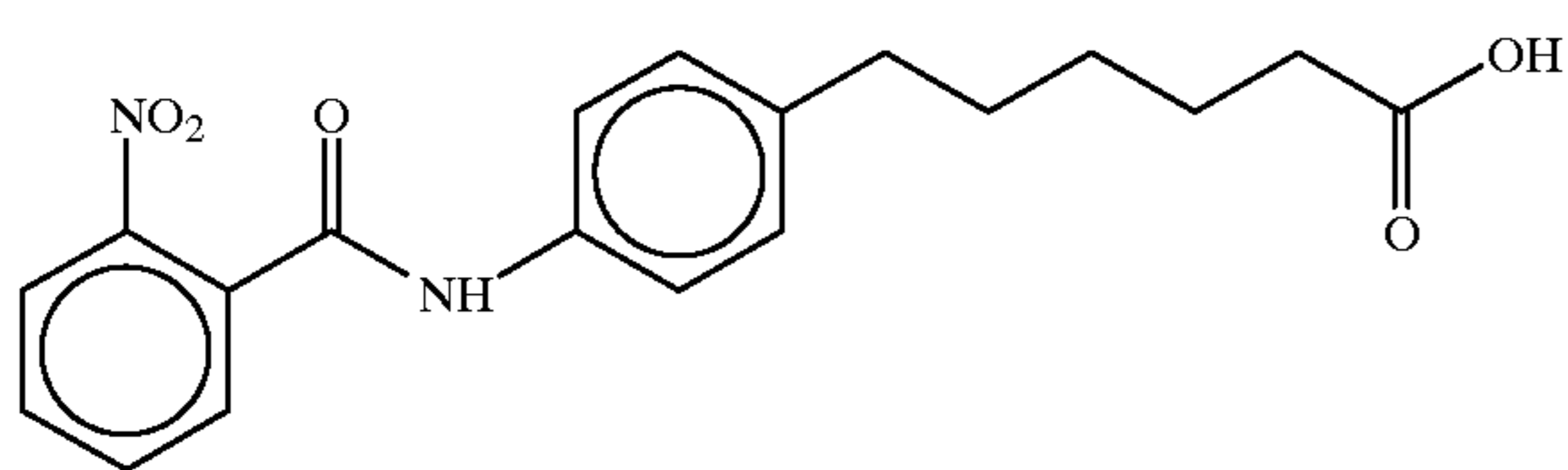
6-(4-(N-2-Nitrobenzoyl)aminophenyl)hexanoic acid
