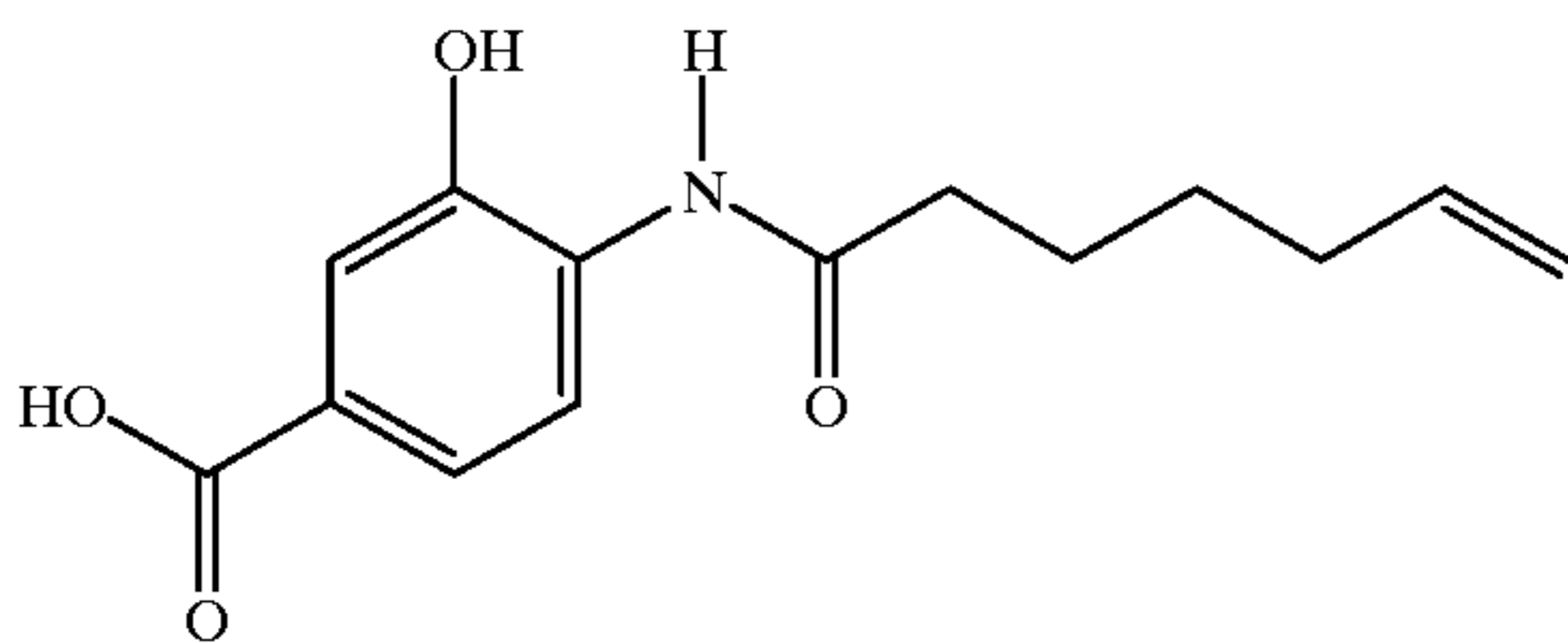
N-(2-hydroxy-4-carboxy)-6-heptenamide
