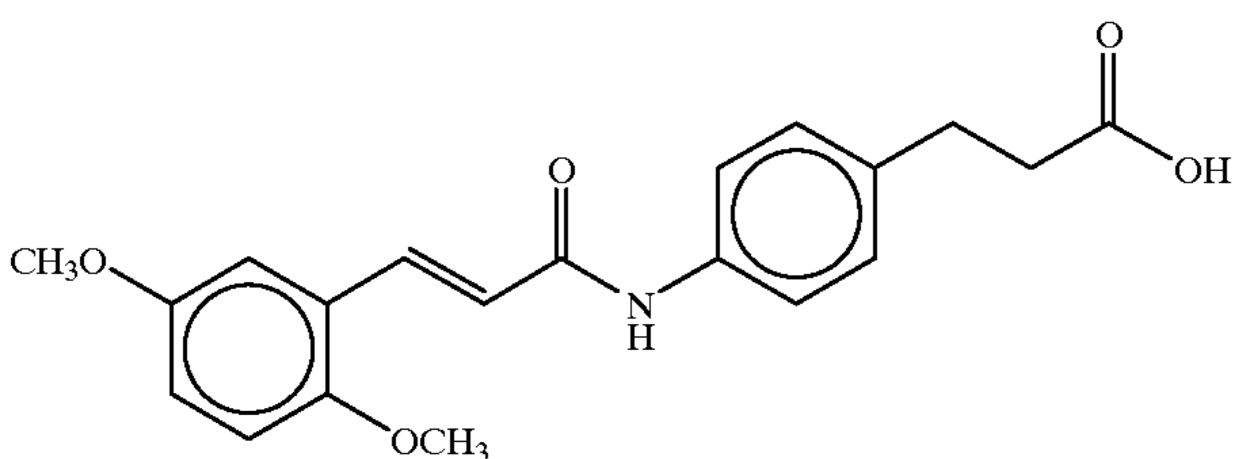
3-(4-(2,5-dimethoxycinnamoyl)aminophenyl)propionic acid
