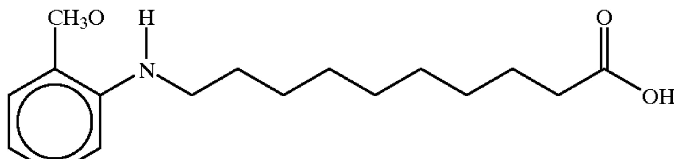
2-Methoxybenzenaminodecanoic acid
