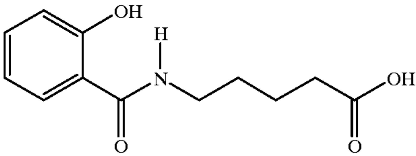
5-(N-salicyloylamino)valeric acid
