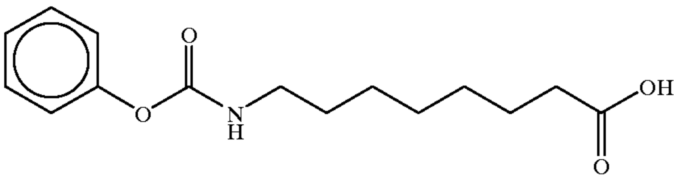
8(phenylcarbonylamino)caprylic acid
