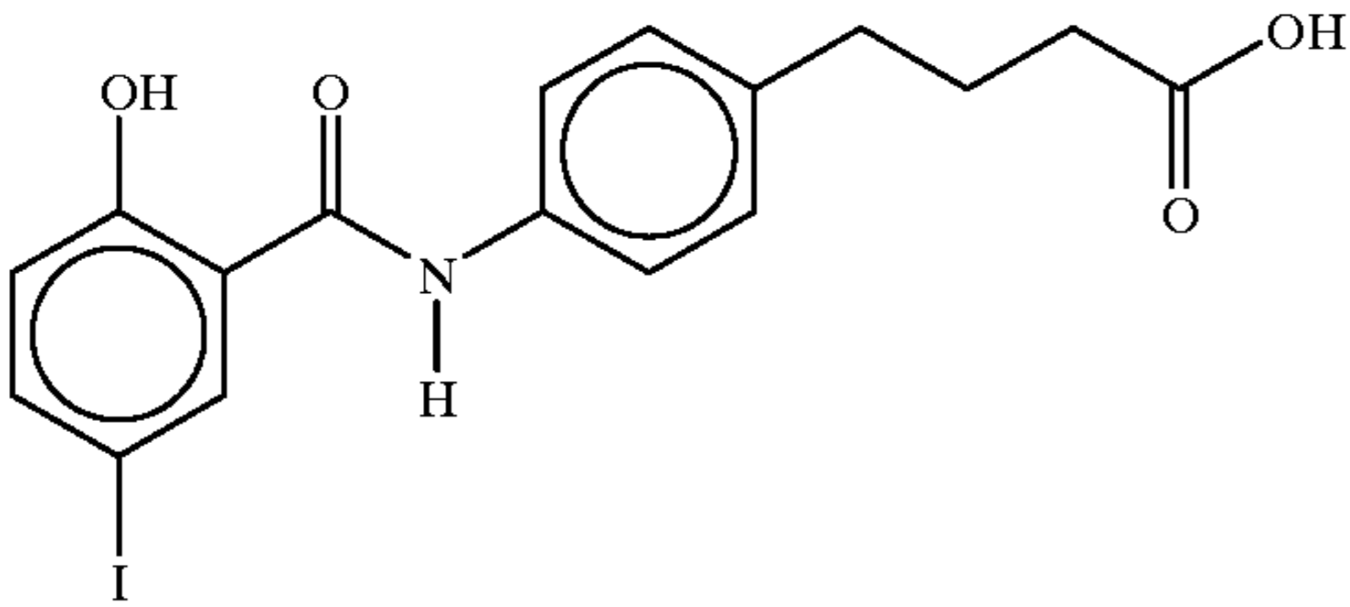
4-{-[N-(2-hydroxy-5-iodobenzoyl)]aminophenyl}butyric acid
