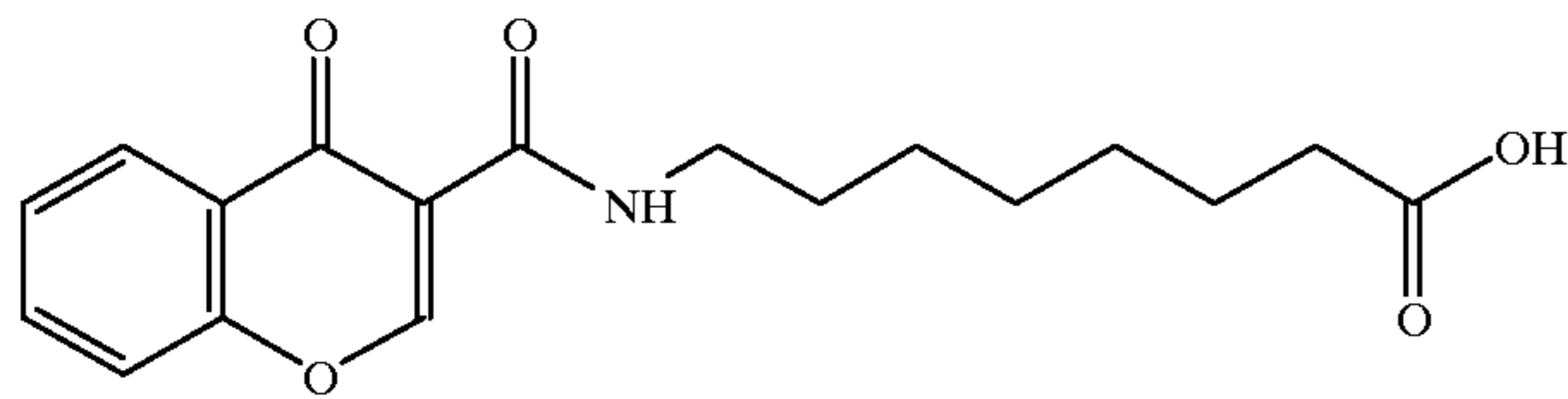
8-(chromone-3-carbonyl)aminocaprylic acid
