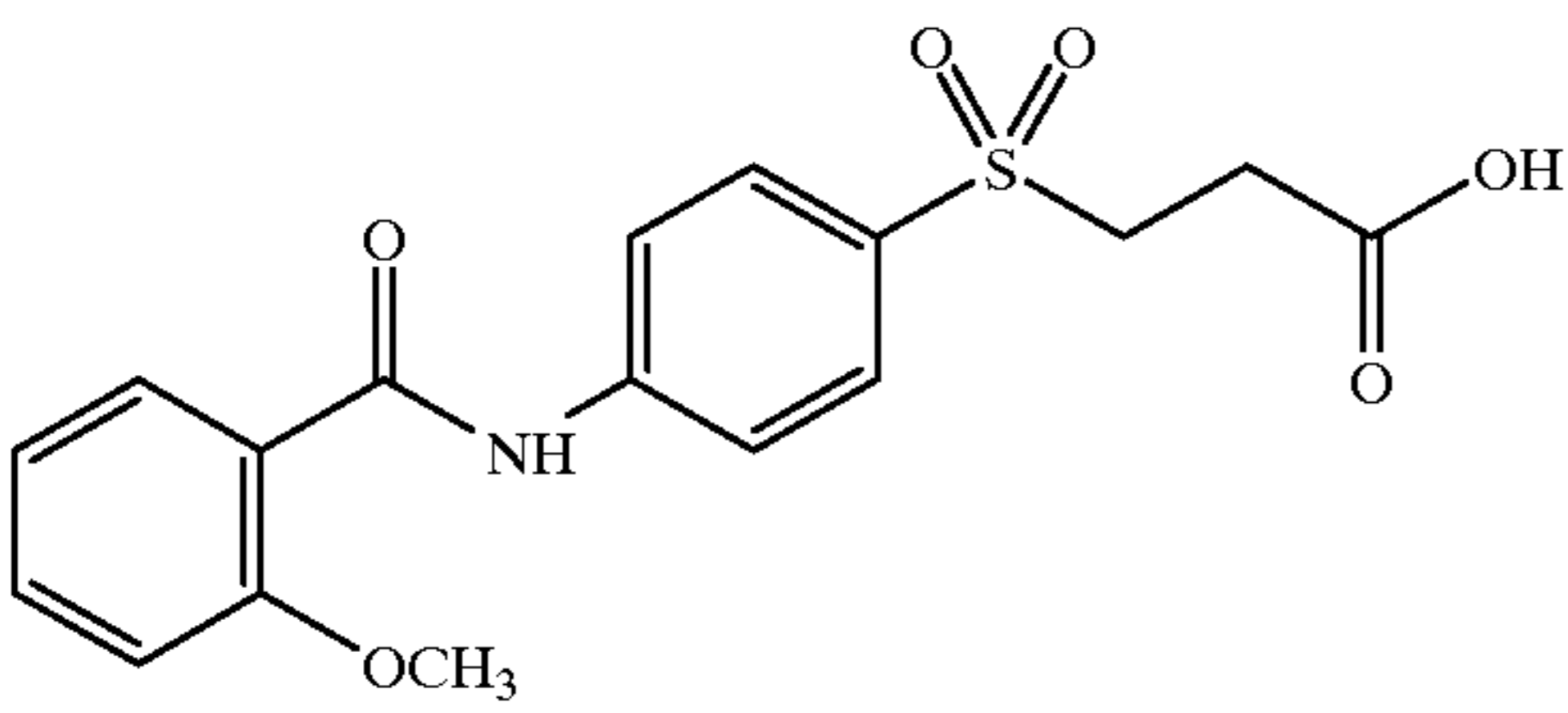
4-(2-methoxybenzoyl)amino 3-carboxypropylsulfone
