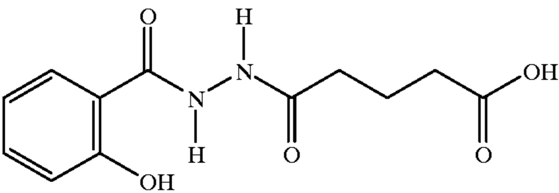
1-salicyloyl-2-glutaryl hydrazide
