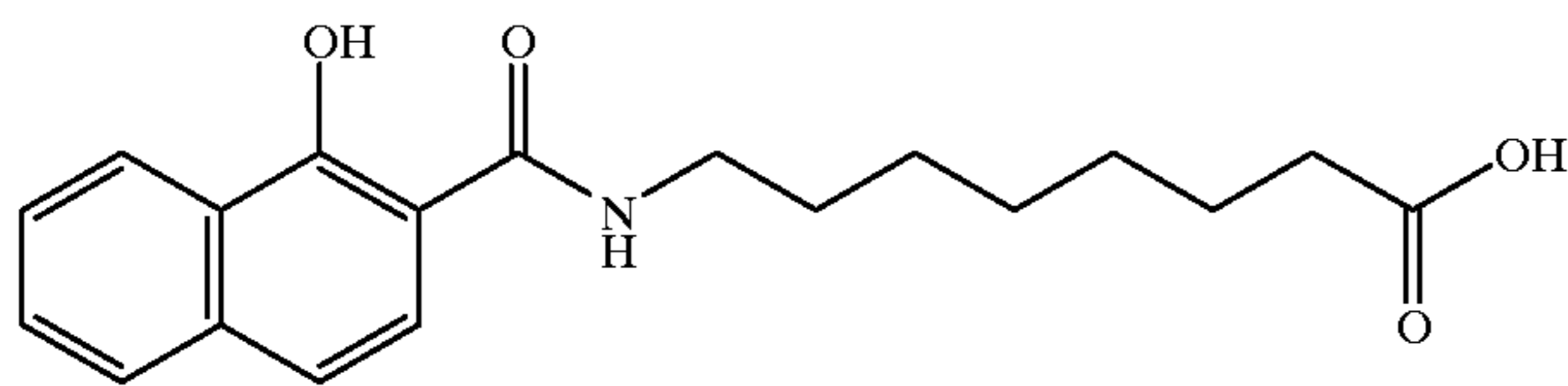
8-(N-1-hydroxy-2-naphthoyl)aminocaprylic acid
