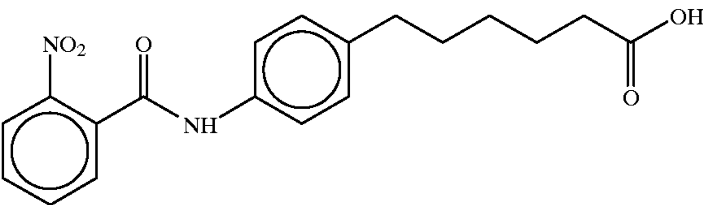
6-(4-(N-2-Nitrobenzoyl)aminophenyl)hexanoic acid
