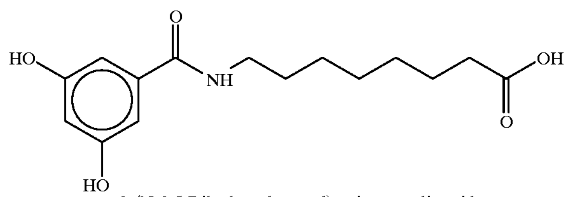
8-(N-3,5 Dihydroxybenzoyl)aminocaprylic acid
