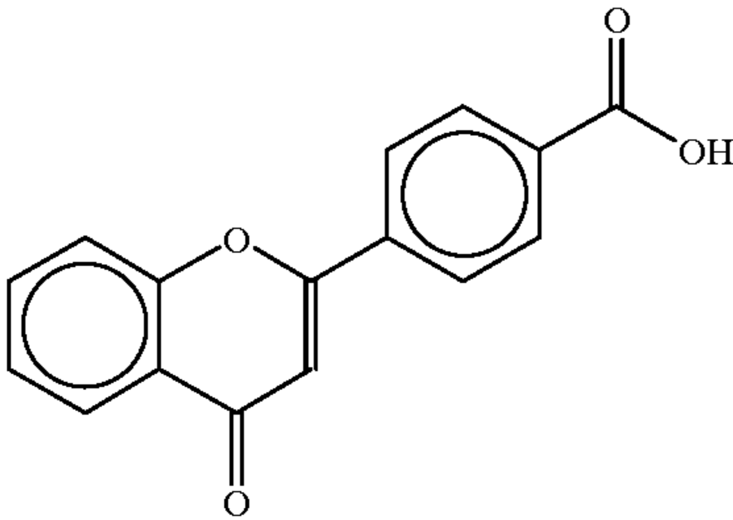
4'-flavonic acid
