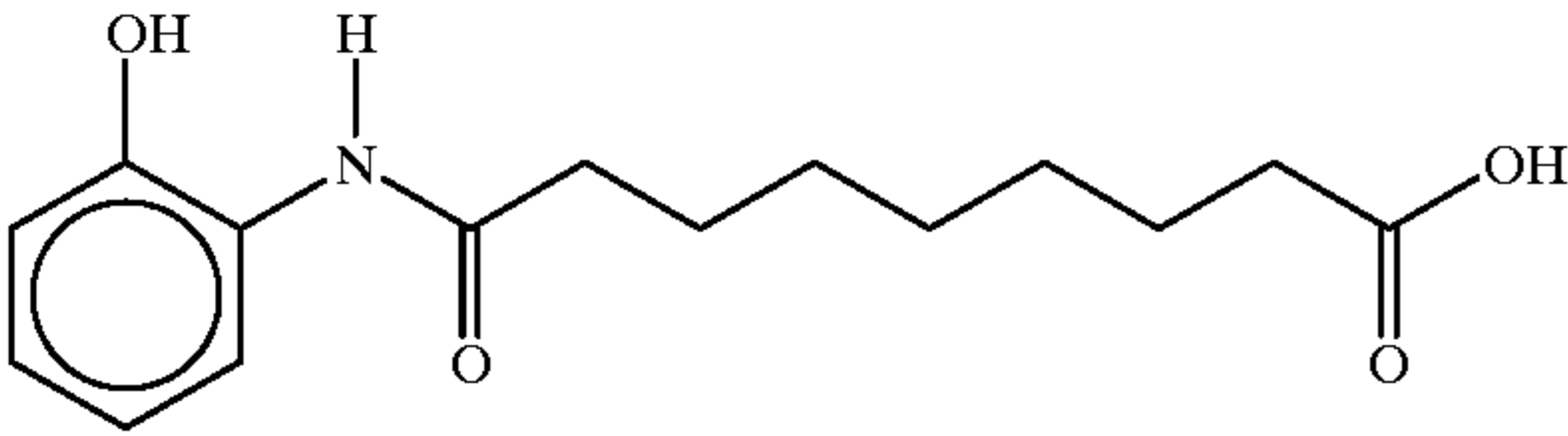
9-(2-hydroxybenzamido)nonanoic acid
