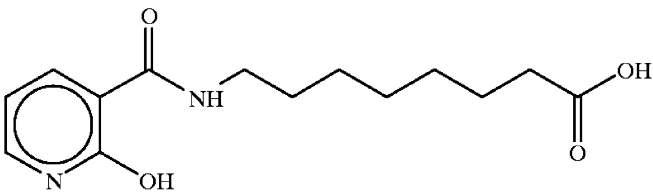
8-(2-Hydroxynicotinoyl)aminocaprylic acid
