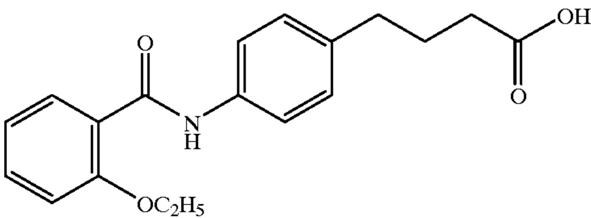
4-(4-(2-ethoxybenzoyl)aminophenyl)butyric acid
