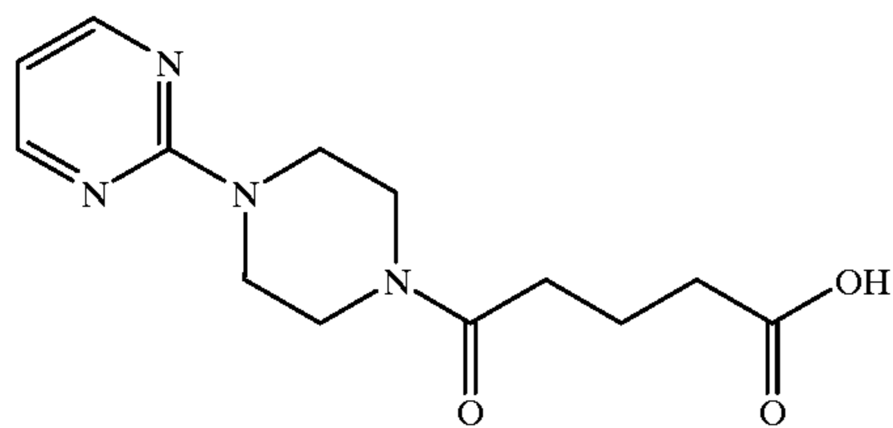
4-(1-(2-pyrimidyl)piperazinoyl)butyric acid
