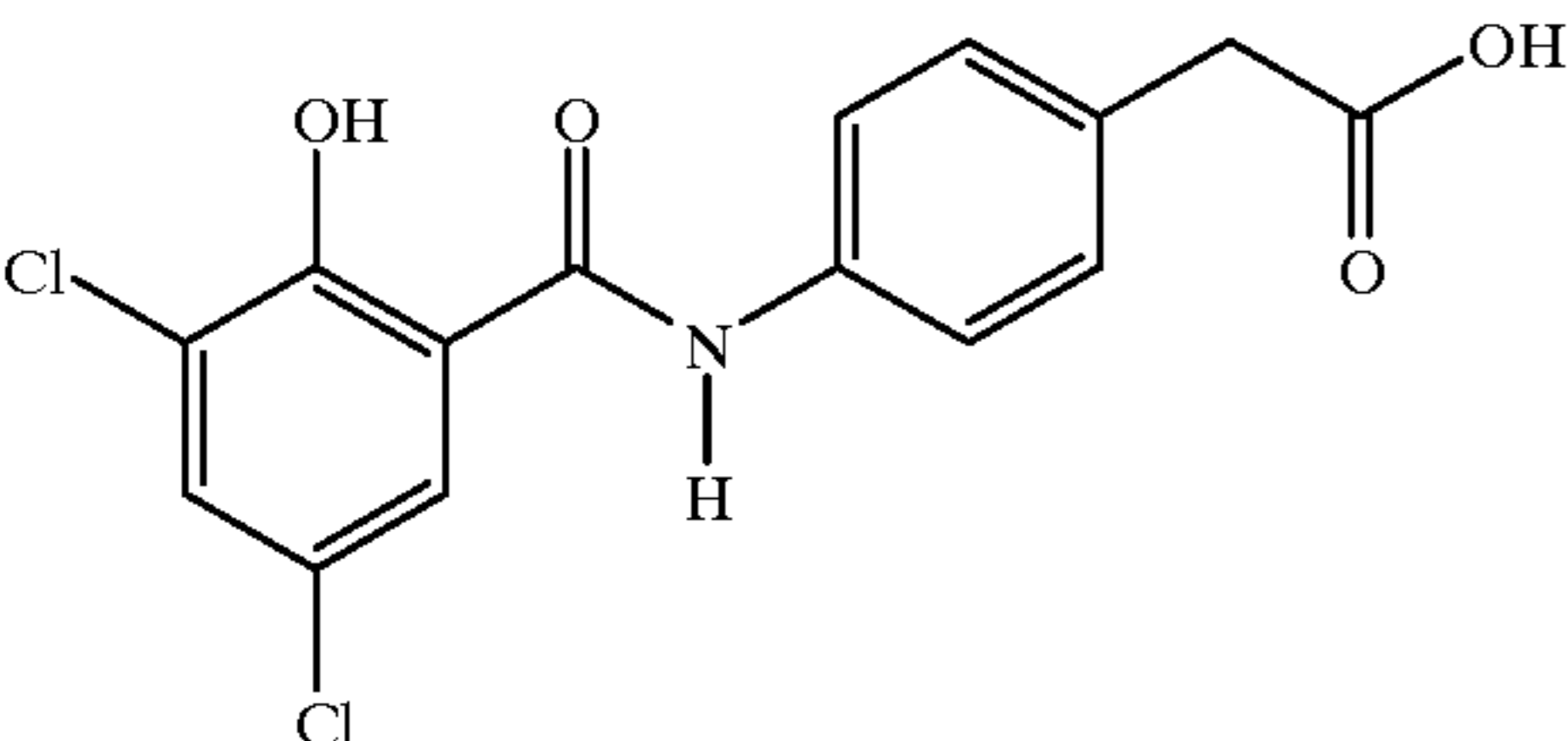
4-[N-(3,5-dichloro-2-hydroxybenzoyl)]aminophenylacetic acid
