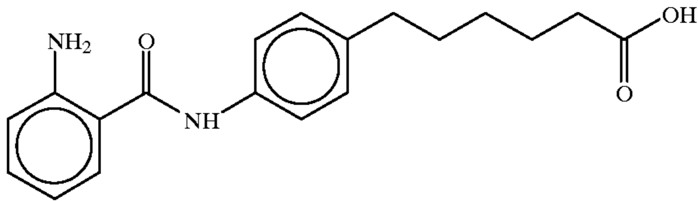
6-(4-(N-2-aminobenzoyl)aminophenyl)hexanoic acid
