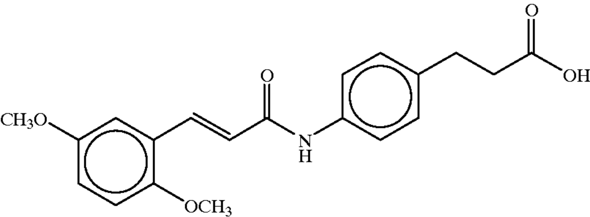
3-(4-(2,5-dimethoxycinnamoyl)aminophenyl)propionic acid
