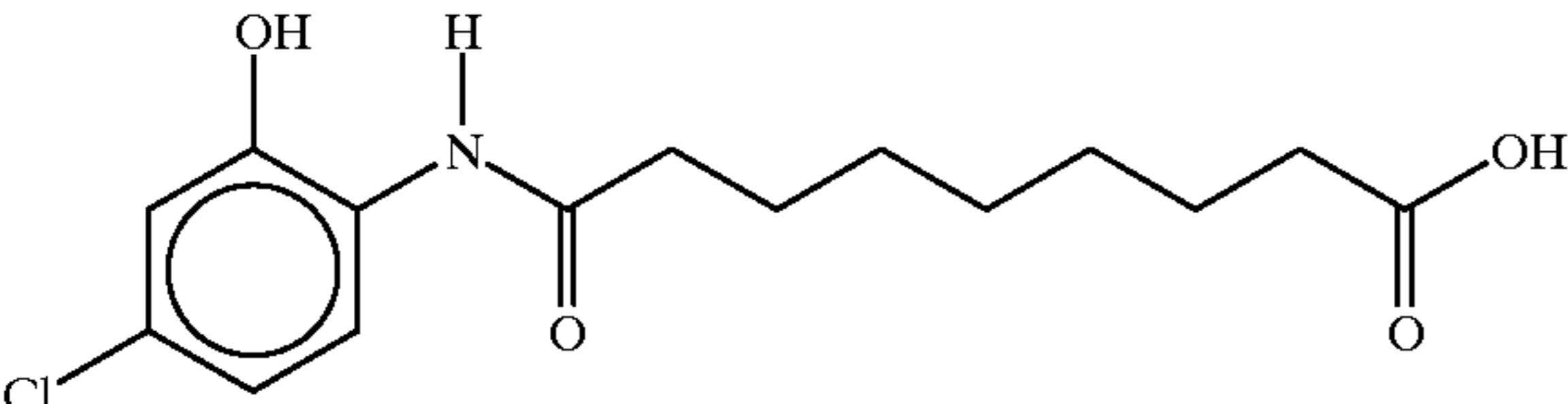
8-(2-hydroxy-5-chloroanilincarbonyl)octanoic acid
