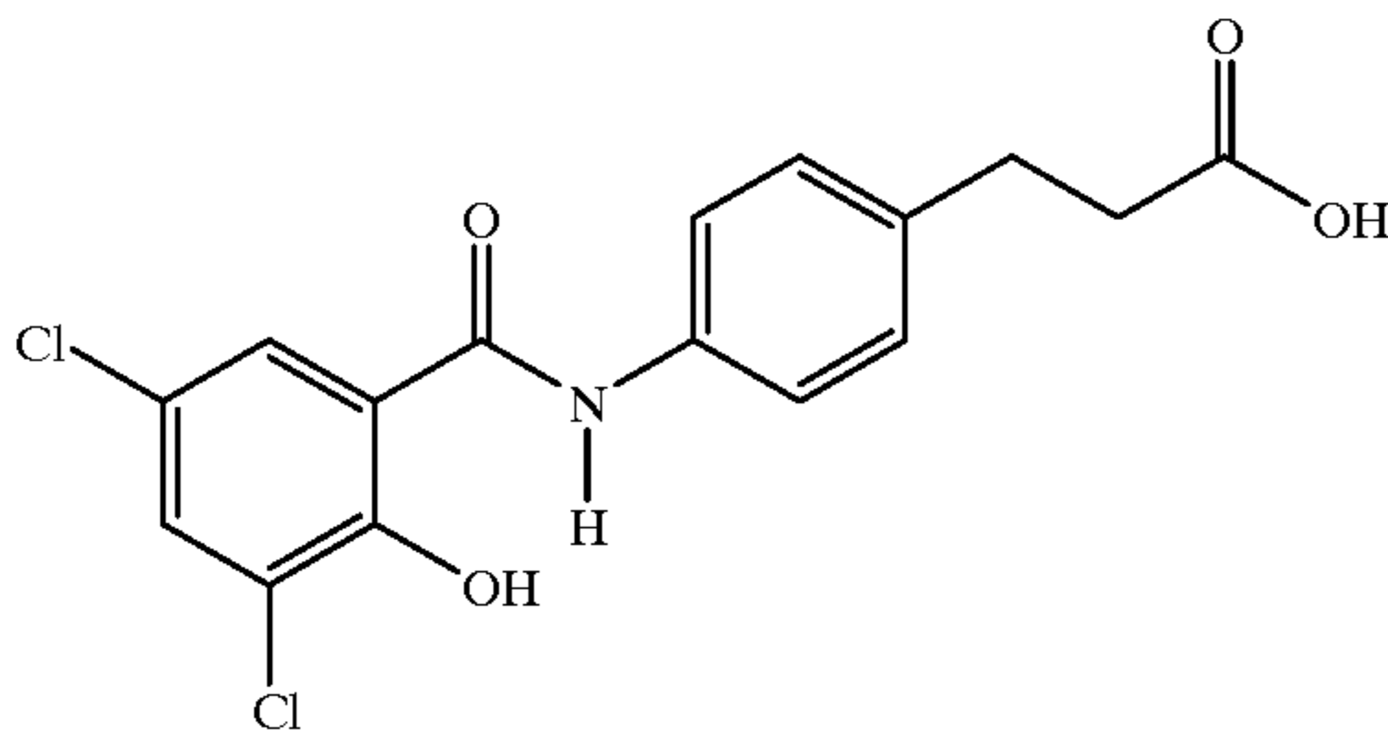
N-[3,5-dichloro-2-hydroxybenzoyl-3-(4-aminophenyl)]propionic acid
