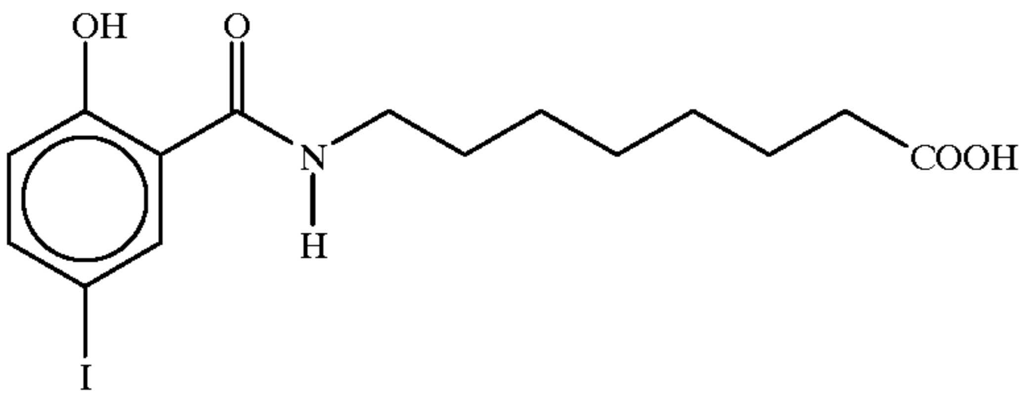
8-(N-2-hydroxy-5-iodobenzoyl)aminocaprylic acid
