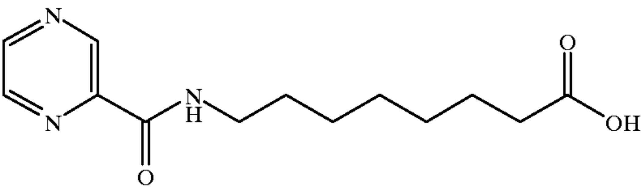
8-(2-pyrazinecarbonyl)aminocaprylic acid
