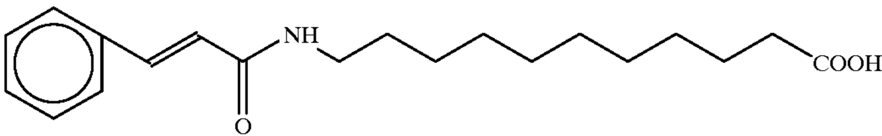
11-cinnamoylaminooundecanoic acid
