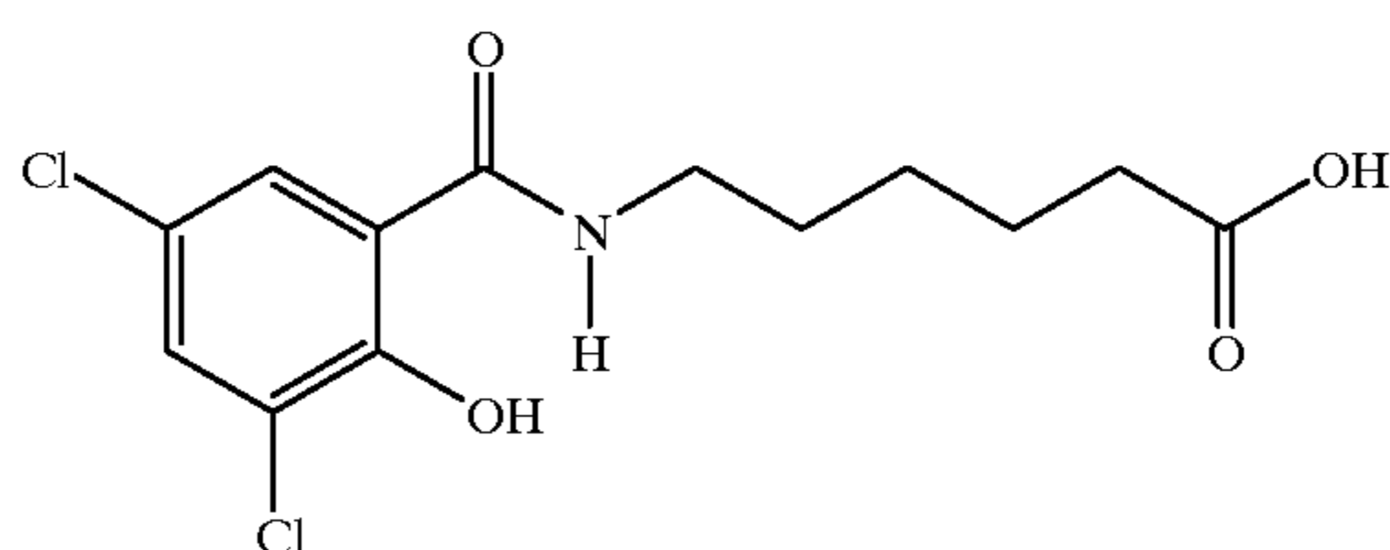
6-N-(3,5-dichloro-2-hydroxybenzoyl)aminocaproic acid
