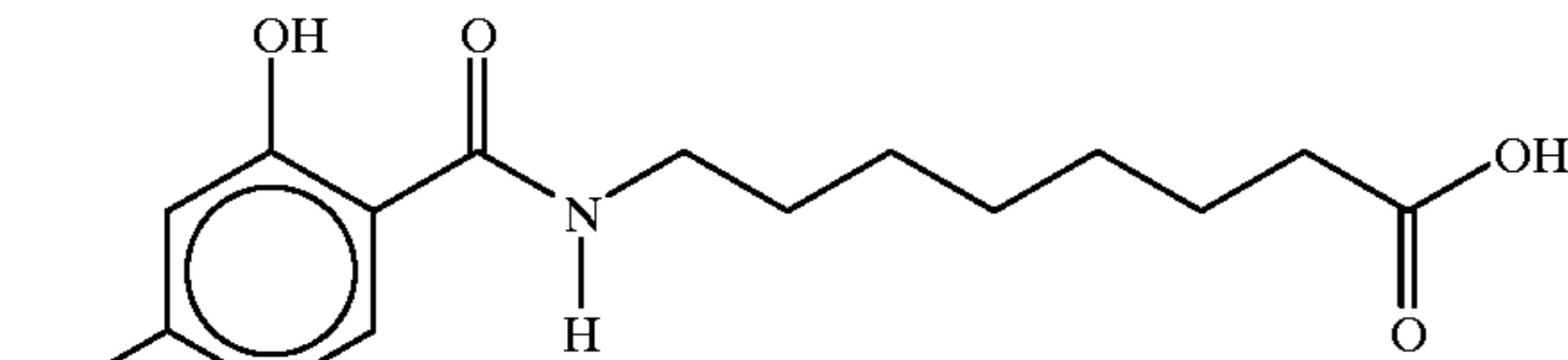
8-(N,4-Dihydroxybenzoyl)aminocaprylic acid
