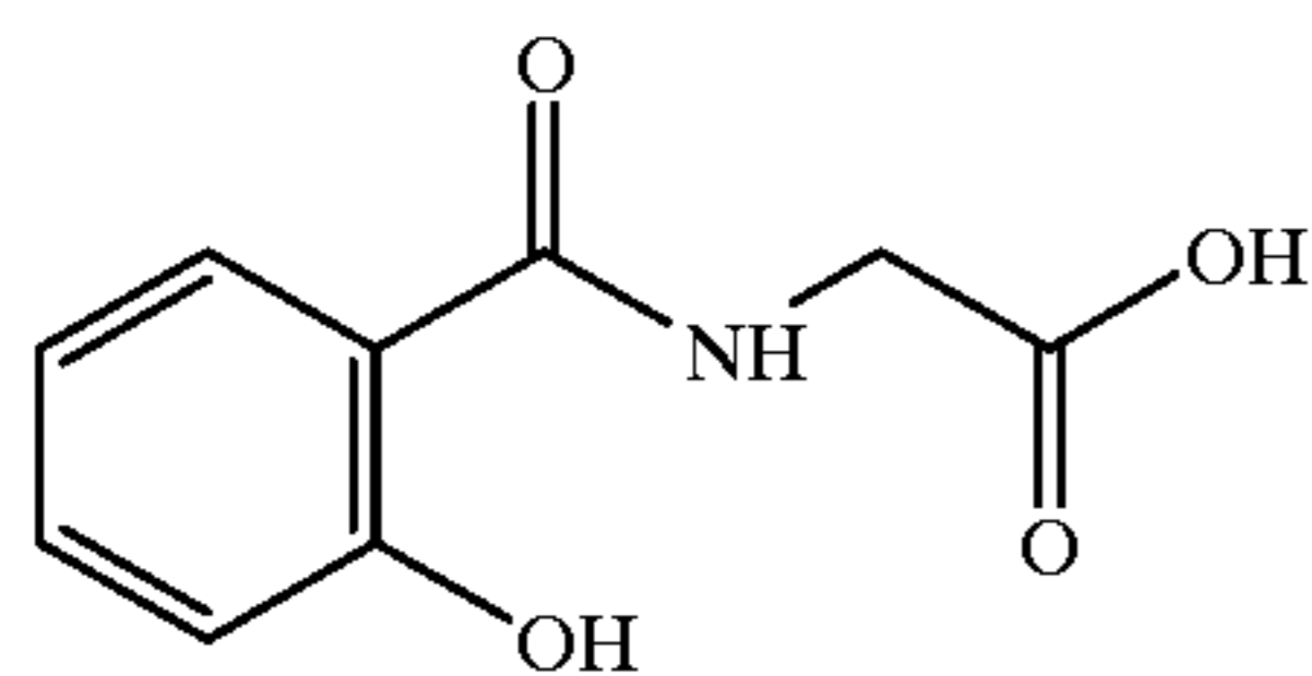
salicyloylglycine
