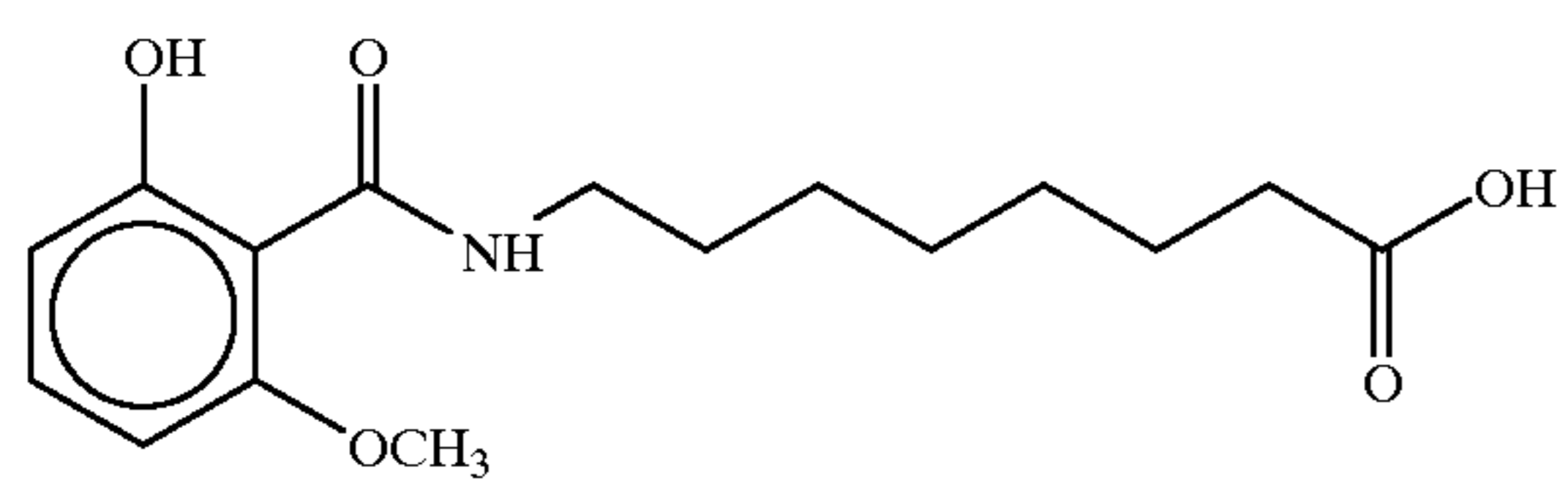
8-(N-2-Hydroxy-6-methoxybenzoyl)aminocaprylic acid
