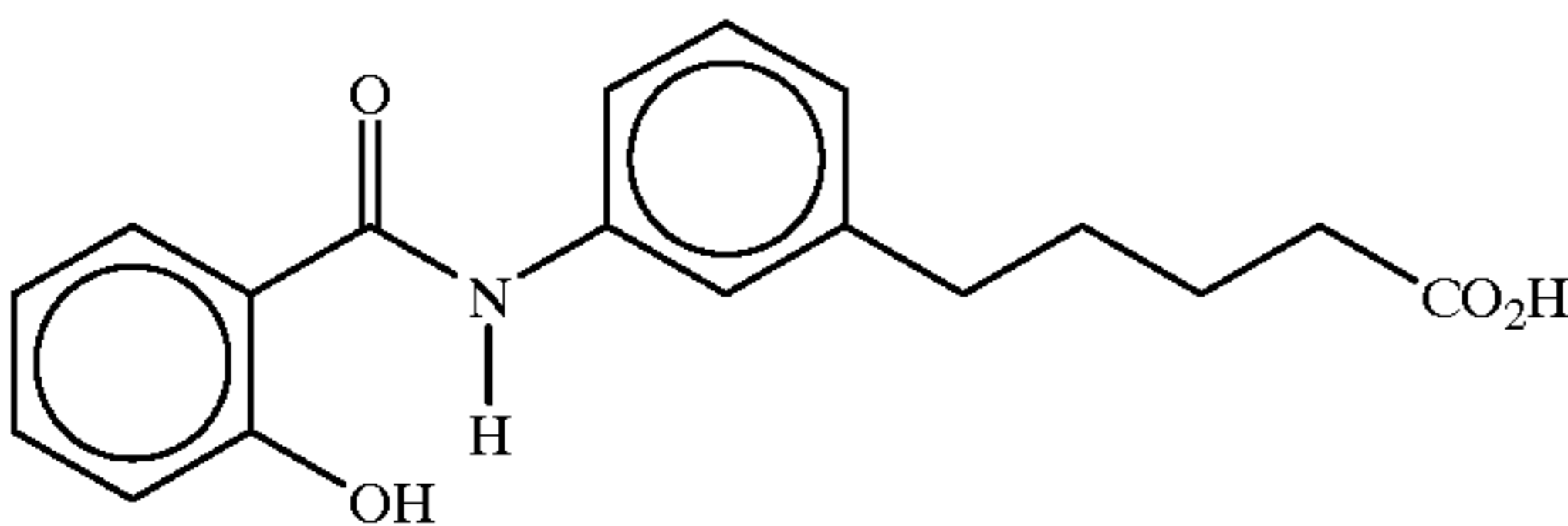
N-Salicyloyl-5-(3-aminophenyl)valeric acid
