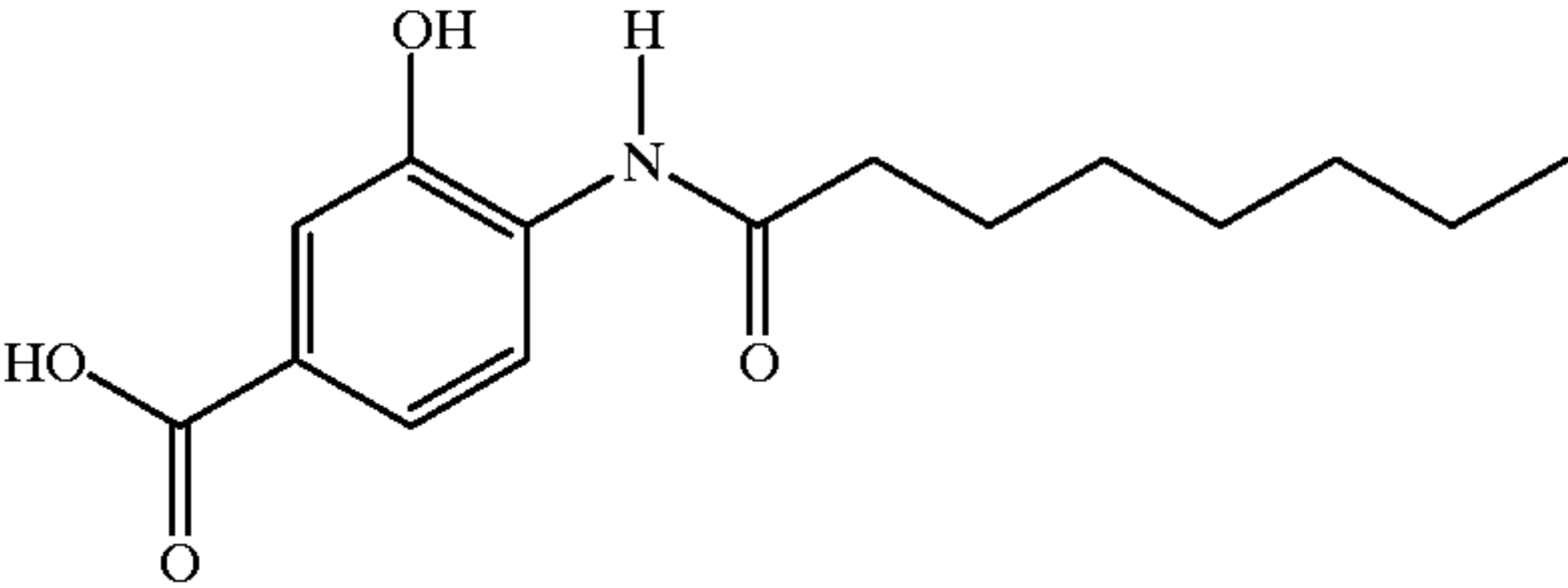
4-octanoylamino-3-hydroxybenzoic acid
