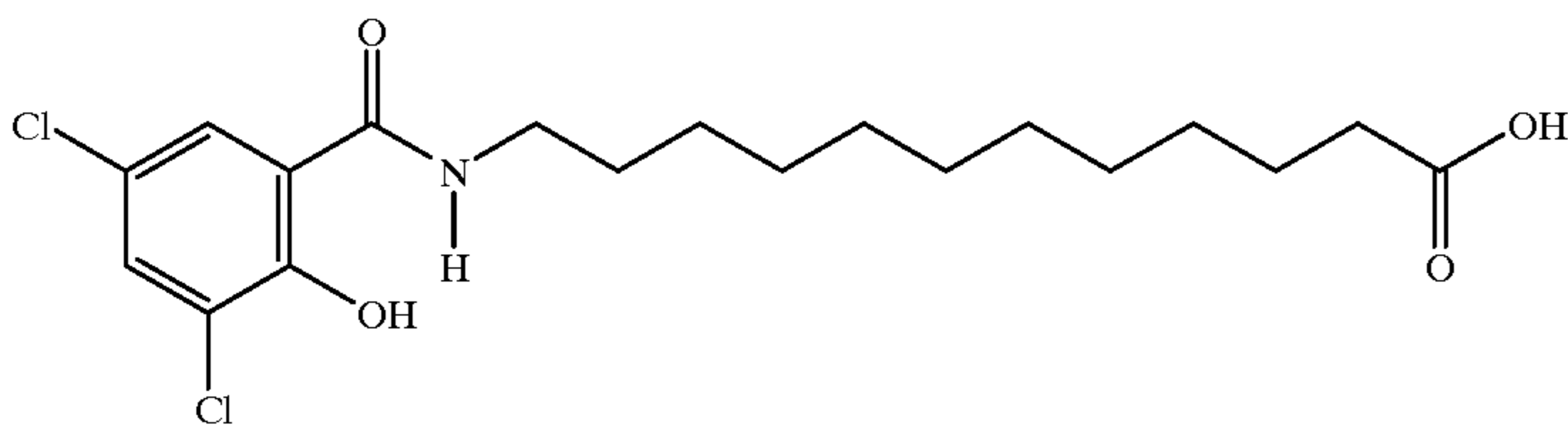
12-N-(3,5-dichloro-2-hydroxybenzoyl)aminododecanoic acid
