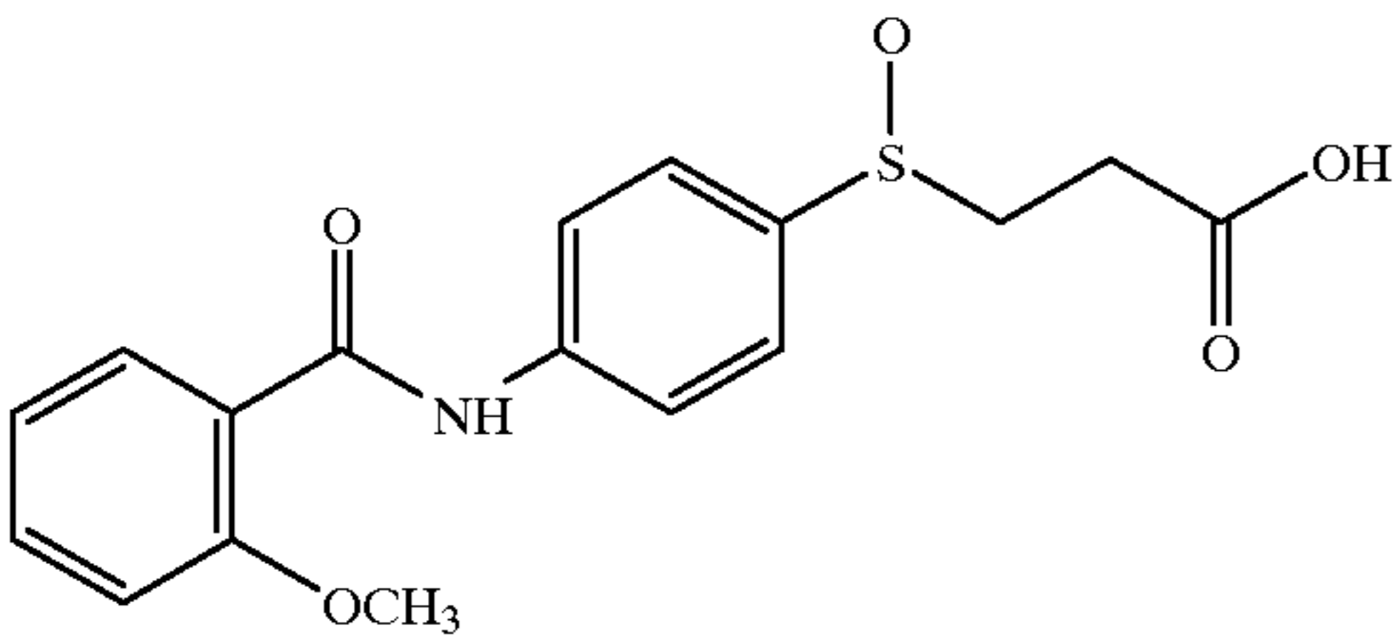
4-(2-methoxybenzoyl)amino 3-carboxysulfoxide
