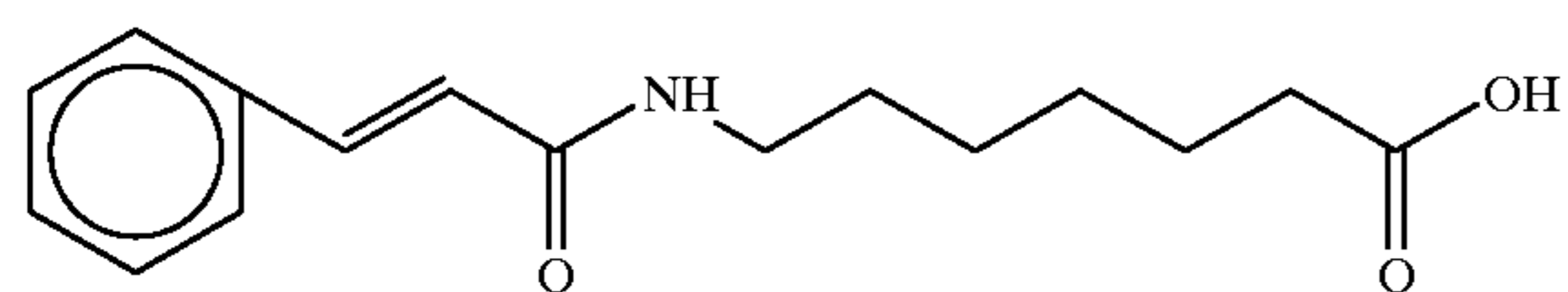
7-cinnamoylaminoheptanoic acid
