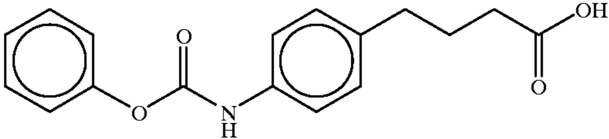
4-(4-phenyloxycarbonylamino)phenylbutyric acid
