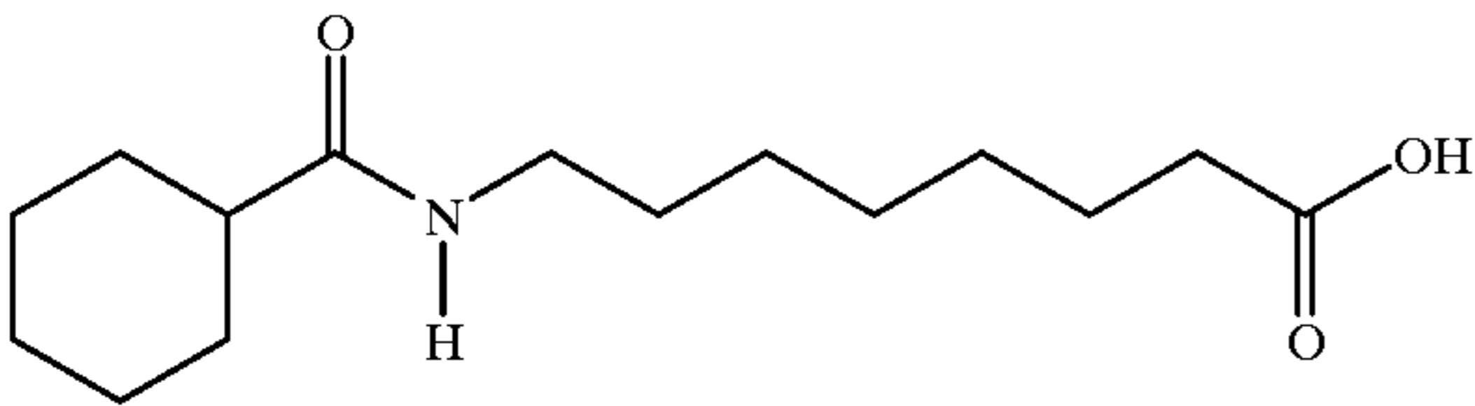
8-N-cyclohexanoylaminovaleric acid
