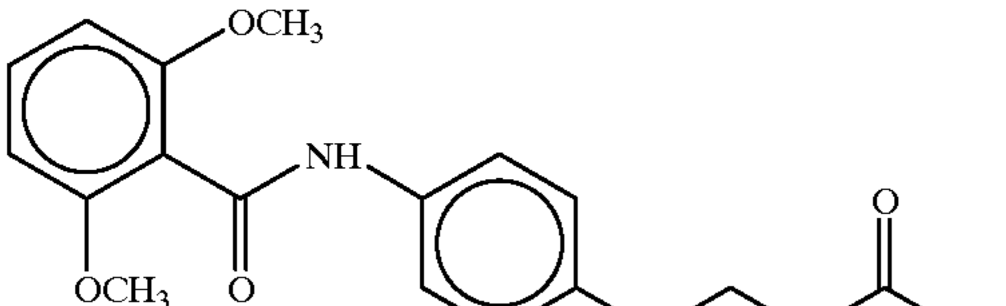
4-(4-(2,6-dimethoxybenzoyl)aminophenyl)butyric acid
