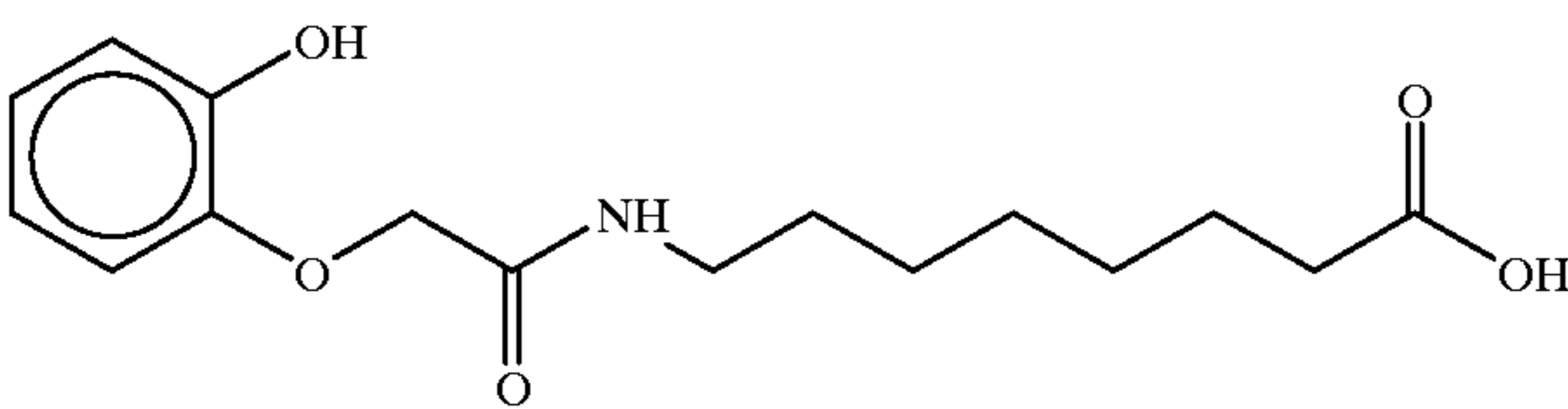
7-(2-hydroxyphenoxyacetyl)aminocaproic acid
