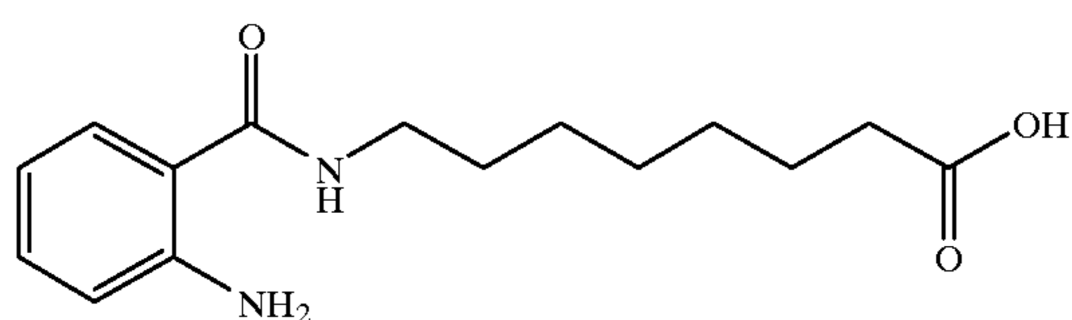
8(2-aminobenzoylamino)caprylic acid
