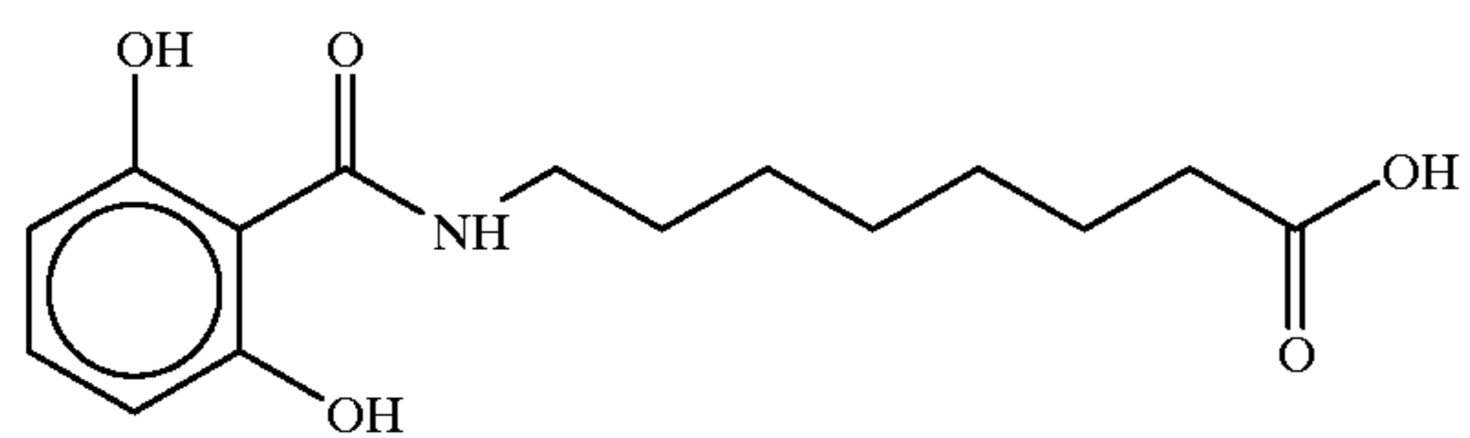
8-(N-2,6-Dihydroxybenzoyl)aminocaprylic acid
