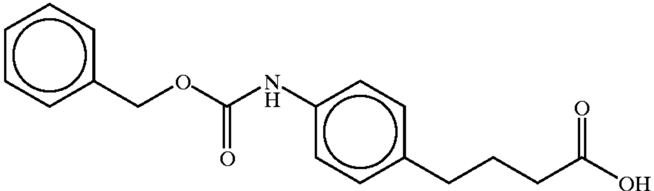
4-(4-benzyloxycarbonylamino)phenylbutyric acid
