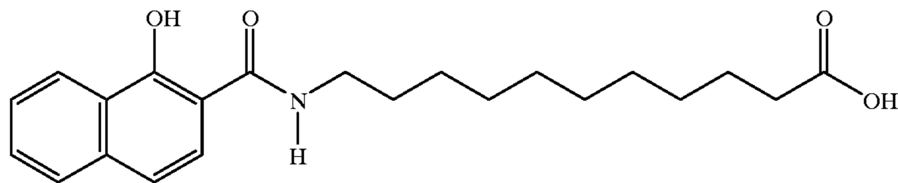
11-N-(1-hydroxy-2-naphthoyl)aminoundecanoic acid
