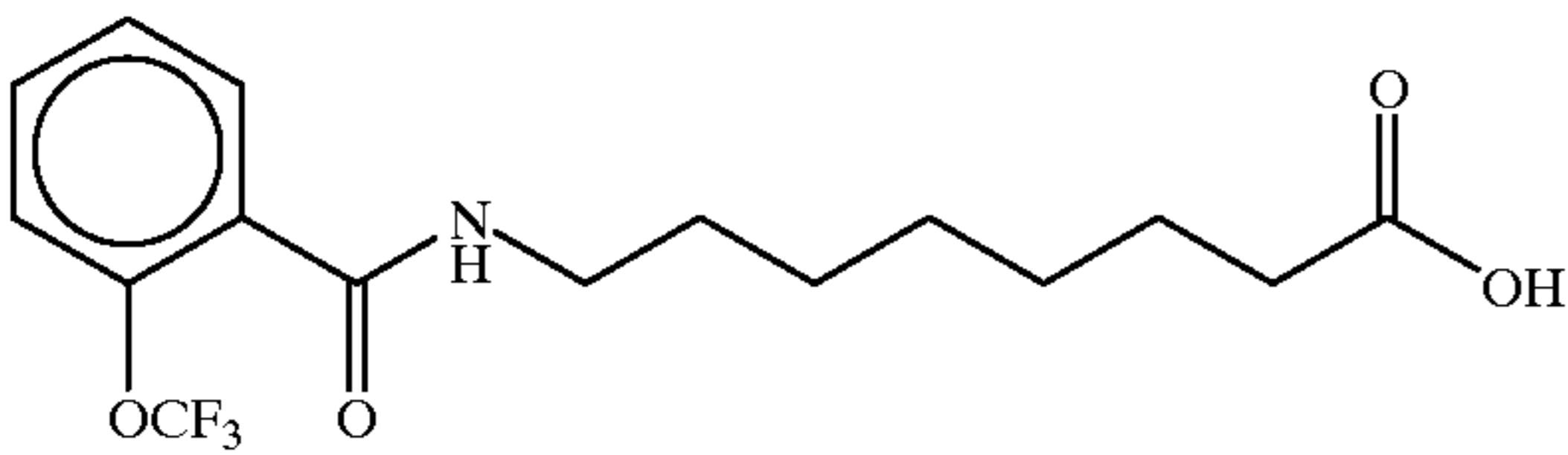
8-(2-(trifluoromethoxy)benzoyl)aminocaprylic acid
