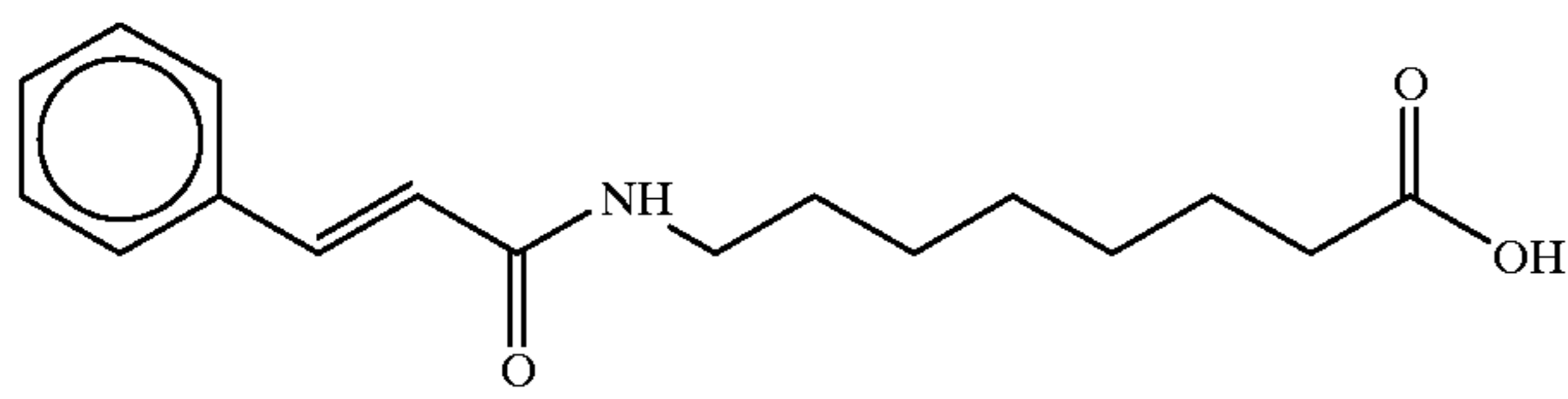
8-cinnamoylaminocaprylic acid
