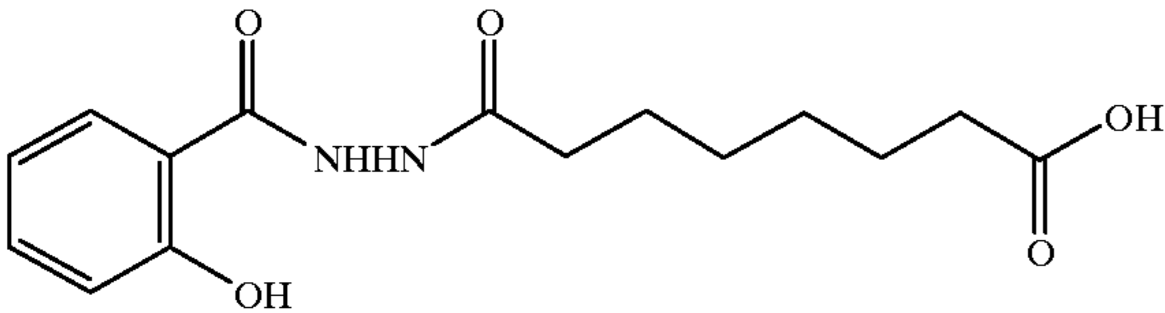
1-salicyloyl-2-suberyl hydrazide
