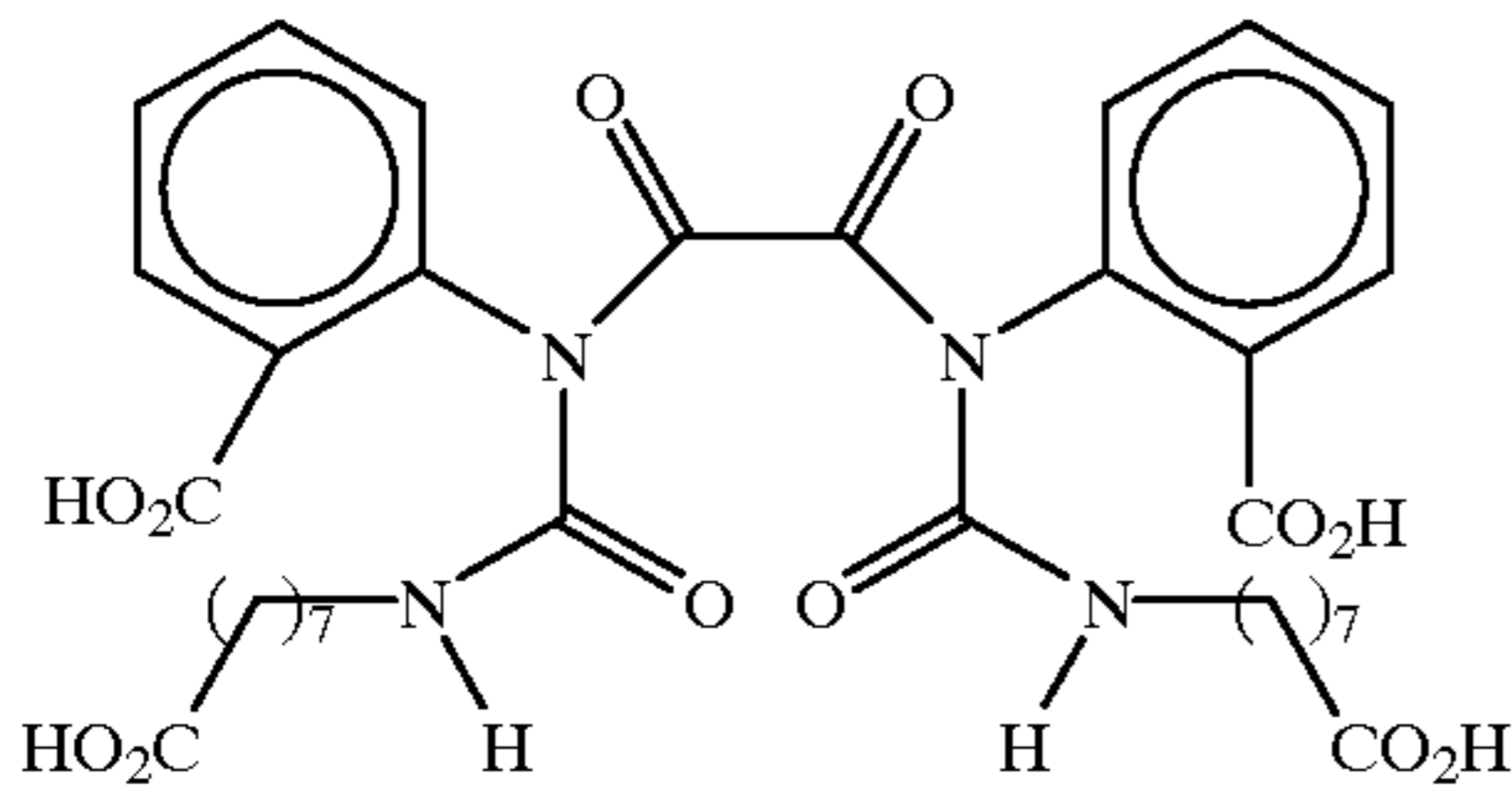
Bis(N-2carboxylphenyl-N-(N'-8-octanoic acid)ureal)oxalyl diamide
