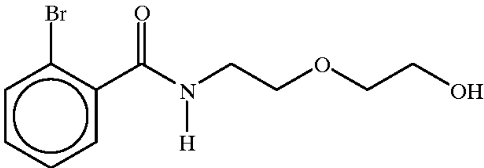
2-[N-(2-bromobenzoyl)aminoethoxy]ethanol
