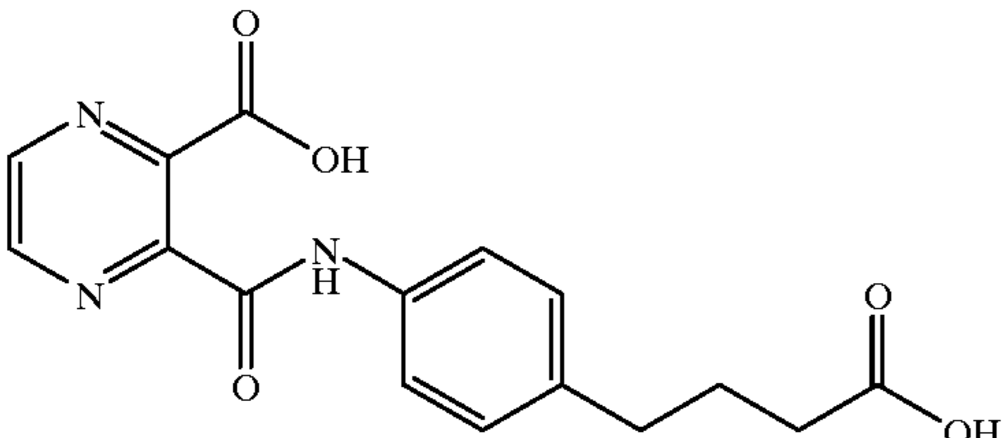
4-(4-(2-(3-carboxyl)pyrazinecarboxyl)aminophenyl)butyric acid
