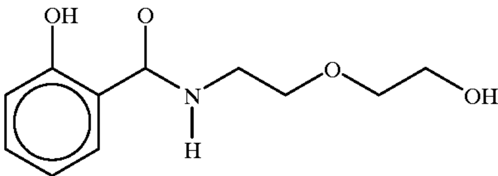
2-[N-(2-hydroxybenzoylamino)ethoxy]ethanol
