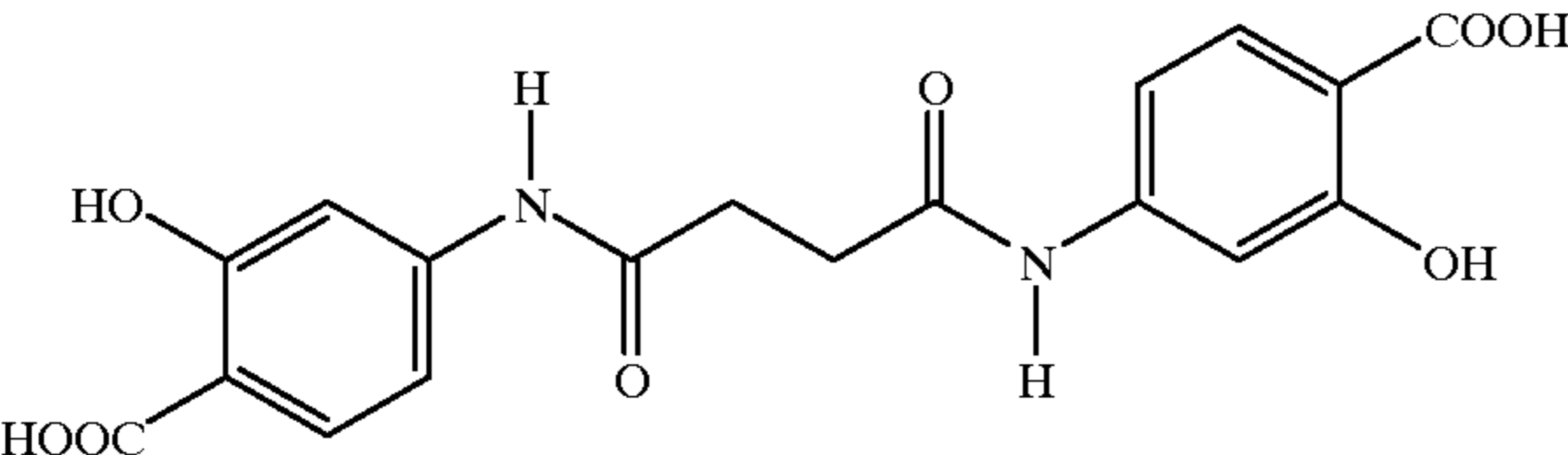
Succinyl-4-aminosalicylic acid
