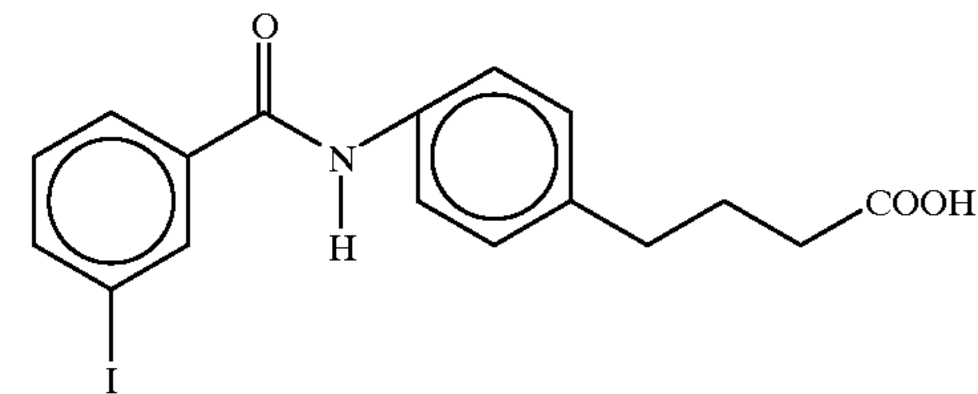
4-[N-[4-(3-iodobenzoyl)aminophenyl]]butyric acid
