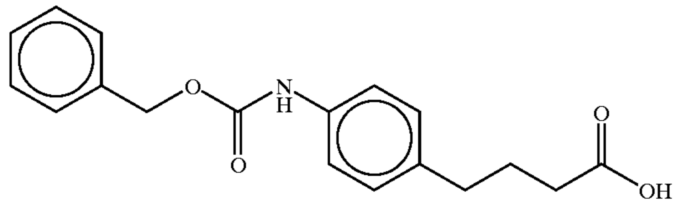
4-(4-benzyloxycarbonylamino)phenylbutyric acid
