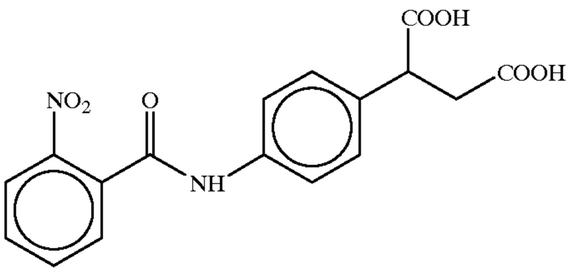
4-(2-Nitrobenzoyl)aminophenylsuccinic acid
