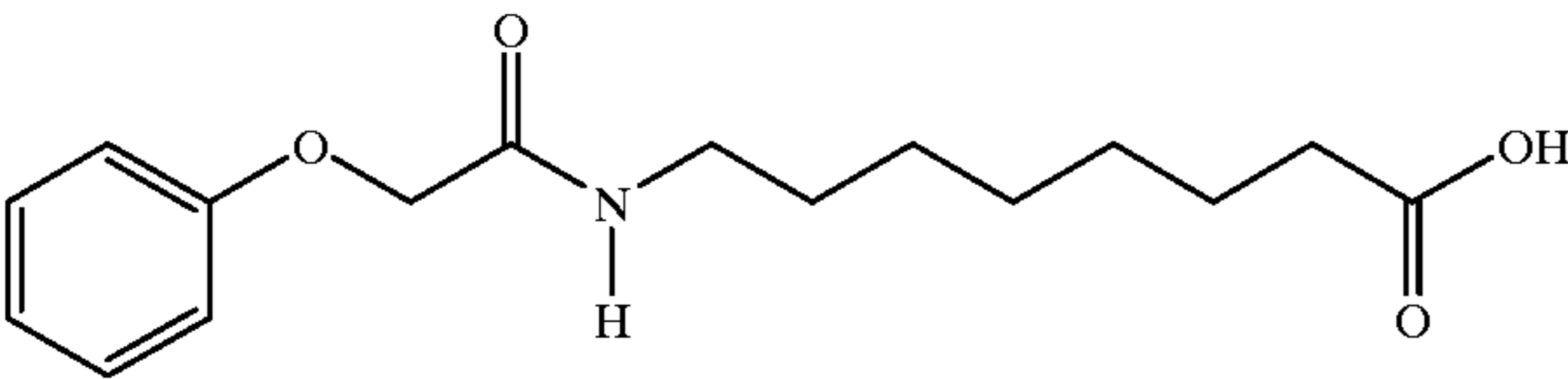
8-(Phenoxyacetyl)aminocaprylic acid
