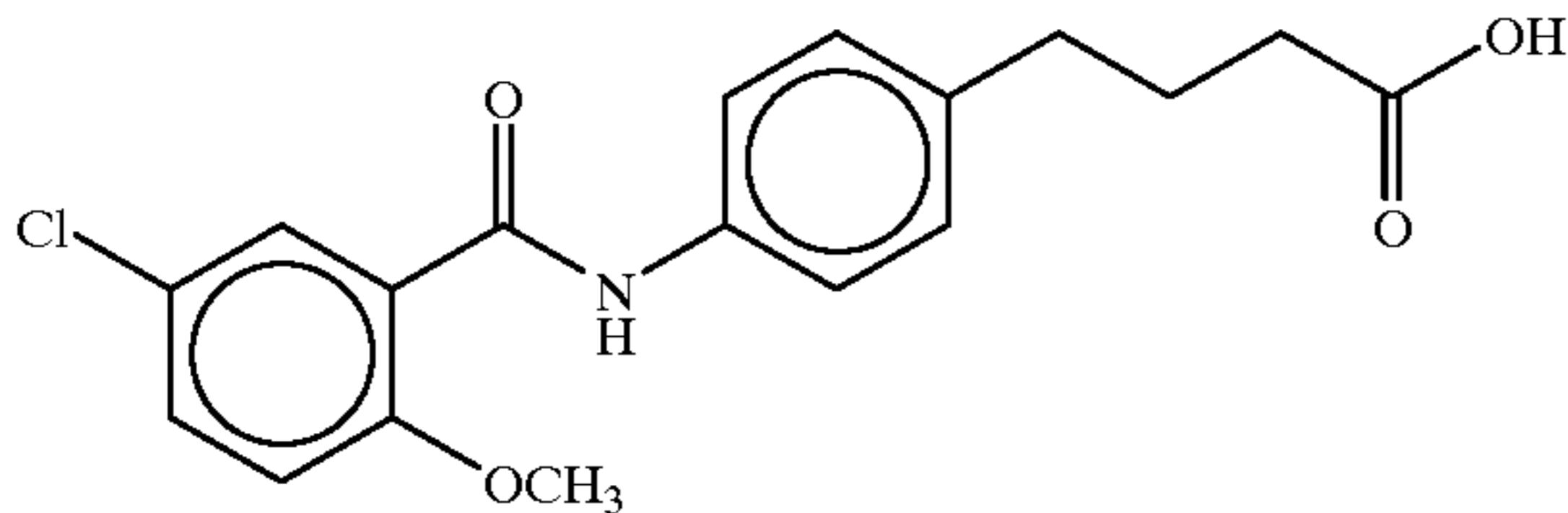
4-(4-(5-chloro-o-anisoyl)aminophenyl)butyric acid
