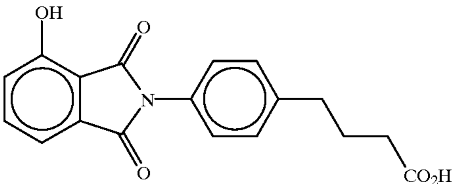
4-(4-(3-hydroxyphthalimido)phenyl)butyric acid
