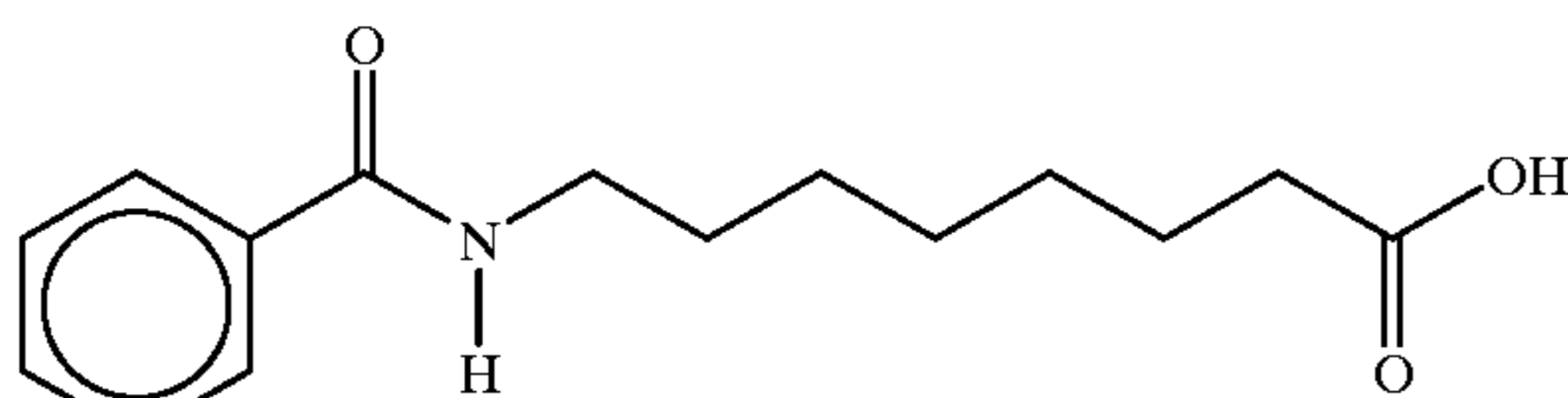
8-(N-benzoyl)aminocaprylic acid
