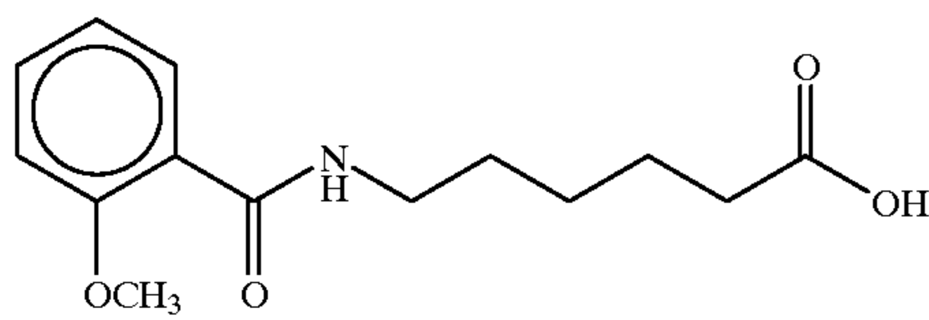
6-(anisoyl)aminocaproic acid
