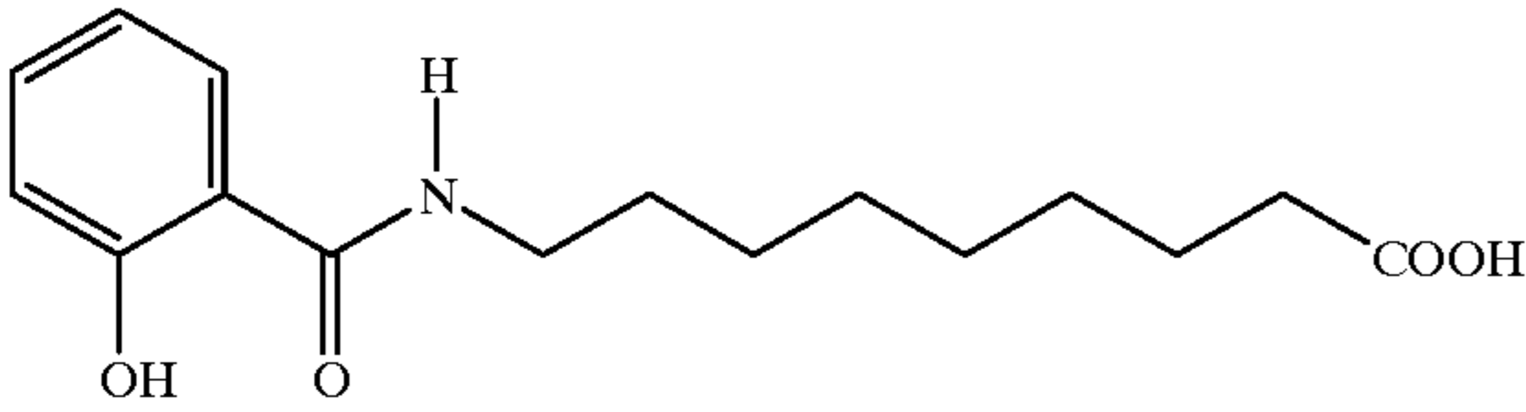
9-Salicyloylaminononanoic acid
