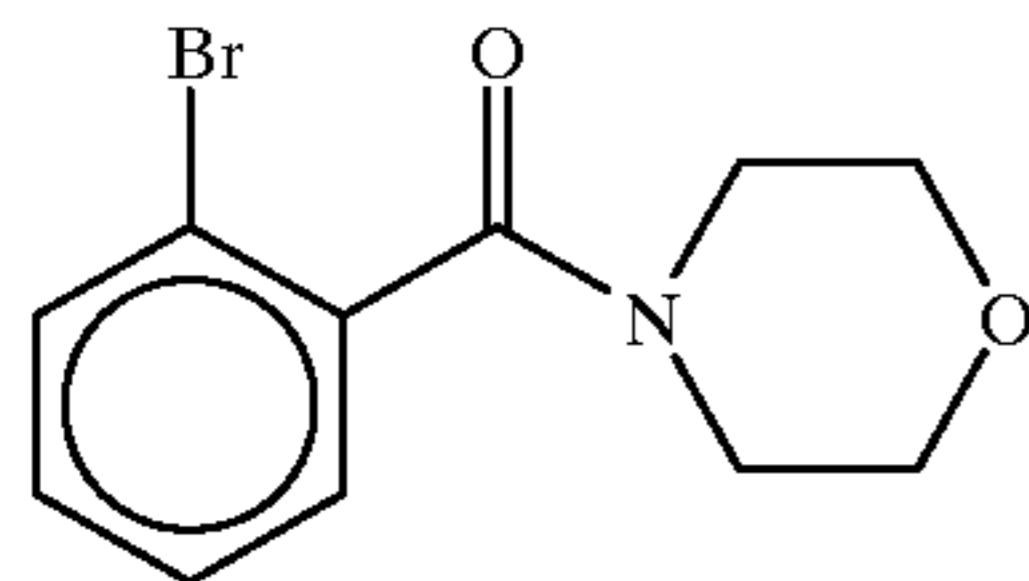
N-(2-bromobenzoyl)morpholine
