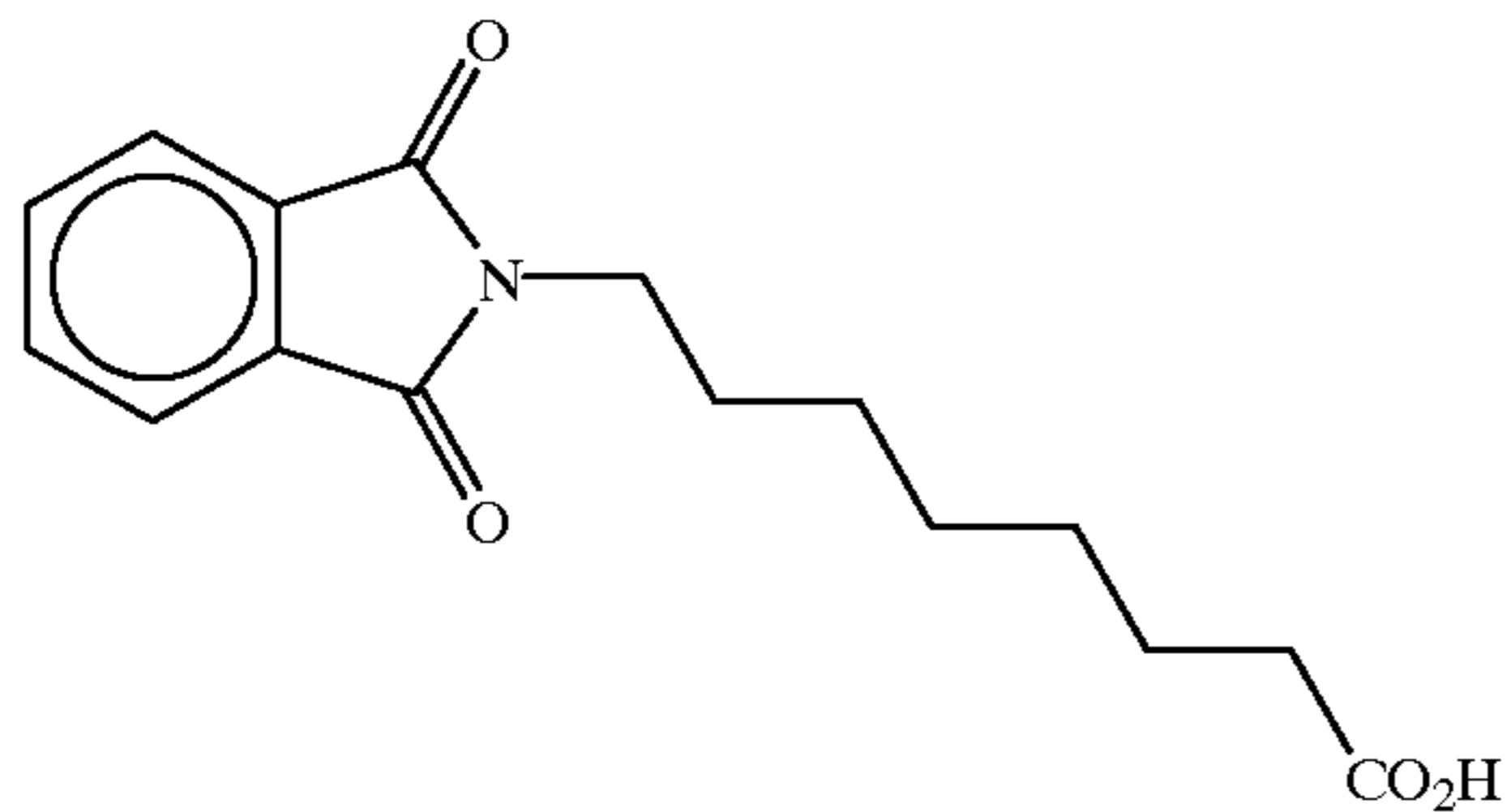
8-(phthalimido)caprylic acid
