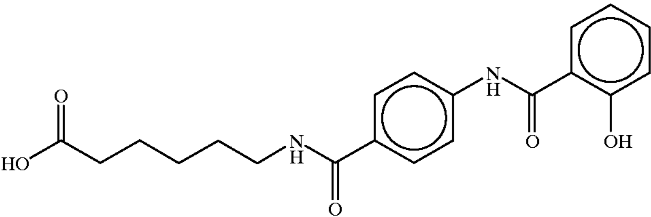
N-(4-salicyloylamino)-6-caproic acid
