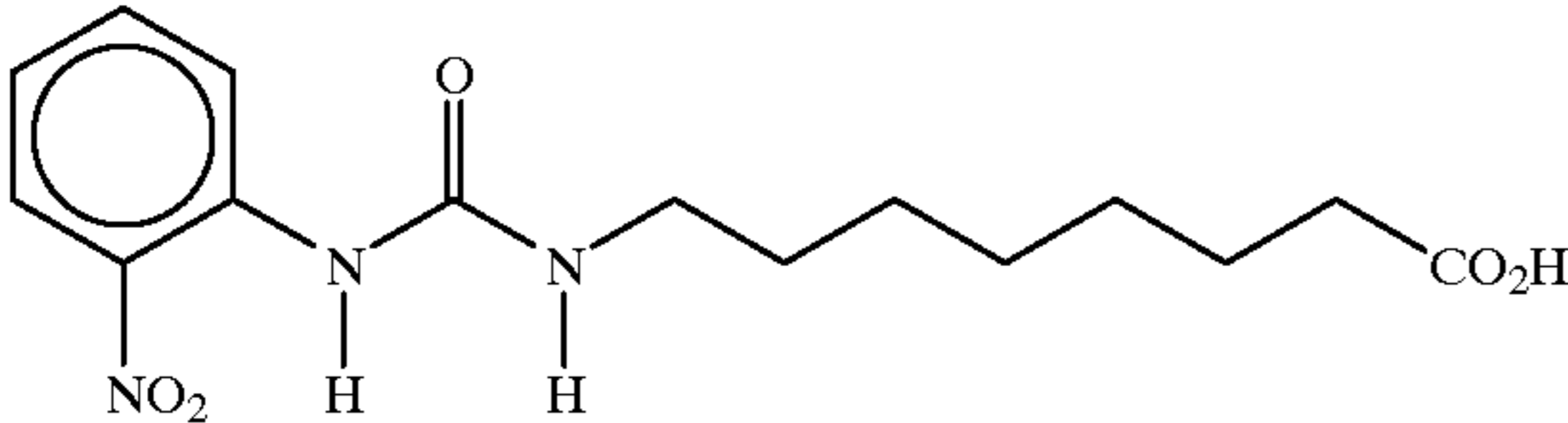
N-2-nitrophenyl-N'-(8-octanoic acid) urea
