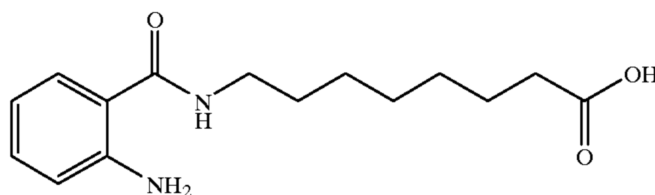
8(2-aminobenzoylamino)caprylic acid
