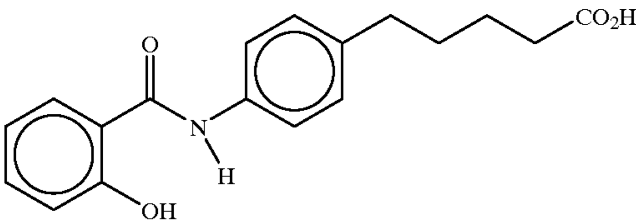
N-salicyl-5-(4-aminophenyl)valeric acid
