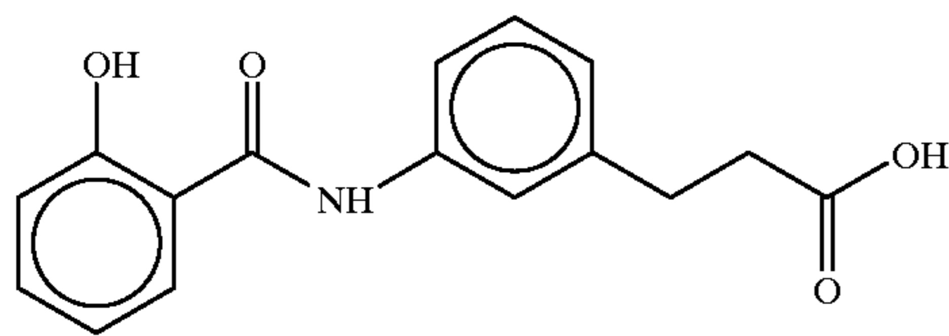
3-(3-(salicyloyl)aminophenyl)propionic acid
