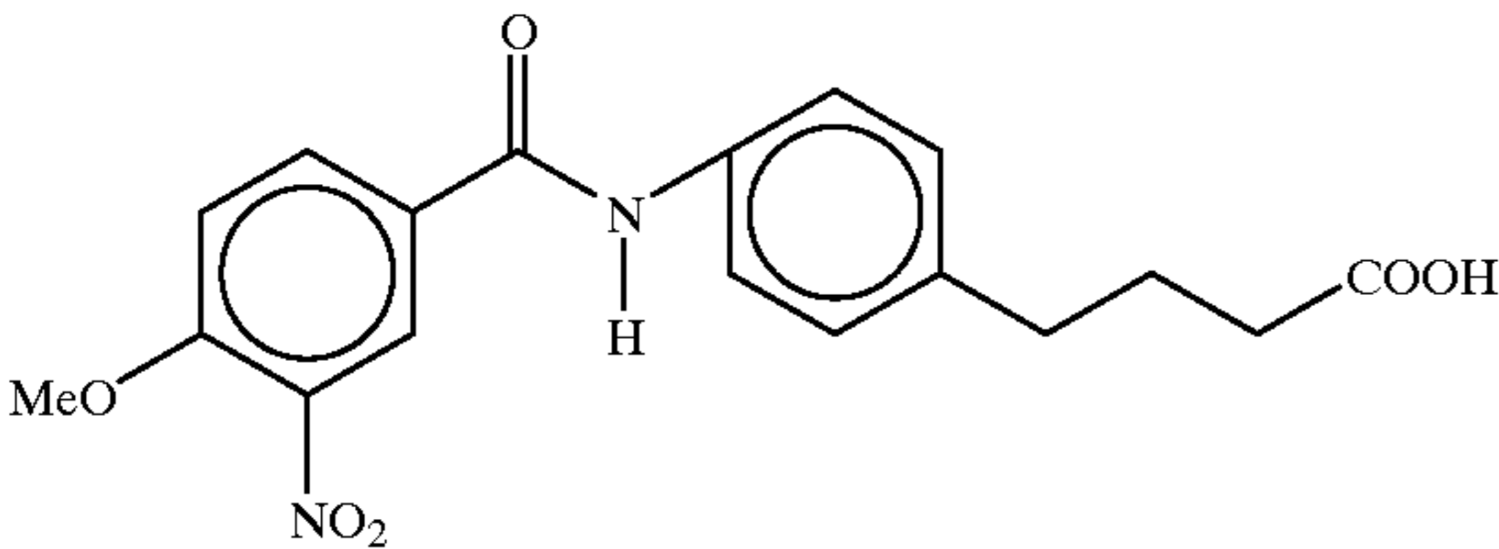
4-[4-N-(methoxy-3-nitrobenzoyl)aminophenyl]butyric acid
