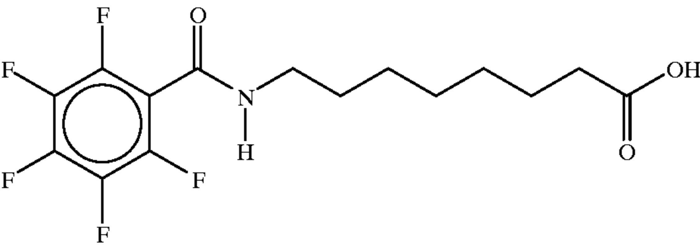
8-(pentafluorobenzoyl)aminocaprylic acid
