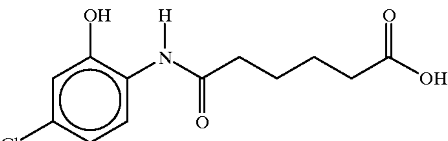
5-(4-chloro-2-hydroxyanilino)valeric acid
