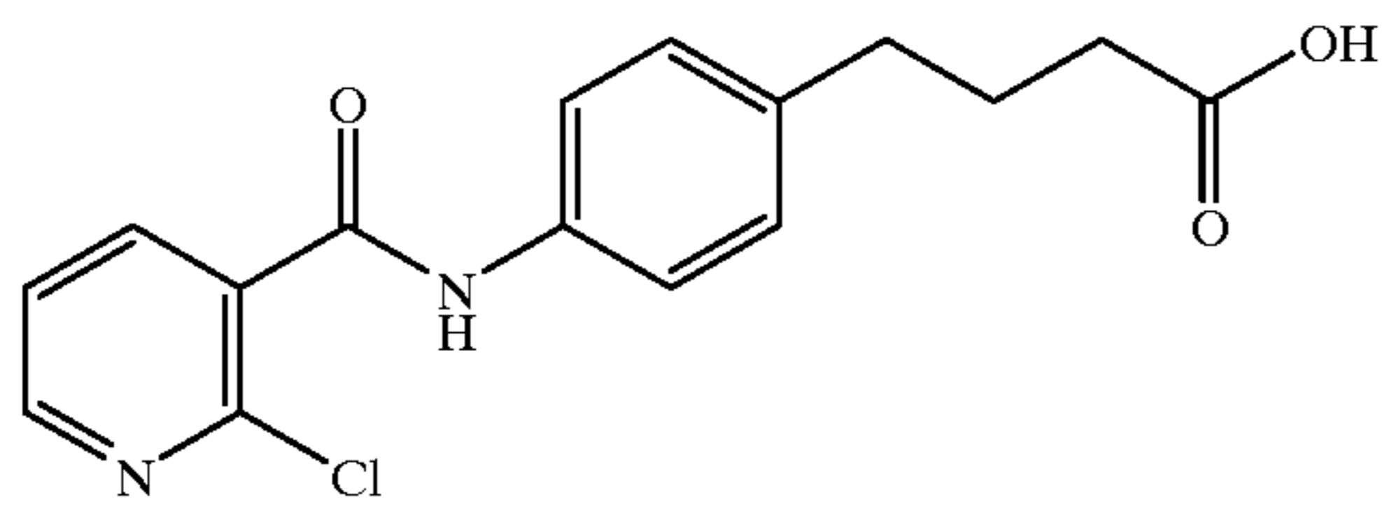
4-(4-(2-chloronicotinoyl)aminophenyl)butyric acid
