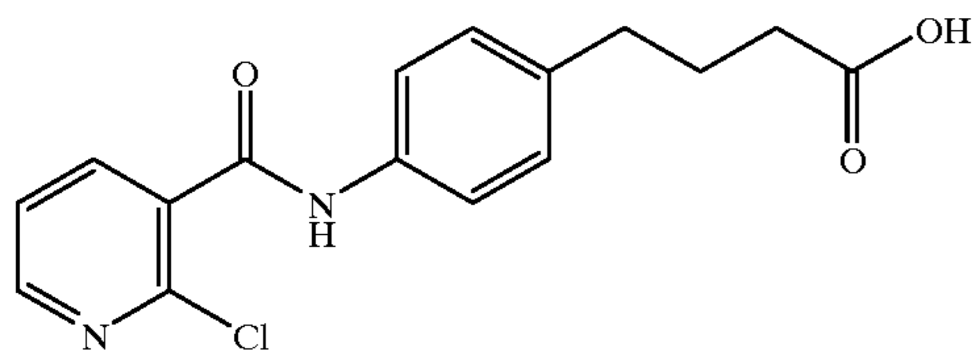
4-(4-(2-chloronicotinoyl)aminophenyl)butyric acid
