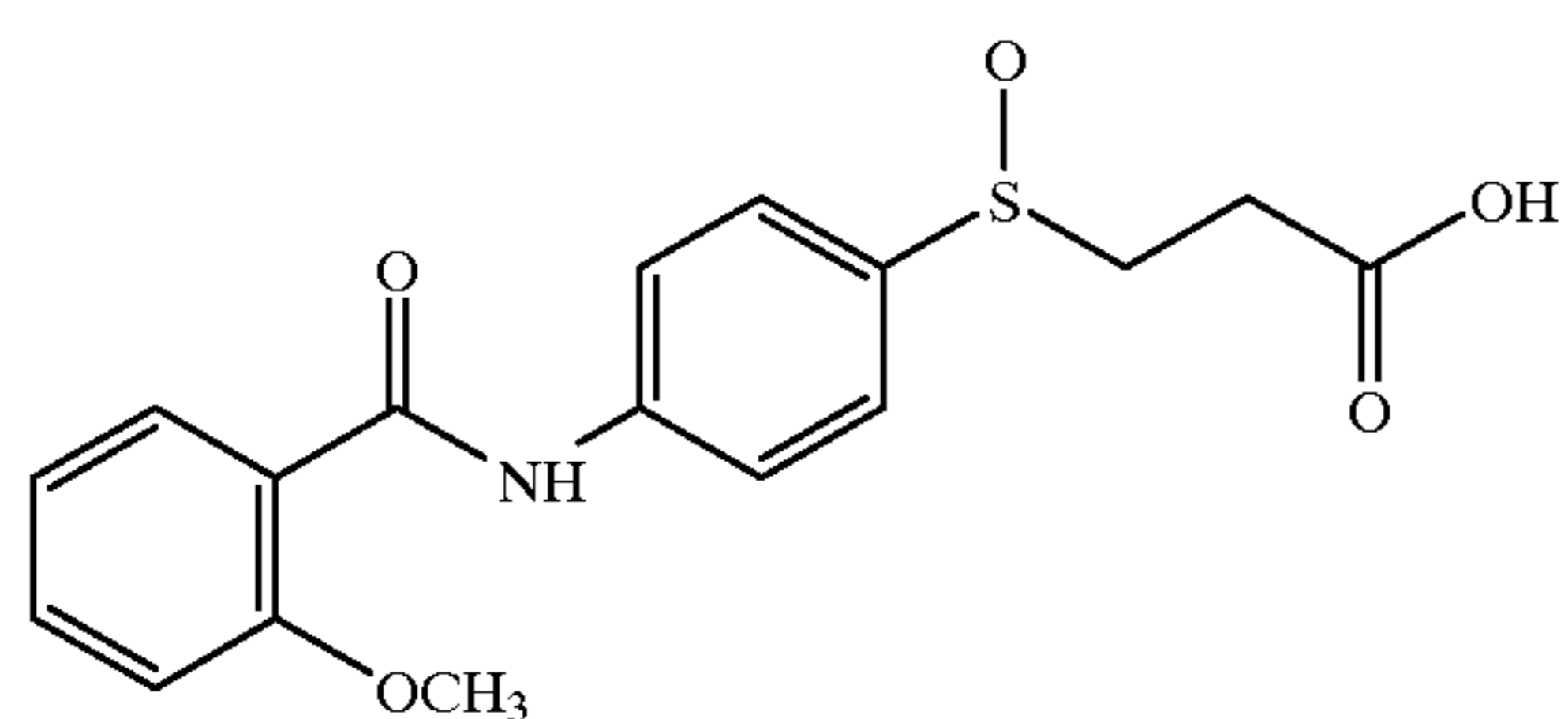
4-(2-methoxybenzoyl)amino 3-carboxysulfoxide
