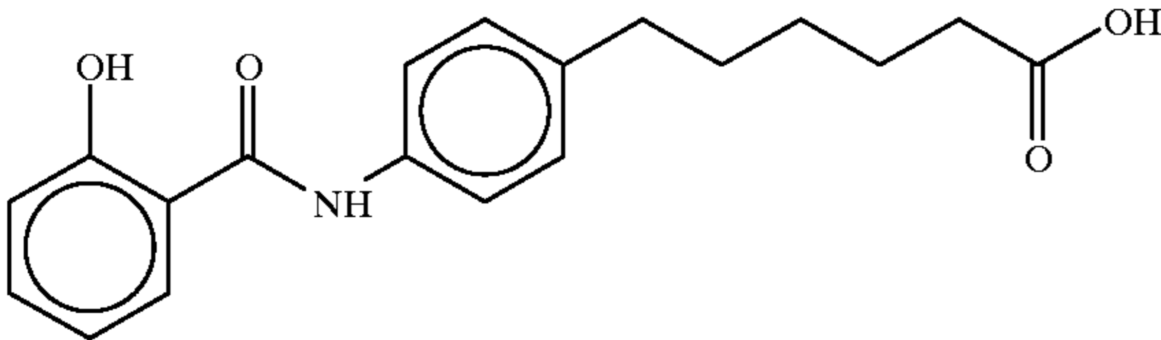
6-(4-(salicyloyl)aminophenyl)hexanoic acid
