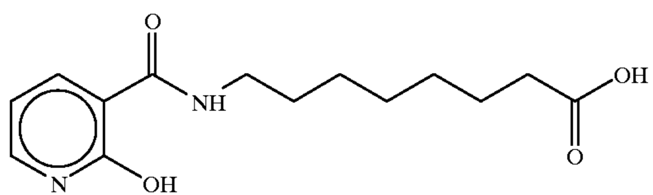
8-(2-Hydroxynicotinoyl)aminocaprylic acid
