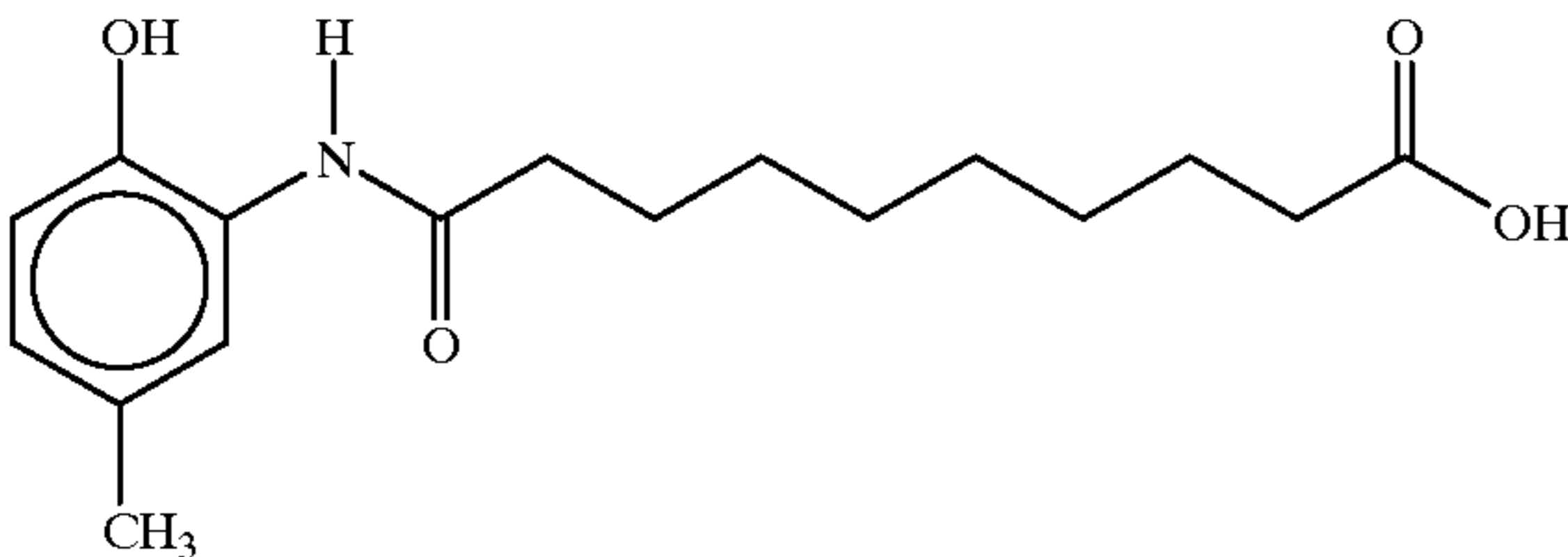
9-(2-hydroxy-5-methylanilincarbonyl)nonanoic acid
