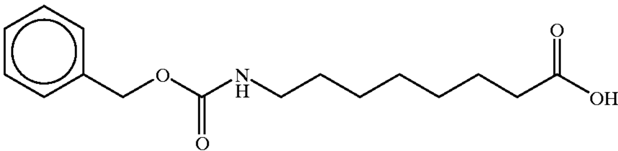
8-(Benzylcarbonylamino)caprylic acid
