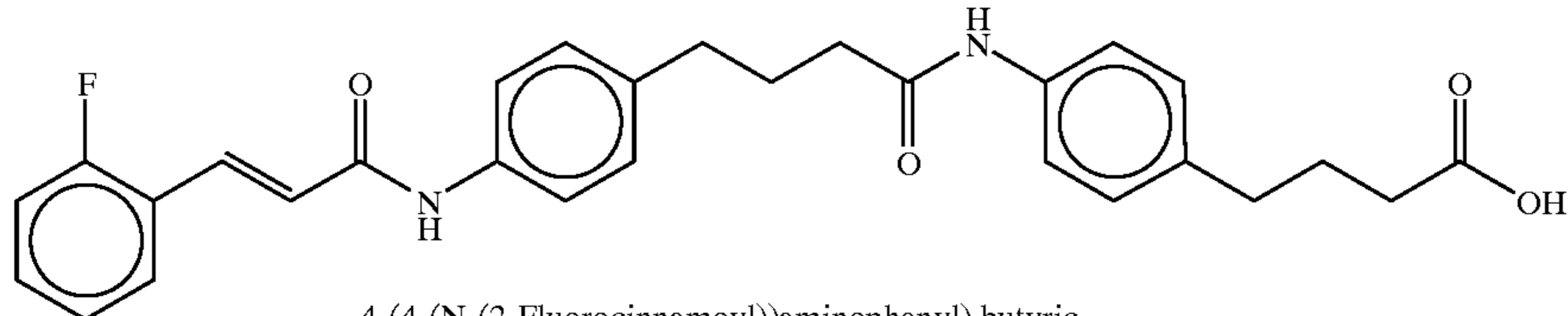
4-(4-(N-(2-Fluorocinnamoyl))aminophenyl) butyric
