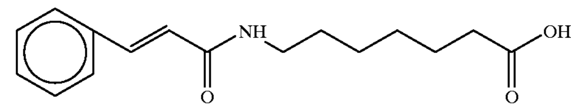
7-cinnamoylaminoheptanoic acid
