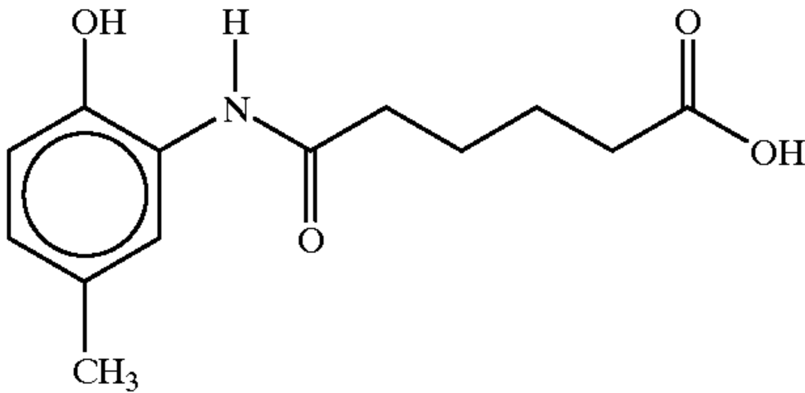
5-(2-hydroxy-5-methylanilincarbonyl)valeric acid
