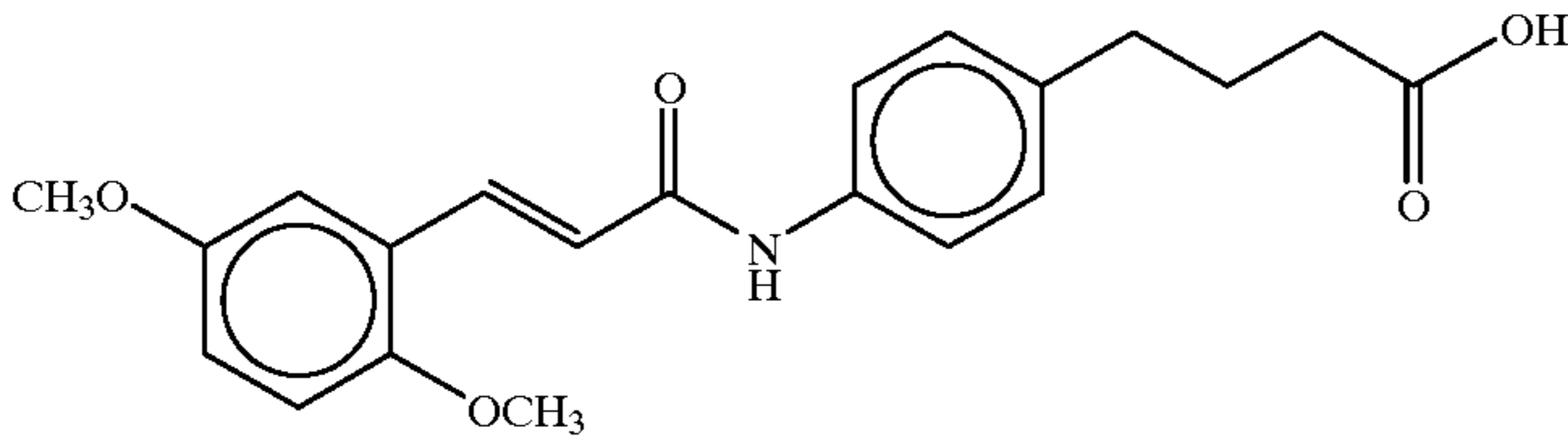
4-(4-(2,5-dimethoxycinnamoyl)aminophenyl)butyric acid
