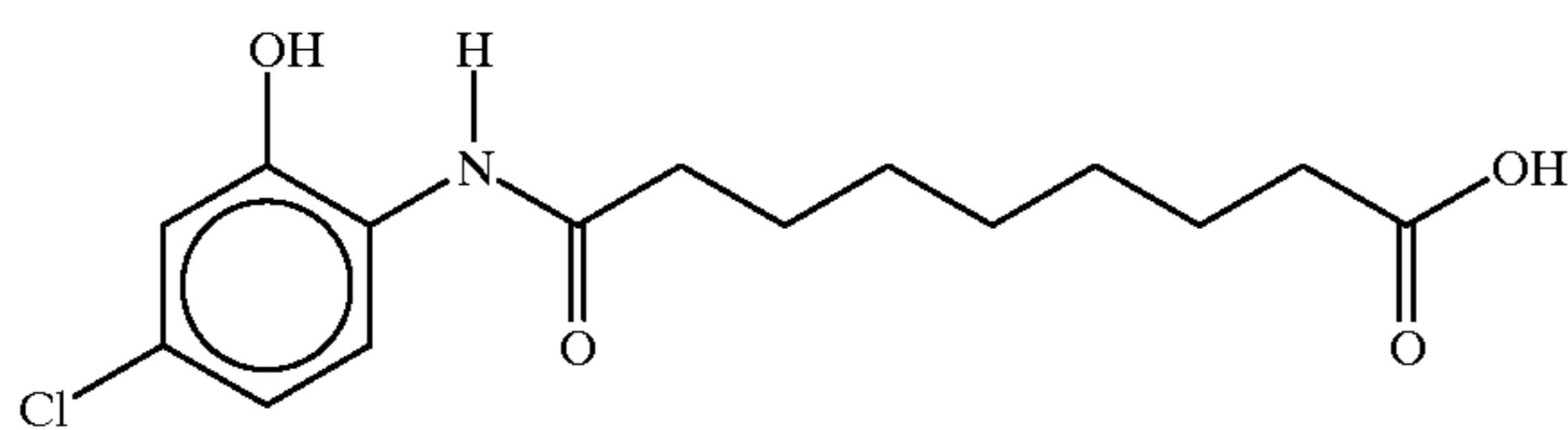
8-(2-hydroxy-5-chloroanilino)octanoic acid
