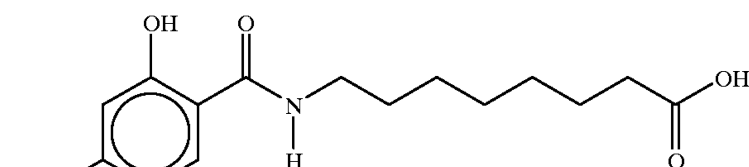
8-(N-2-Hydroxy-4-methoxybenzoyl)aminocaprylic acid
