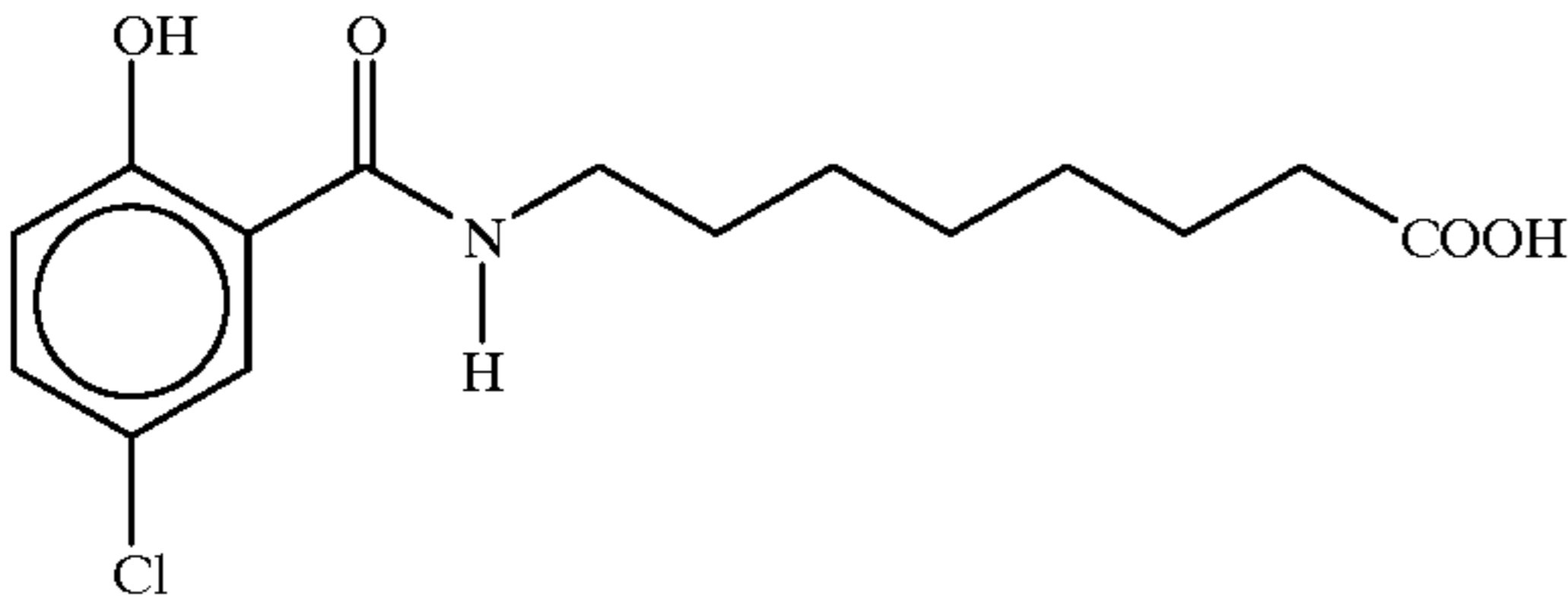
8-(N-2-hydroxy-5-chlorobenzoyl)aminocaprylic acid
