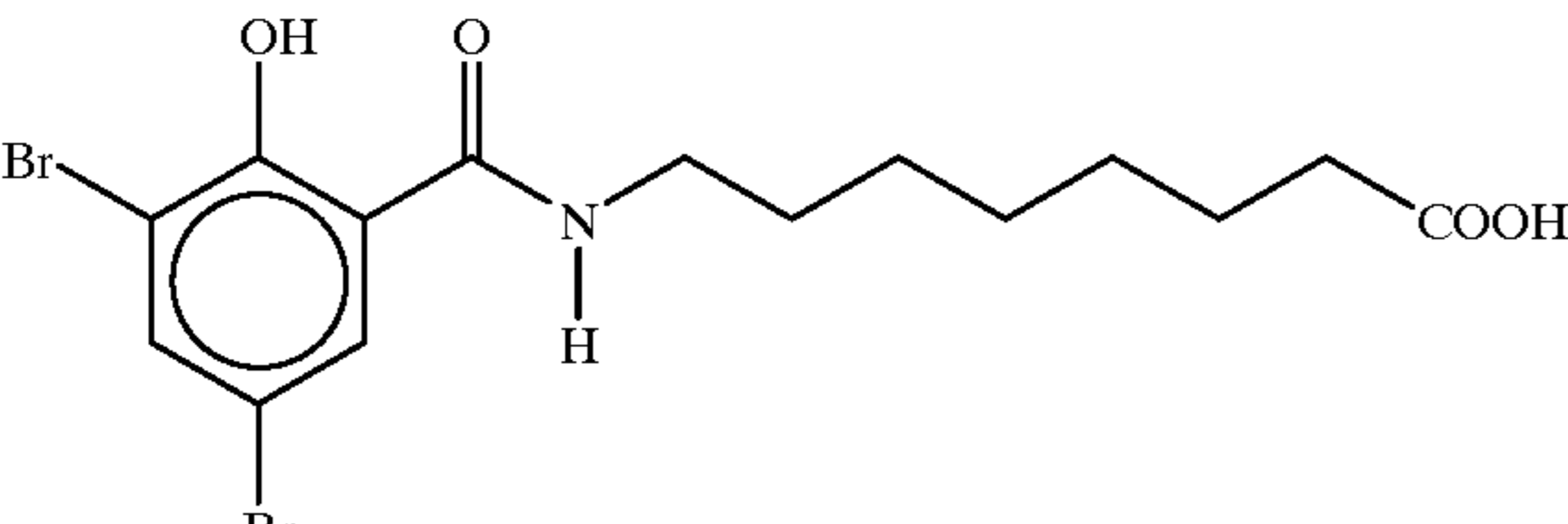
8-[N-(2-acetoxy-3,5-dibromobenzoyl)]aminocaprylic acid
