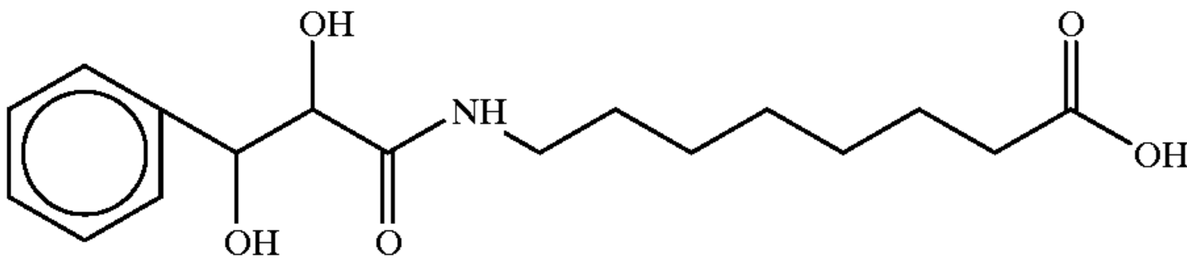
(3Phenyl2,3dihydroxypropanoyl)8aminocaprylic acid
