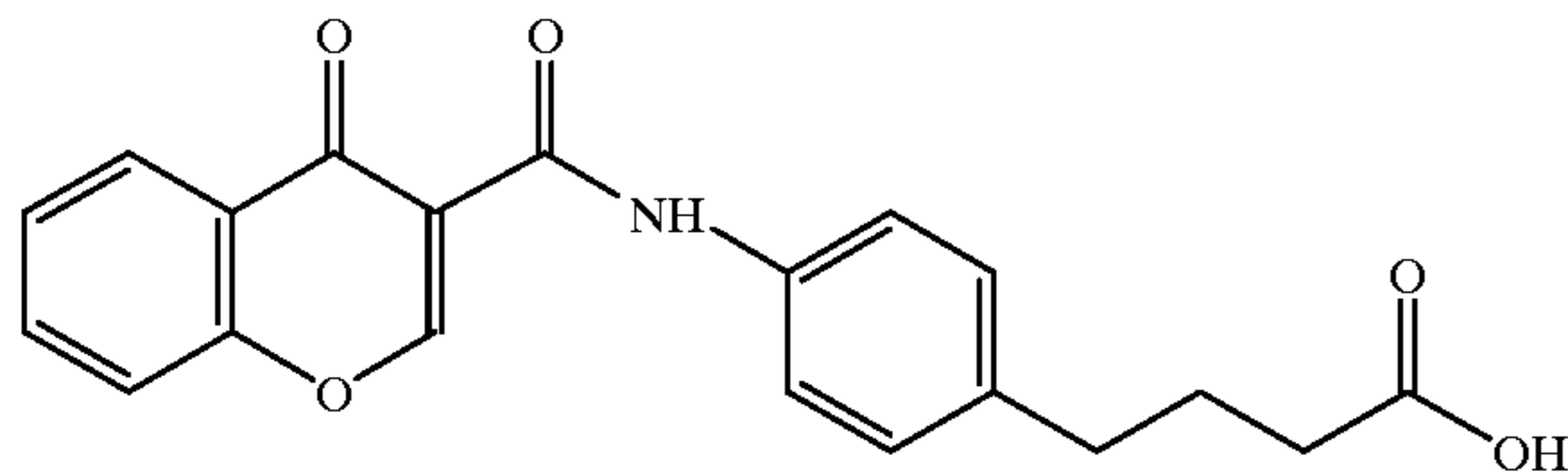
4-(4-(chromone-3-carbonyl)aminophenyl)butyric acid
