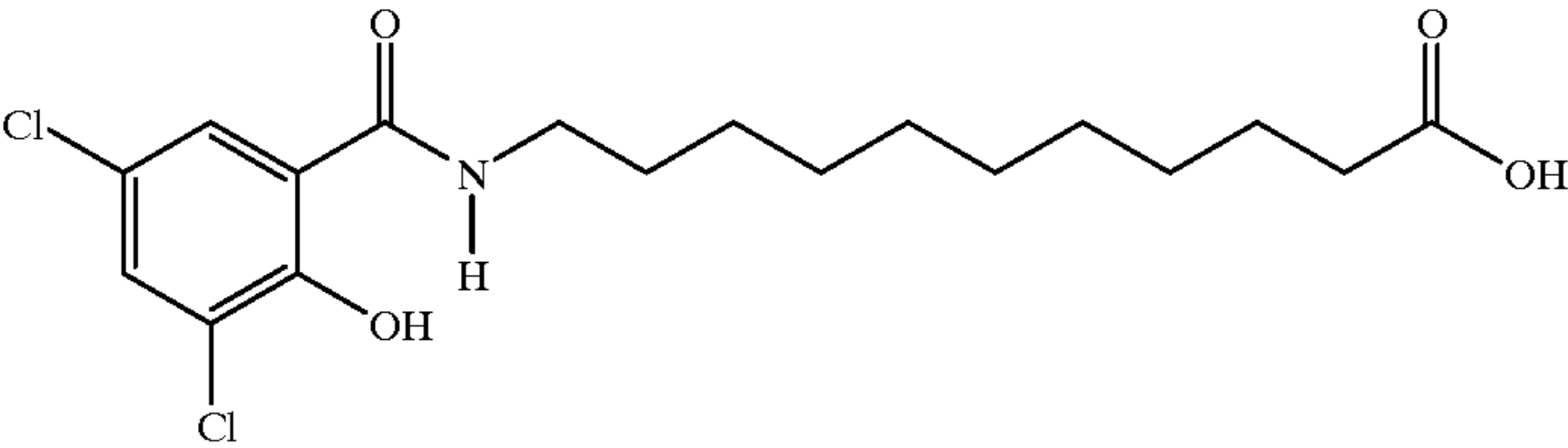
11-N-(3,5-dichloro-2-hydroxybenzoyl)aminoundecanoic acid
