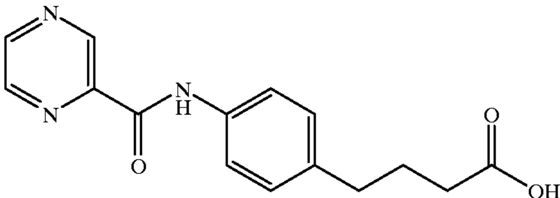
4-(4-(2-pyrazinecarbonyl)aminophenyl)butyric acid
