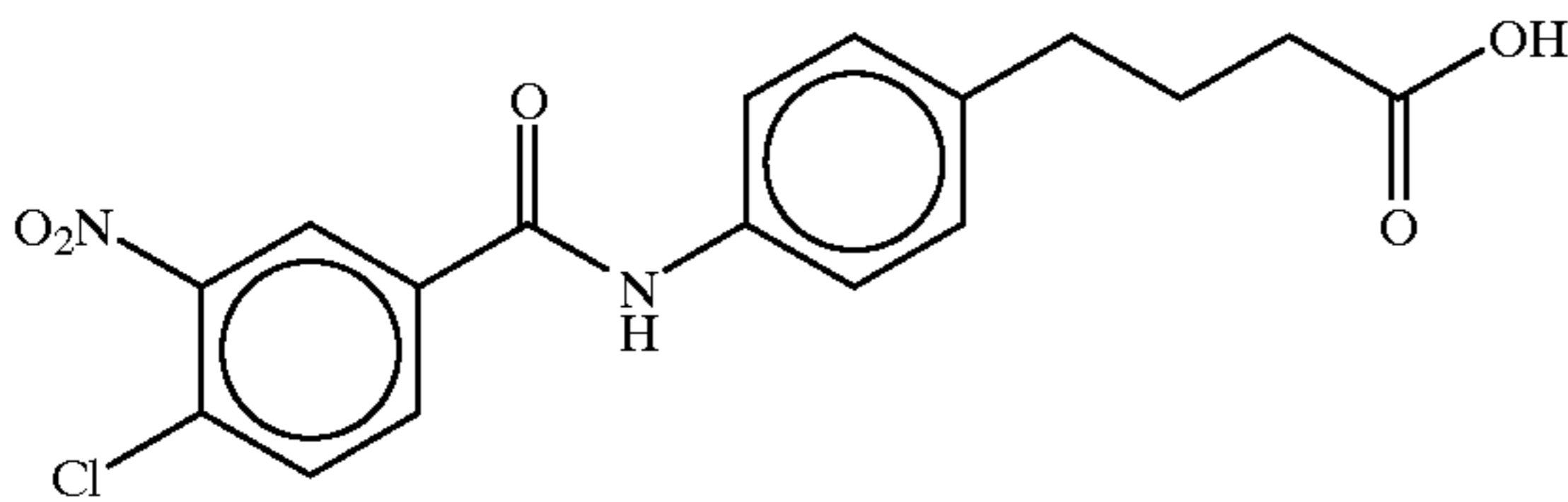
4-(4-(4-chloro-3-nitrobenzoyl)aminophenyl)butyric acid
