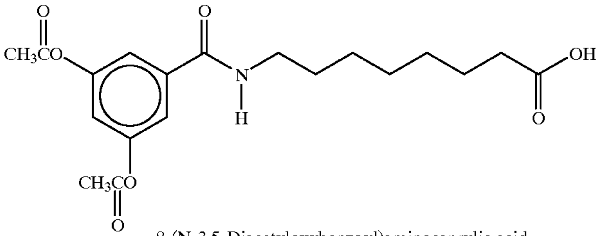
8-(N-3,5-Diacetyloxybenzoyl)aminocaprylic acid
