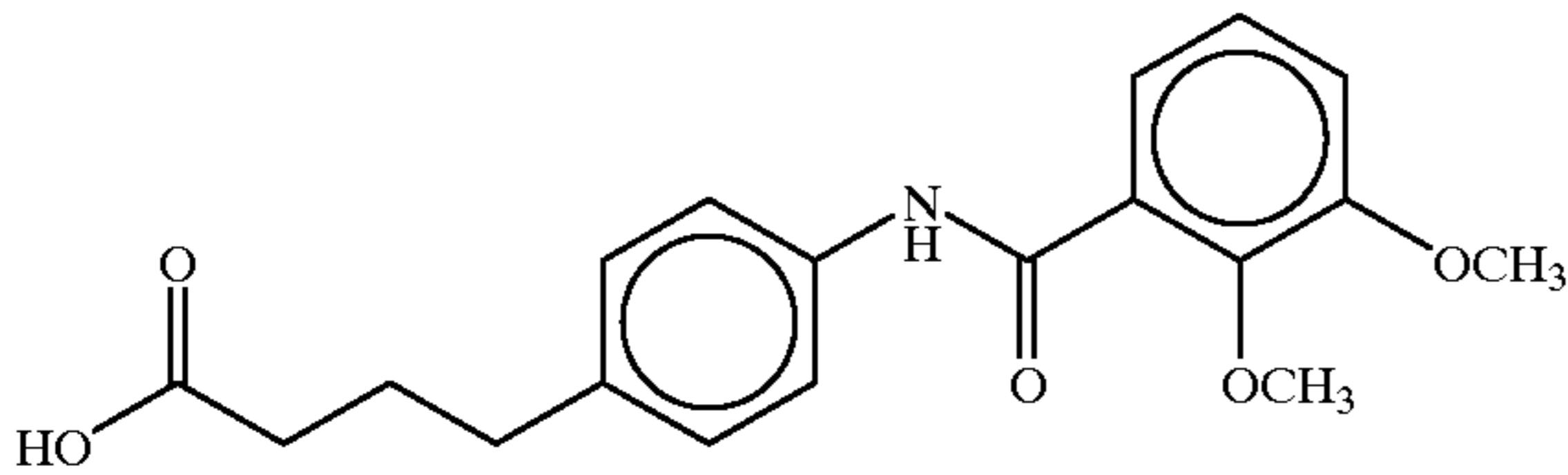
4-(4-(2,3-dimethoxybenzoyl)aminophenyl)butyric acid
