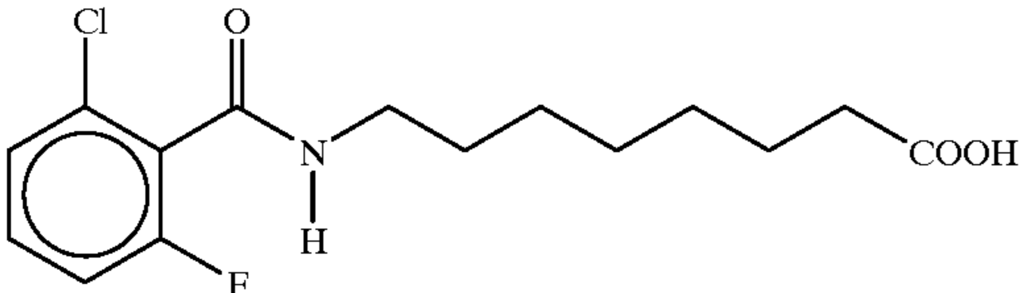
8-N-(2-chloro-6-fluorobenzoyl)aminocaprylic acid
