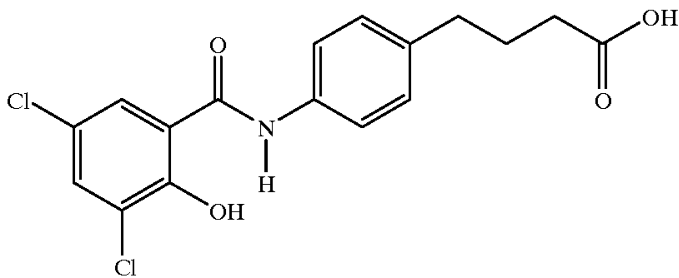
N-[3,5-dichloro-2-hydroxybenzoyl-4(4-aminophenyl)]butyric acid
