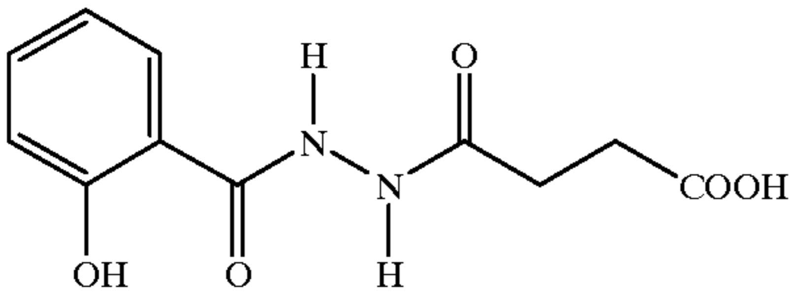
1-Salicyloyl-2-succinyl hydrazide
