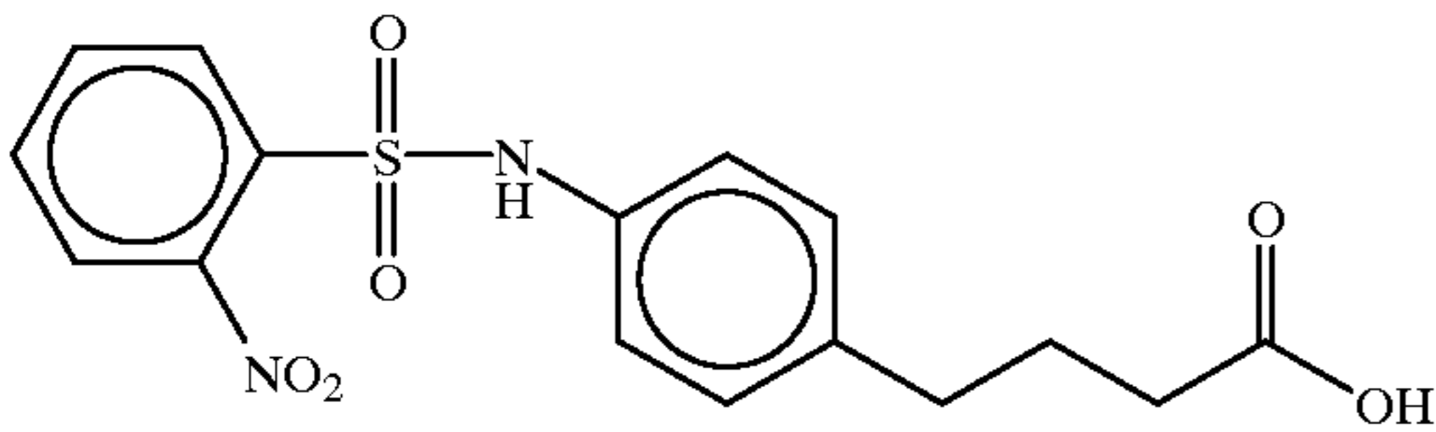
4-(4-(2-nitrobenzenesulfonyl)aminophenyl)butyric acid
