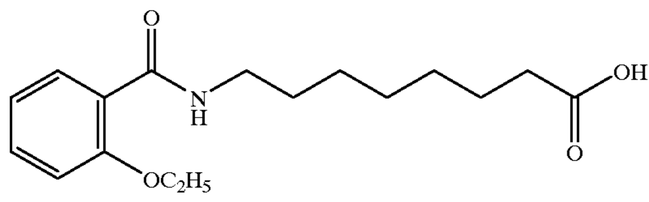
8-(2-ethoxybenzoyl)aminocaprylic acid
