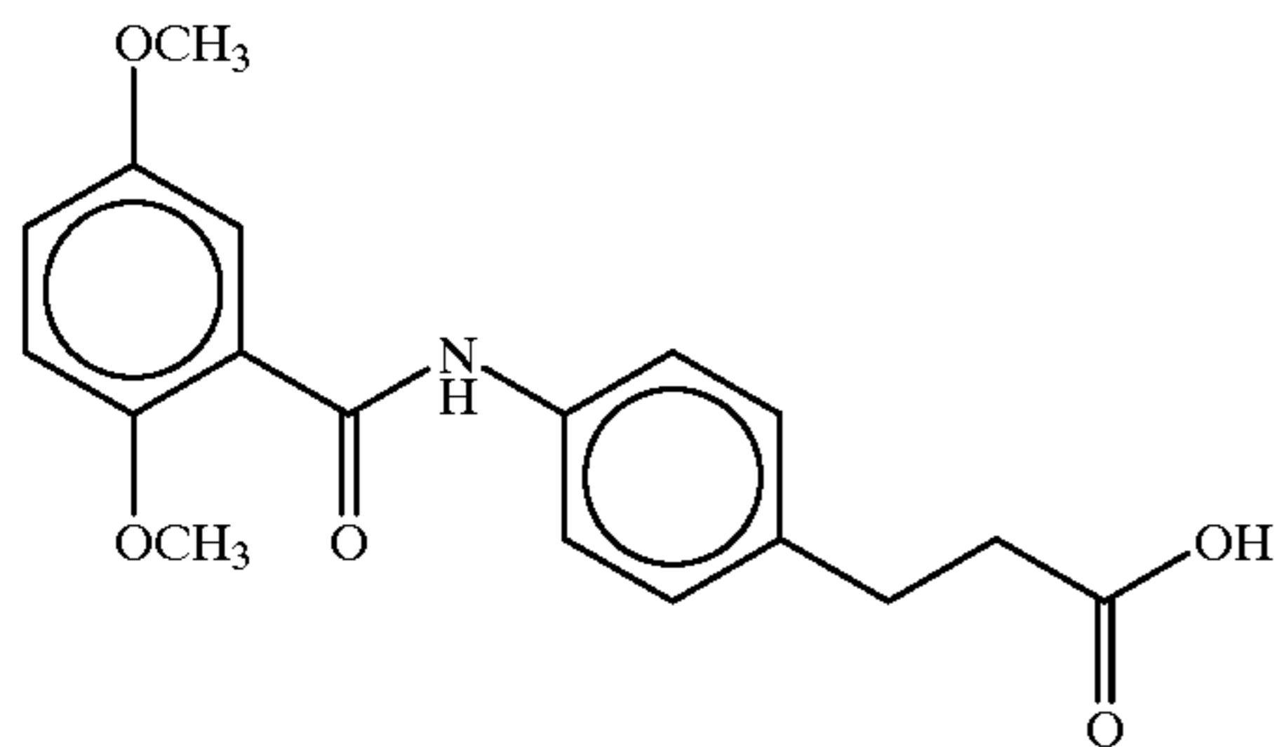
3-(4-(2,5-dimethoxybenzoyl)aminophenyl)propionic acid
