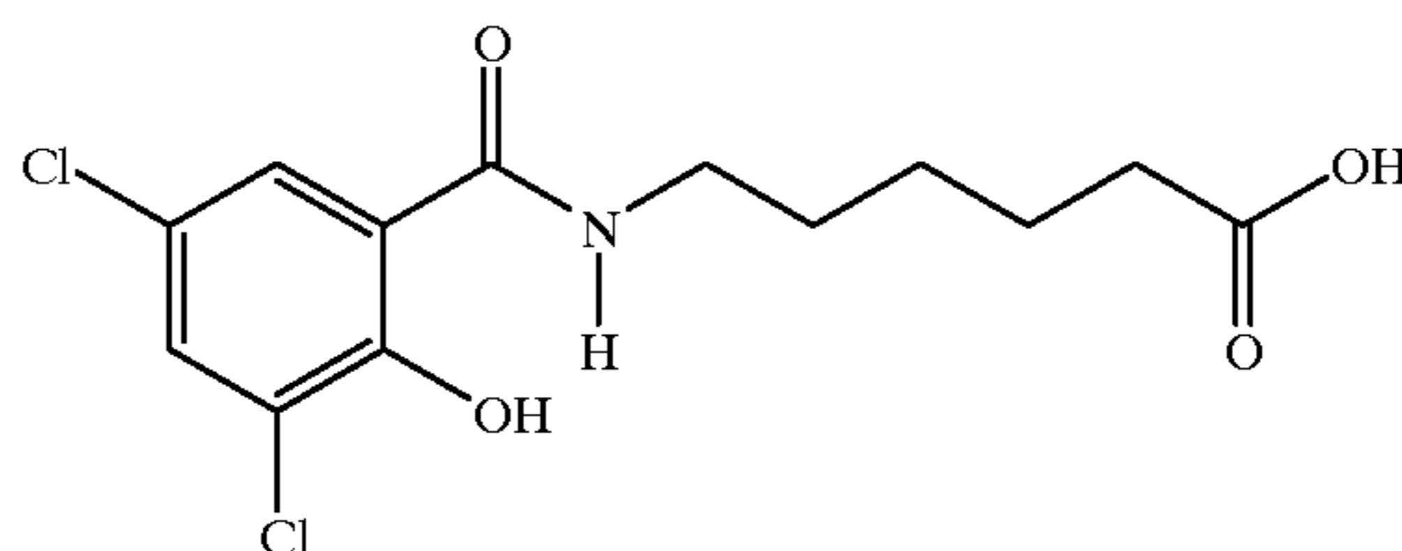
6-N-(3,5-dichloro-2-hydroxybenzoyl)aminocaproic acid
