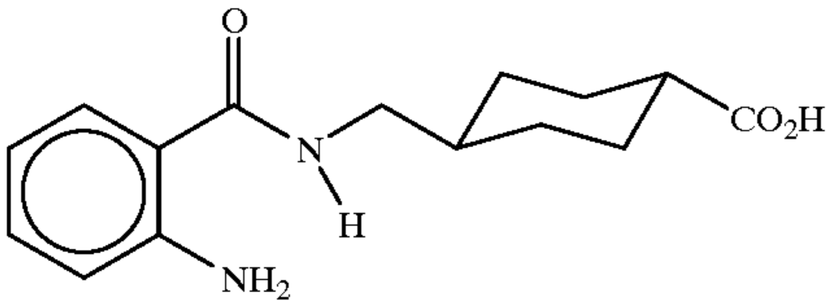
trans-4-(2-aminobenzamidomethyl)cyclohexanecarboxylic acid
