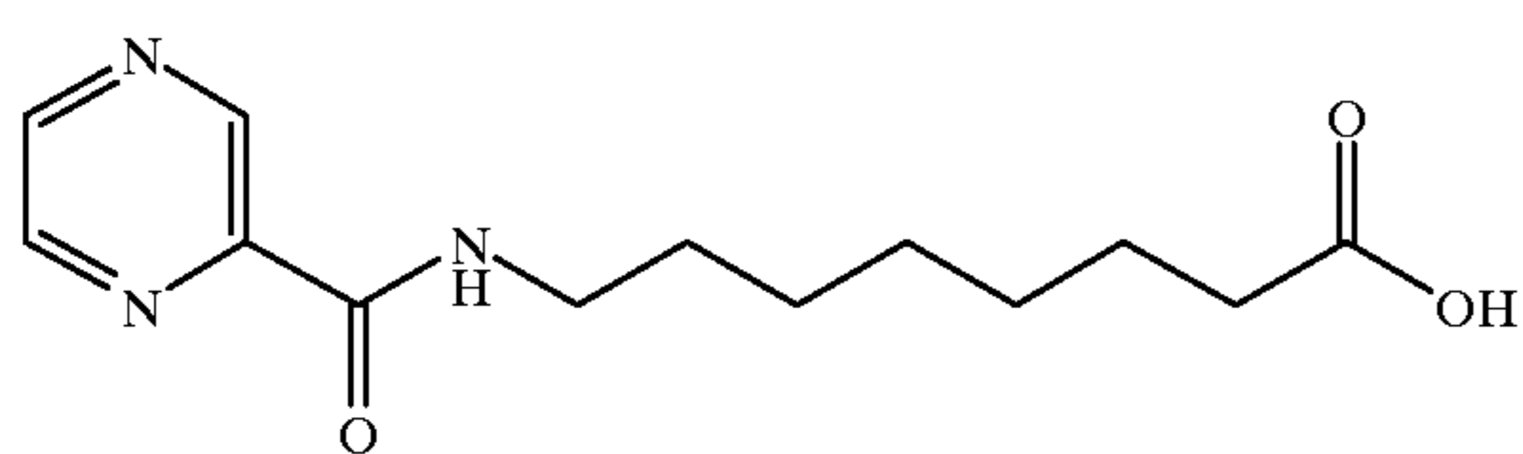
8-(2-pyrazinecarbonyl)aminocaprylic acid
