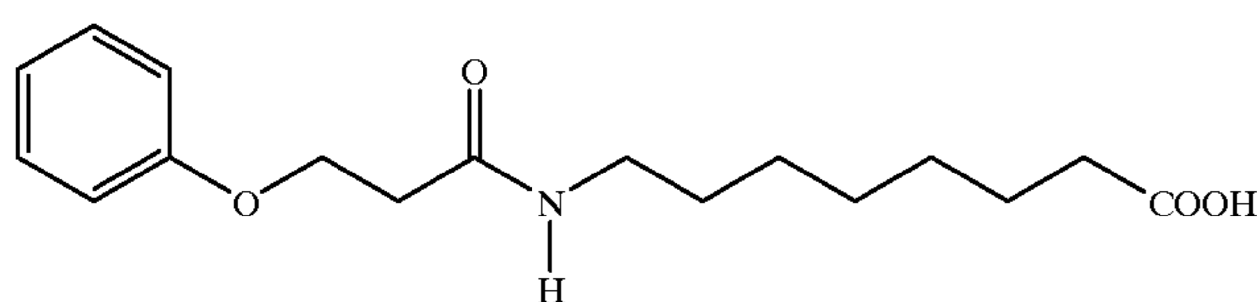
8-(3-Phenoxypropionylamino)caprylic acid
