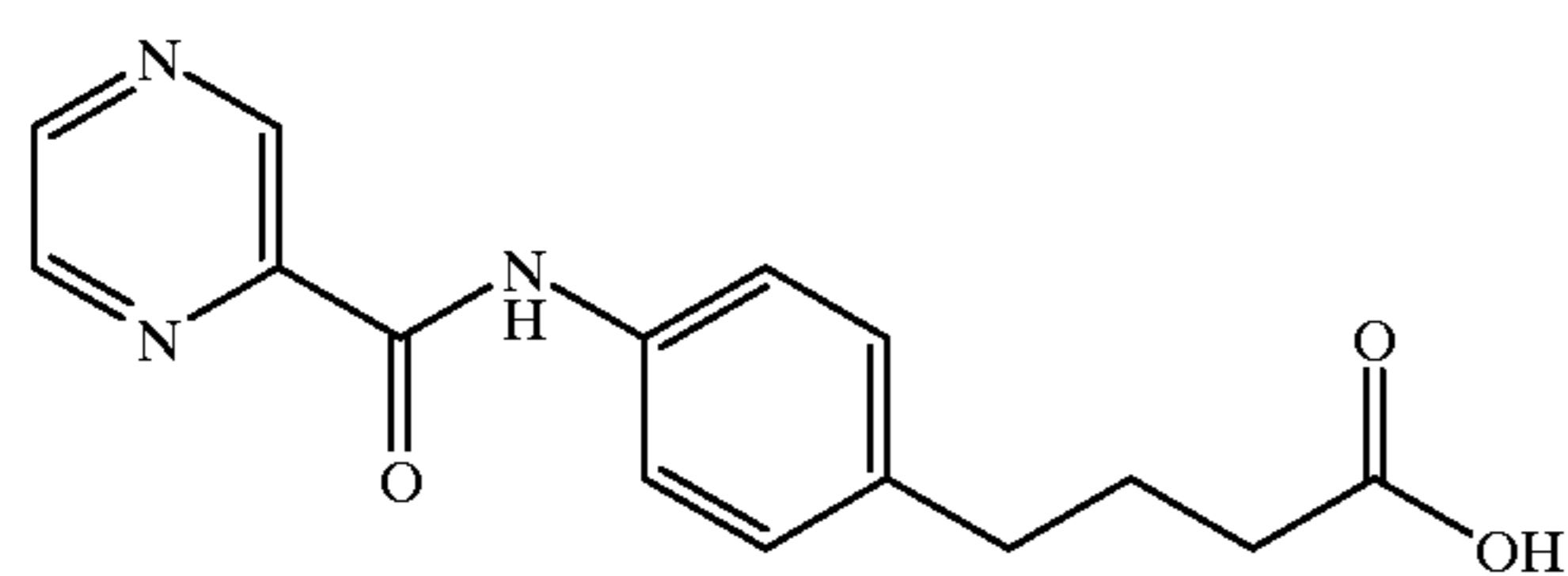
4-(4-(2-pyrazinecarbonyl)aminophenyl)butyric acid
