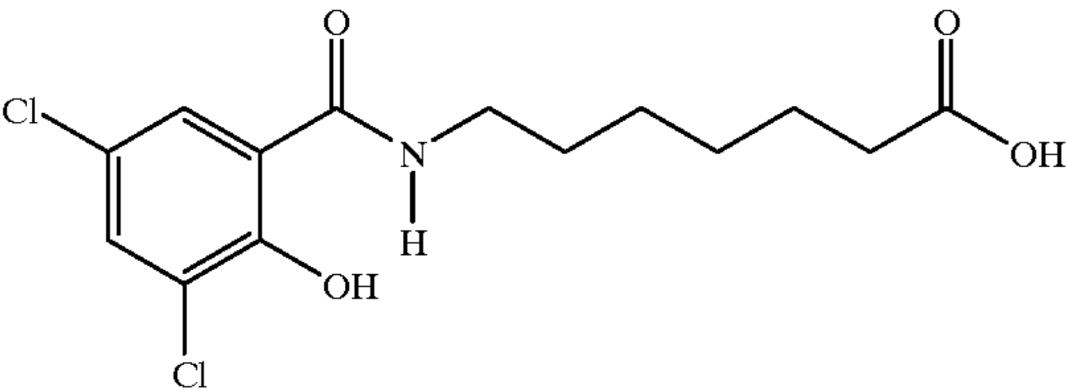
7-N-(3,5-dichloro-2-hydroxybenzoyl)aminoheptanoic acid
