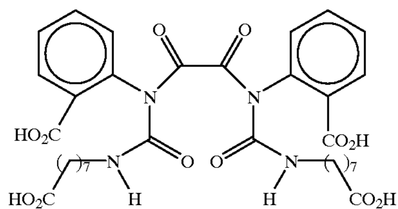
Bis(N-2-carboxylphenyl-N-(N'-8-octanoic acid)ureal)oxalyl diamide
