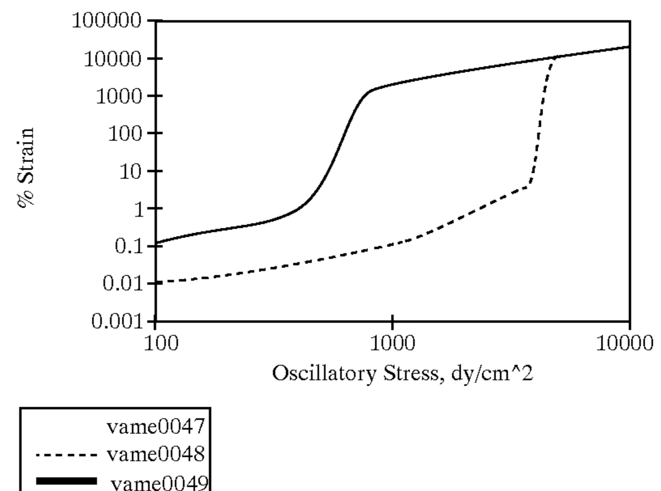
Methyl Ester % Strain Vs Oscillatory Stress
