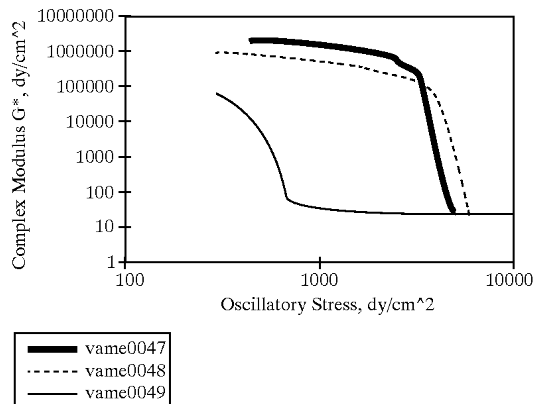
Methyl Ester Complex Modulus Vs Oscillatory Stress at 1 Hz
