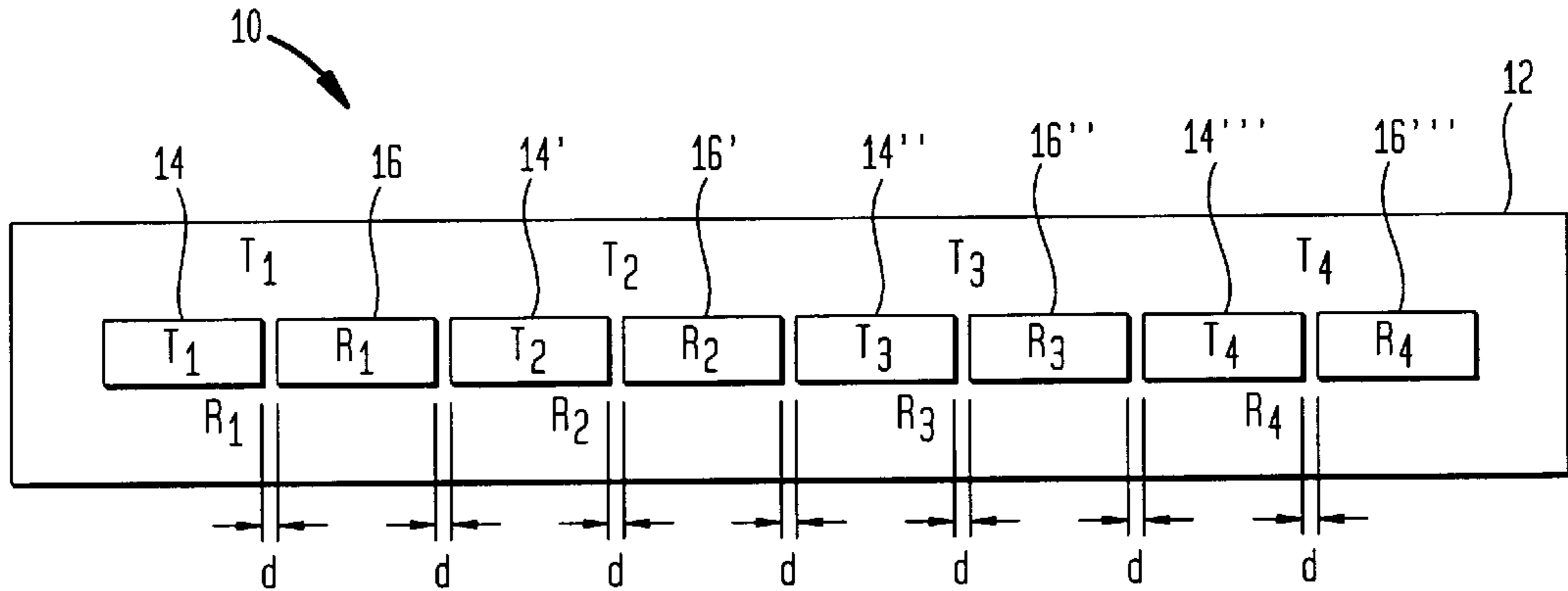
FIG. 1 (PRIOR ART)
