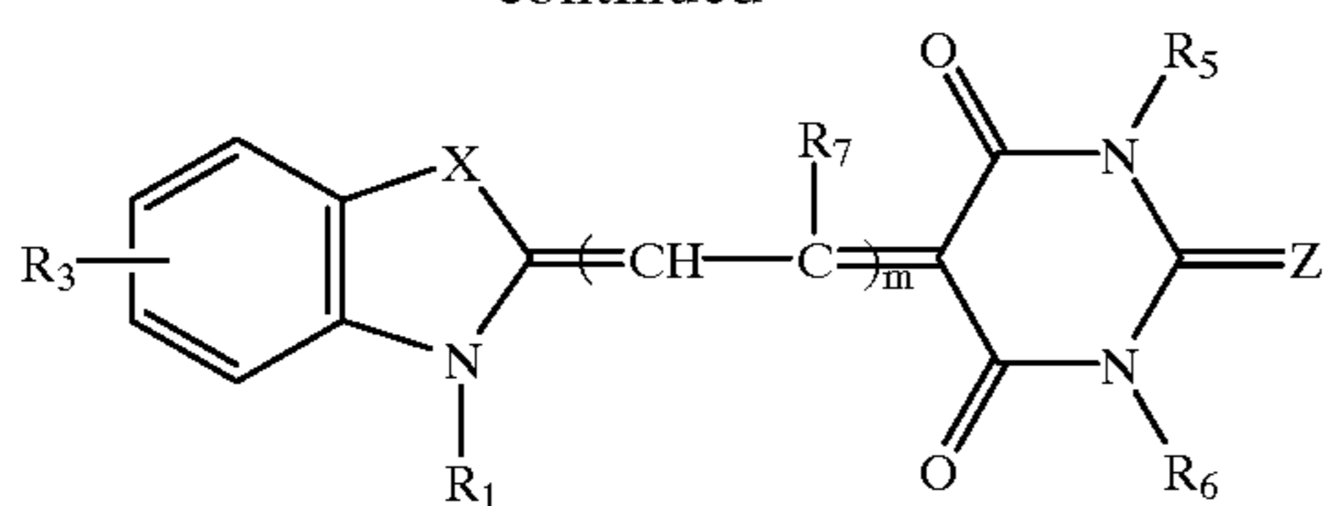
MERCOYANINE
