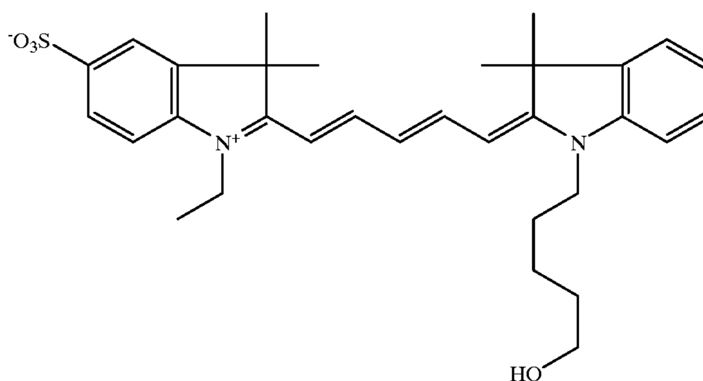
1-Ethyl-2-{5-[1-(5-hydroxypentyl)-3,3-dimethyl-2,3-dihydro-1H-benzo[b]azol-2-yliden]-1,3-pentadienyl}-3,3-dimethyl-3H-benzo[b]azolium-5-sulfonate
