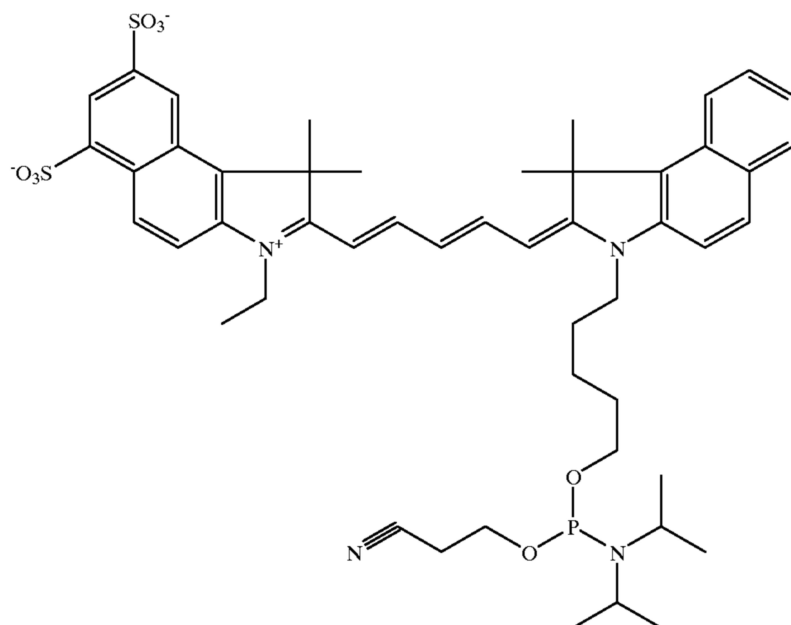
Potassium 3-ethyl-2-{5-[3-(5-hydroxypentyl)-1,1-dimethyl-2,3-dihydro-1H-naphtho[2,1-b]azol-2-ylidene]-1,3-pentadienyl}-1,1-dimethyl-1H-Naphtho[2,1-b]azolium-6,8[disulfonate
