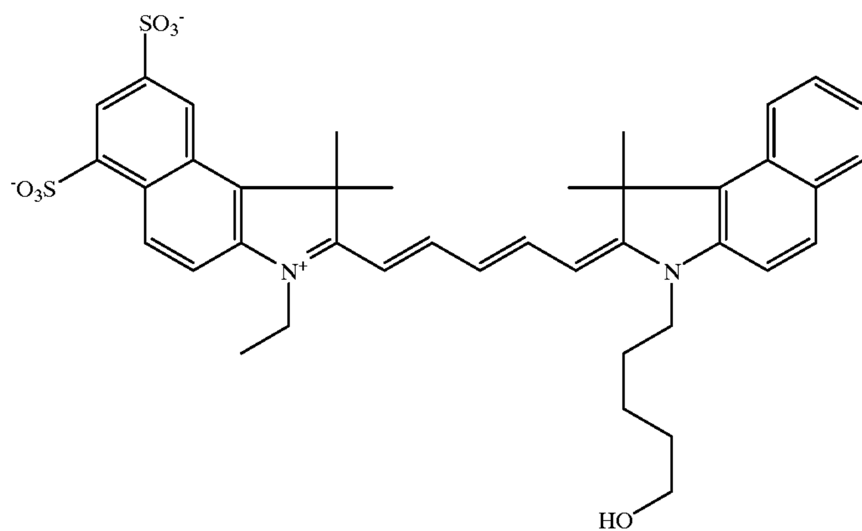
Potassium 3-ethyl-2-{5-[3-(5-hydroxypentyl)-1,1-dimethyl-2,3-dihydro-1H-naphtho[2,1-b]azol-2-ylidene]-1,3-pentadienyl}-1,1-dimethyl-1H-Naphtho[2,1-b]azolium-6,8[disulfonate
