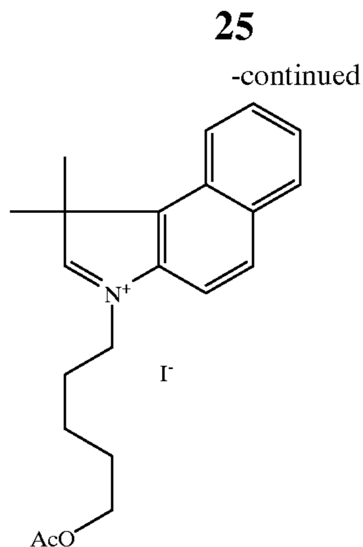
1,1,2-Trimethyl-3-(5-methylcarbonyloxy-pentyl)- 1H-naphtho[2,1-b]azolium iodide
