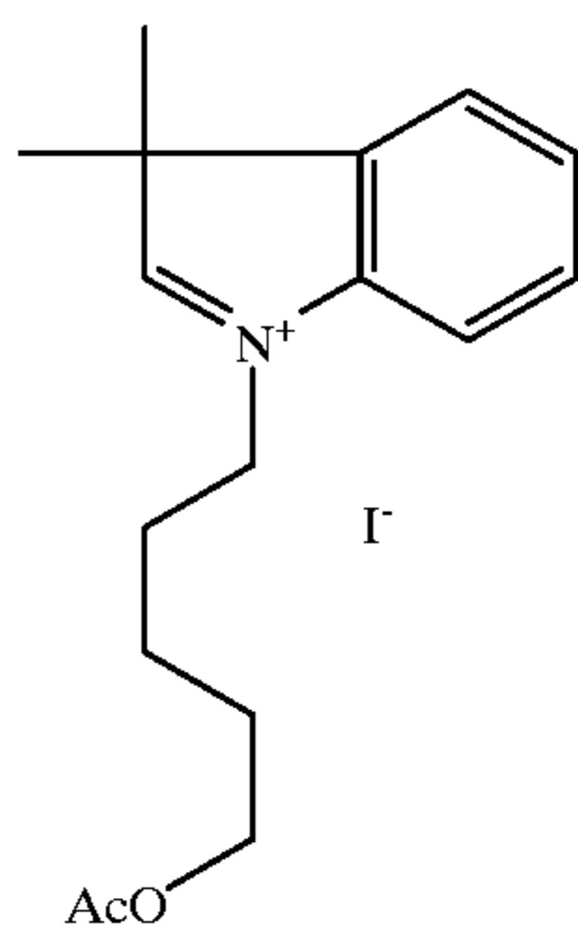
2,3,3-Trimethyl-1-(5-methylcarbonyloxy)pentyl-3H-benzo[b]azolium iodide
