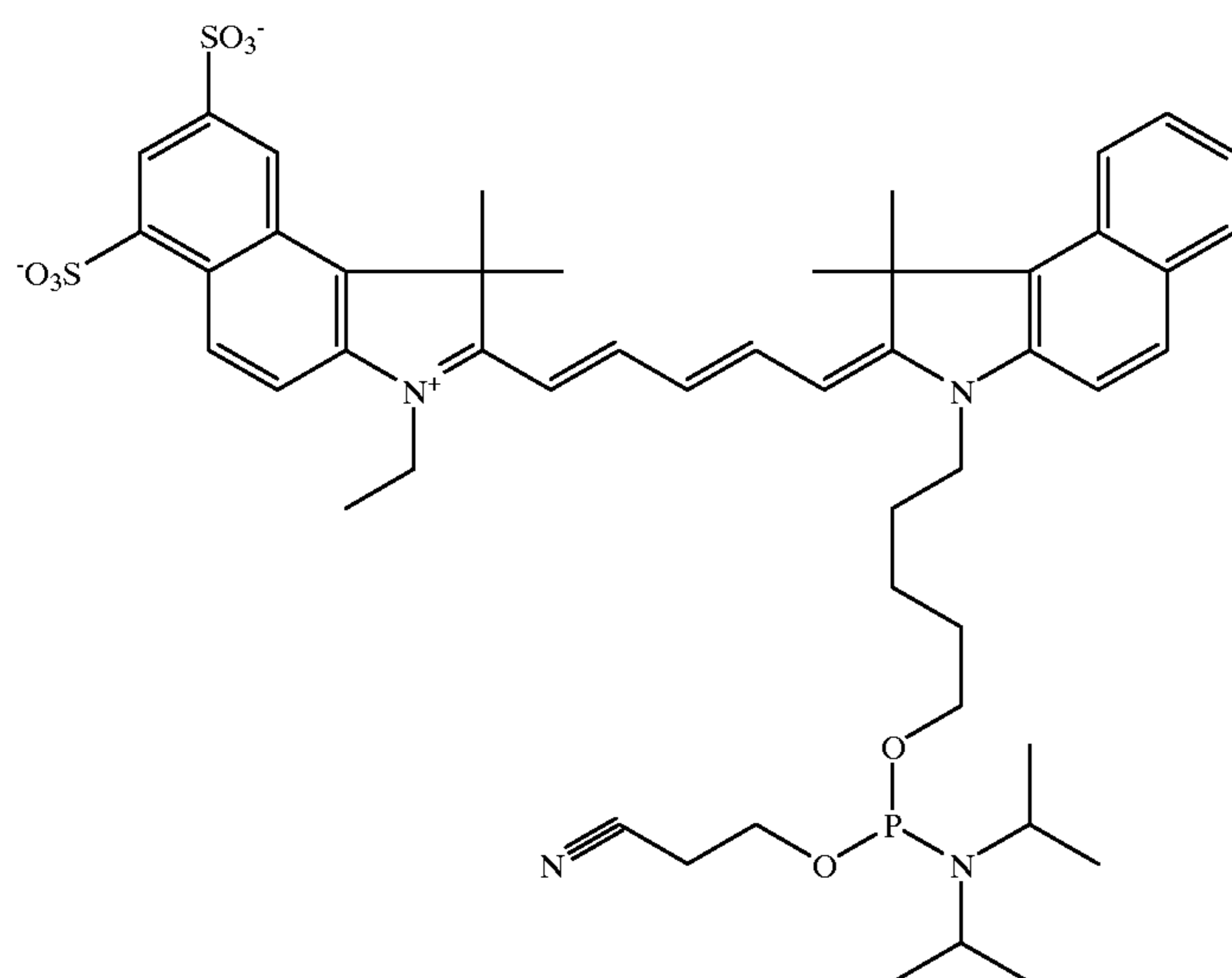
Potassium 3-ethyl-2-{5-[3-(5-hydroxypentyl)-1,1-dimethyl-2,3-dihydro-1H-naphtho[2,1-b]azol-2-ylidene]-1,3-pentadienyl}-1,1-dimethyl-1H-Naphtho[2,1-b]azolium-6,8[disulfonate
