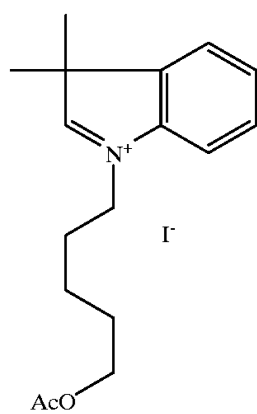
2,3,3-Trimethyl-1-(5-methylcarbonyloxy)pentyl-3H-benzo[b]azolium iodide
