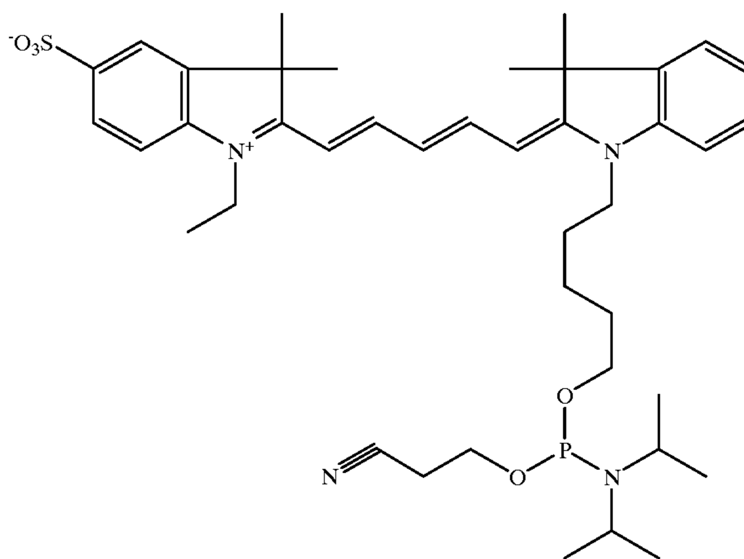
1-Ethyl-2-{5-[1-(5-(2-cyanoethyl-N,N-diisopropylphosphoramidite)pentyl)-3,3-dimethyl-2,3-dihydro-1H-benzo[b]azol-2-yliden]-1,3-pentadienyl}-3,3-dimethyl-3H-benzo[b]azolium-5-sulfonate (Example 1)
