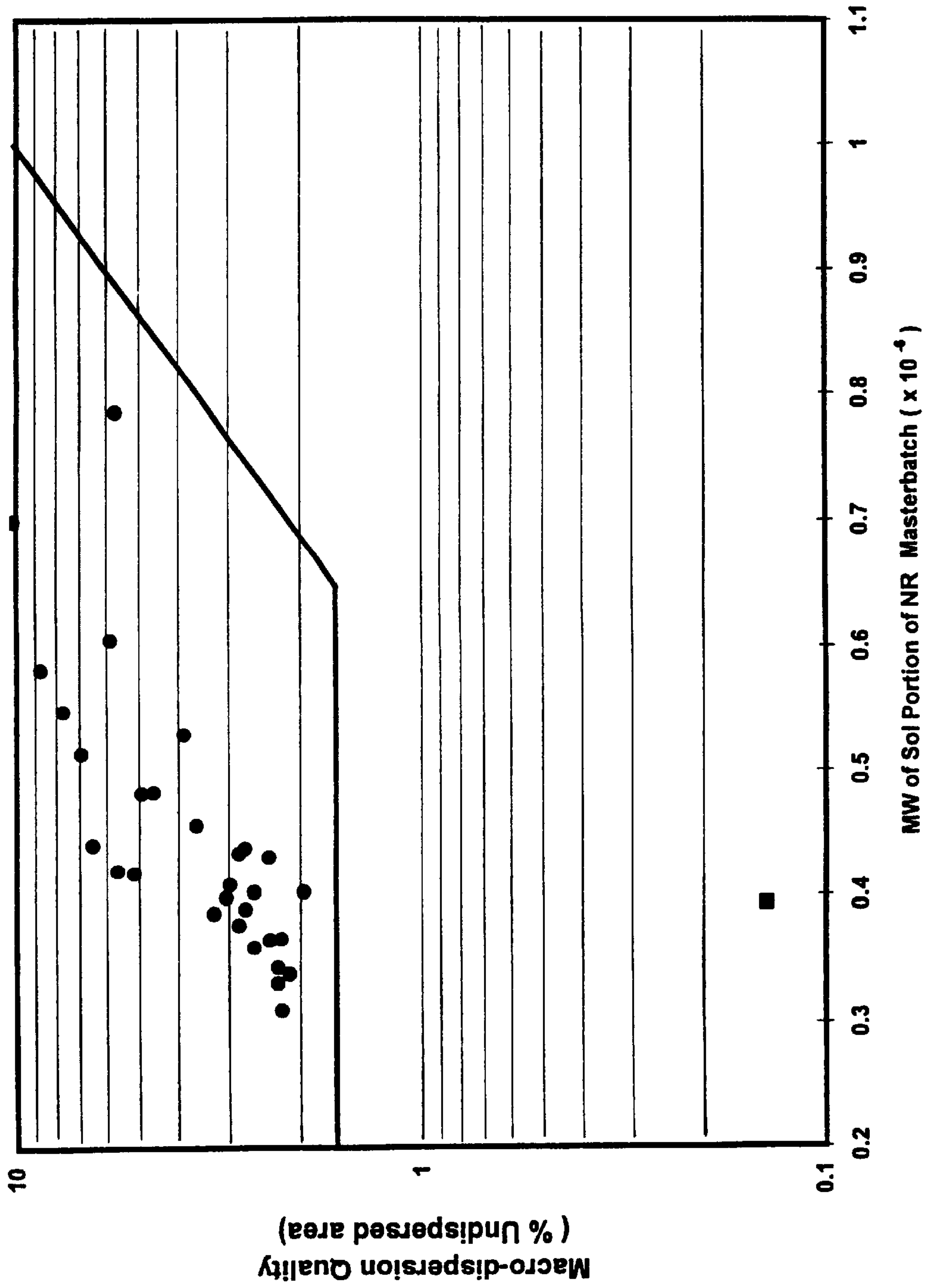
FIG. 15 Dispersion Quality and MW sol of NR Masterbatches (BLACK PEARL 800 Carbon Black, 55 phr)
