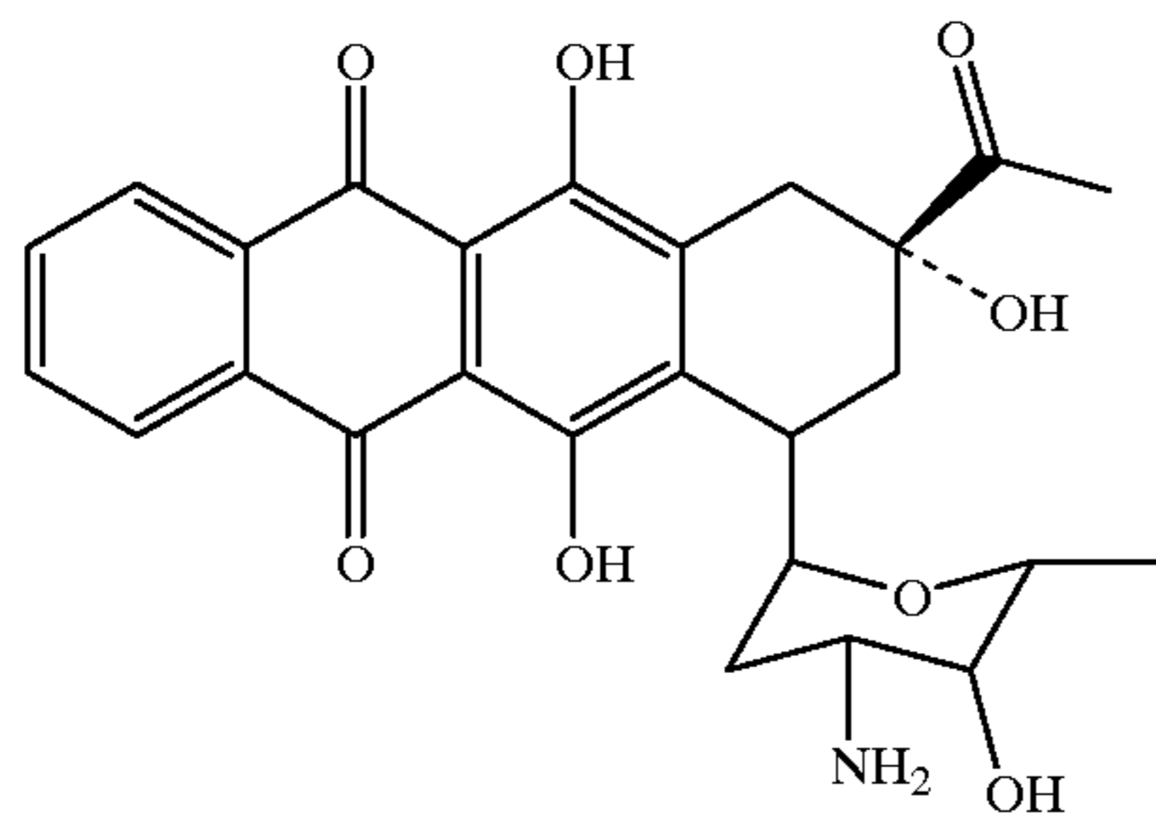
Idarubicin
