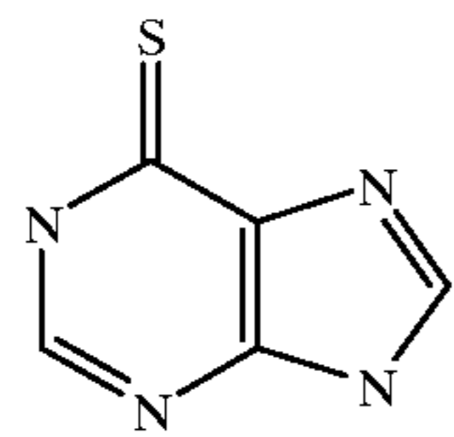
6-Mercaptopurine
