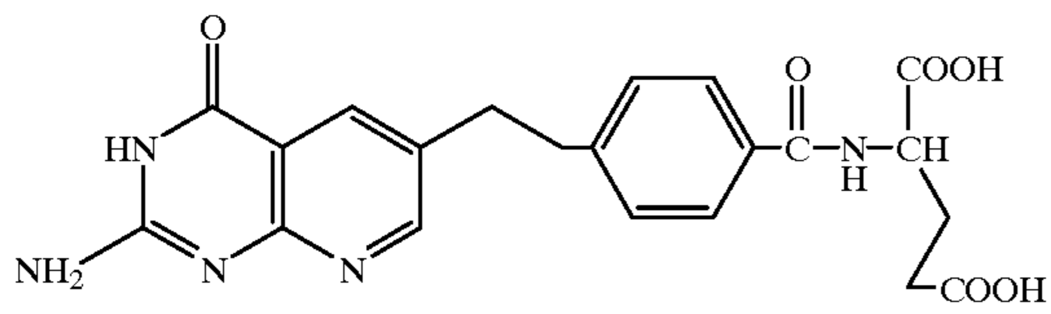
5,10-dideaza tetrahydrofolate
