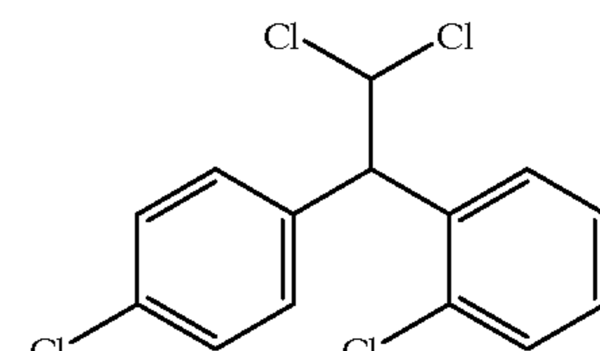
Mitotane
