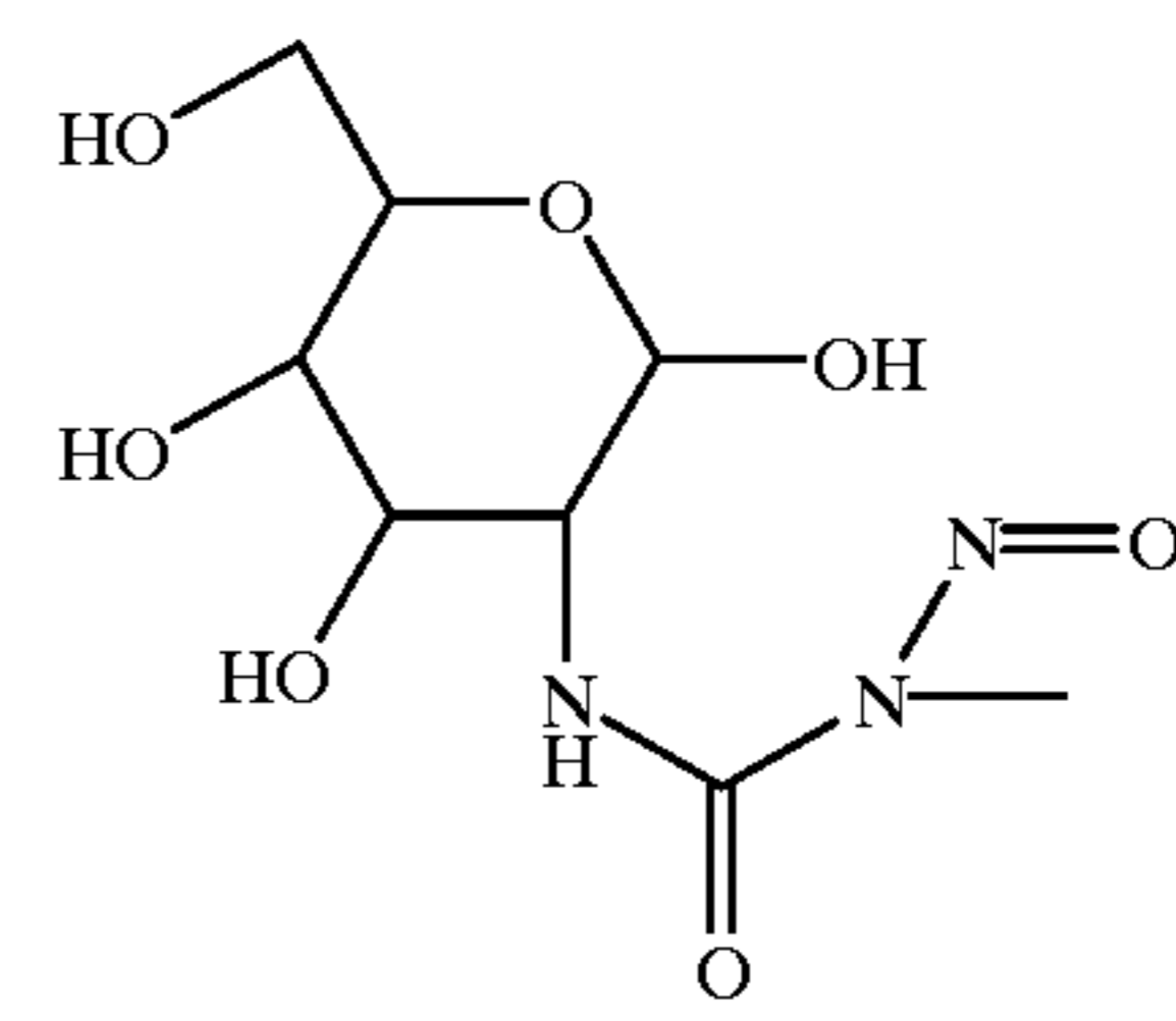
Streptozocin
