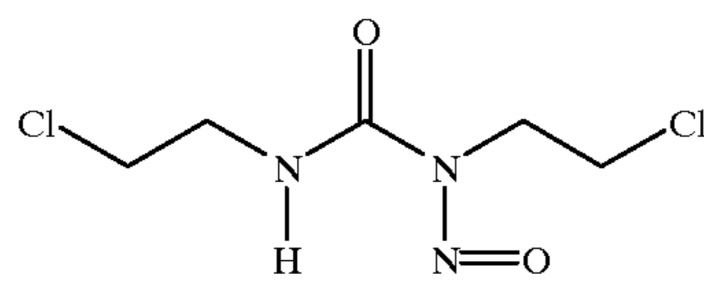
Carmustine (BCNU)
