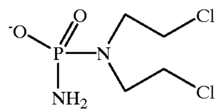
Phosphoramidate Mustard
