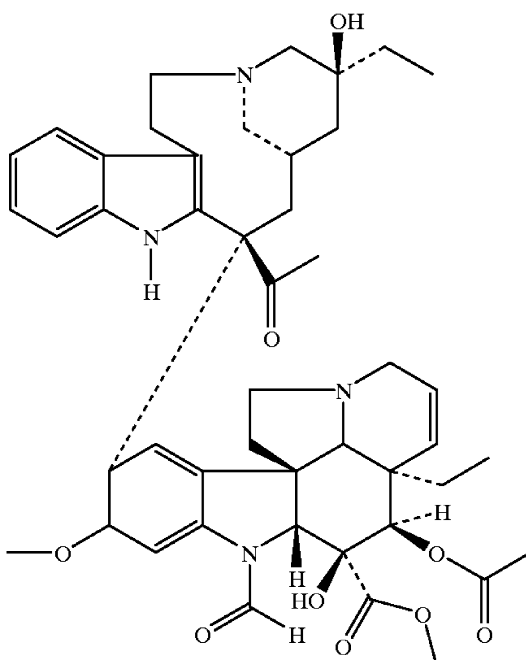
Vincristine
