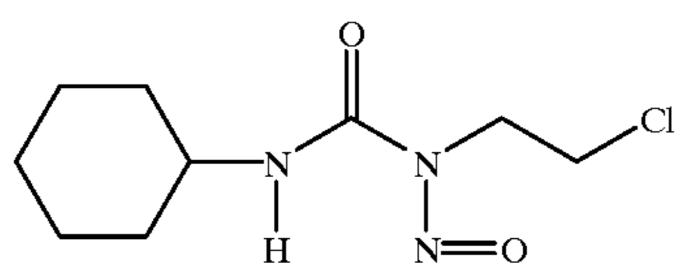
Lomustine (CCNU)
