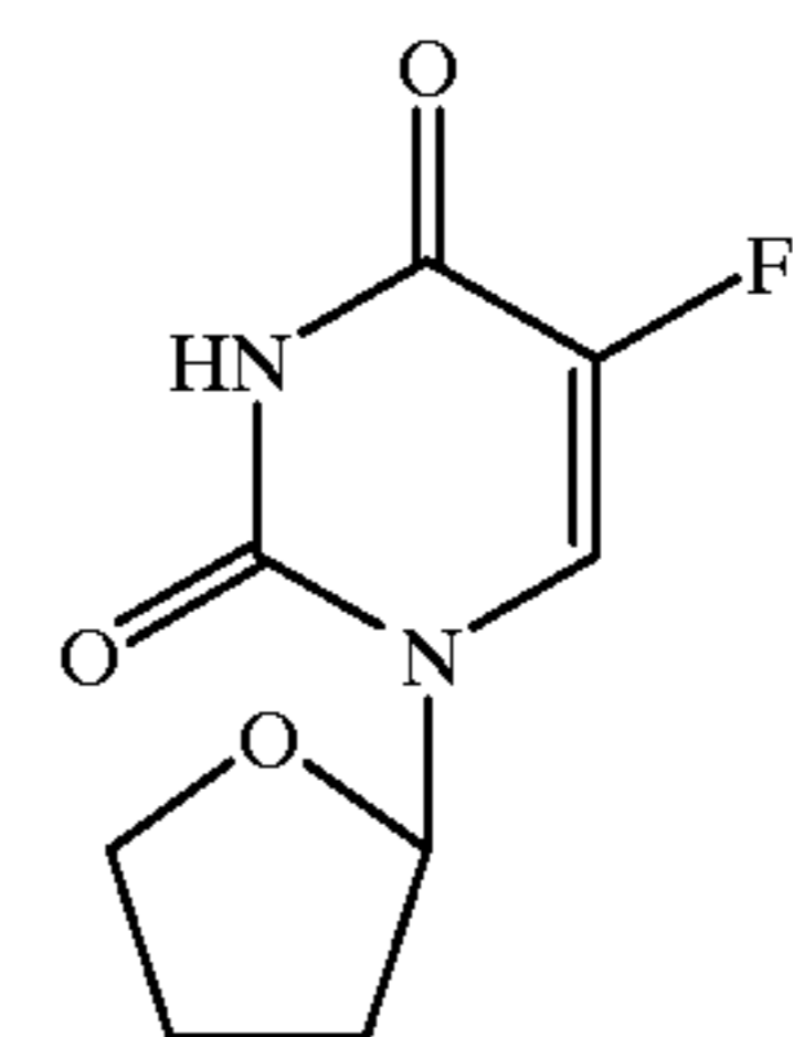
Ftorafur
