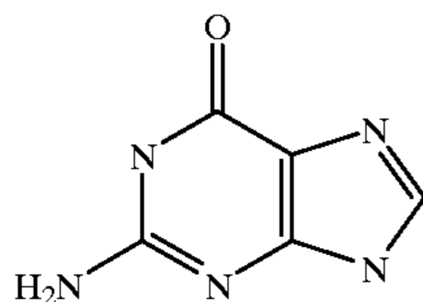
Guanine
