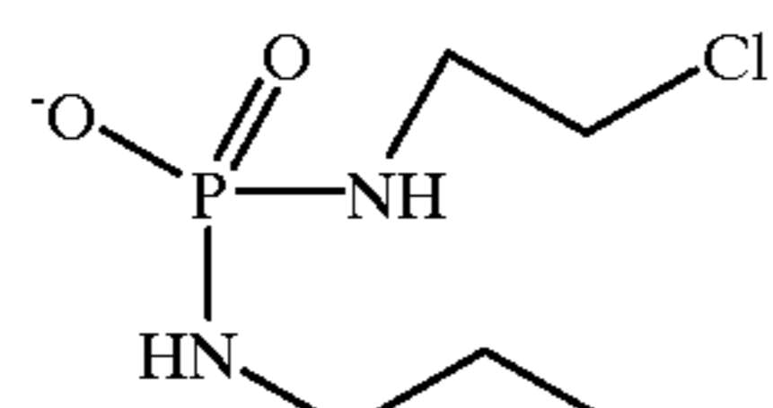
Isophosphoramidate Mustard
