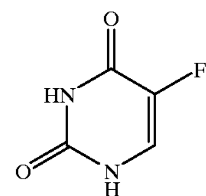
Fluorouracil (5-FU)
