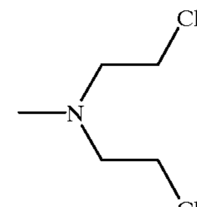
Mechlorethamine
