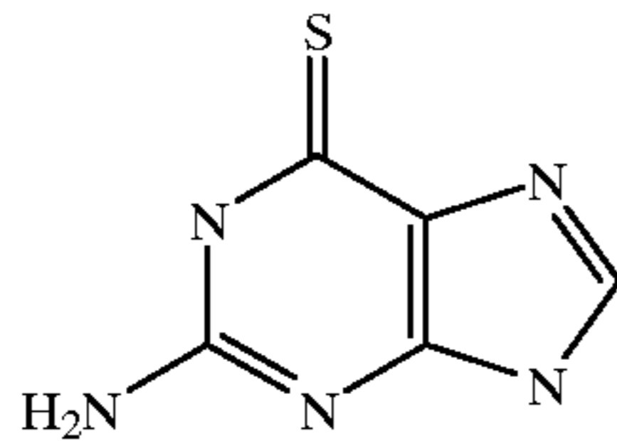
6-Thioguanine
