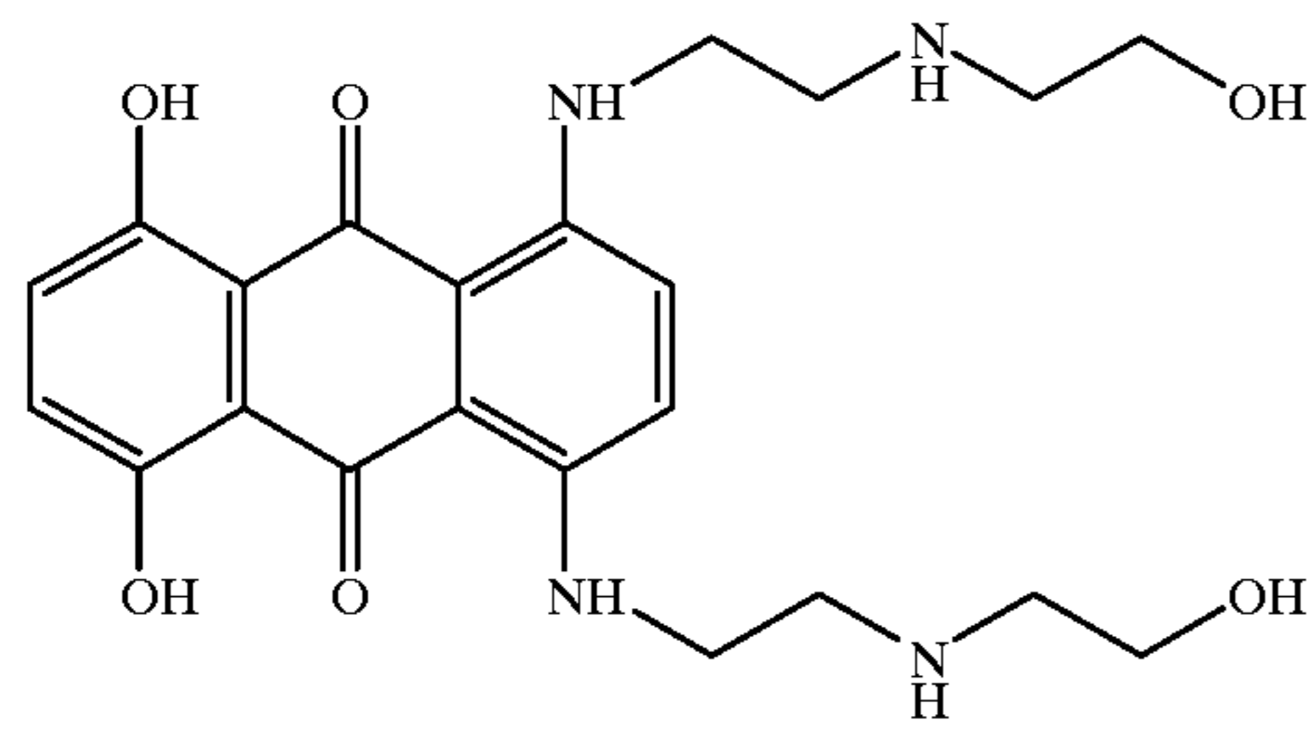
Mitoxantrone
