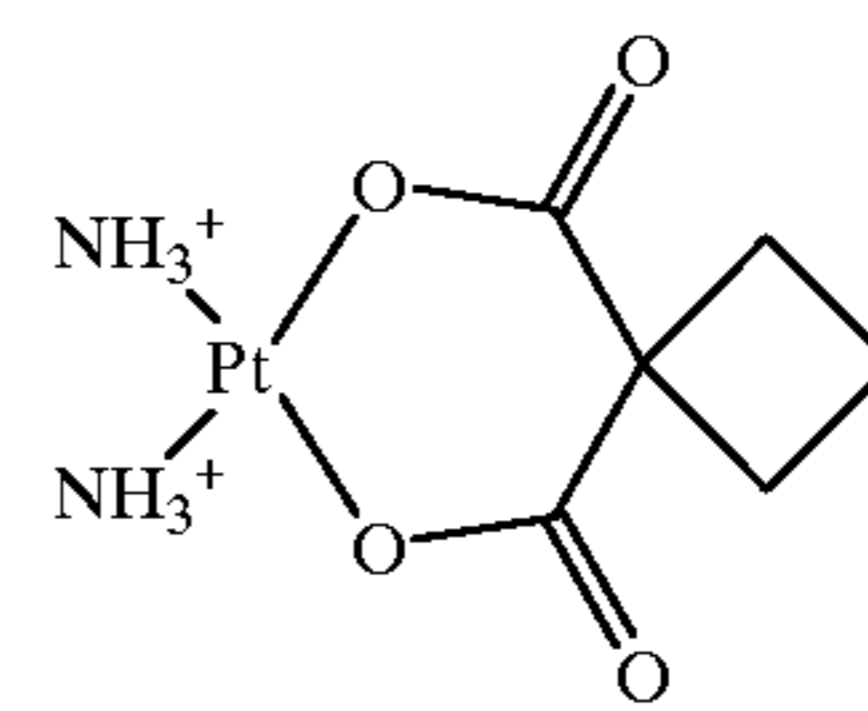
Carboplatin
