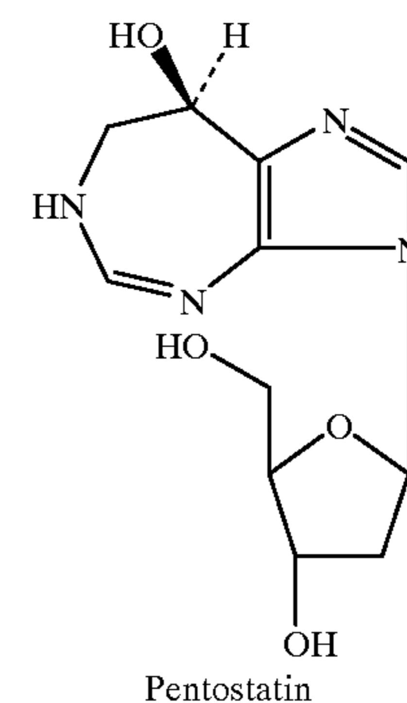
Pentostatin
