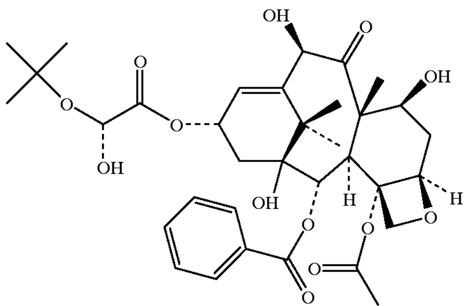
Taxotere
