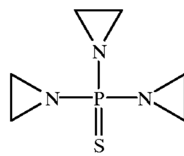
Thiotepa
