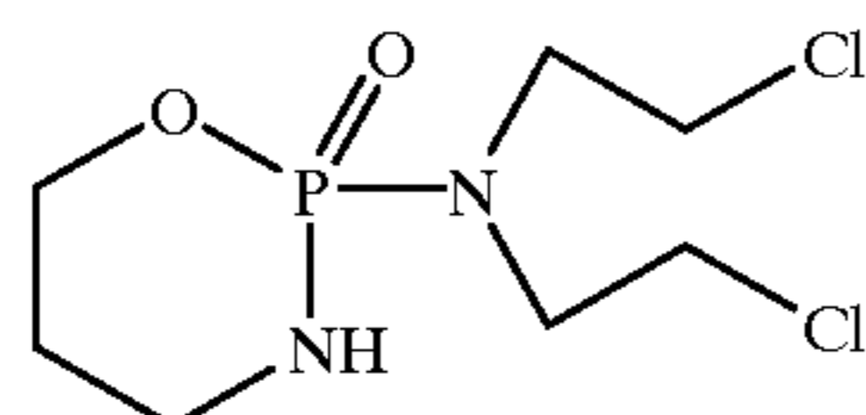
Cyclophosphamide
