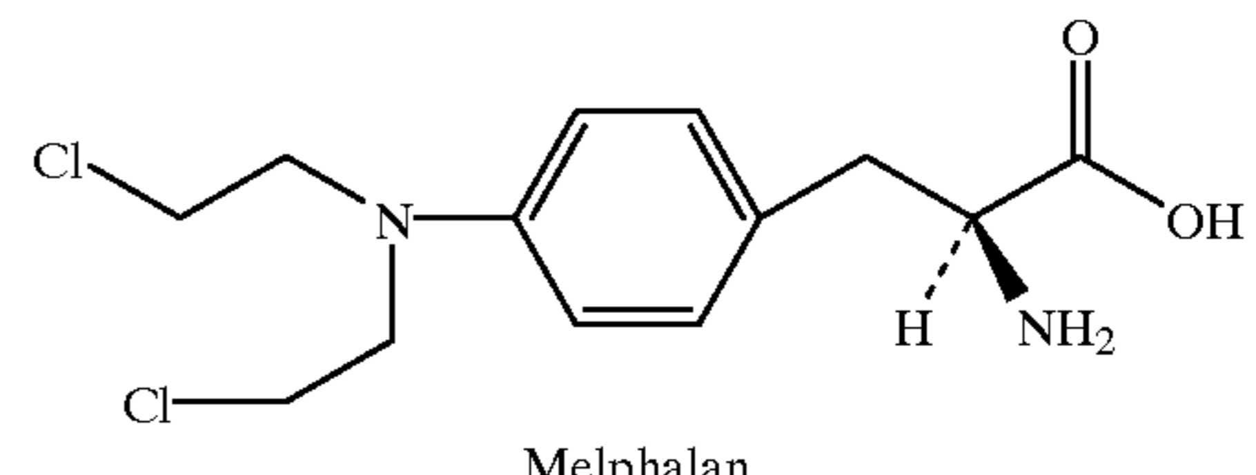
Melphalan
