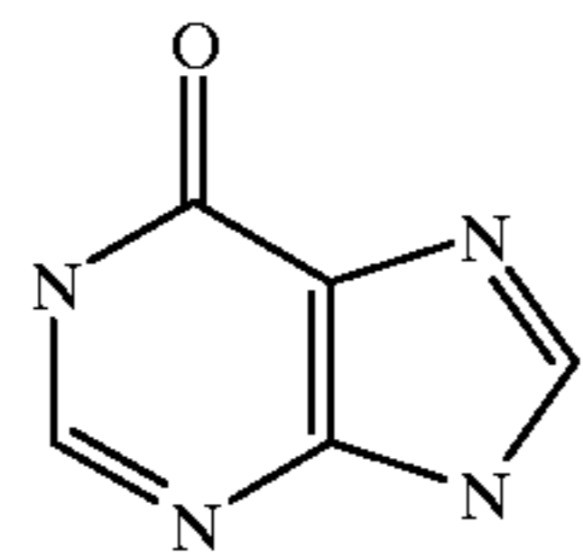
Hypoxanthine
