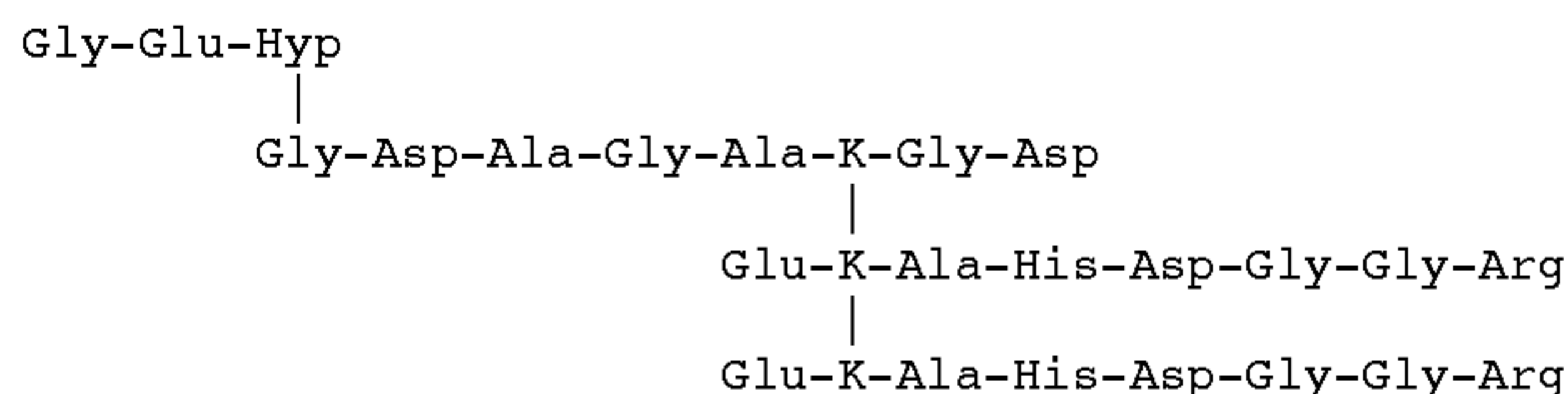
FORMULA V
