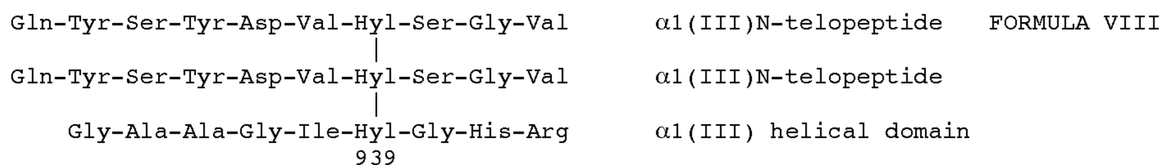
FORMULA IX
