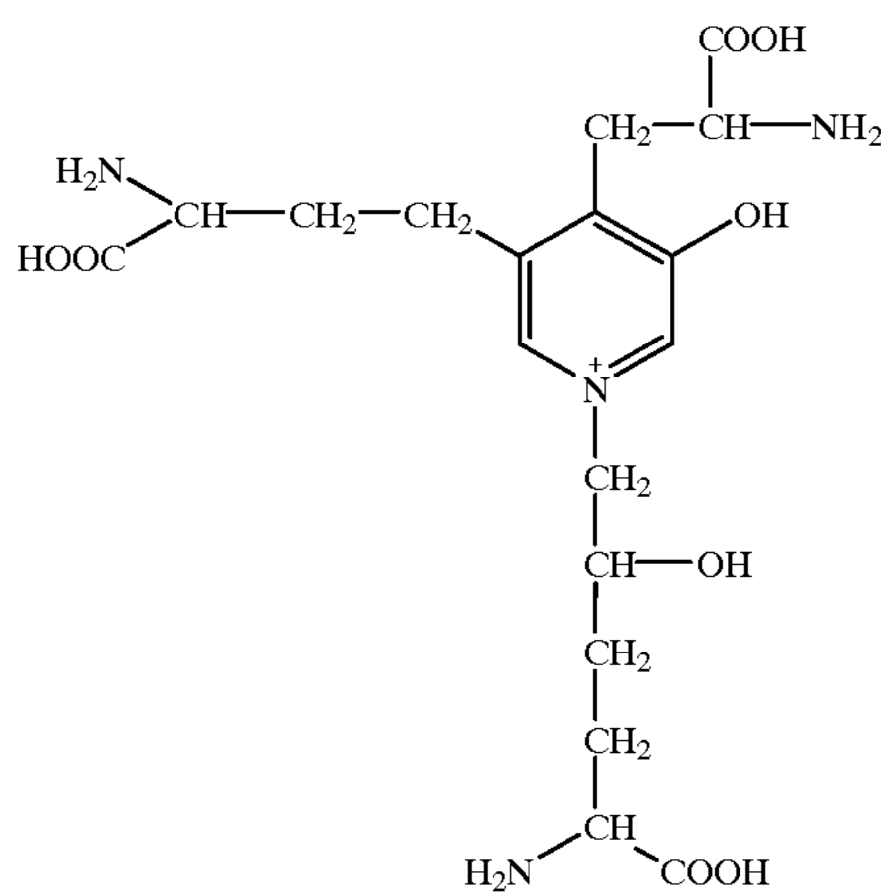
FORMULA II
