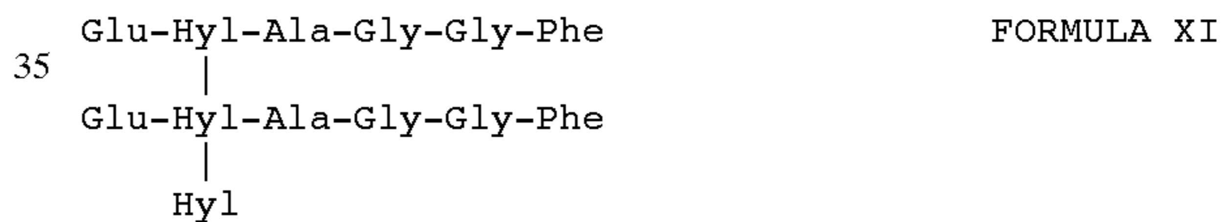
FORMULA XI
